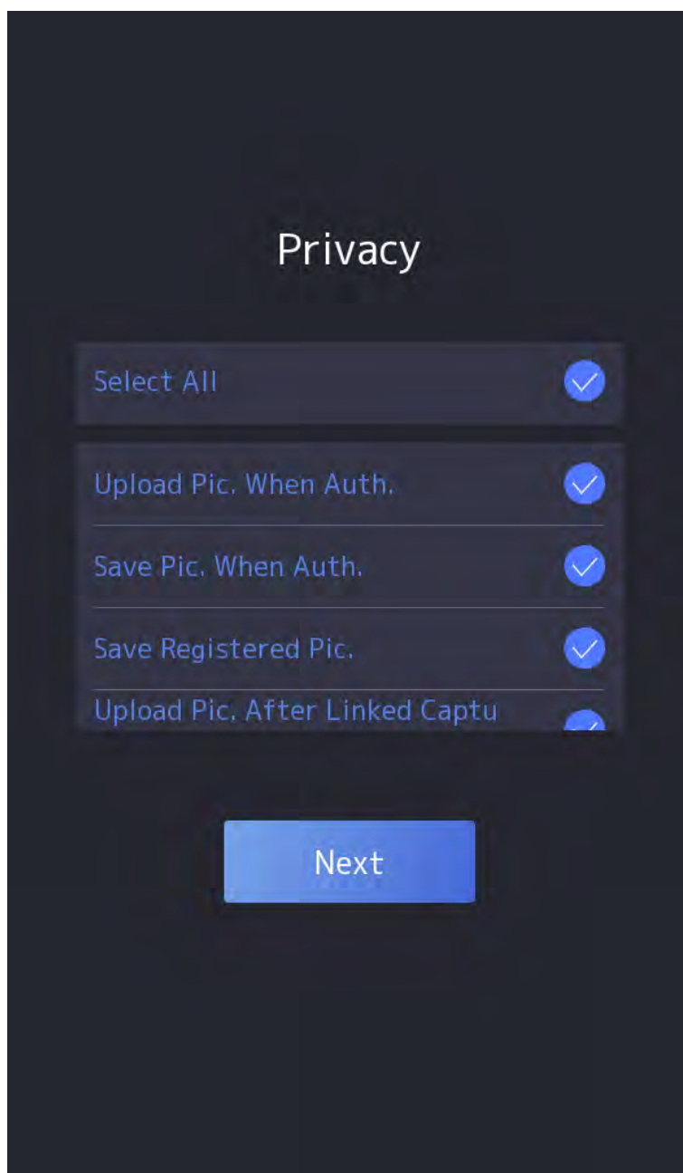
Figure 6-6 Privacy
