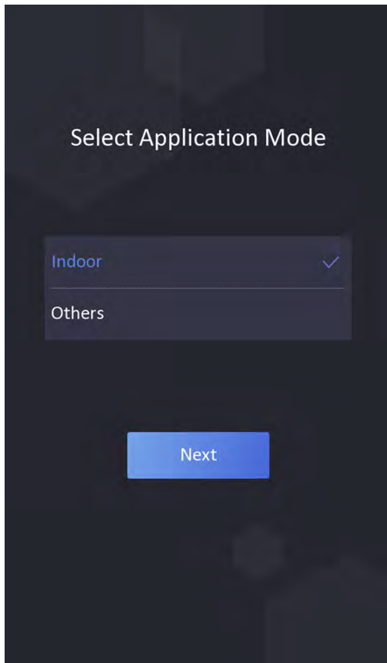
Figure 6-3 Welcome Page
