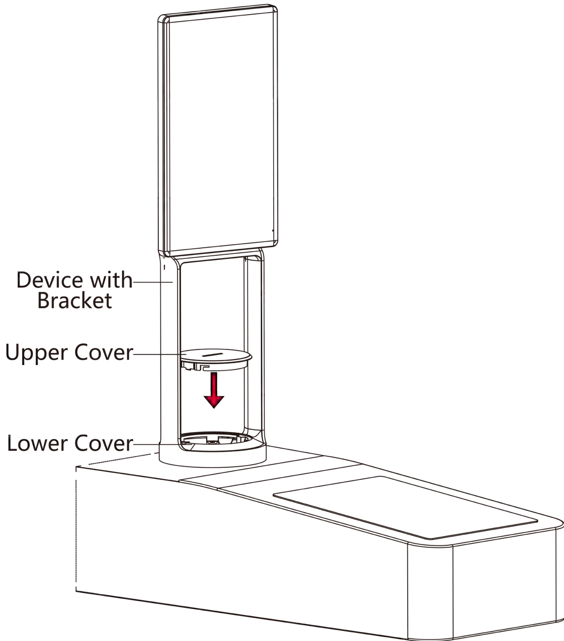
Figure 3-6 Secure Upper Cover
