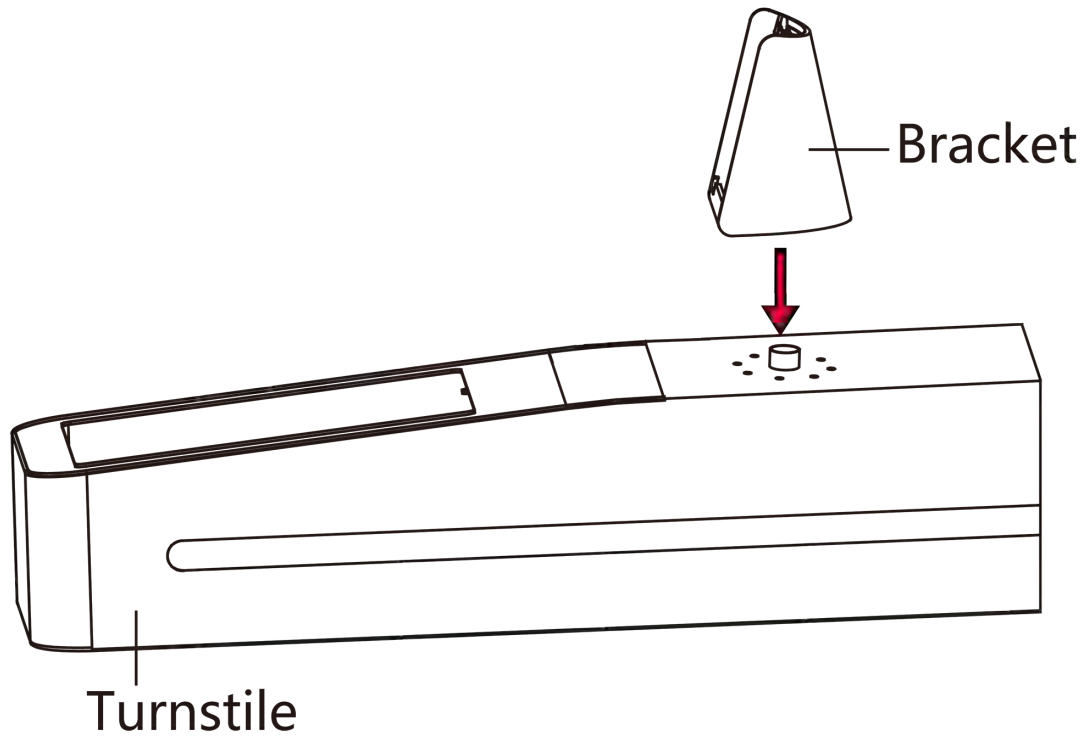
Figure 3-11 Install Bracket on Turnstile
