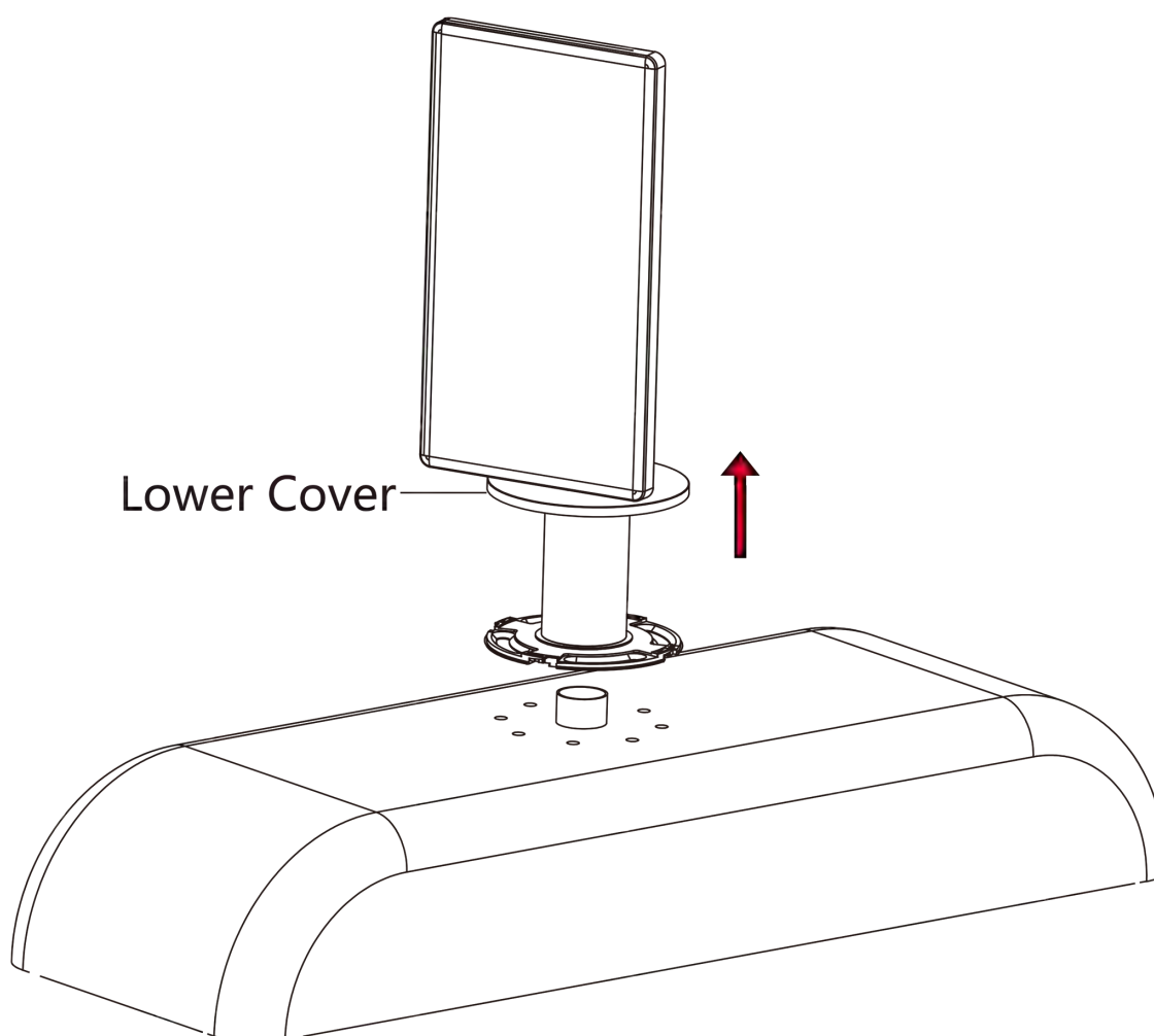
Figure 3-7 Remove Lower Cover
