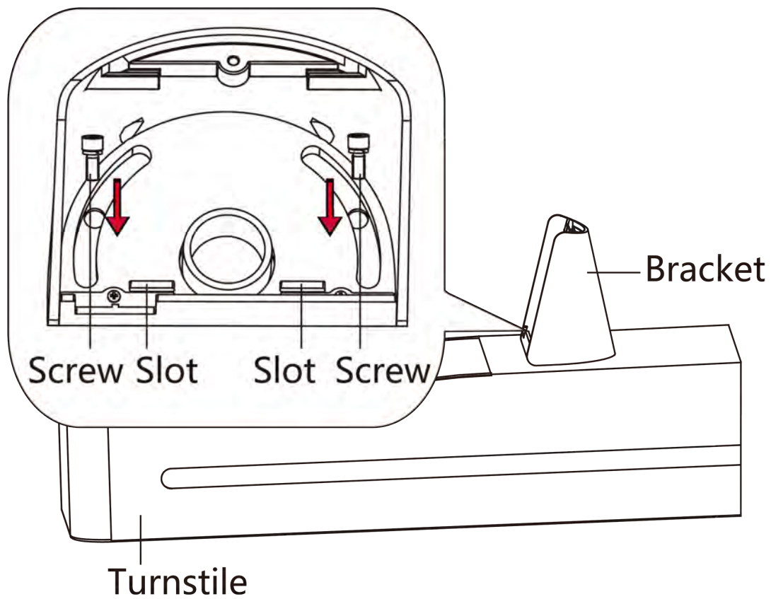
Figure 3-14 Secure Bracket
