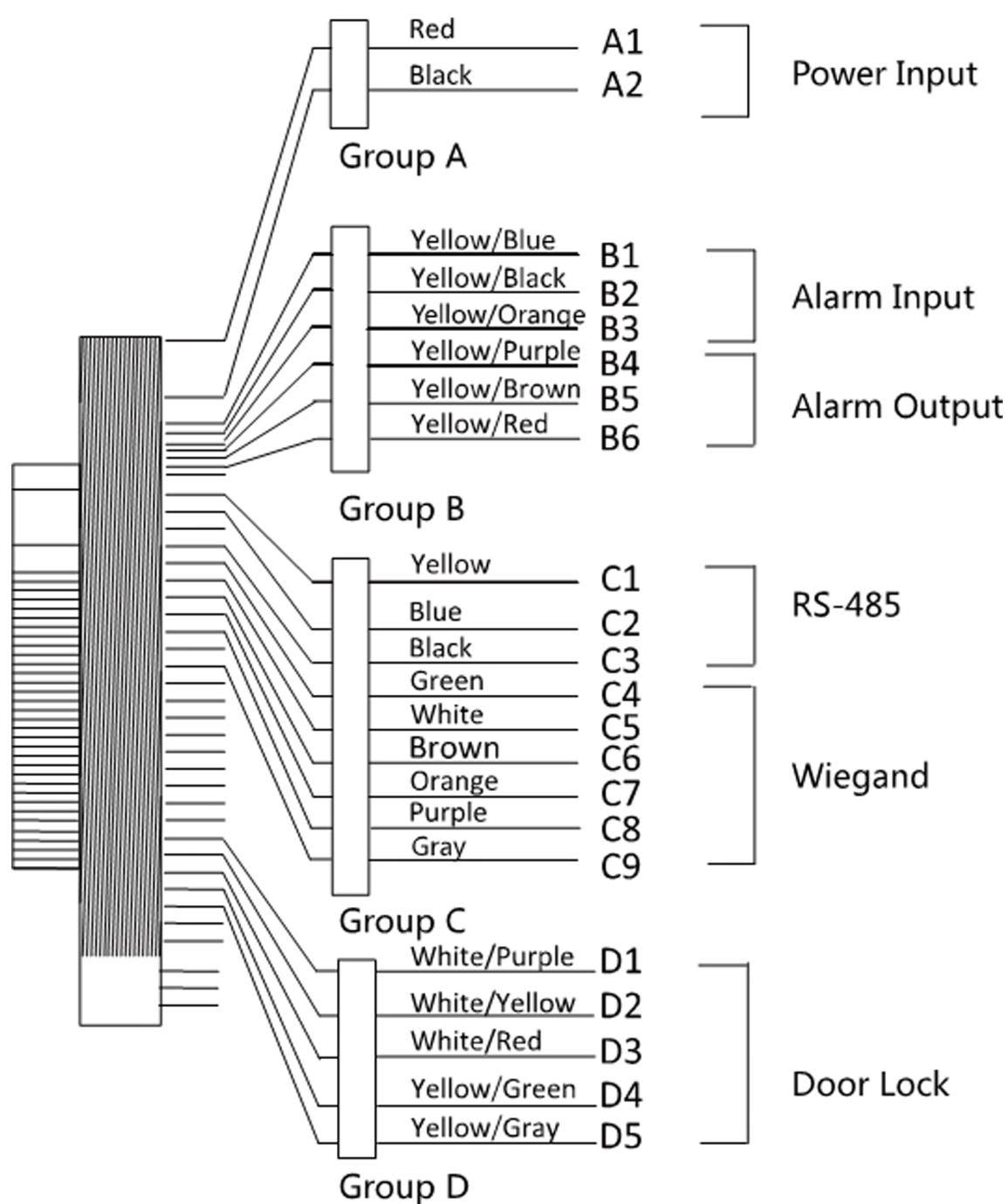
Figure 4-1 Terminal Diagram
