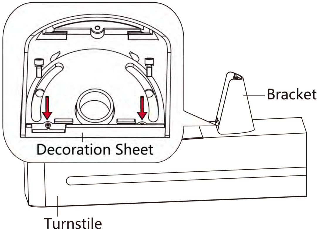
Figure 3-12 Remove Screws
