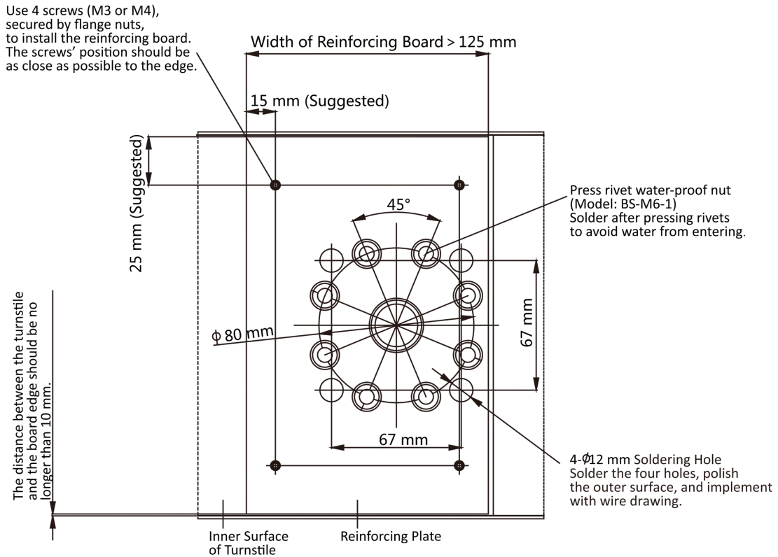
Figure 3-1 Drill Holes on Turnstile
