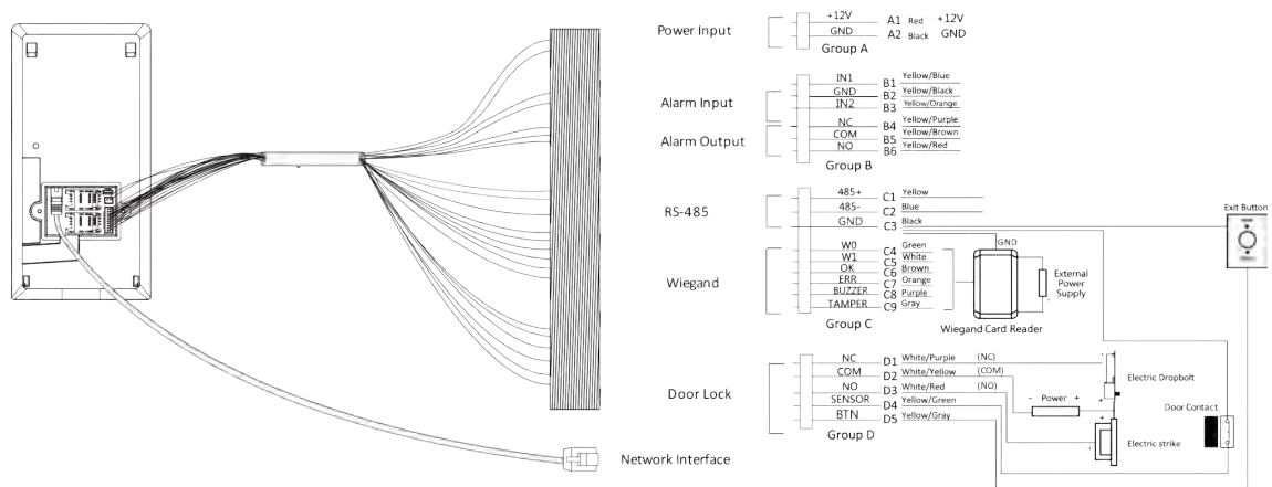
Figure 4-2 Device Wiring
