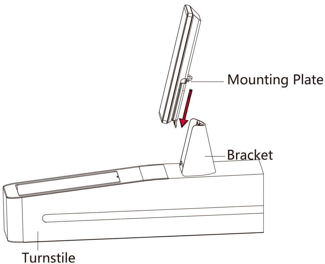
Figure 3-15 Install Device
