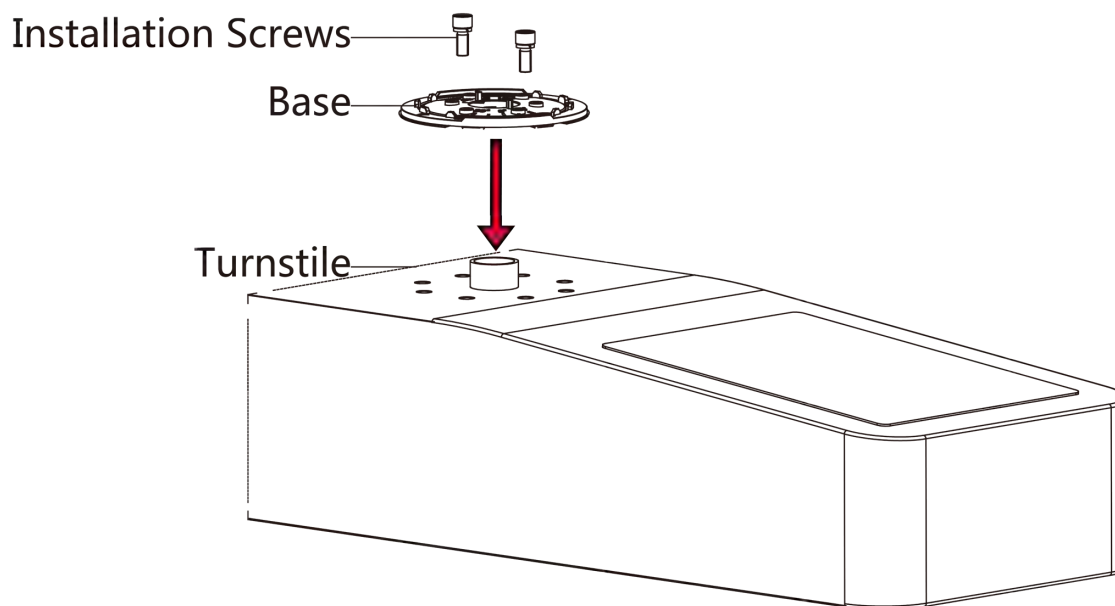
Figure 3-3 Install Base
