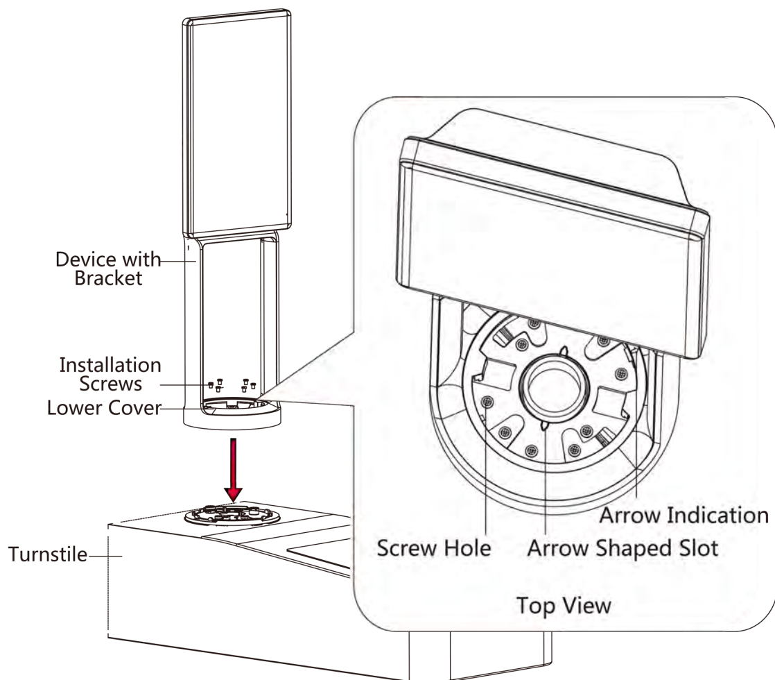
Figure 3-5 Secure Lower Cover and Turnstile
