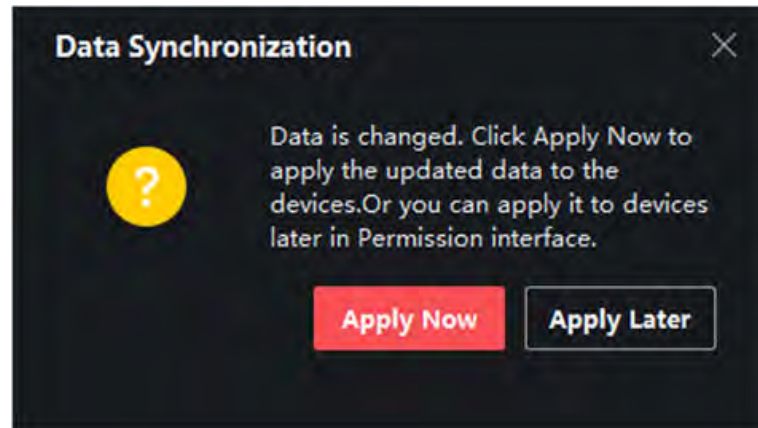
Figure 9-11 Data Synchronization
