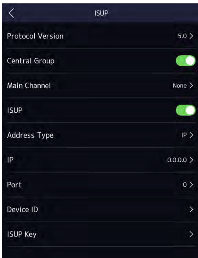
Figure 7-9 ISUP Settings
