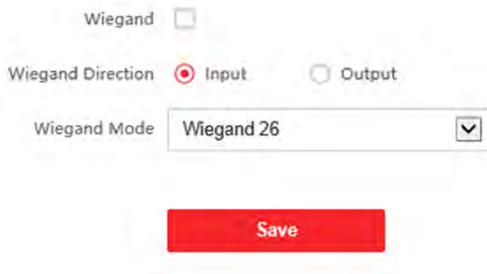
Figure 8-13 Wiegand Page
