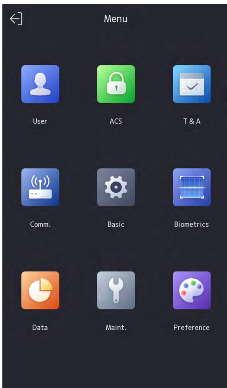
Figure 7-3 Home Page
