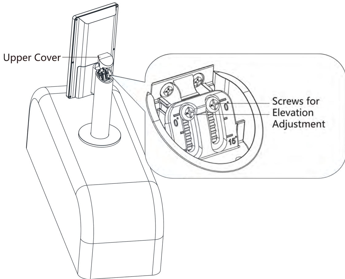
Figure 3-10 Adjust Elevation
