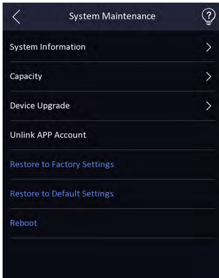
Figure 7-16 Maintenance Page
