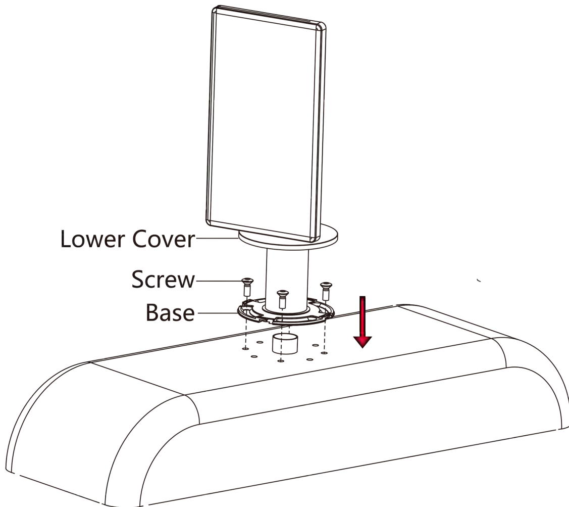
Figure 3-8 Secure Bracket and Turnstile
