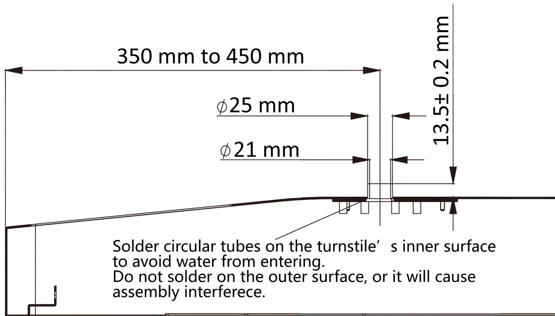
Figure 3-2 Solder Tubes
