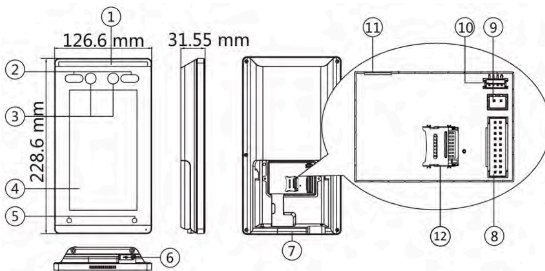
Figure 2-1 Face Recognition Terminal Diagram
