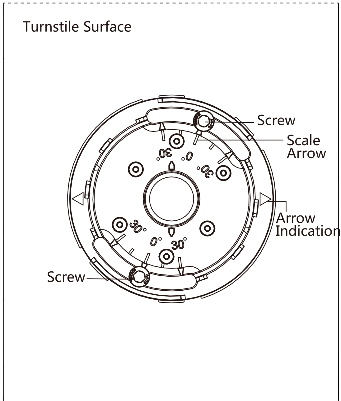
Figure 3-4 Screw Position
