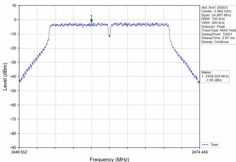
802.11g_HCH_2462MHz_Ant1 (SISO) NTN
