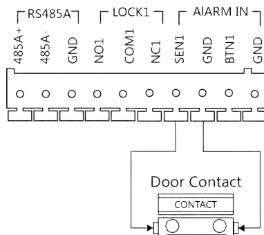
Figure 2-5 Door Contact Wiring
