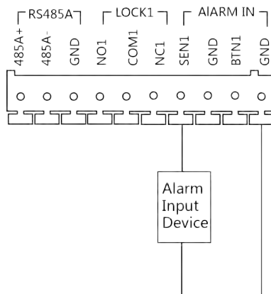
Figure 2-4 Alarm Input Device Wiring
