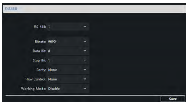
Figure 6-7 RS-485 Settings
