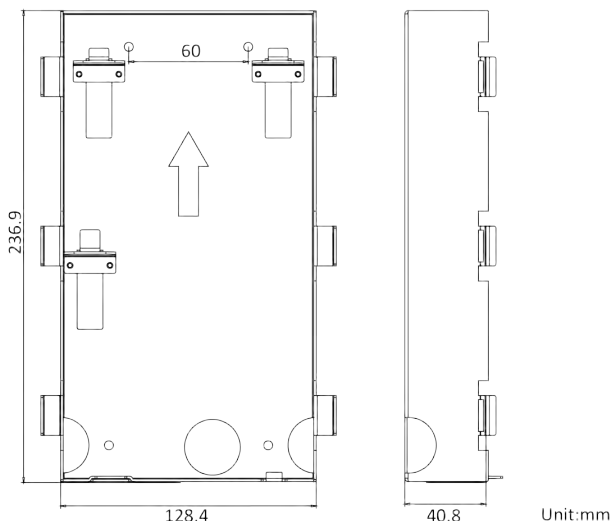
Figure 3-2 Gang Box
