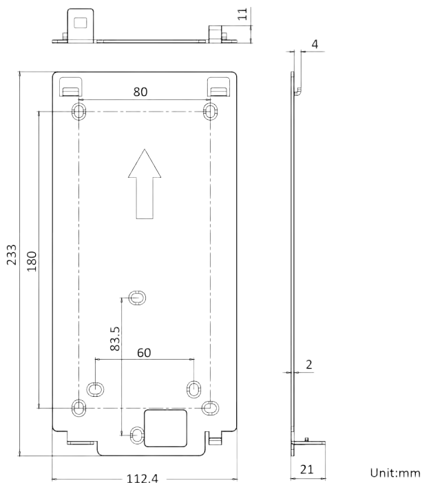
Figure 3-13 Mounting Plate
