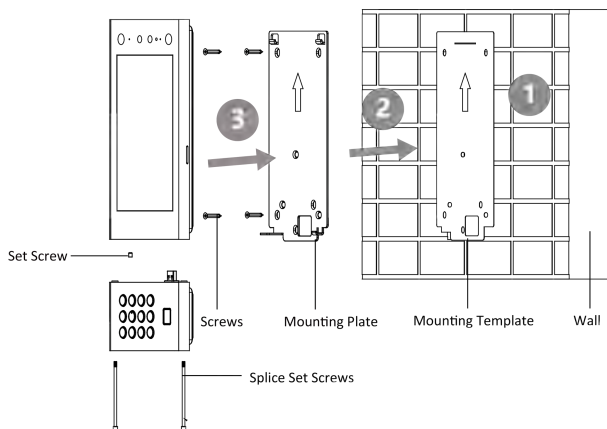
Figure 3-11 Surface Mounting
