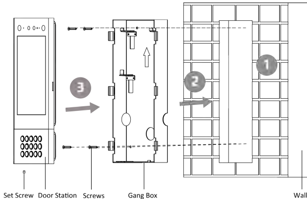
Figure 3-8 Flush Mounting
