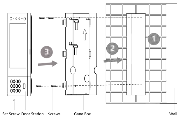
Figure 3-12 Flush Mounting
