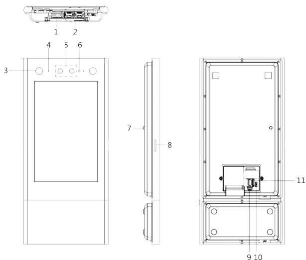
Figure 1-4 Door Station with 4G Module
