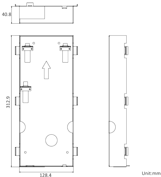
Figure 3-14 Gang Box
