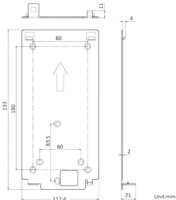
Figure 3-5 Mounting Plate
