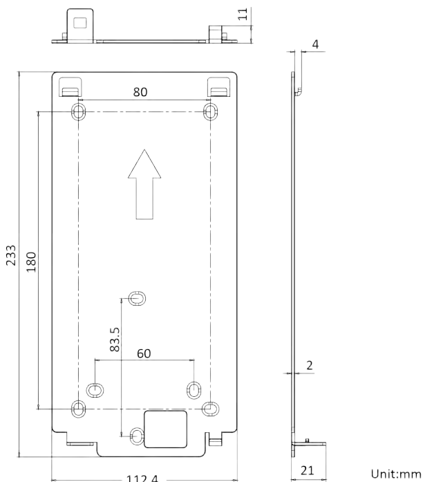
Figure 3-9 Mounting Plate
