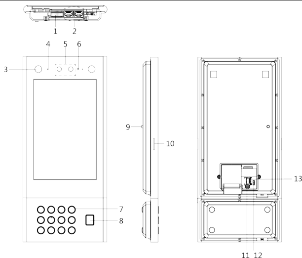
Figure 1-3 Door Station with Fingerprint Module
