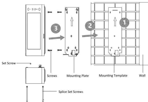
Figure 3-15 Surface Mounting
