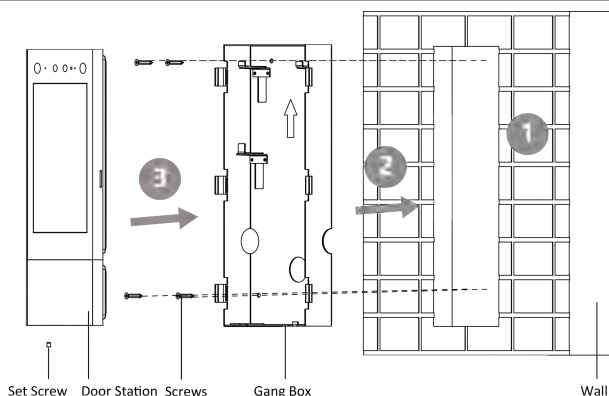
Figure 3-16 Flush Mounting
