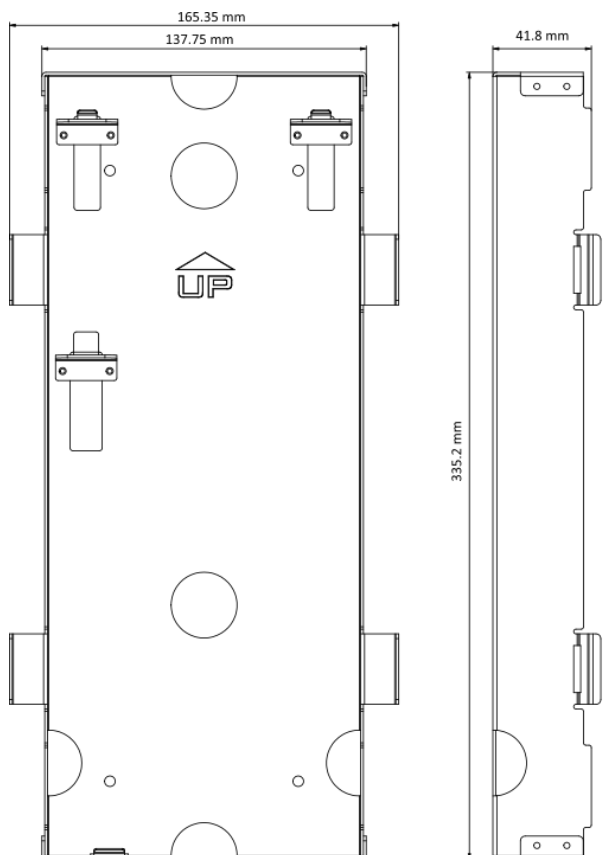
Figure 3-14 Gang Box
