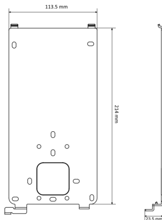
Figure 3-2 Mounting Plate
