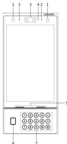
Figure 1-3 Front View
