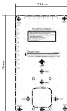
Figure 3-12 Mounting Template
