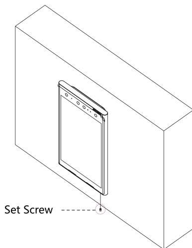
Figure 3-17 Fix Device
