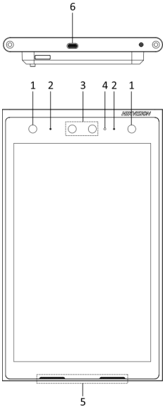
Figure 1-1 Front View
