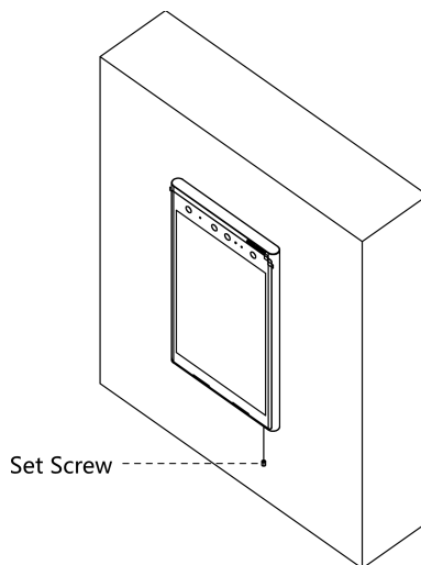
Figure 3-11 Fix Device
