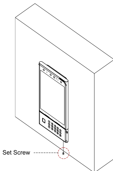
Figure 3-23 Fix Device
