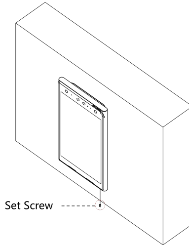
Figure 3-6 Fix Device
