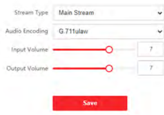
Figure 6-11 Audio Settings
