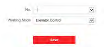
Figure 6-18 RS-485 Settings
