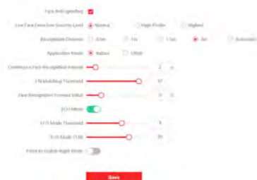
Figure 6-19 Smart Settings
