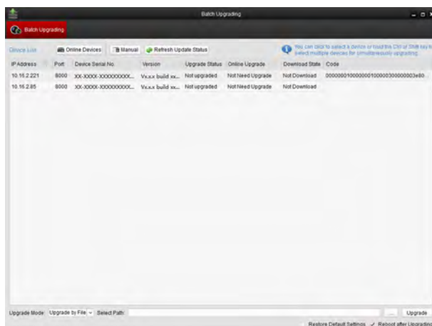
Figure 8-3 Batch Upgrading
