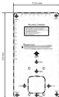
Figure 3-1 Mounting Template
