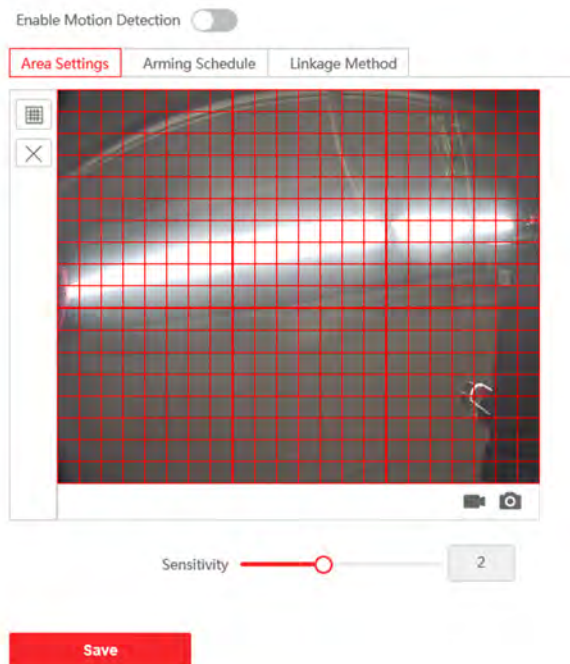
Figure 6-12 Motion Detection
