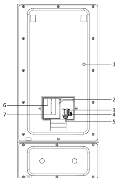
Figure 1-4 Rear View
