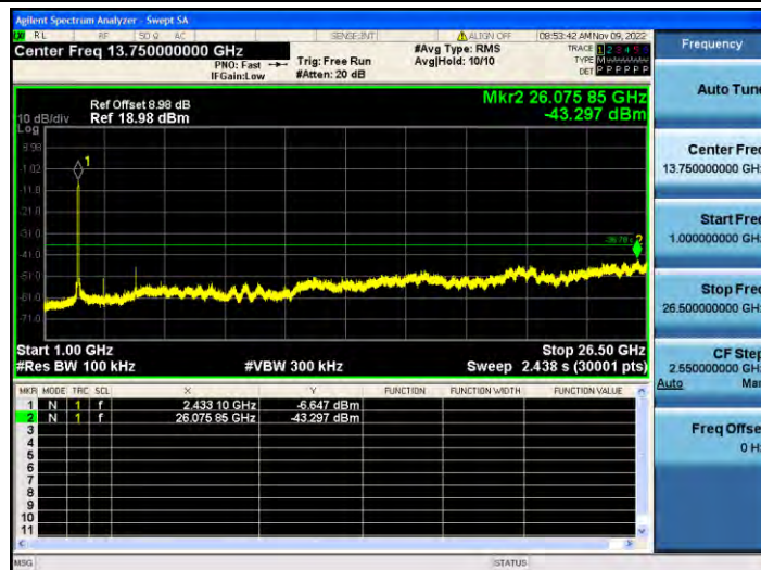
11N40SISO_Ant1_2452_0~Reference
