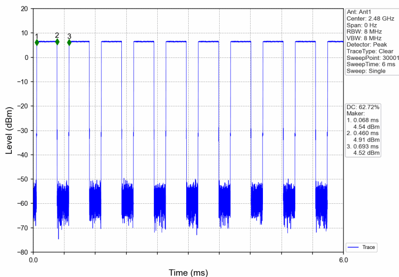
1M_HCH_2480MHz_DataRate= Ant1_NTNV
