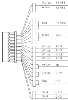
Figure 2-1 Terminal Description
