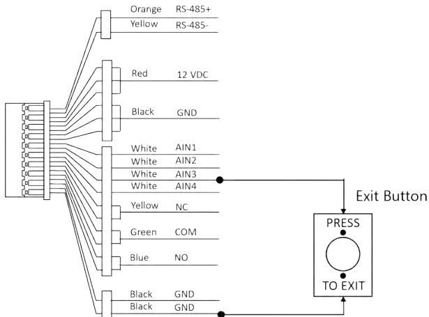
Figure 2-4 Exit Button Wiring
