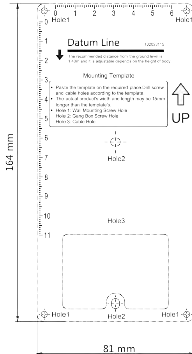
Figure 3-4 Mounting Template
