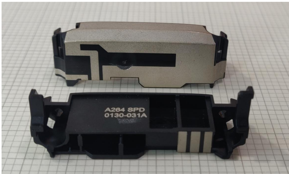
Figure 1 Antenna picture
