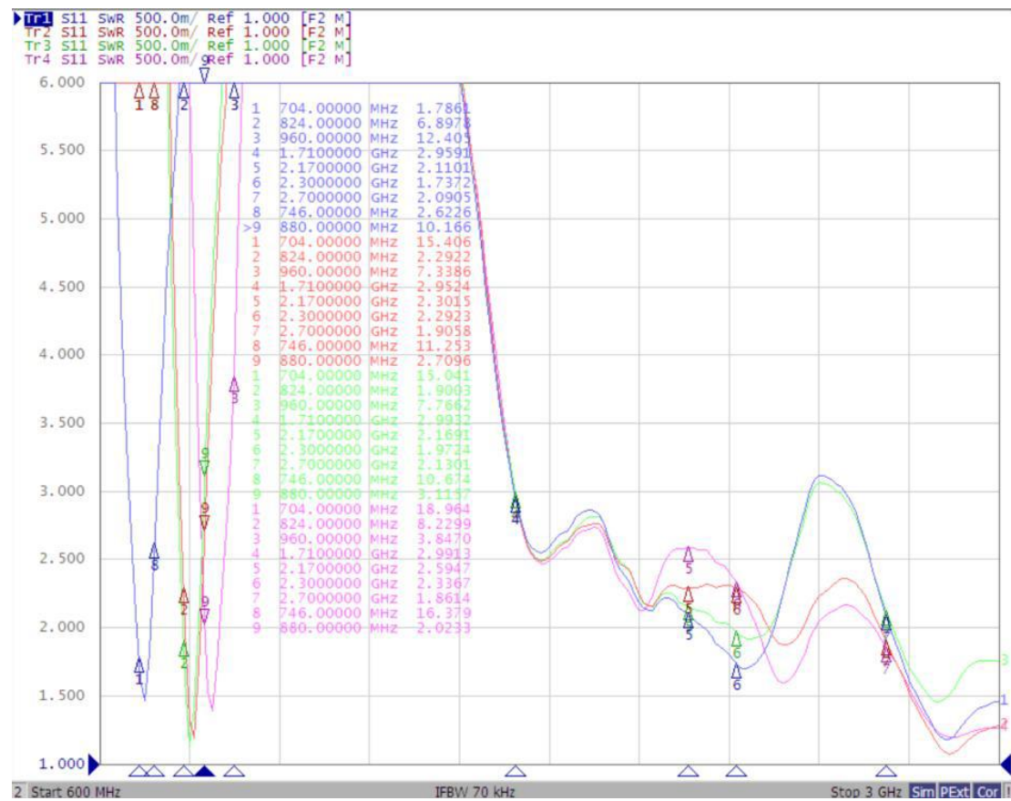
Figure 5 VSWR
