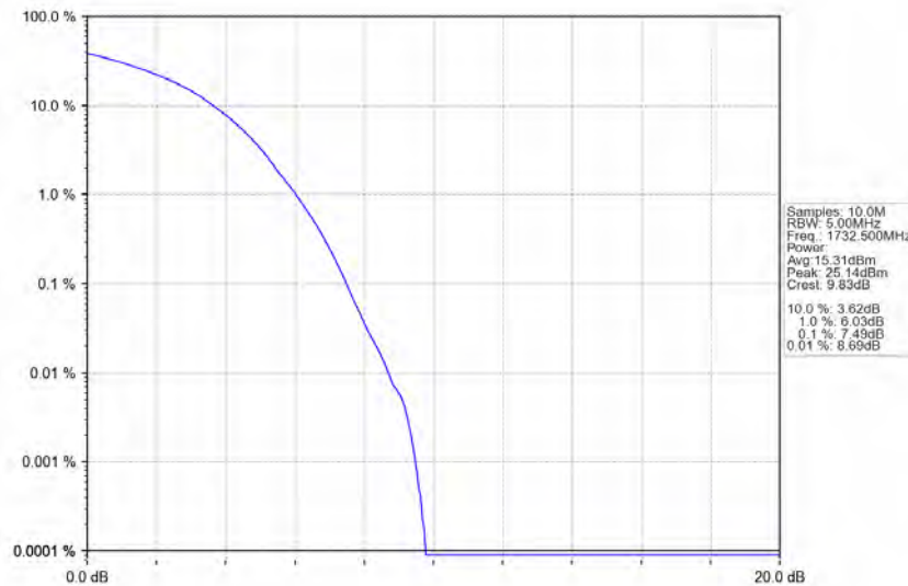
Band4_20MHz_64QAM_MCH_1732.5MHz_RB_100_0_NTNV
