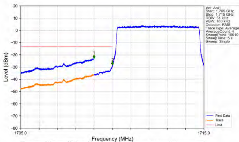
Band4_5MHz_QPSK_LCH_1712.5MHz_RB_25_0_NTNV
