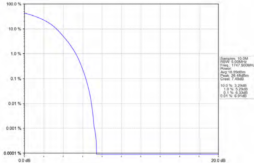
Band4_15MHz_QPSK_HCH_1747.5MHz_RB_75_0_NTNV
