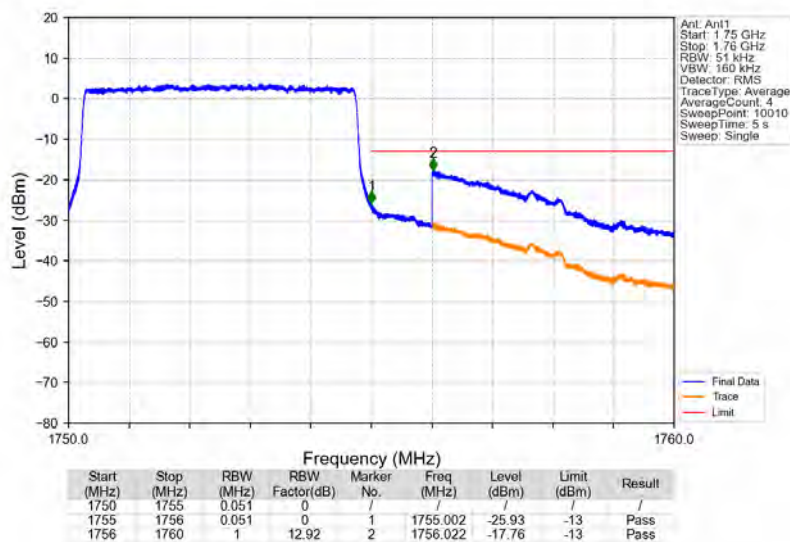
Band4_5MHz_QPSK_HCH_1752.5MHz_RB_25_0_NTNV
