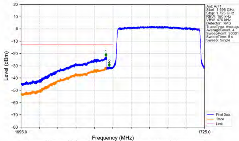
Band4_15MHz_16QAM_LCH_1717.5MHz_RB_75_0_NTNV
