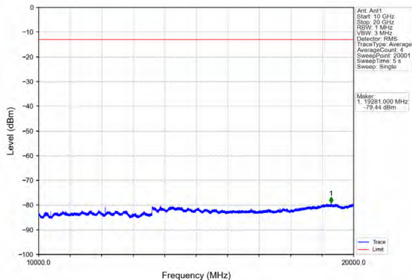
Band4_5MHz_QPSK_MCH_1732.5MHz_RB_1_0_NTNV
