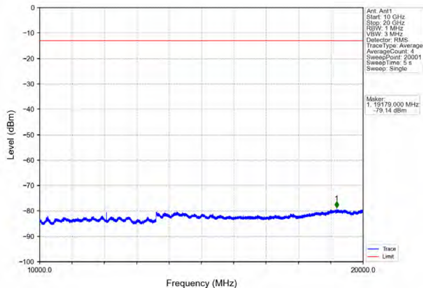
Band4_20MHz_16QAM_MCH_1732.5MHz_RB_1_0_NTNV
