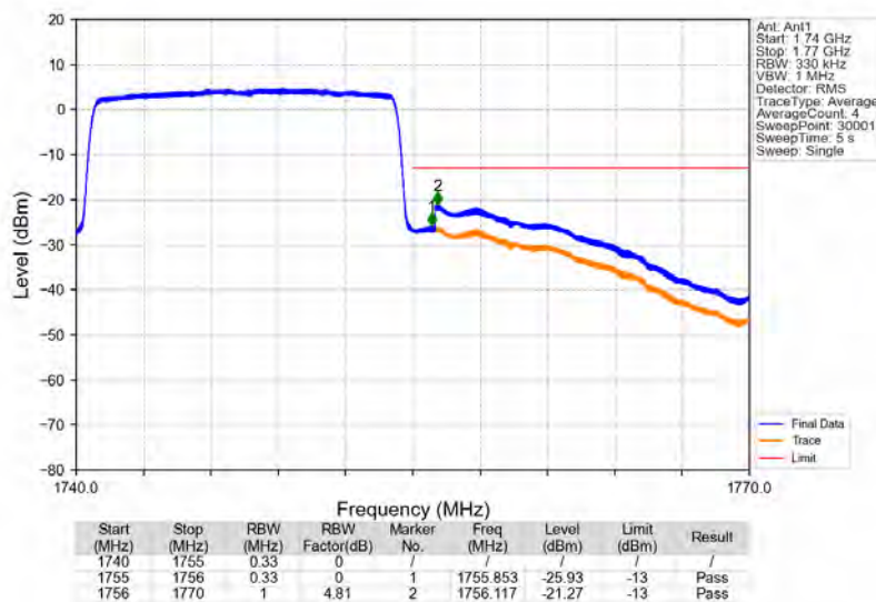
Band4_15MHz_16QAM_HCH_1747.5MHz_RB_75_0_NTNV
