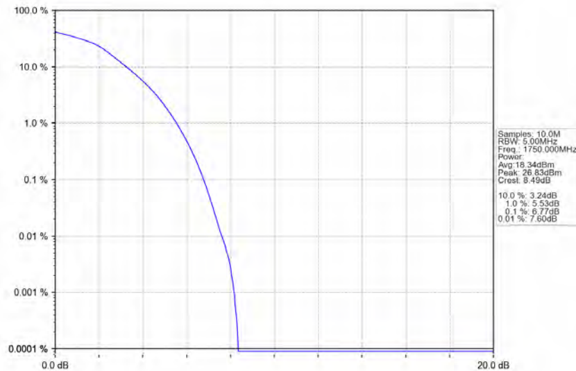
Band4_10MHz_64QAM_HCH_1750MHz_RB_50_0_NTNV
