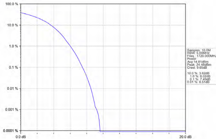
Band4_20MHz_64QAM_LCH_1720MHz_RB_100_0_NTNV
