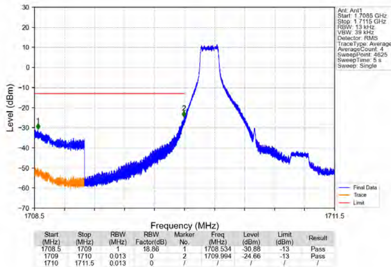
Band4_1.4MHz_64QAM_LCH_1710.7MHz_RB_1_0_NTNV
