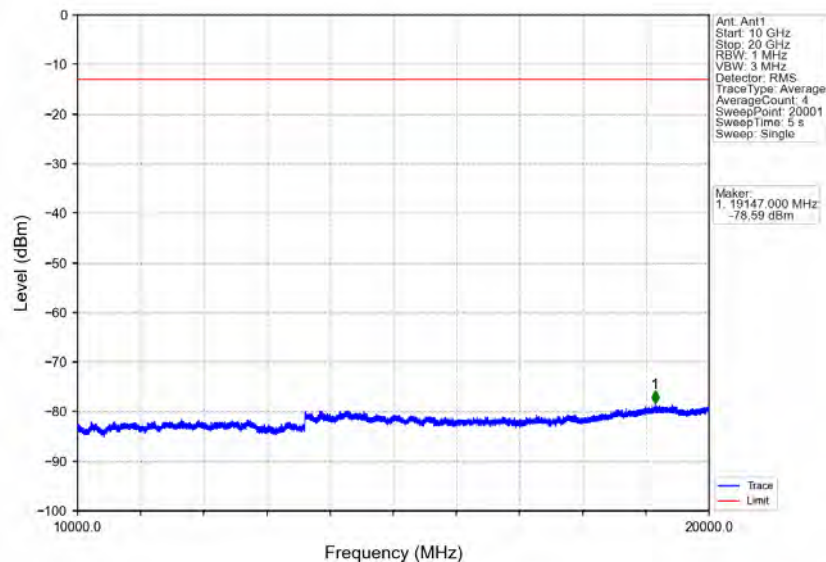
Band4_3MHz_64QAM_MCH_1732.5MHz_RB_1_0_NTNV
