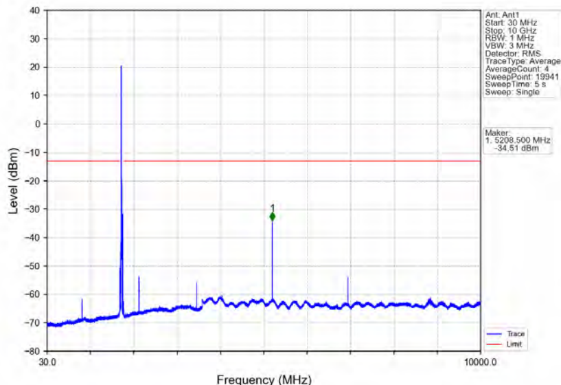
Band4 20MHz 16QAM HCH 1745MHz RB 1 0 NTNV
