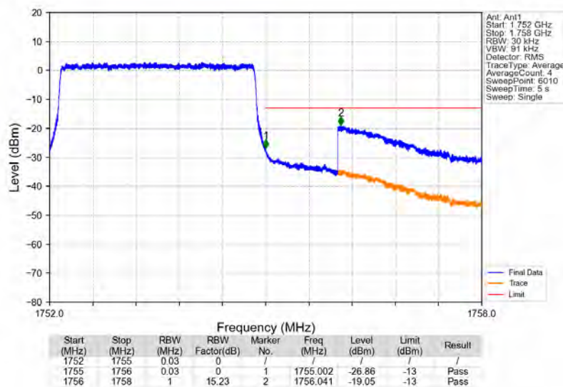
Band4_3MHz_16QAM_HCH_1753.5MHz_RB_15_0_NTNV
