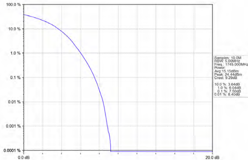
Band4_20MHz_64QAM_HCH_1745MHz_RB_100_0_NTNV
