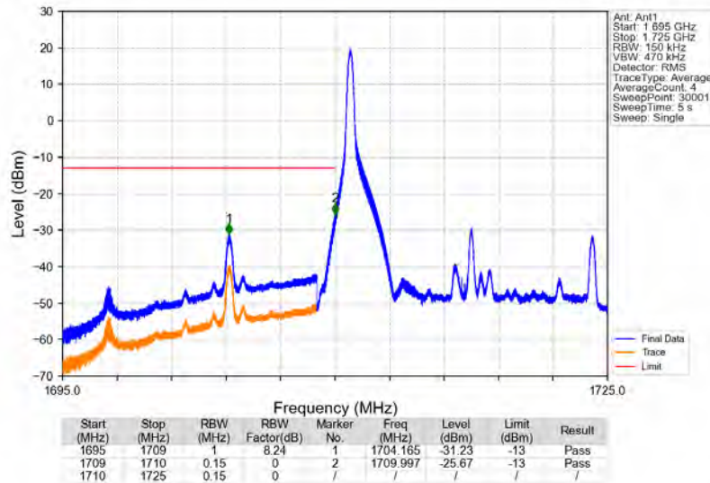
Band4_15MHz_64QAM_LCH_1717.5MHz_RB_1_0_NTNV
