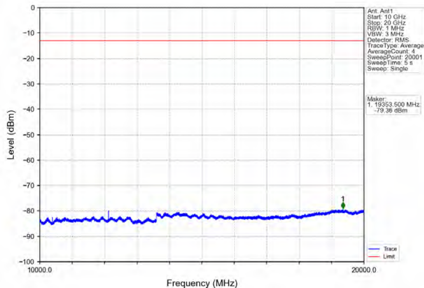
Band4_3MHz_QPSK_MCH_1732.5MHz_RB_1_0_NTNV
