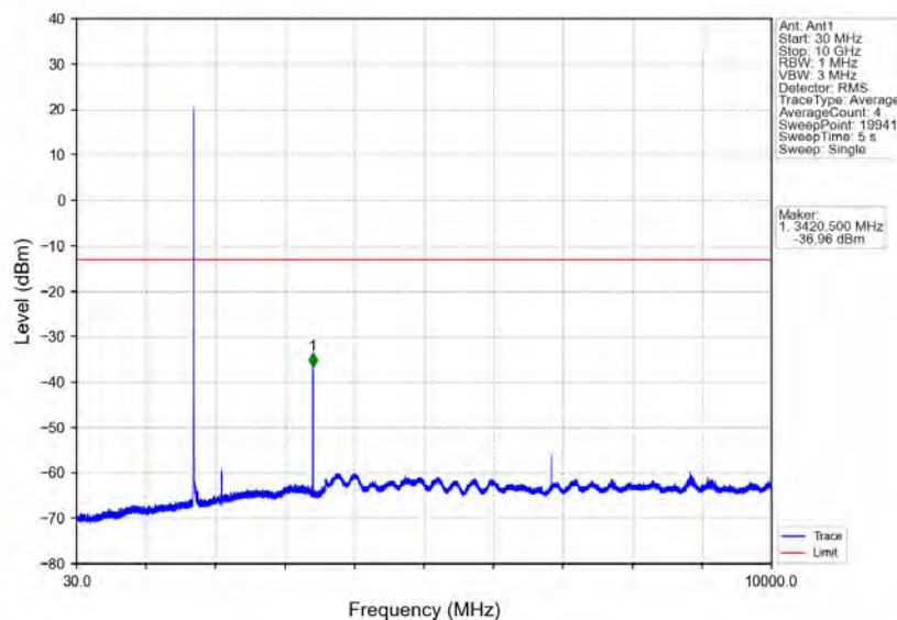
Band4_1.4MHz_64QAM_LCH_1710.7MHz_RB_1_0_NTNV
