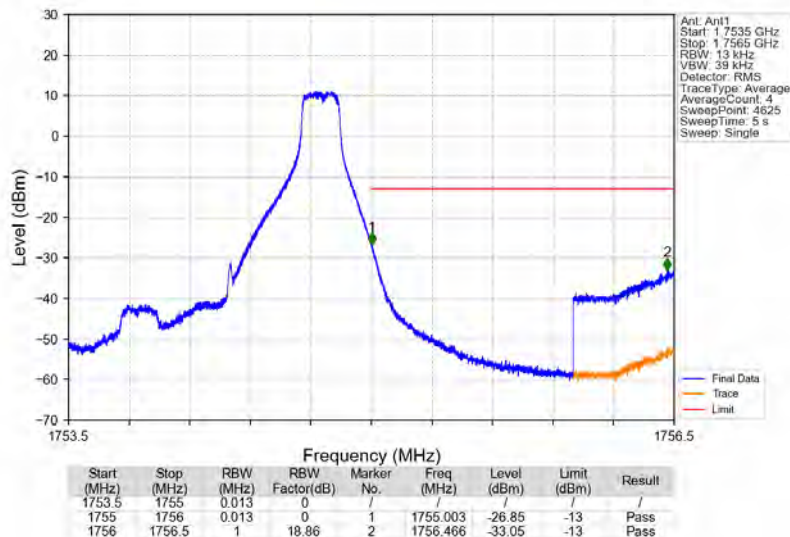
Band4_1.4MHz_64QAM_HCH_1754.3MHz_RB_1_5_NTNV
