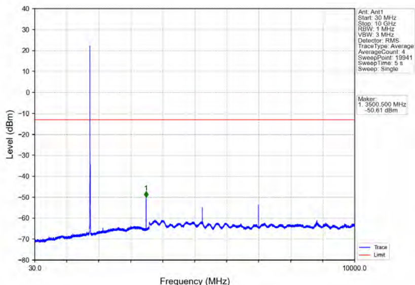
Band4_5MHz_QPSK_HCH_1752.5MHz_RB_1_0_NTNV
