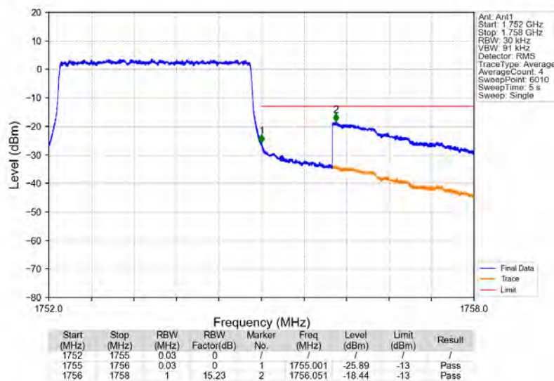
Band4_3MHz_QPSK_HCH_1753.5MHz_RB_15_0_NTNV
