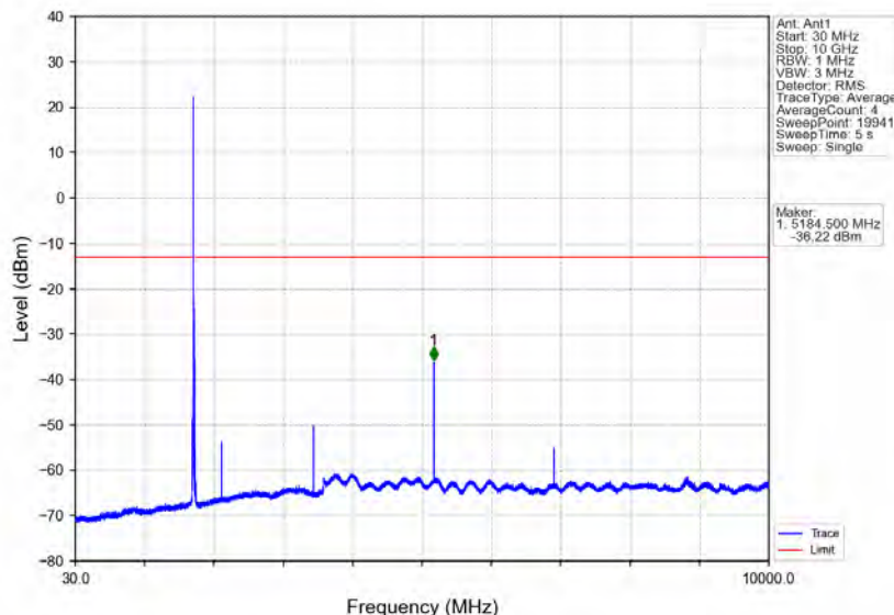
Band4_10MHz_QPSK_MCH_1732.5MHz_RB_1_0_NTNV
