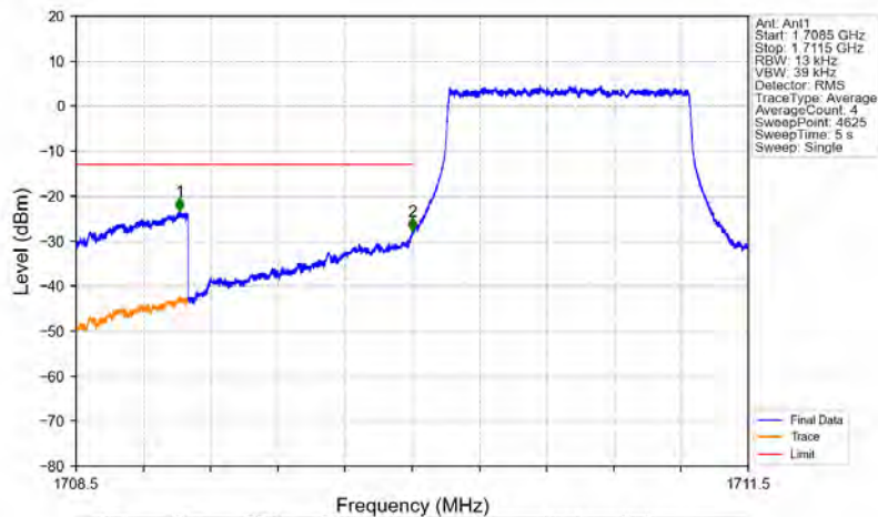
Band4_1.4MHz_16QAM_LCH_1710.7MHz_RB_6_0_NTNV
