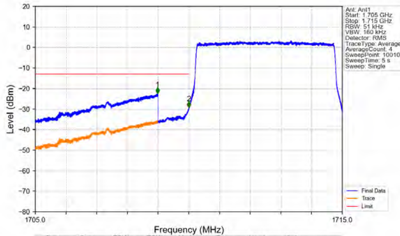
Band4_5MHz_16QAM_LCH_1712.5MHz_RB_25_0_NTNV
