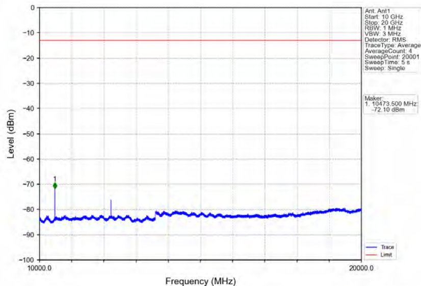
Band4 10MHz 16QAM HCH 1750MHz RB 1 0 NTNV
