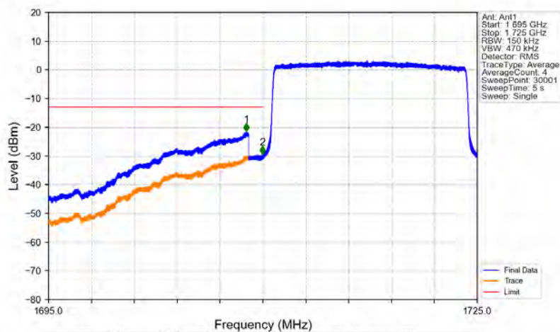
Band4_15MHz_QPSK_LCH_1717.5MHz_RB_75_0_NTNV
