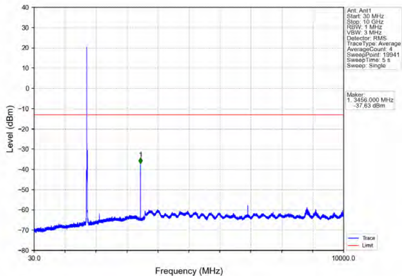
Band4_10MHz_64QAM_MCH_1732.5MHz_RB_1_0_NTNV
