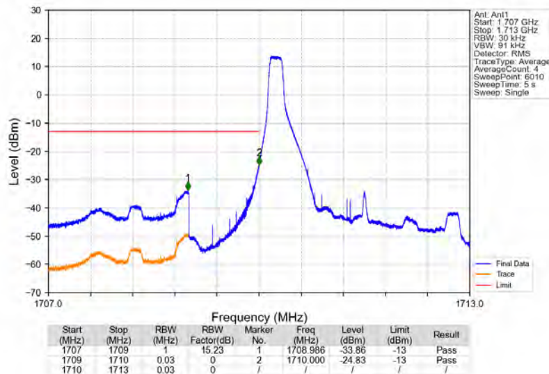
Band4_3MHz_64QAM_LCH_1711.5MHz_RB_1_0_NTNV
