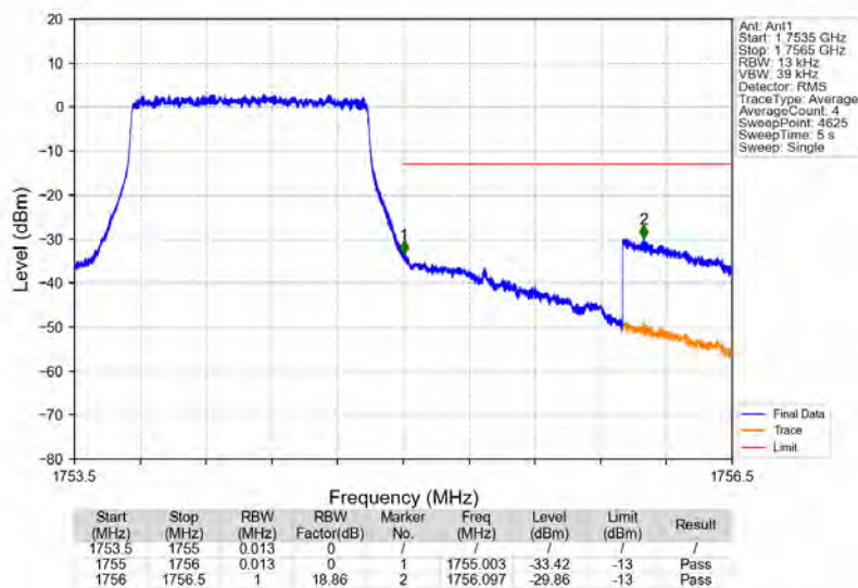
Band4_1.4MHz_64QAM_HCH_1754.3MHz_RB_6_0_NTNV
