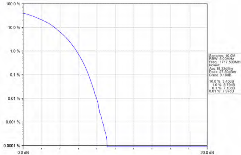
Band4_15MHz_16QAM_LCH_1717.5MHz_RB_75_0_NTNV
