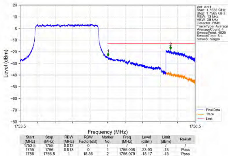
Band4_1.4MHz_16QAM_HCH_1754.3MHz_RB_6_0_NTNV
