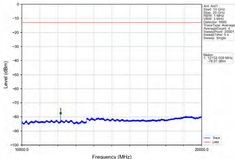
Band4 20MHz 16QAM HCH 1745MHz RB 1 0 NTNV
