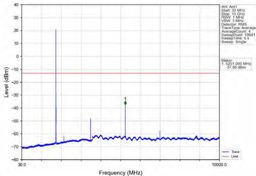
Band4_5MHz_16QAM_HCH_1752.5MHz_RB_1_0_NTNV
