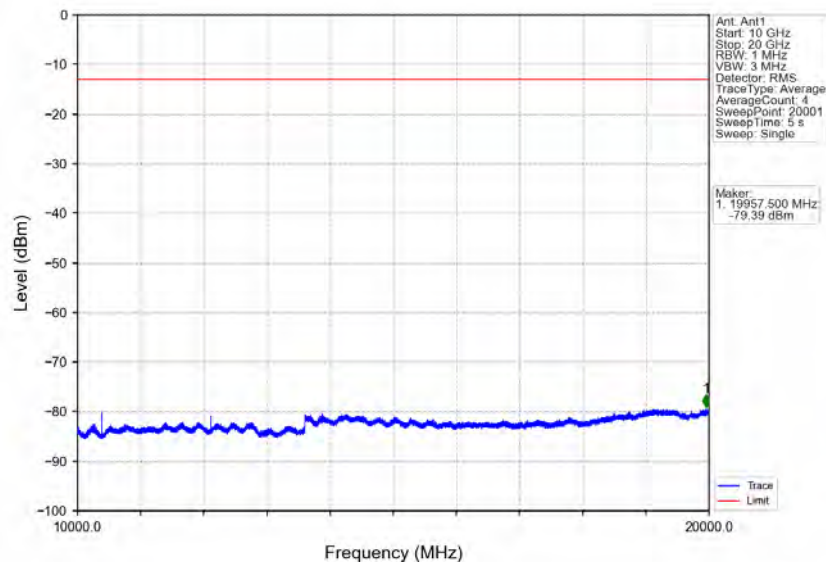
Band4_5MHz_16QAM_MCH_1732.5MHz_RB_1_0_NTNV
