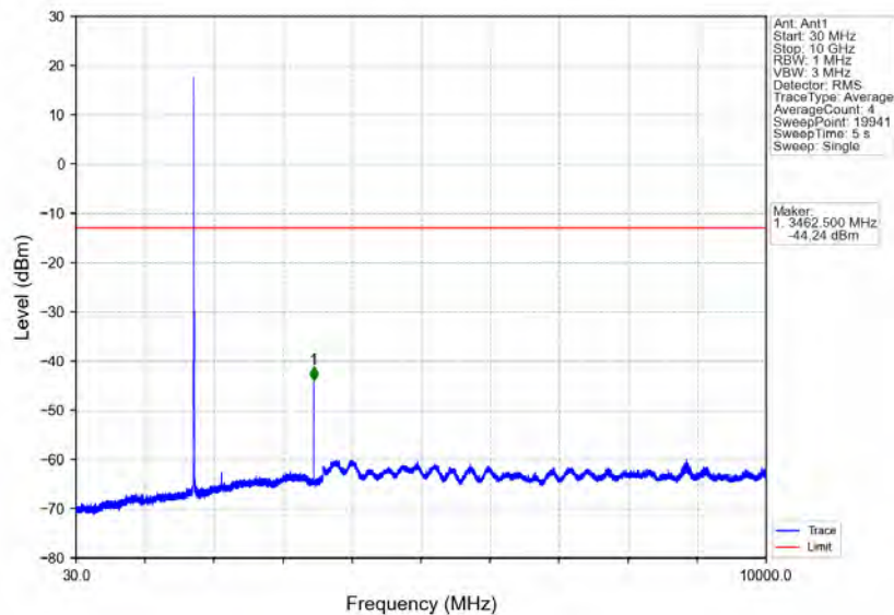
Band4_3MHz_64QAM_MCH_1732.5MHz_RB_1_0_NTNV
