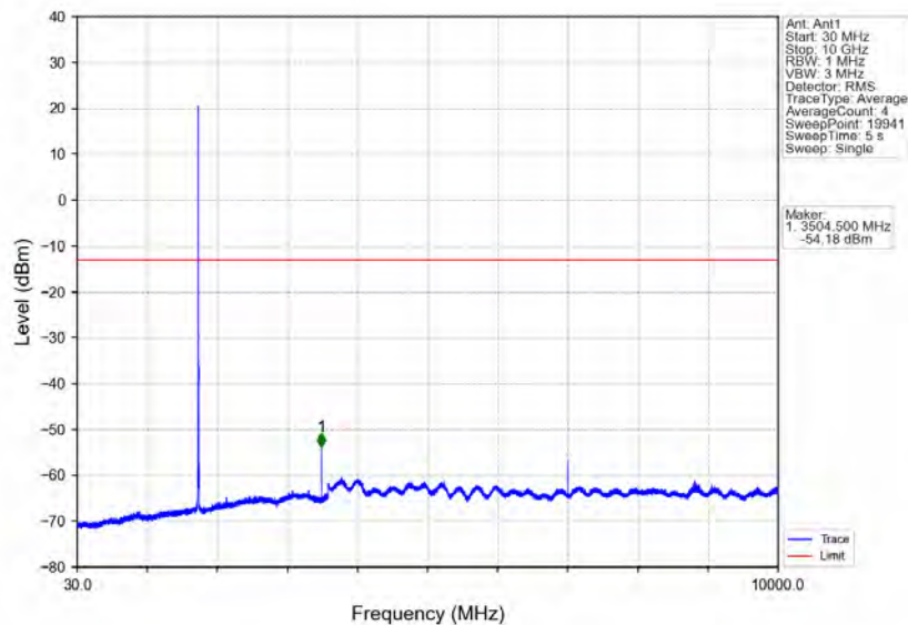
Band4_3MHz_16QAM_HCH_1753.5MHz_RB_1_0_NTNV
