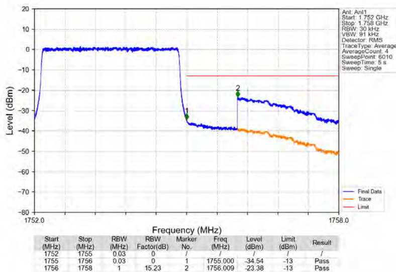
Band4_3MHz_64QAM_HCH_1753.5MHz_RB_15_0_NTNV
