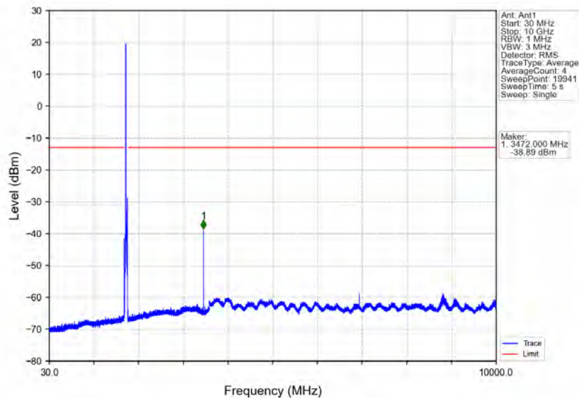
Band4 20MHz 64QAM HCH 1745MHz RB 1 0 NTNV
