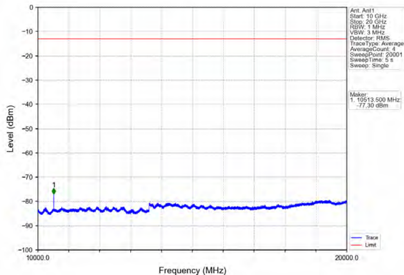
Band4_3MHz_16QAM_HCH_1753.5MHz_RB_1_0_NTNV
