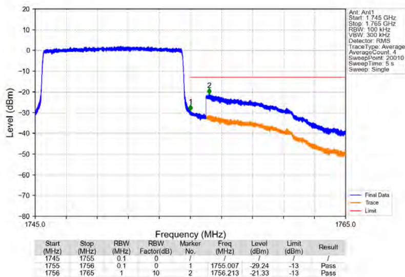
Band4_10MHz_16QAM_HCH_1750MHz_RB_50_0_NTNV
