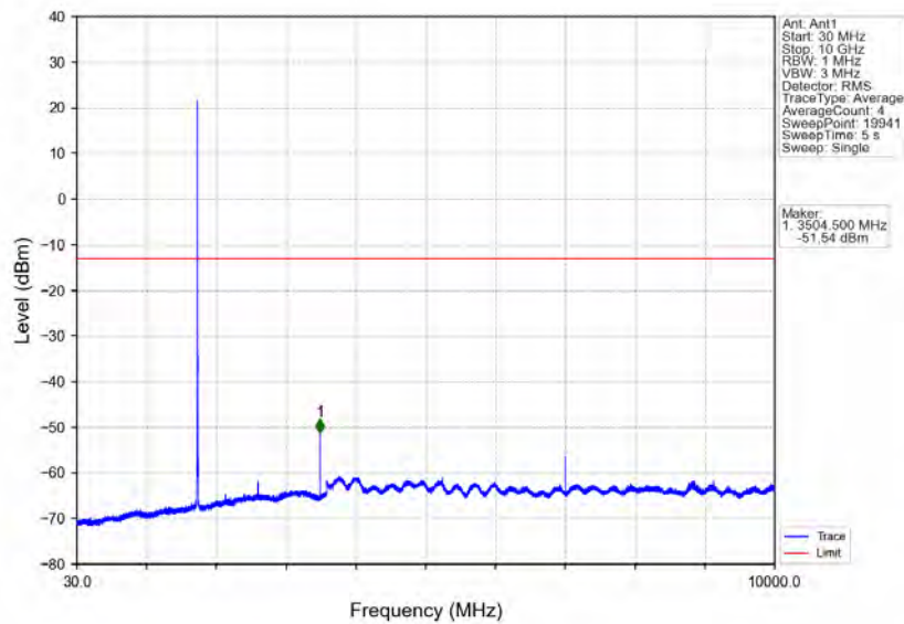
Band4_3MHz_QPSK_HCH_1753.5MHz_RB_1_0_NTNV
