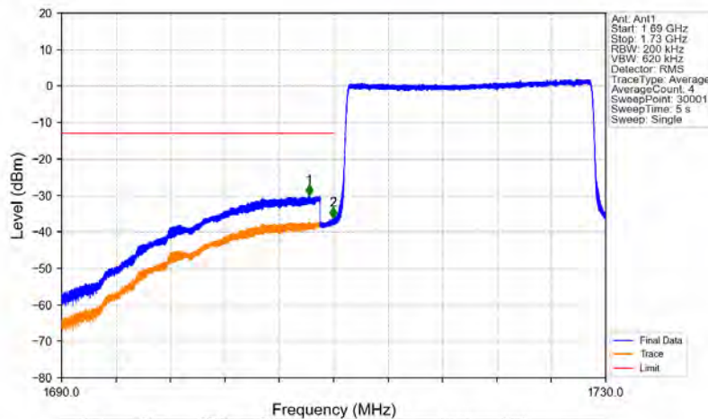
Band4_20MHz_64QAM_LCH_1720MHz_RB_100_0_NTNV
