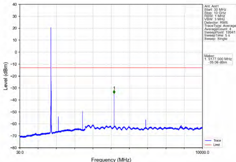
Band4_15MHz_16QAM_MCH_1732.5MHz_RB_1_0_NTNV
