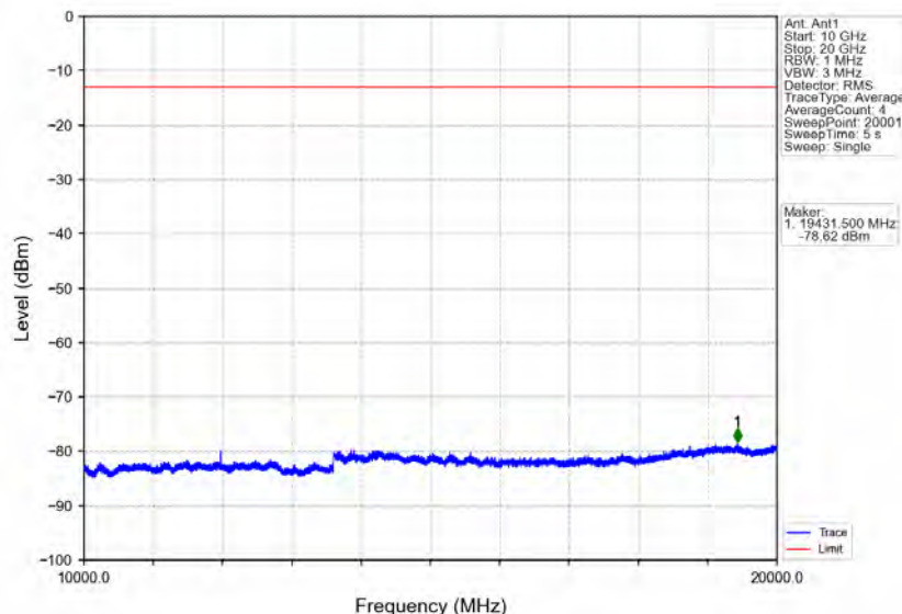
Band4_1.4MHz_64QAM_LCH_1710.7MHz_RB_6_0_NTNV
