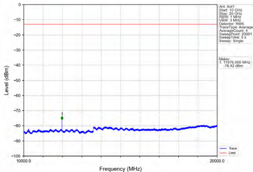
Band4_15MHz_16QAM_LCH_1717.5MHz_RB_75_0_NTNV
