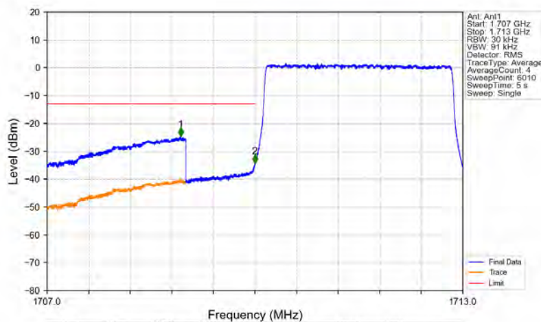
Band4_3MHz_64QAM_LCH_1711.5MHz_RB_15_0_NTNV
