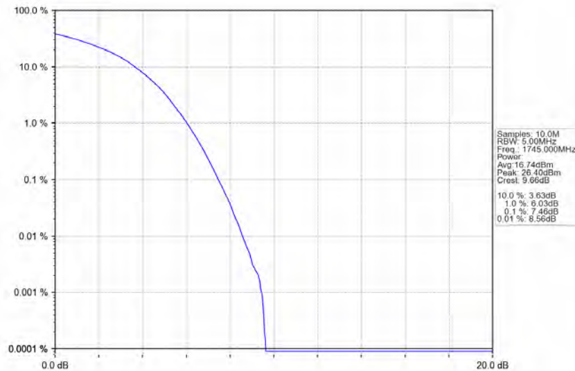
Band4_20MHz_16QAM_HCH_1745MHz_RB_100_0_NTNV
