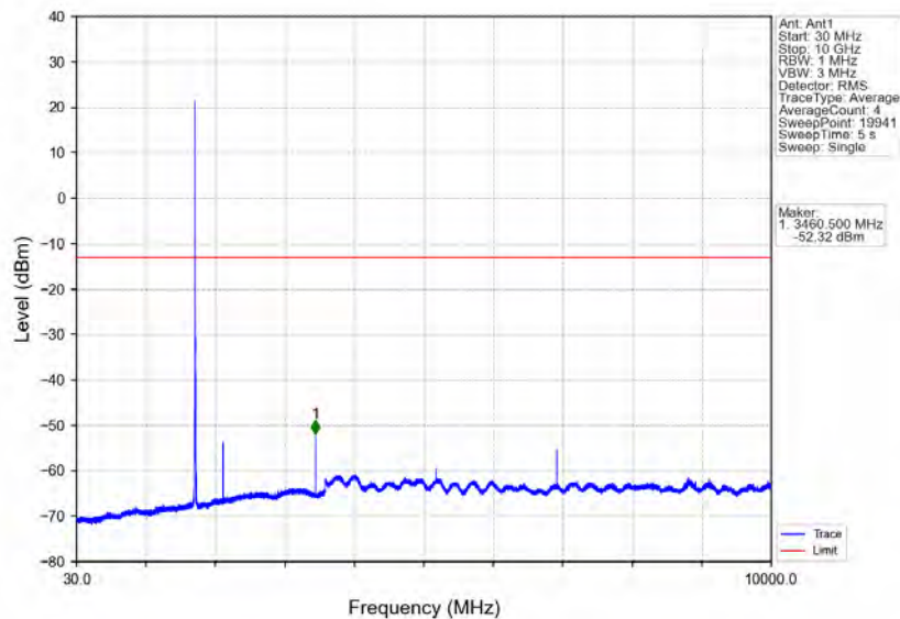
Band4_5MHz_16QAM_MCH_1732.5MHz_RB_1_0_NTNV
