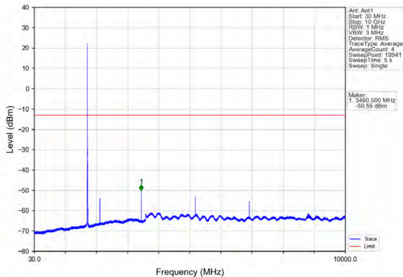
Band4_5MHz_QPSK_MCH_1732.5MHz_RB_1_0_NTNV
