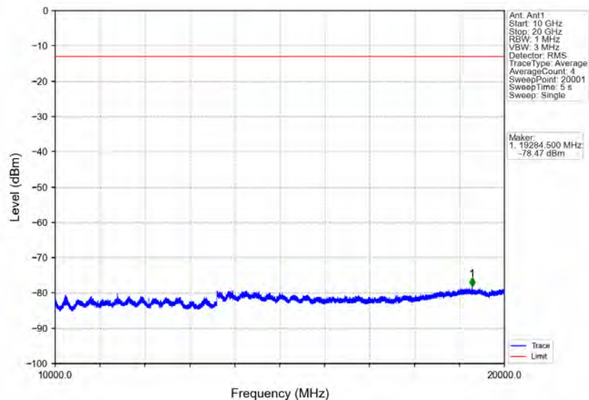
Band4_15MHz_64QAM_MCH_1732.5MHz_RB_1_0_NTNV
