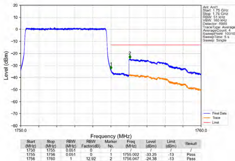
Band4_5MHz_64QAM_HCH_1752.5MHz_RB_25_0_NTNV
