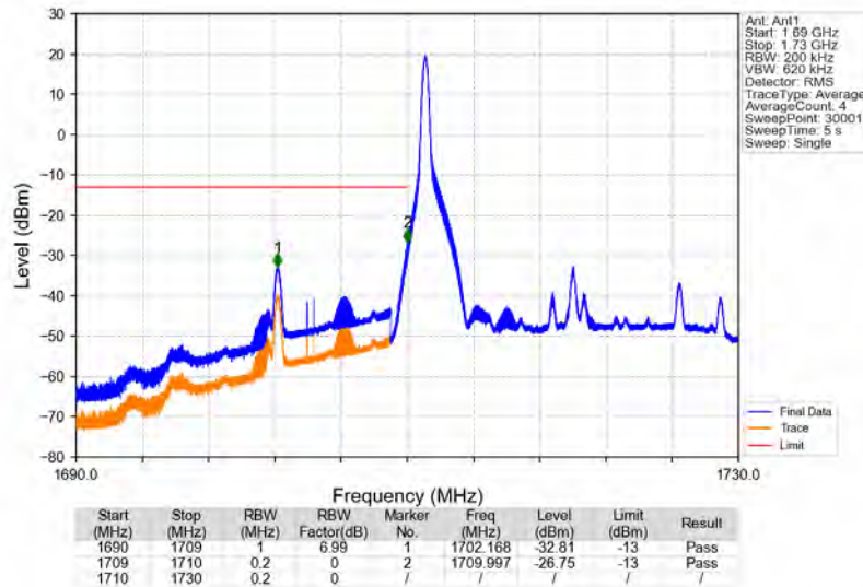
Band4_20MHz_64QAM_LCH_1720MHz_RB_1_0_NTNV
