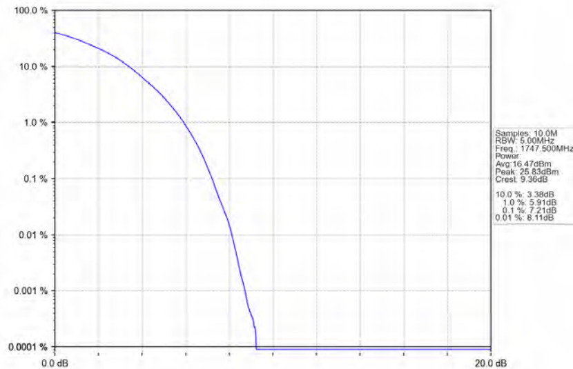
Band4_15MHz_64QAM_HCH_1747.5MHz_RB_75_0_NTNV
