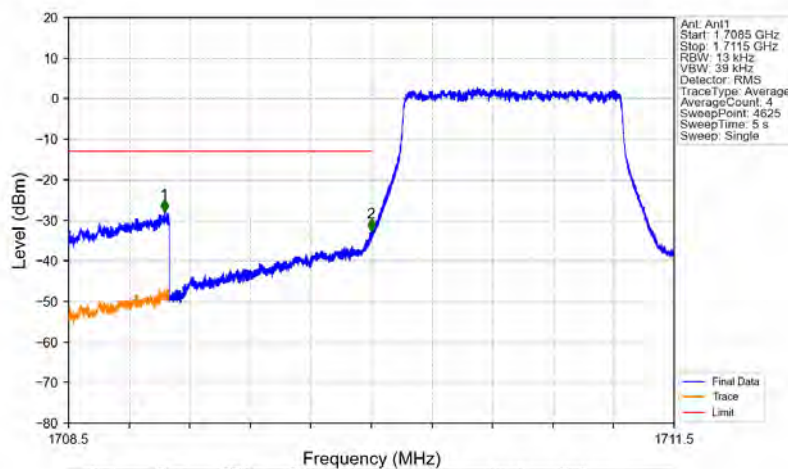
Band4_1.4MHz_64QAM_LCH_1710.7MHz_RB_6_0_NTNV
