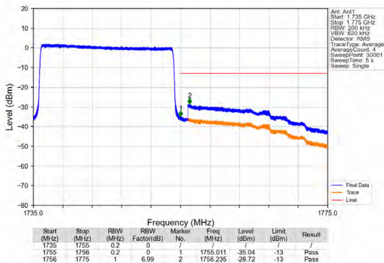
Band4_20MHz_64QAM_HCH_1745MHz_RB_100_0_NTNV
