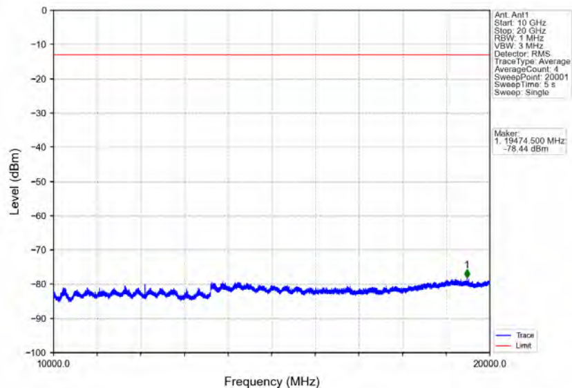
Band4_10MHz_64QAM_MCH_1732.5MHz_RB_1_0_NTNV
