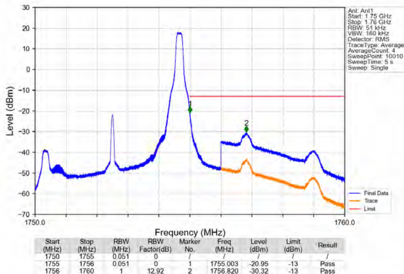
Band4_5MHz_QPSK_HCH_1752.5MHz_RB_1_24_NTNV
