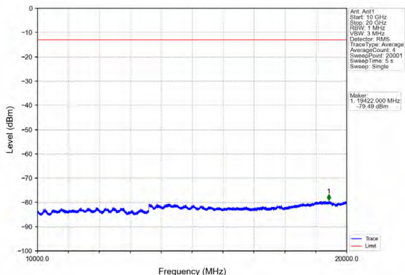
Band4_5MHz_QPSK_HCH_1752.5MHz_RB_1_0_NTNV
