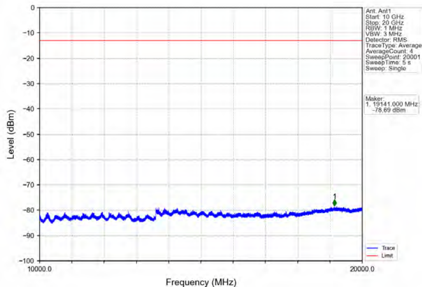
Band4 20MHz 64QAM HCH 1745MHz RB 1 0 NTNV
