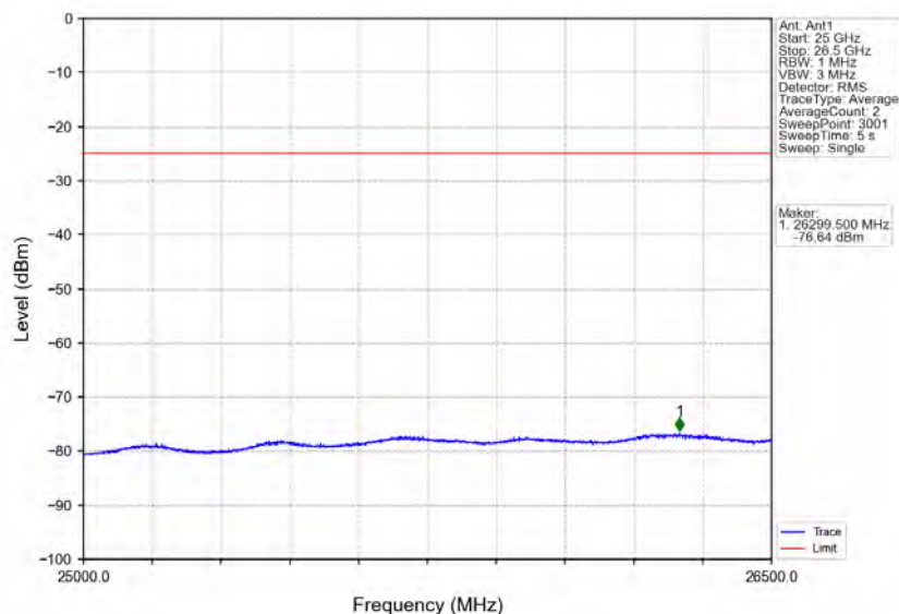
Band7_5MHz_64QAM_HCH_2567.5MHz_RB_1_24_NTNV
