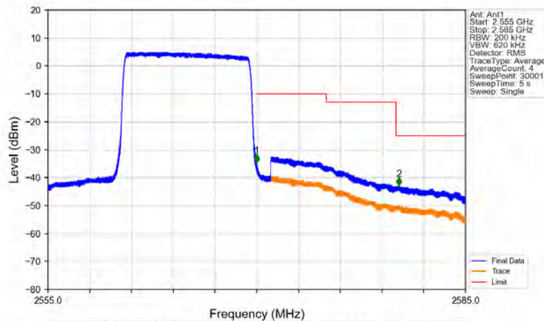
Band7_10MHz_64QAM_HCH_2565MHz_RB_50_0_NTNV
