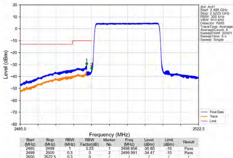
Band7_15MHz_64QAM_LCH_2507.5MHz_RB_75_0_NTNV
