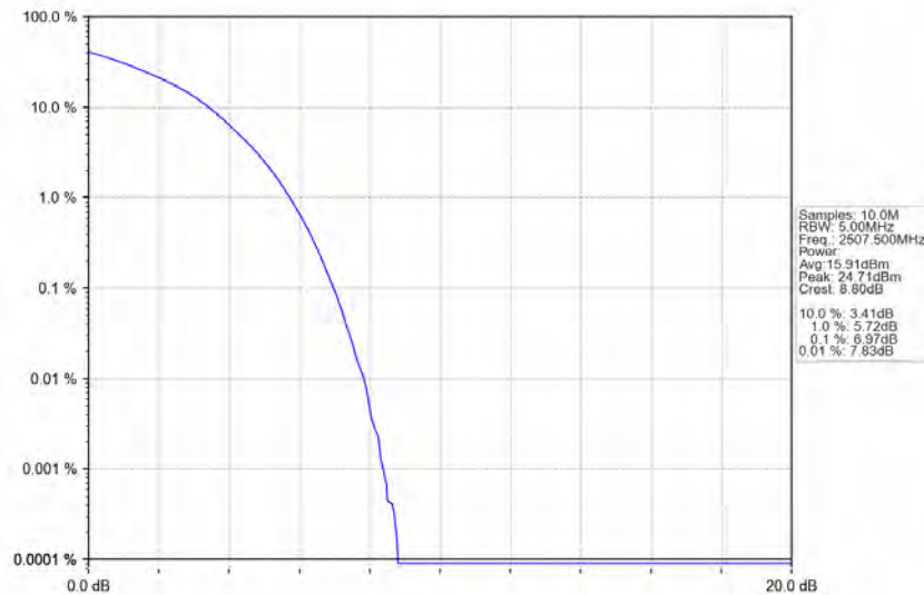
Band7_15MHz_16QAM_LCH_2507.5MHz_RB_75_0_NTNV
