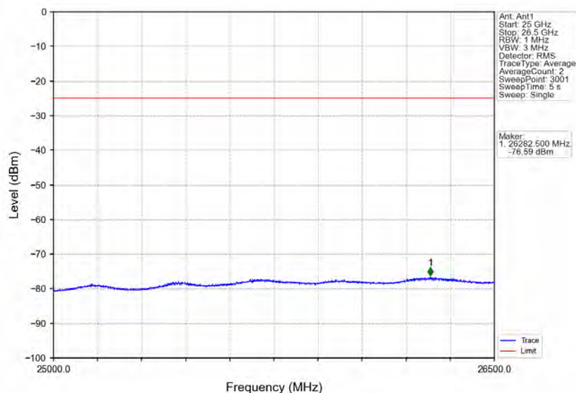
Band7_15MHz_64QAM_HCH_2562.5MHz_RB_1_74_NTNV
