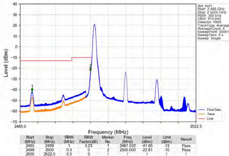
Band7_15MHz_QPSK_LCH_2507.5MHz_RB_1_0_NTNV
