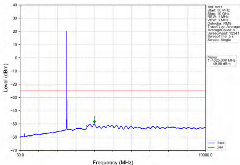
Band7_15MHz_16QAM_MCH_2535MHz_RB_1_0_NTNV
