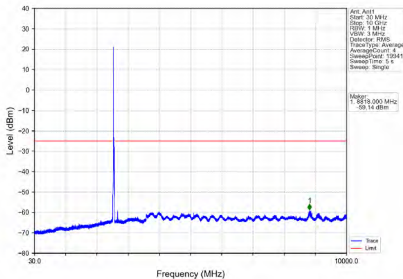
Band7_15MHz_64QAM_HCH_2562.5MHz_RB_1_0_NTNV
