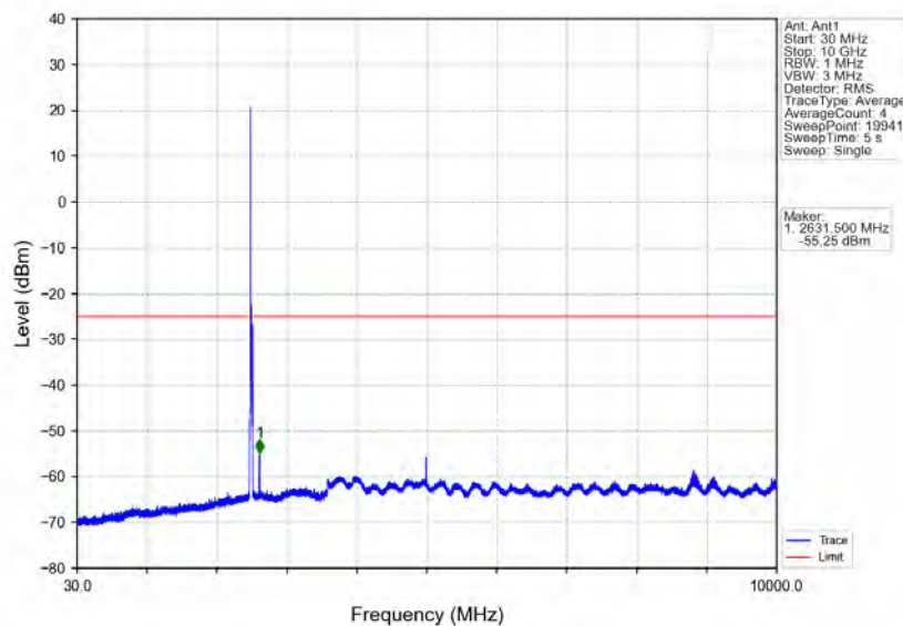
Band7_15MHz_64QAM_LCH_2507.5MHz_RB_1_0_NTNV
