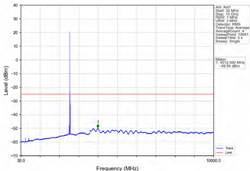
Band7_15MHz_QPSK_HCH_2562.5MHz_RB_1_0_NTNV
