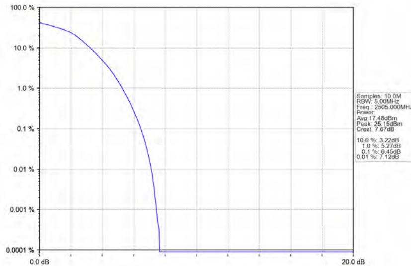
Band7_10MHz_16QAM_LCH_2505MHz_RB_50_0_NTNV
