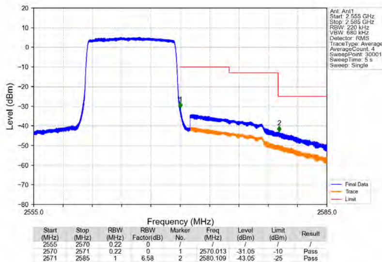
Band7_10MHz_16QAM_HCH_2565MHz_RB_50_0_NTNV
