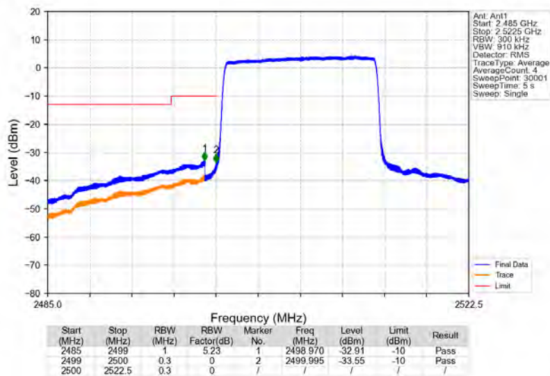
Band7_15MHz_16QAM_LCH_2507.5MHz_RB_75_0_NTNV
