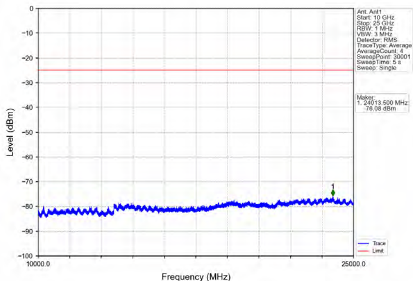
Band7_15MHz_64QAM_LCH_2507.5MHz_RB_1_0_NTNV
