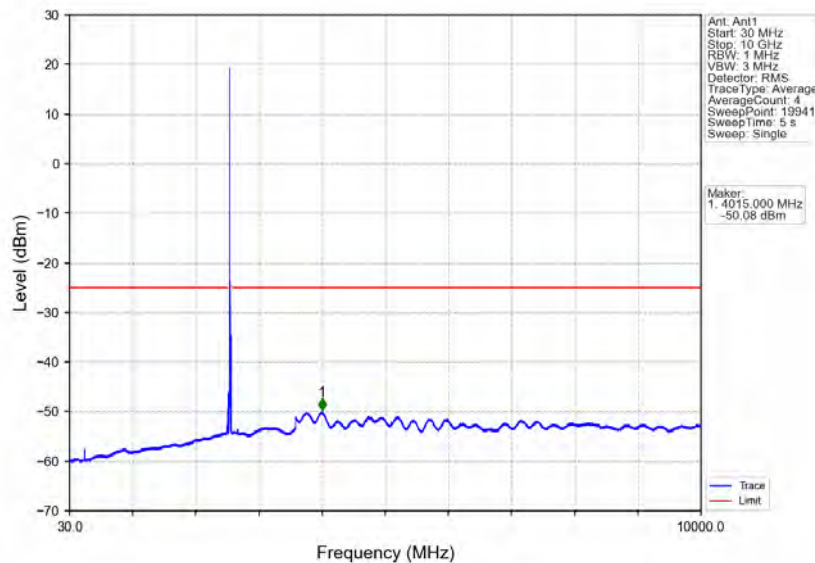
Band7_15MHz_16QAM_HCH_2562.5MHz_RB_1_0_NTNV
