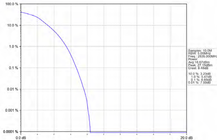
Band7_10MHz_64QAM_MCH_2535MHz_RB_50_0_NTNV
