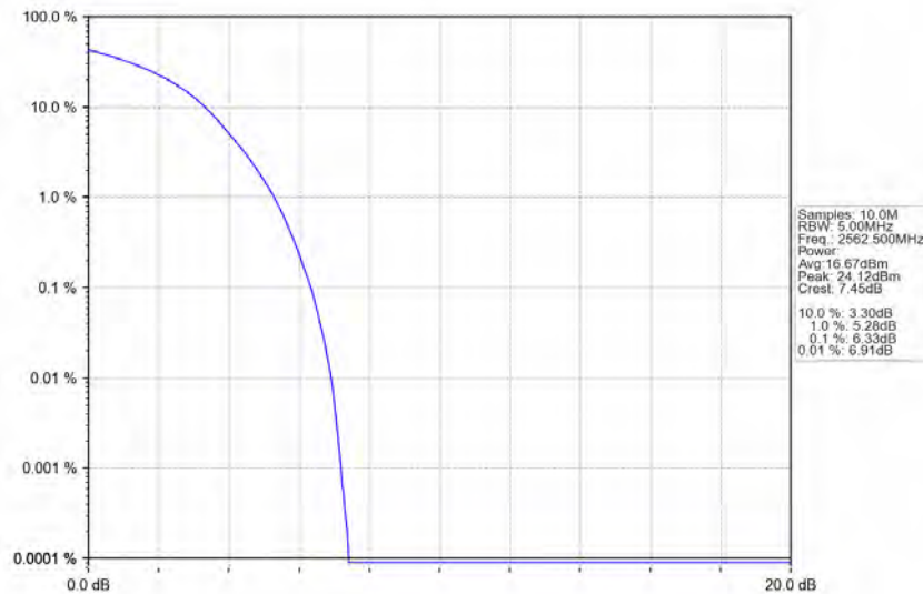
Band7_15MHz_QPSK_HCH_2562.5MHz_RB_75_0_NTNV
