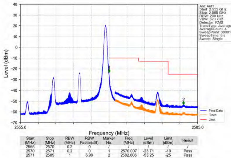
Band7_10MHz_16QAM_HCH_2565MHz_RB_1_49_NTNV
