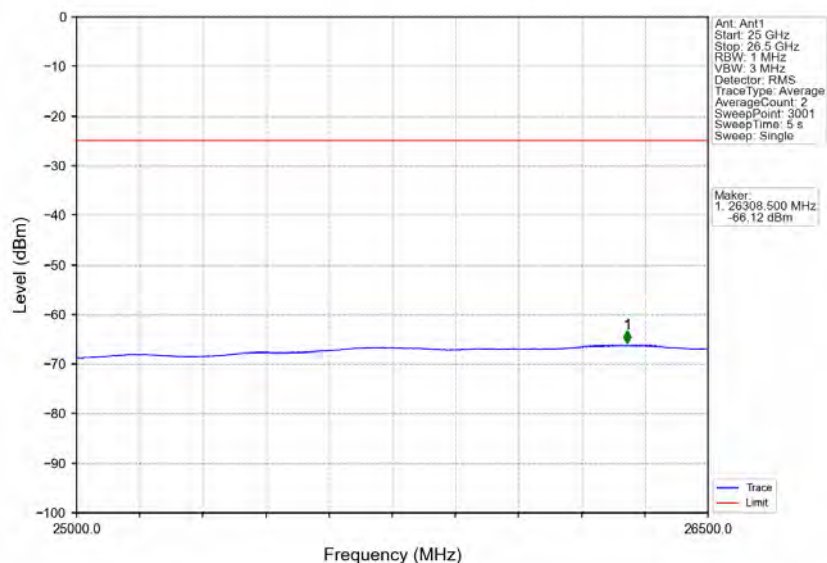
Band7_15MHz_16QAM_LCH_2507.5MHz_RB_75_0_NTNV
