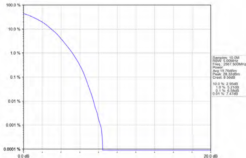
Band7_5MHz_64QAM_HCH_2567.5MHz_RB_25_0_NTNV
