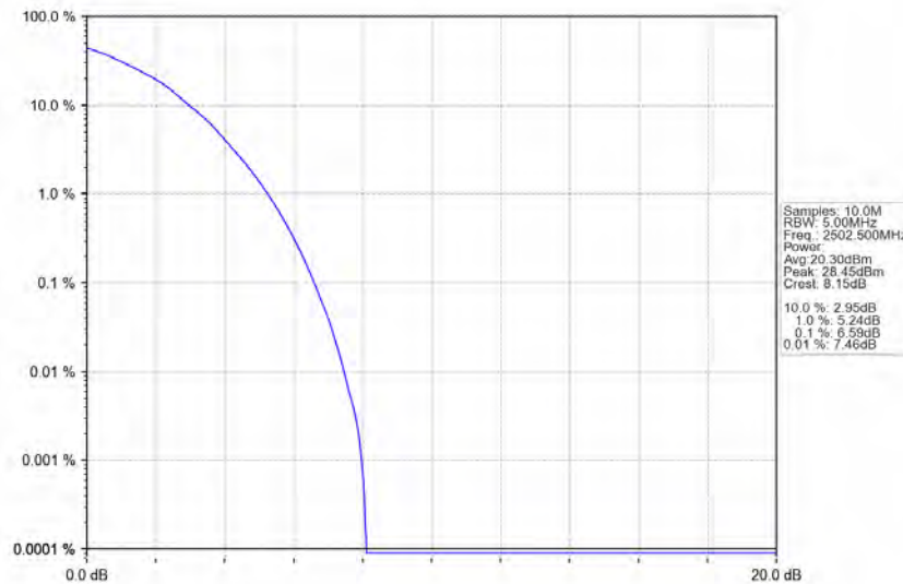
Band7_5MHz_64QAM_LCH_2502.5MHz_RB_25_0_NTNV
