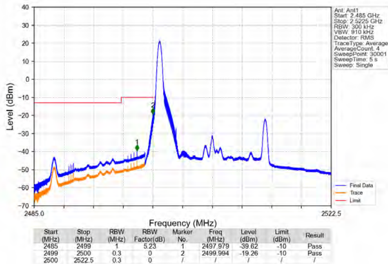
Band7_15MHz_64QAM_LCH_2507.5MHz_RB_1_0_NTNV
