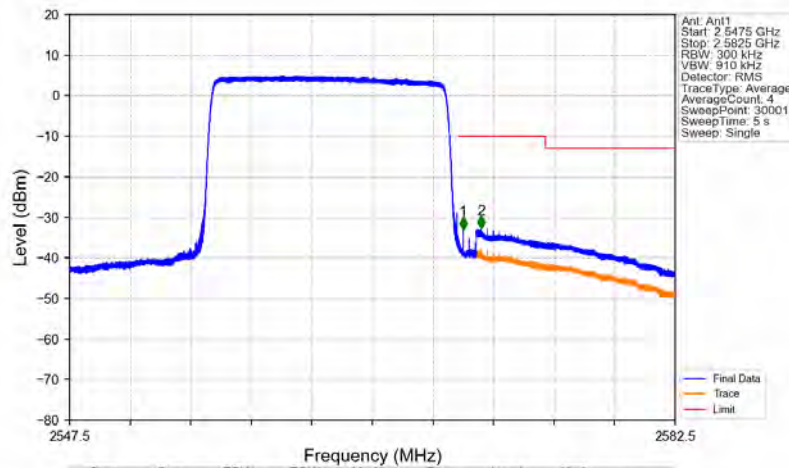
Band7_15MHz_64QAM_HCH_2562.5MHz_RB_75_0_NTNV
