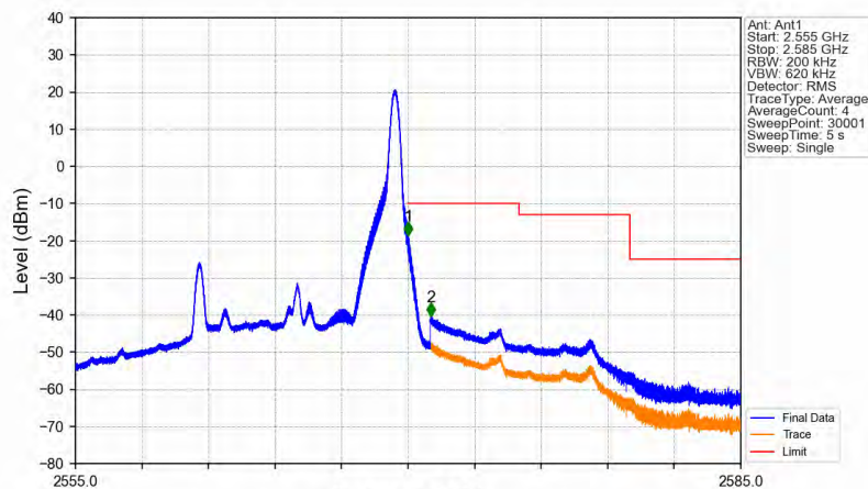
Band7_10MHz_64QAM_HCH_2565MHz_RB_1_49_NTNV
