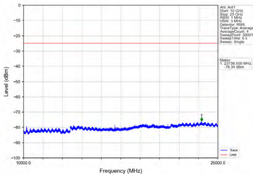
Band7_15MHz_64QAM_HCH_2562.5MHz_RB_1_0_NTNV
