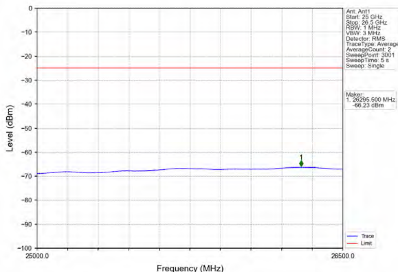
Band7_15MHz_16QAM_HCH_2562.5MHz_RB_1_0_NTNV
