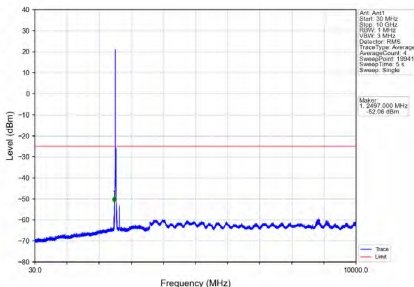
Band7_15MHz_64QAM_MCH_2535MHz_RB_1_0_NTNV
