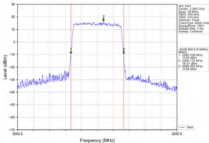
Band7_10MHz_64QAM_HCH_2565MHz_RB_50_0_NTNV
