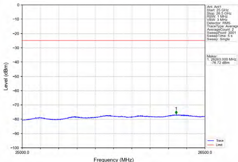
Band7_15MHz_64QAM_MCH_2535MHz_RB_1_0_NTNV
