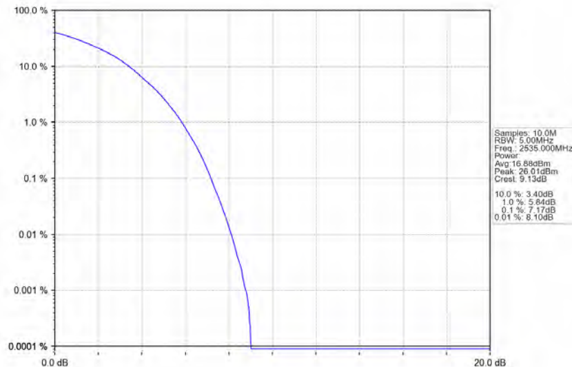
Band7_15MHz_64QAM_MCH_2535MHz_RB_75_0_NTNV
