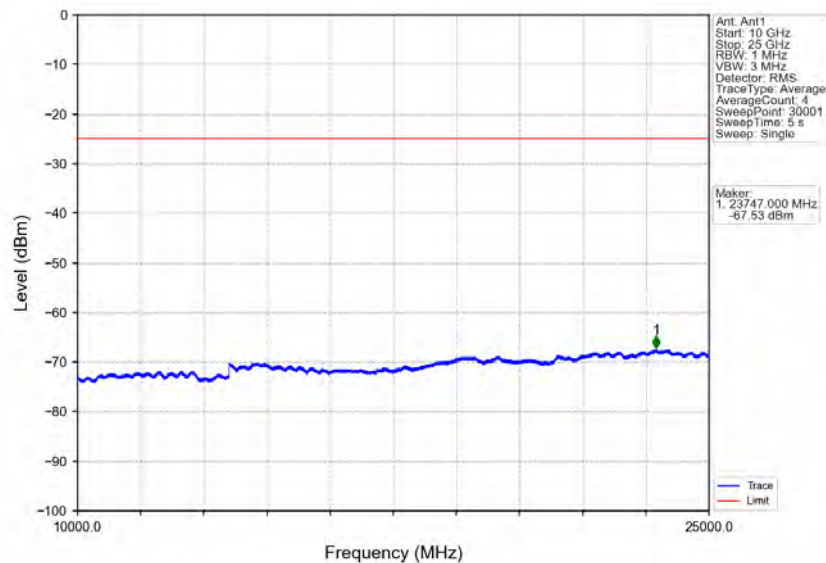
Band7_5MHz_16QAM_HCH_2567.5MHz_RB_1_0_NTNV
