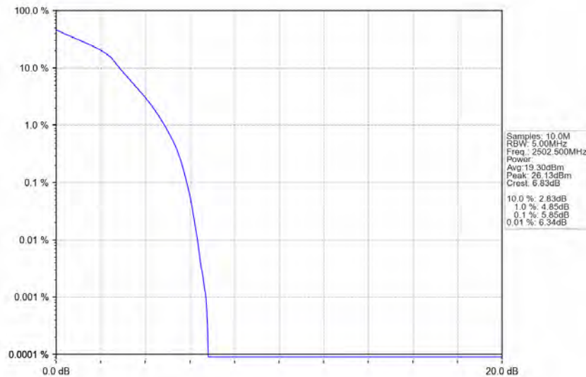
Band7_5MHz_16QAM_LCH_2502.5MHz_RB_25_0_NTNV
