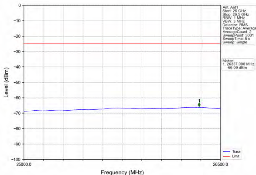
Band7_5MHz_16QAM_LCH_2502.5MHz_RB_25_0_NTNV
