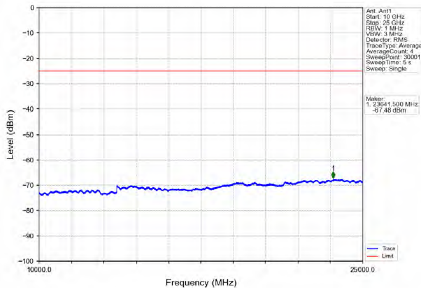
Band7_15MHz_16QAM_LCH_2507.5MHz_RB_1_0_NTNV
