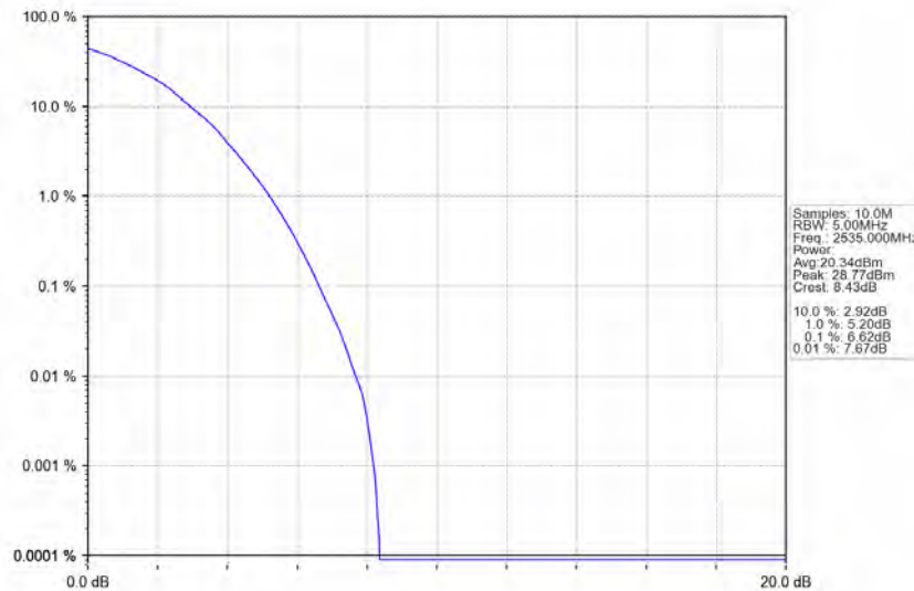
Band7_5MHz_64QAM_MCH_2535MHz_RB_25_0_NTNV
