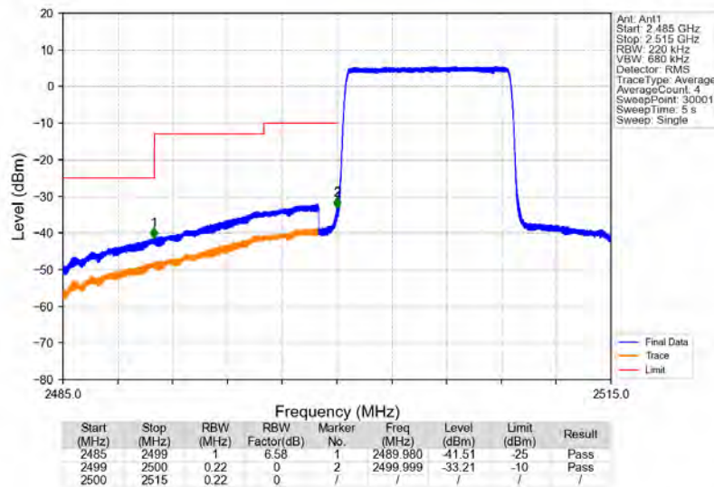
Band7_10MHz_64QAM_LCH_2505MHz_RB_50_0_NTNV
