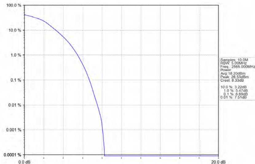
Band7_10MHz_64QAM_HCH_2565MHz_RB_50_0_NTNV
