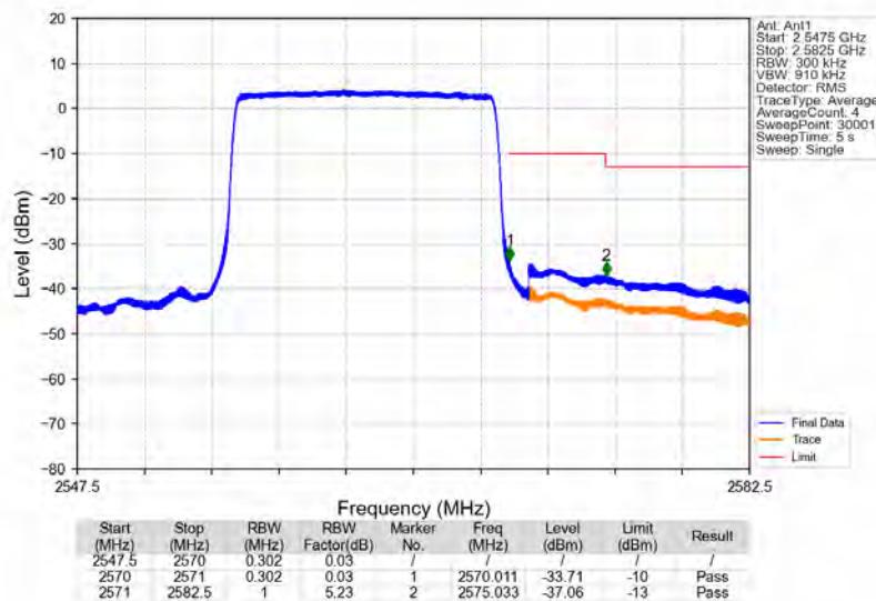
Band7_15MHz_16QAM_HCH_2562.5MHz_RB_75_0_NTNV
