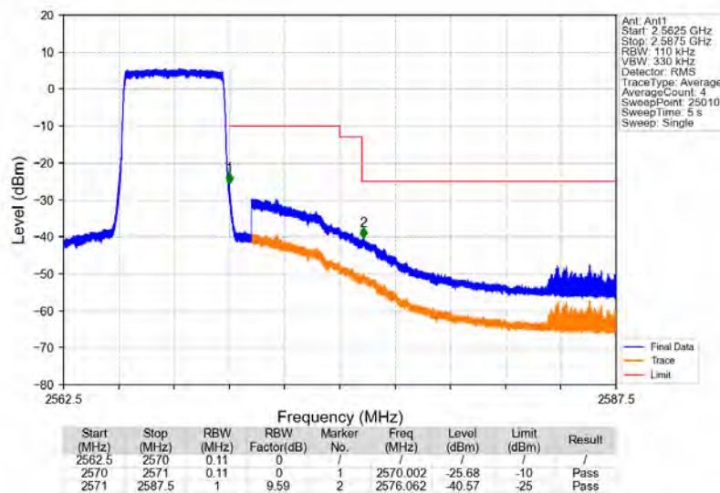
Band7_5MHz_16QAM_HCH_2567.5MHz_RB_25_0_NTNV
