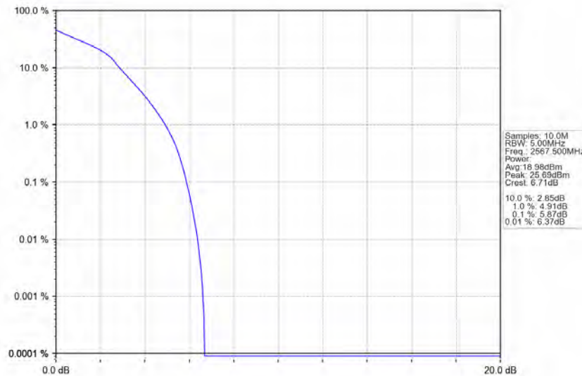
Band7_5MHz_16QAM_HCH_2567.5MHz_RB_25_0_NTNV
