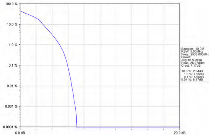
Band7_5MHz_16QAM_MCH_2535MHz_RB_25_0_NTNV
