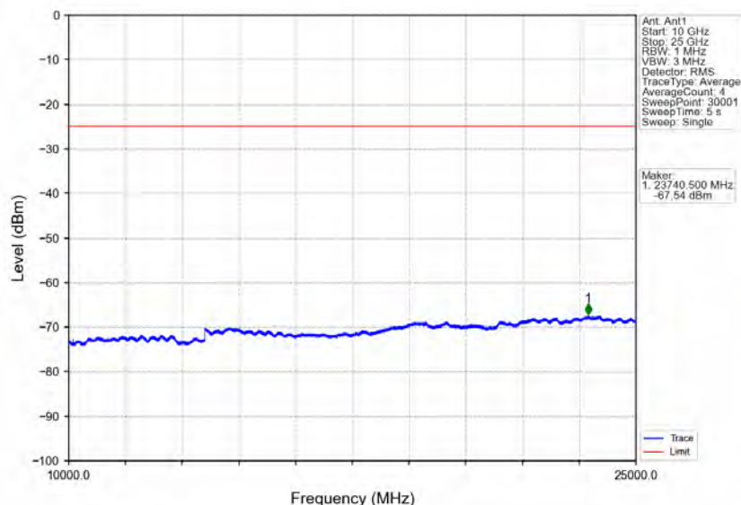
Band7_15MHz_16QAM_MCH_2535MHz_RB_1_0_NTNV
