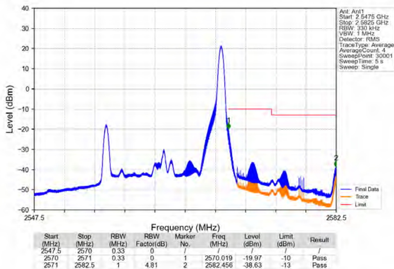
Band7_15MHz_64QAM_HCH_2562.5MHz_RB_1_74_NTNV
