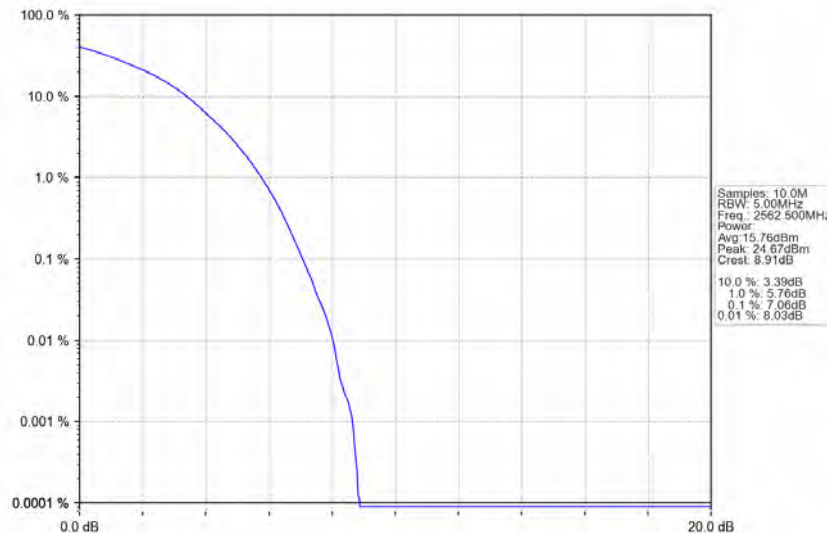
Band7_15MHz_16QAM_HCH_2562.5MHz_RB_75_0_NTNV
