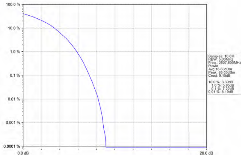
Band7_15MHz_64QAM_LCH_2507.5MHz_RB_75_0_NTNV
