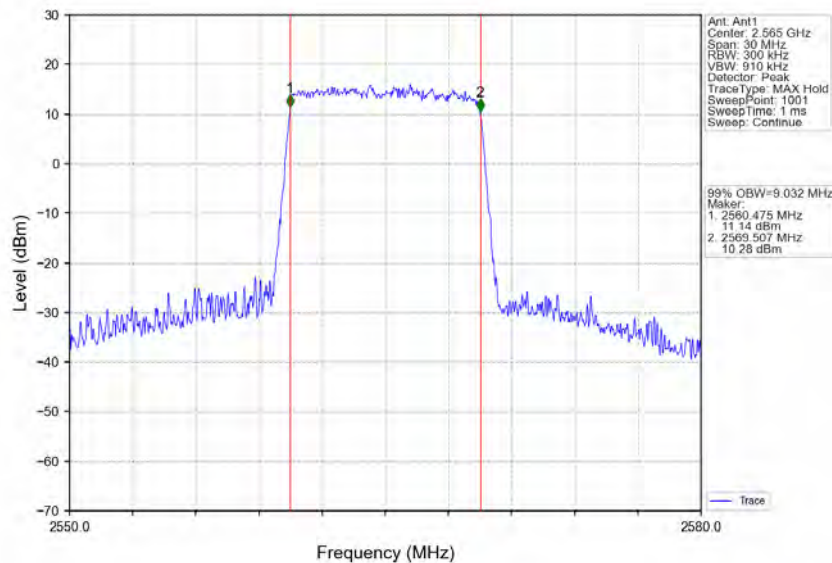
Band7_10MHz_64QAM_HCH_2565MHz_RB_50_0_NTNV
