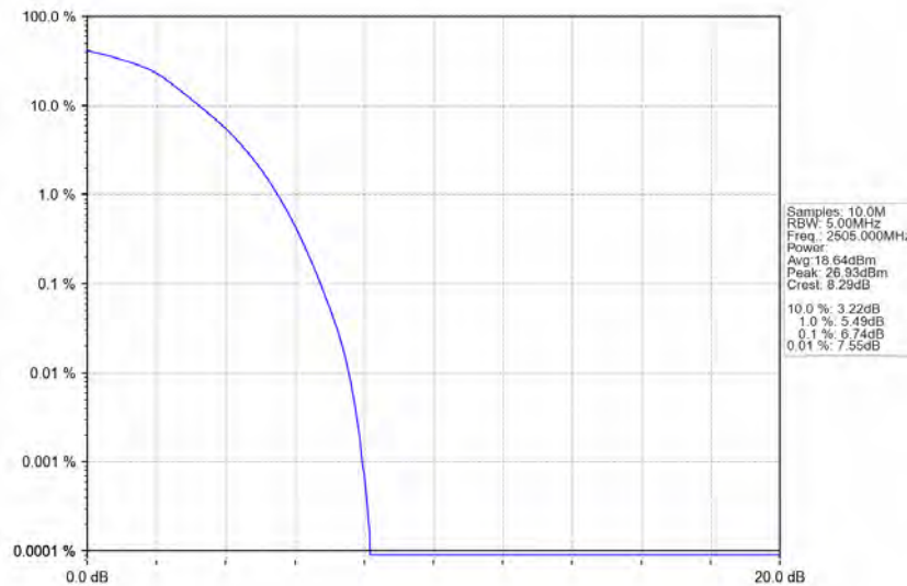
Band7_10MHz_64QAM_LCH_2505MHz_RB_50_0_NTNV
