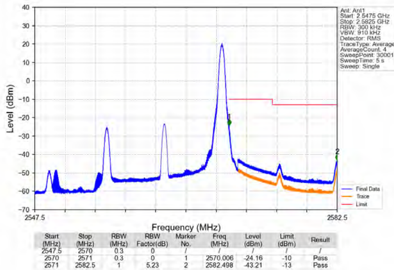
Band7_15MHz_16QAM_HCH_2562.5MHz_RB_1_74_NTNV
