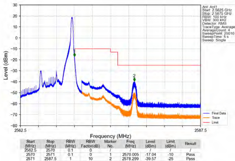
Band7_5MHz_64QAM_HCH_2567.5MHz_RB_1_24_NTNV
