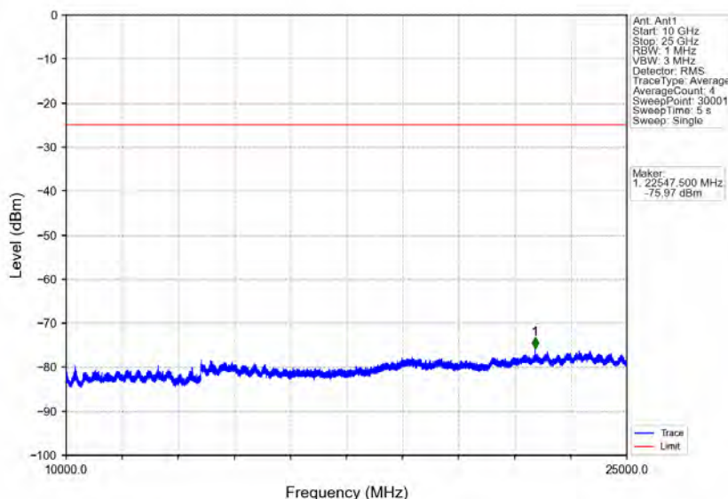
Band7_10MHz_64QAM_HCH_2565MHz_RB_1_0_NTNV
