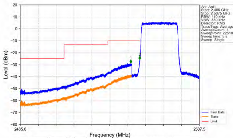
Band7_5MHz_16QAM_LCH_2502.5MHz_RB_25_0_NTNV
