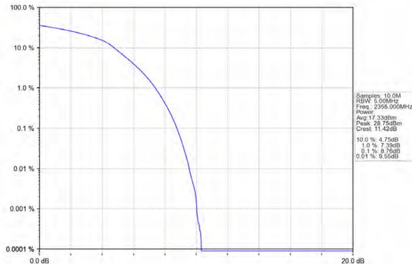
Band40b_10MHz_64QAM_HCH_2355MHz_RB_50_0_NTNV
