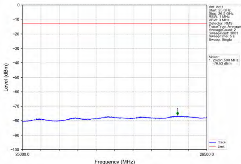
Band40b_5MHz_64QAM_LCH_2352.5MHz_RB_1_0_NTNV
