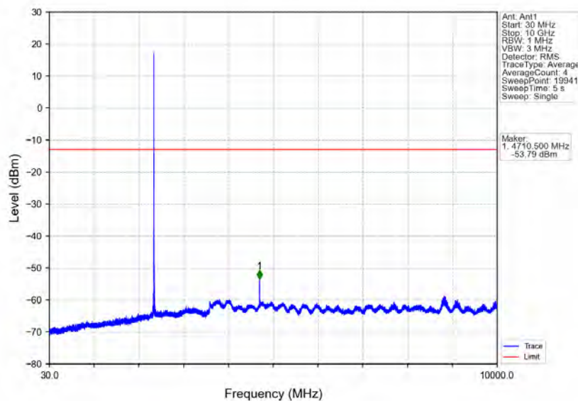
Band40b_5MHz_64QAM_HCH_2357.5MHz_RB_1_0_NTNV
