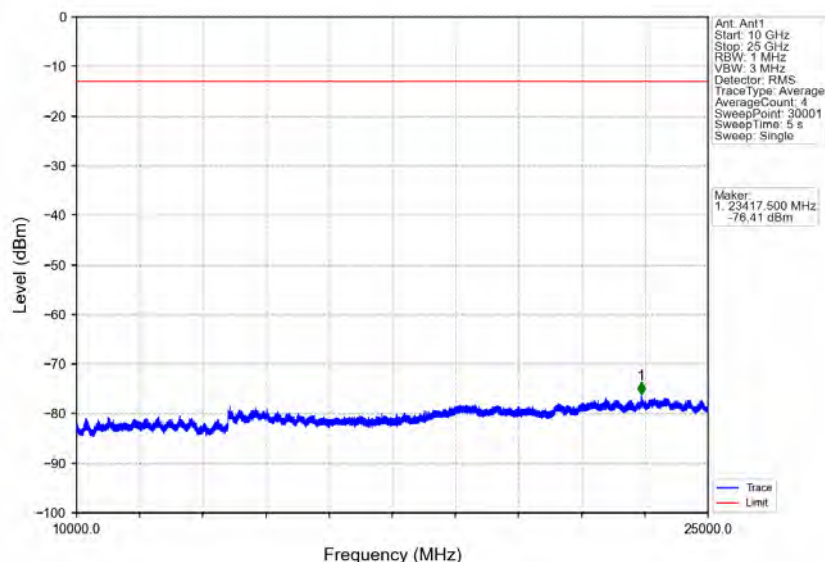
Band40b_10MHz_64QAM_HCH_2355MHz_RB_1_0_NTNV
