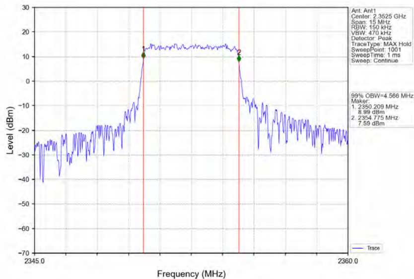
Band40b_5MHz_16QAM_LCH_2352.5MHz_RB_25_0_NTNV
