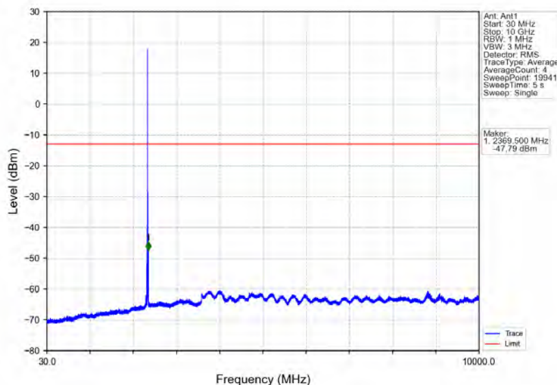
Band40b_5MHz_16QAM_LCH_2352.5MHz_RB_1_0_NTNV
