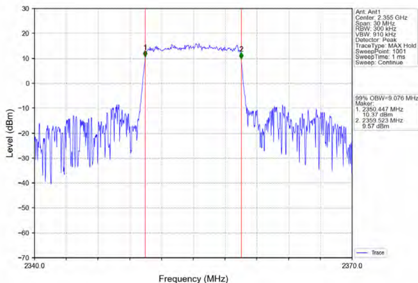
Band40b_10MHz_64QAM_LCH_2355MHz_RB_50_0_NTNV
