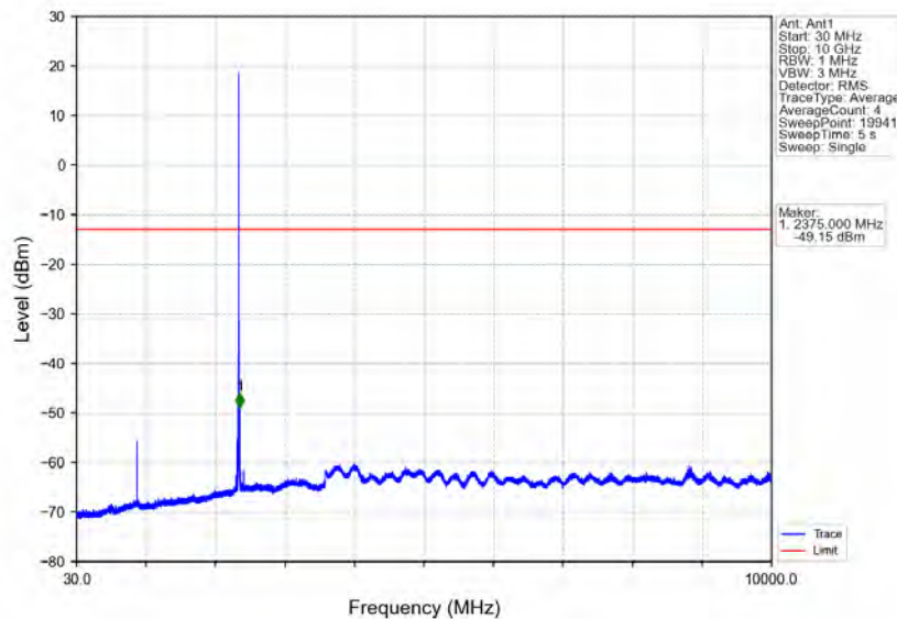
Band40b_5MHz_QPSK_HCH_2357.5MHz_RB_1_0_NTNV
