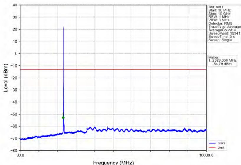
Band40b_10MHz_16QAM_HCH_2355MHz_RB_1_0_NTNV
