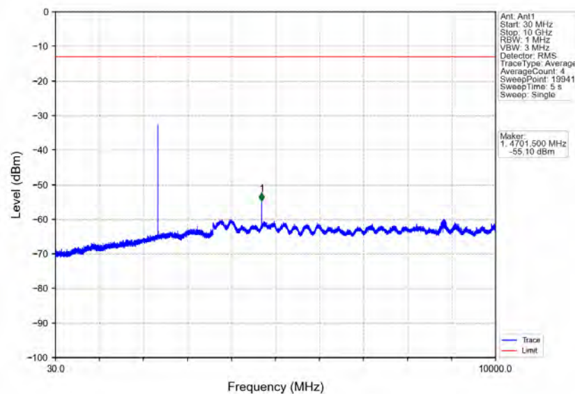
Band40b_10MHz_64QAM_MCH_2355MHz_RB_1_0_NTNV
