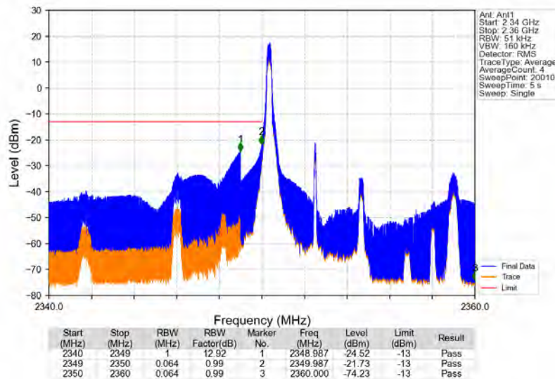
Band40b_5MHz_16QAM_LCH_2352.5MHz_RB_1_0_NTNV
