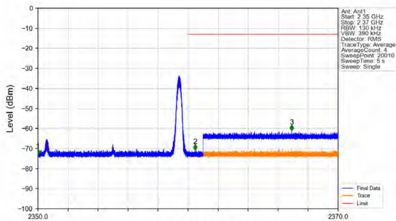
Band40b_10MHz_64QAM_HCH_2355MHz_RB_1_49_NTNV
