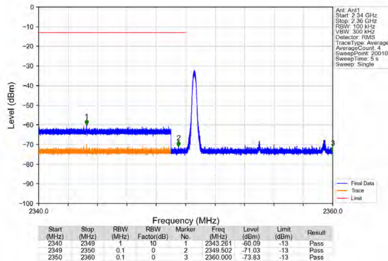
Band40b_10MHz_64QAM_LCH_2355MHz_RB_1_0_NTNV
