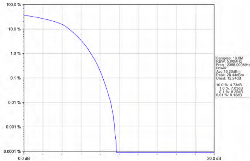
Band40b_10MHz_16QAM_HCH_2355MHz_RB_50_0_NTNV
