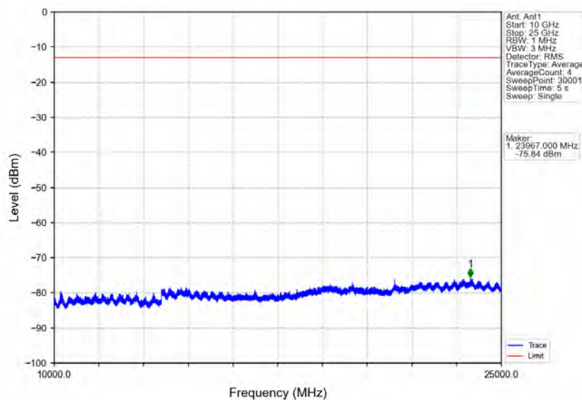
Band40b_5MHz_64QAM_HCH_2357.5MHz_RB_1_0_NTNV
