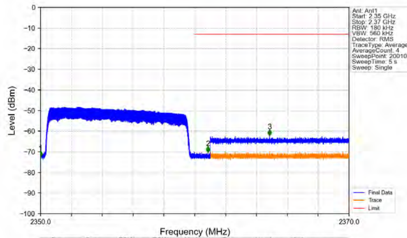
Band40b_10MHz_64QAM_HCH_2355MHz_RB_50_0_NTNV
