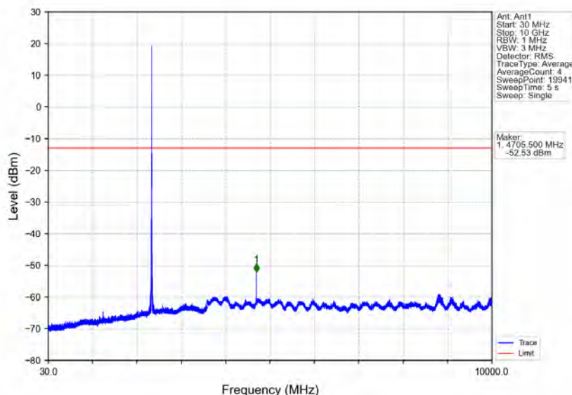
Band40b_5MHz_64QAM_MCH_2355MHz_RB_1_0_NTNV
