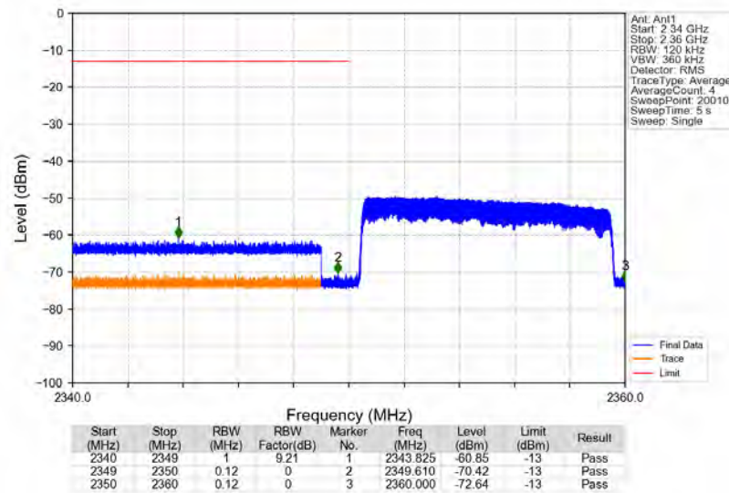
Band40b_10MHz_64QAM_LCH_2355MHz_RB_50_0_NTNV
