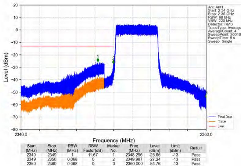
Band40b_5MHz_QPSK_LCH_2352.5MHz_RB_25_0_NTNV
