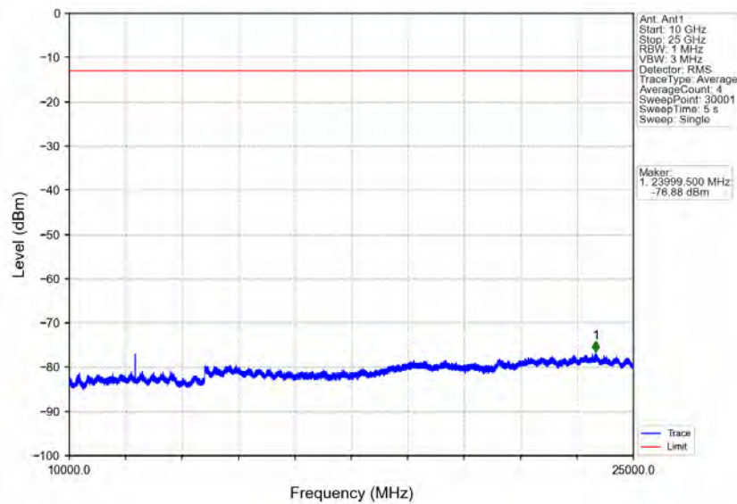
Band40b_5MHz_QPSK_LCH_2352.5MHz_RB_1_0_NTNV
