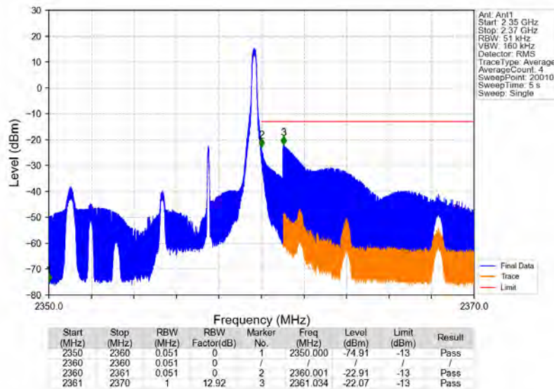
Band40b_5MHz_16QAM_HCH_2357.5MHz_RB_1_24_NTNV
