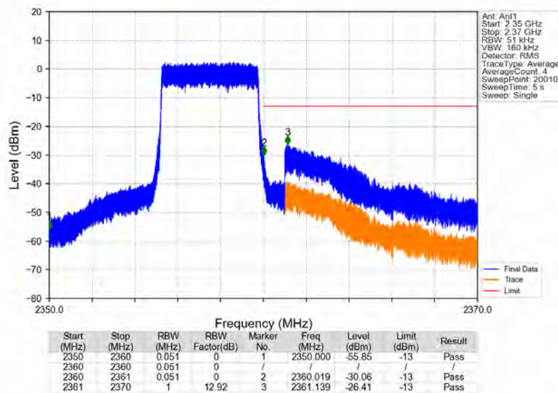
Band40b_5MHz_16QAM_HCH_2357.5MHz_RB_25_0_NTNV
