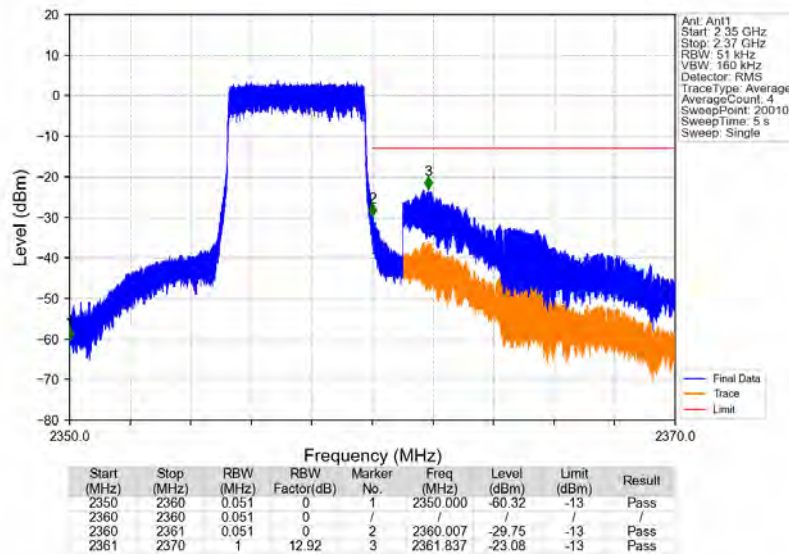
Band40b_5MHz_QPSK_HCH_2357.5MHz_RB_25_0_NTNV
