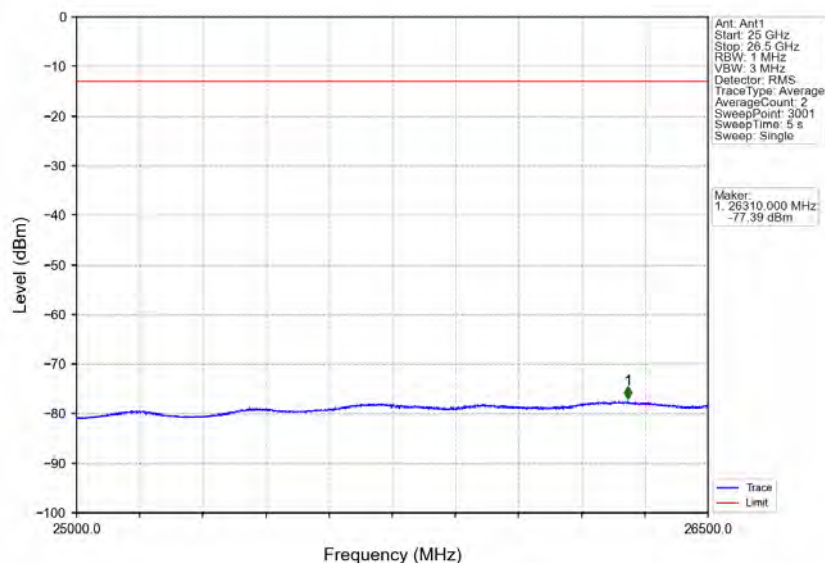
Band40b_10MHz_16QAM_HCH_2355MHz_RB_1_0_NTNV
