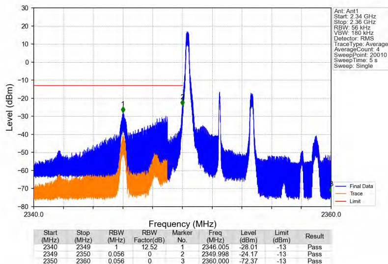
Band40b_5MHz_64QAM_LCH_2352.5MHz_RB_1_0_NTNV
