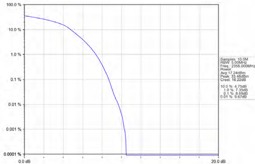
Band40b_10MHz_64QAM_LCH_2355MHz_RB_50_0_NTNV
