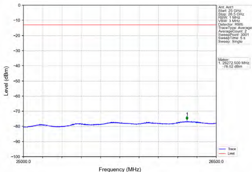
Band40b_5MHz_64QAM_HCH_2357.5MHz_RB_1_24_NTNV
