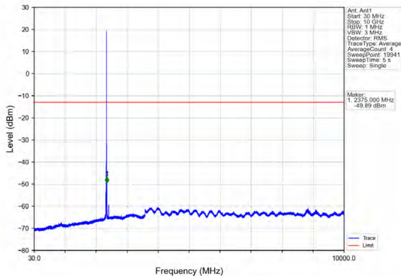
Band40b_5MHz_16QAM_HCH_2357.5MHz_RB_1_0_NTNV
