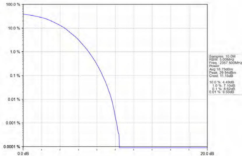
Band40b_5MHz_64QAM_HCH_2357.5MHz_RB_25_0_NTNV
