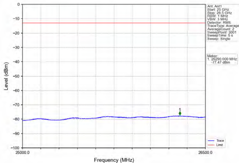
Band40b_5MHz_16QAM_HCH_2357.5MHz_RB_1_0_NTNV
