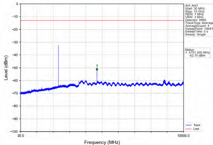
Band40b_10MHz_64QAM_LCH_2355MHz_RB_1_0_NTNV
