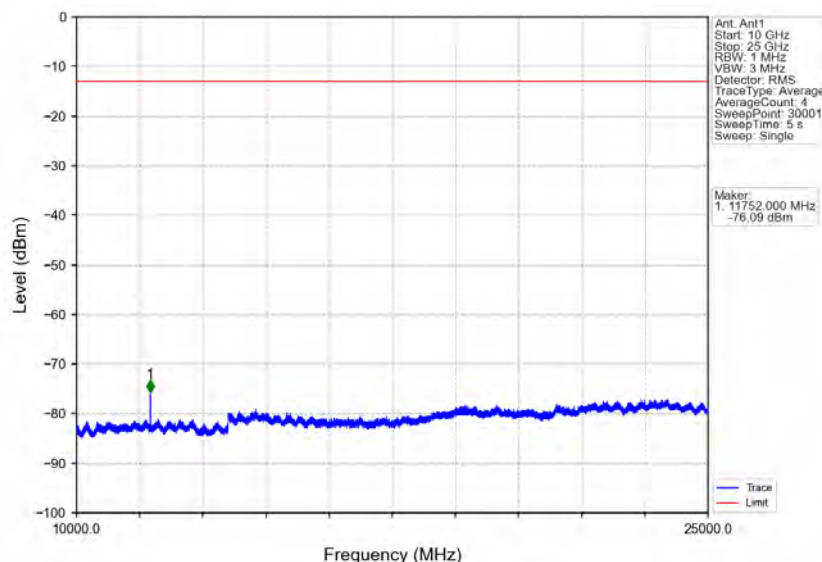
Band40b_5MHz_16QAM_LCH_2352.5MHz_RB_1_0_NTNV
