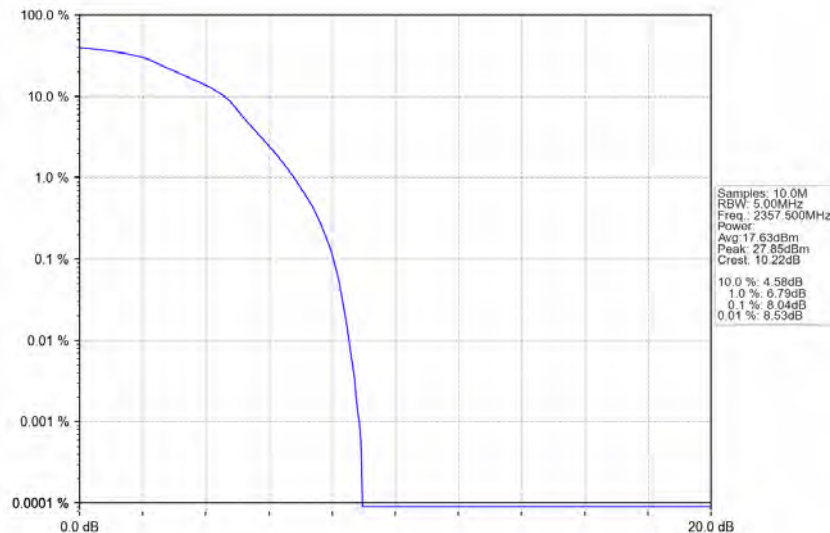
Band40b_5MHz_16QAM_HCH_2357.5MHz_RB_25_0_NTNV
