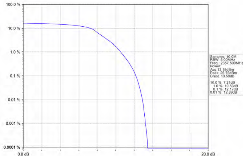
Band40b_5MHz_QPSK_HCH_2357.5MHz_RB_25_0_NTNV
