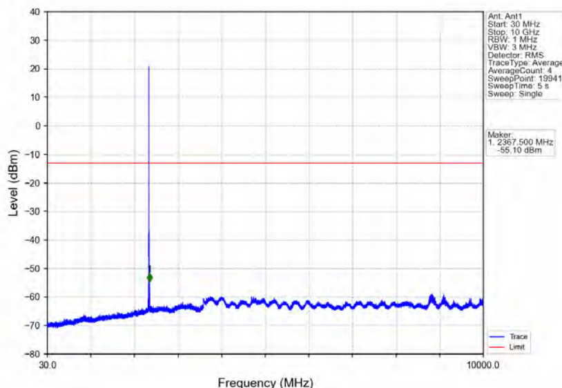
Band40b_5MHz_64QAM_LCH_2352.5MHz_RB_1_0_NTNV
