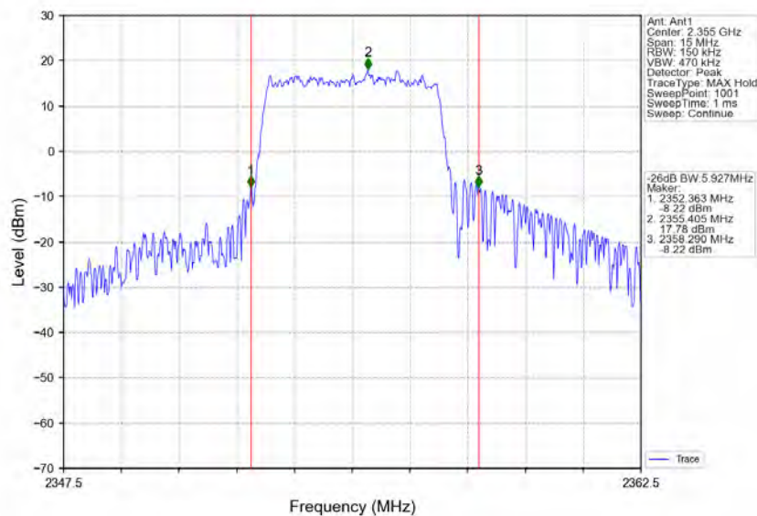
Band40b_5MHz_64QAM_MCH_2355MHz_RB_25_0_NTNV
