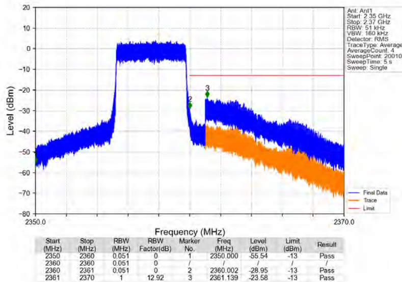
Band40b_5MHz_64QAM_HCH_2357.5MHz_RB_25_0_NTNV
