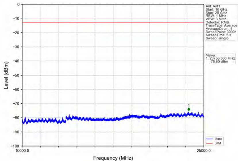
Band40b_5MHz_64QAM_MCH_2355MHz_RB_1_0_NTNV
