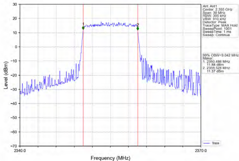
Band40b_10MHz_64QAM_HCH_2355MHz_RB_50_0_NTNV
