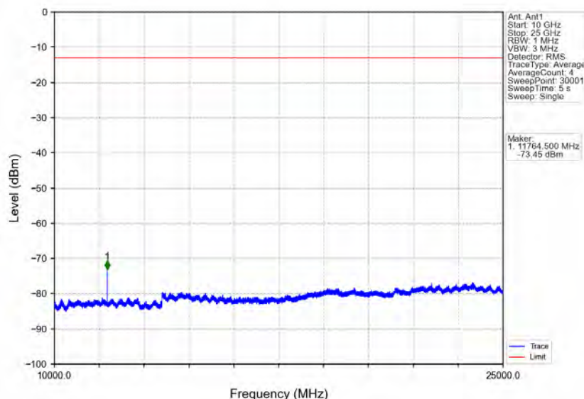
Band40b_5MHz_16QAM_MCH_2355MHz_RB_1_0_NTNV
