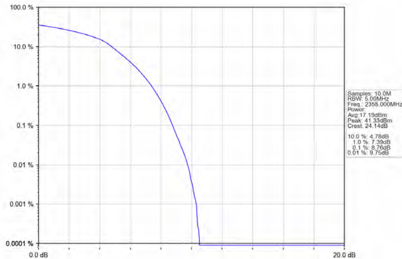
Band40b_10MHz_64QAM_MCH_2355MHz_RB_50_0_NTNV
