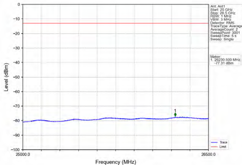
Band40b_5MHz_16QAM_LCH_2352.5MHz_RB_25_0_NTNV
