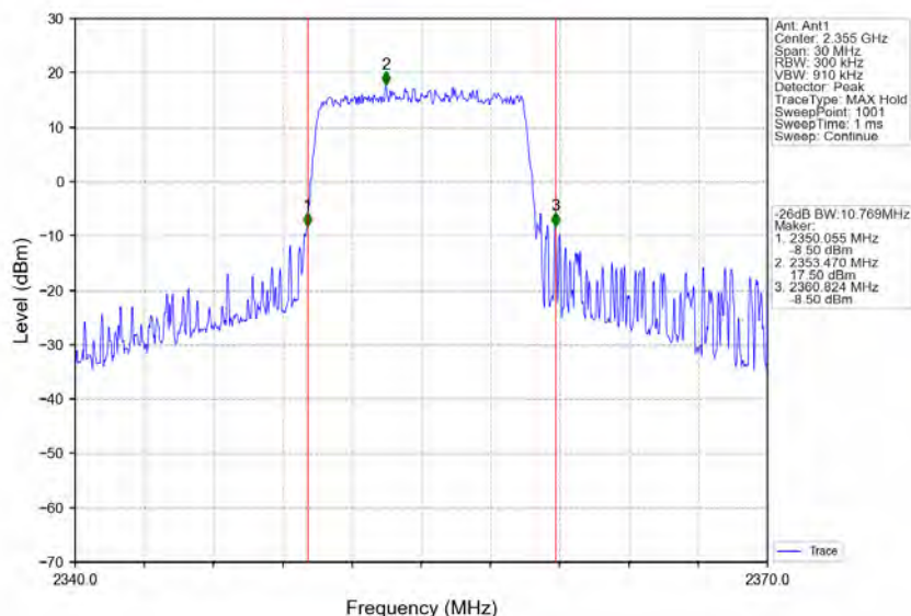
Band40b_10MHz_64QAM_HCH_2355MHz_RB_50_0_NTNV
