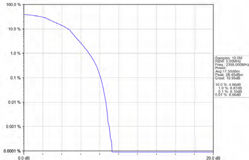
Band40b_5MHz_16QAM_MCH_2355MHz_RB_25_0_NTNV
