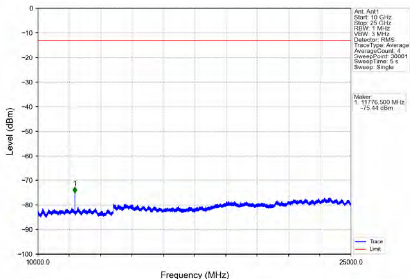
Band40b_5MHz_16QAM_HCH_2357.5MHz_RB_1_0_NTNV
