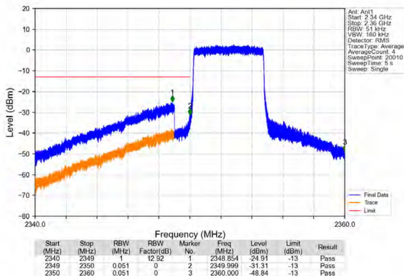
Band40b_5MHz_64QAM_LCH_2352.5MHz_RB_25_0_NTNV
