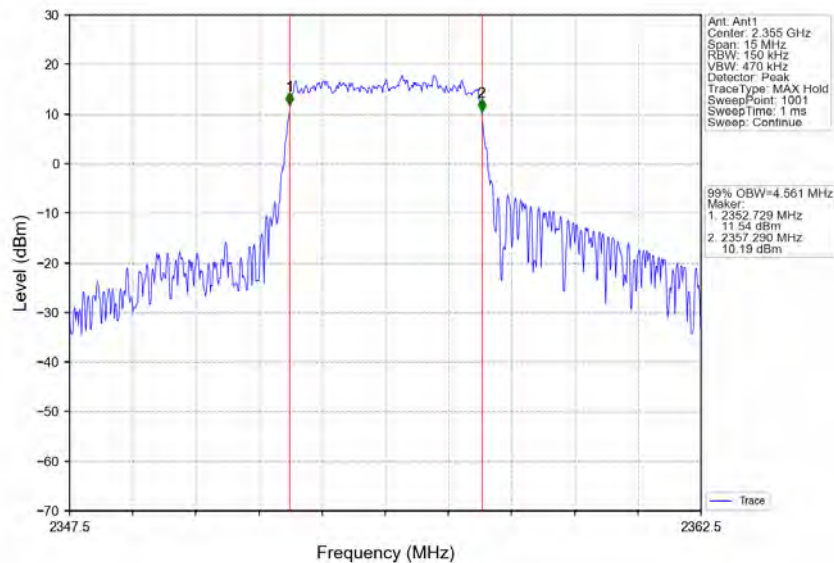
Band40b_5MHz_64QAM_MCH_2355MHz_RB_25_0_NTNV
