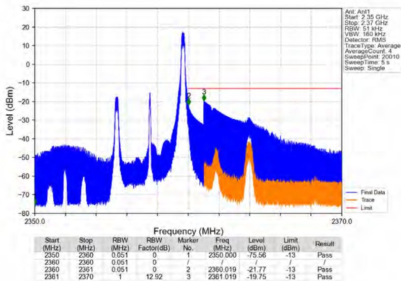
Band40b_5MHz_64QAM_HCH_2357.5MHz_RB_1_24_NTNV
