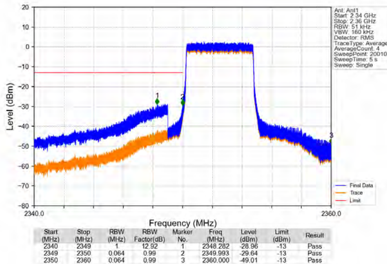
Band40b_5MHz_16QAM_LCH_2352.5MHz_RB_25_0_NTNV
