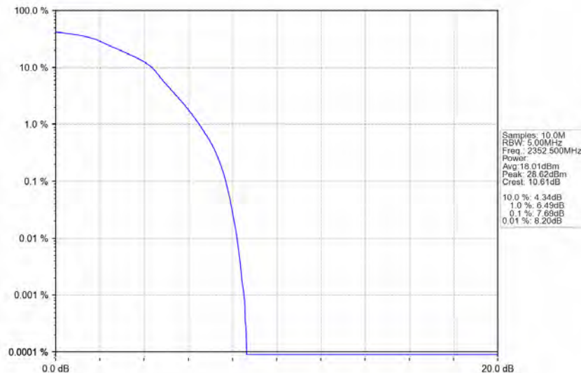
Band40b_5MHz_16QAM_LCH_2352.5MHz_RB_25_0_NTNV
