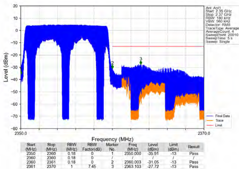
Band40b_10MHz_16QAM_HCH_2355MHz_RB_50_0_NTNV
