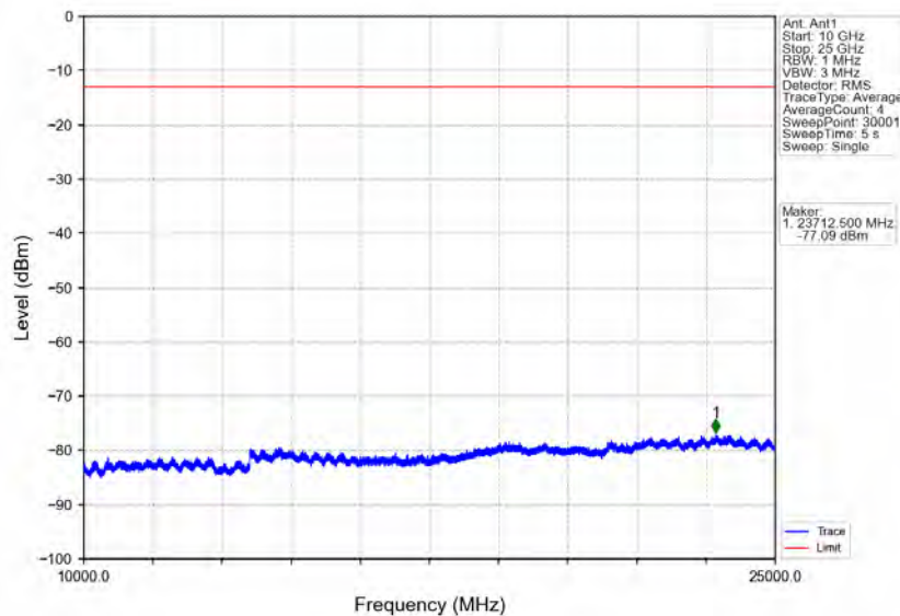
Band40b_5MHz_QPSK_HCH_2357.5MHz_RB_1_0_NTNV
