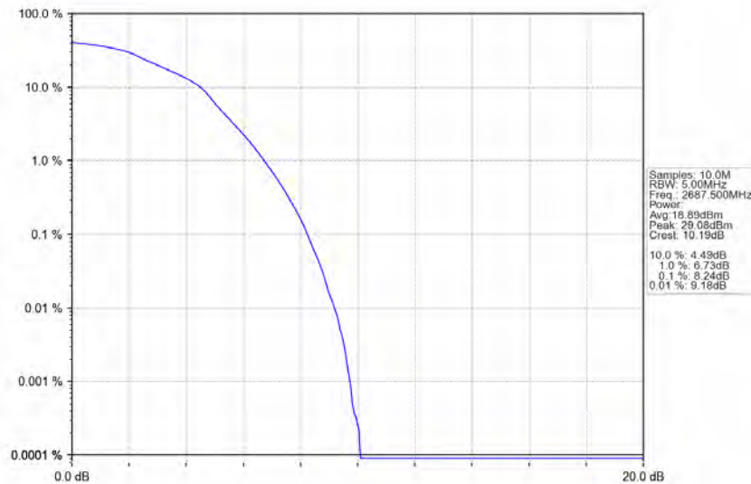
Band41_5MHz_16QAM_HCH_2687.5MHz_RB_25_0_NTNV
