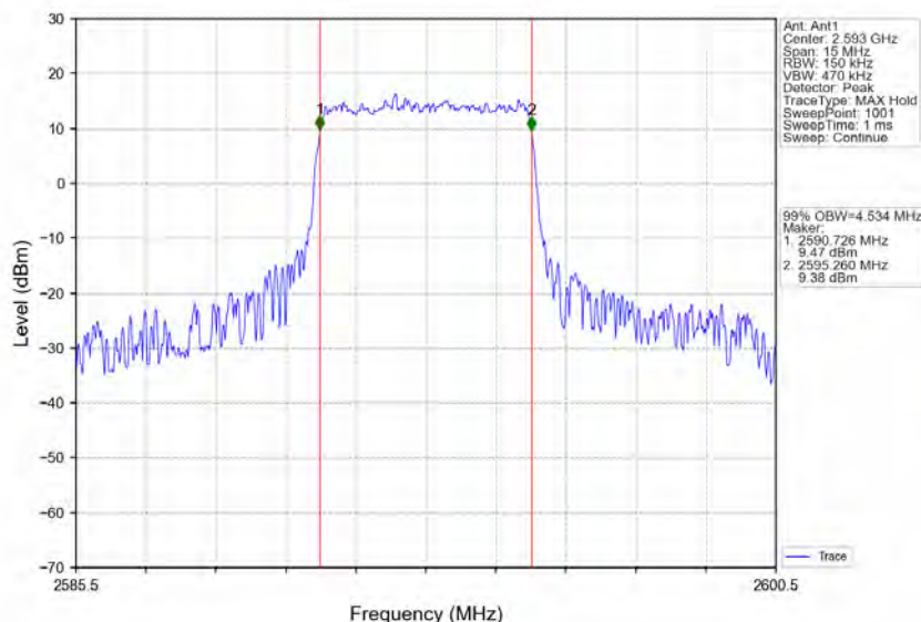
Band41_5MHz_64QAM_MCH_2593MHz_RB_25_0_NTNV
