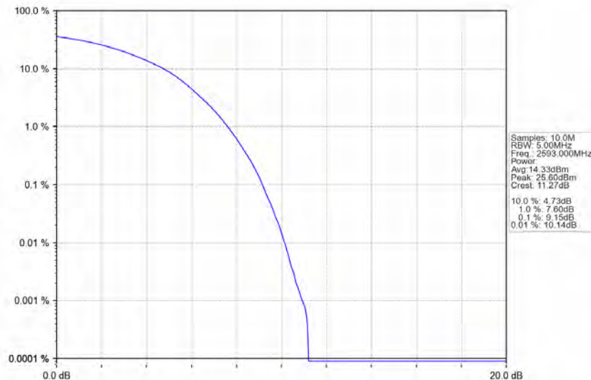
Band41_15MHz_64QAM_MCH_2593MHz_RB_75_0_NTNV
