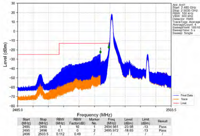
Band41_5MHz_64QAM_LCH_2498.5MHz_RB_1_0_NTNV
