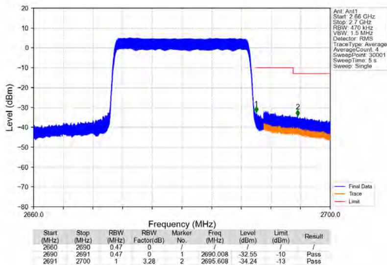
Band41_20MHz_64QAM_HCH_2680MHz_RB_100_0_NTNV
