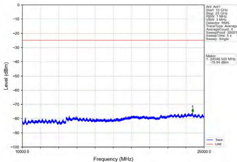
Band41_20MHz_16QAM_LCH_2506MHz_RB_1_0_NTNV
