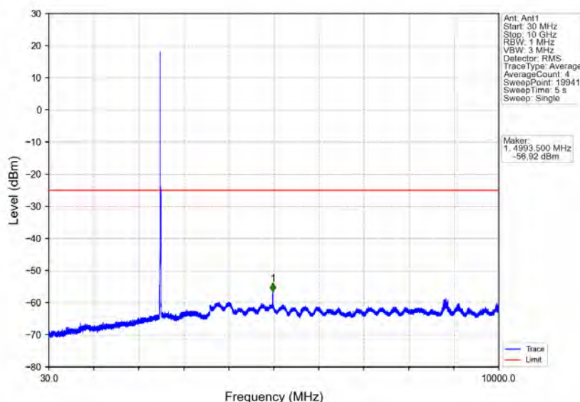
Band41_10MHz_64QAM_LCH_2501MHz_RB_1_0_NTNV
