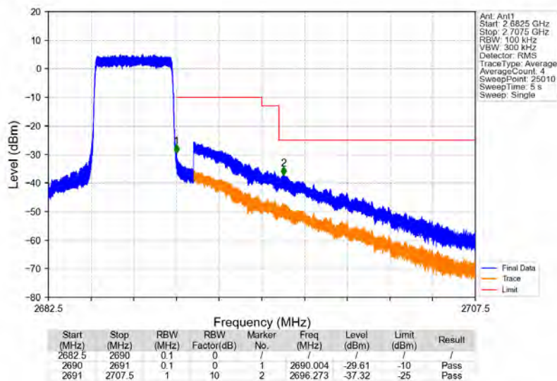
Band41_5MHz_16QAM_HCH_2687.5MHz_RB_25_0_NTNV
