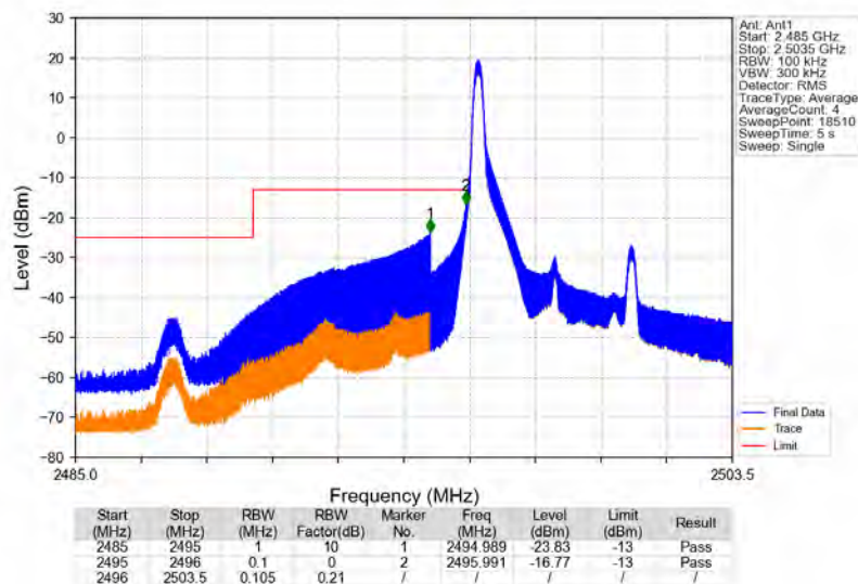
Band41_5MHz_16QAM_LCH_2498.5MHz_RB_1_0_NTNV
