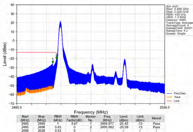
Band41_20MHz_16QAM_LCH_2506MHz_RB_1_0_NTNV
