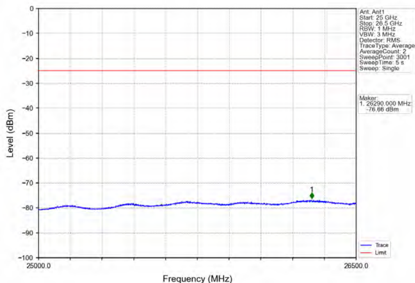
Band41_15MHz_64QAM_HCH_2682.5MHz_RB_1_74_NTNV
