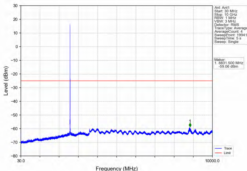
Band41_5MHz_64QAM_MCH_2593MHz_RB_1_0_NTNV
