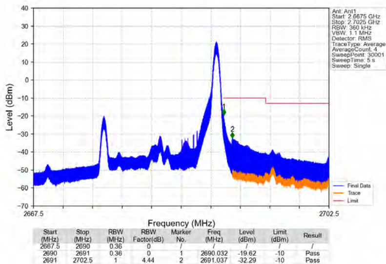
Band41_15MHz_64QAM_HCH_2682.5MHz_RB_1_74_NTNV
