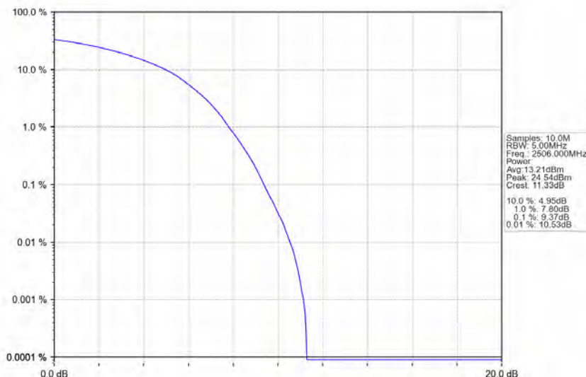
Band41_20MHz_64QAM_LCH_2506MHz_RB_100_0_NTNV
