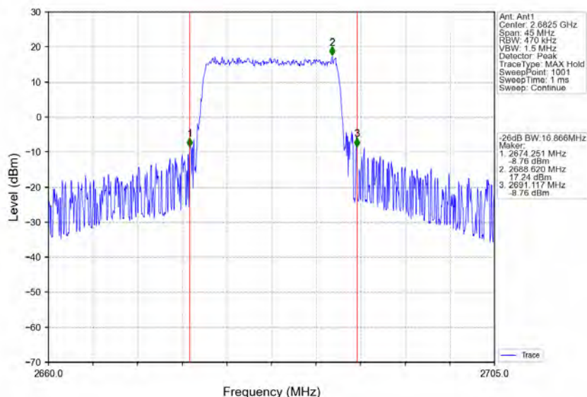
Band41_15MHz_16QAM_HCH_2682.5MHz_RB_75_0_NTNV
