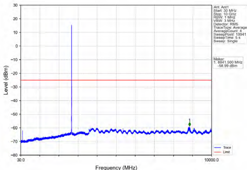
Band41_5MHz_16QAM_HCH_2687.5MHz_RB_1_0_NTNV
