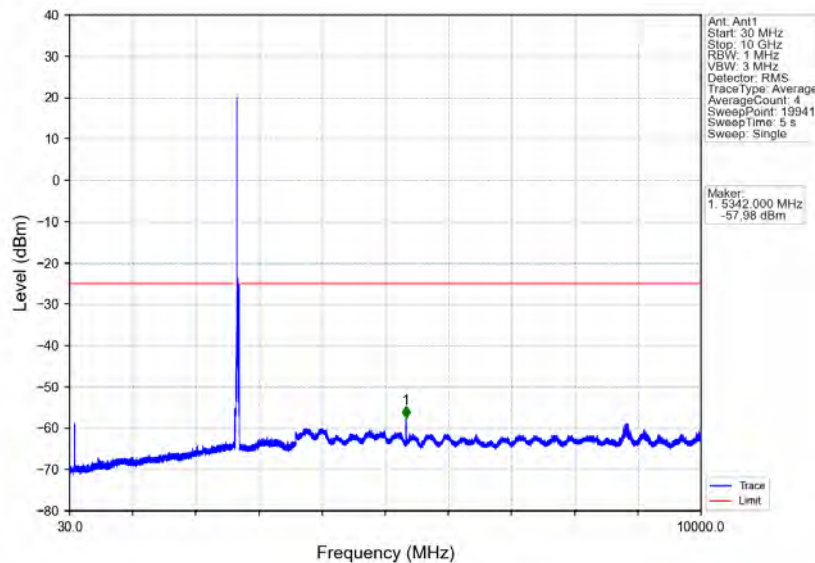
Band41_20MHz_16QAM_HCH_2680MHz_RB_1_0_NTNV
