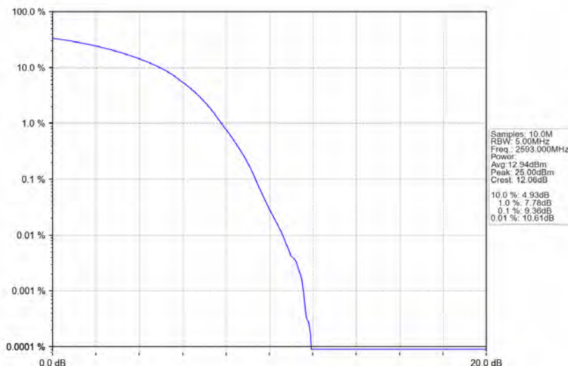
Band41_20MHz_64QAM_MCH_2593MHz_RB_100_0_NTNV
