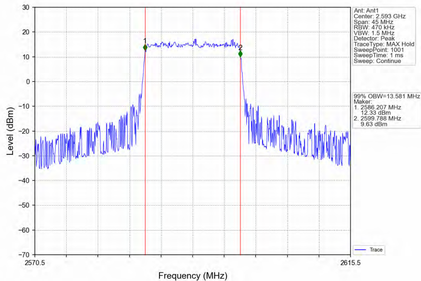
Band41_15MHz_64QAM_MCH_2593MHz_RB_75_0_NTNV
