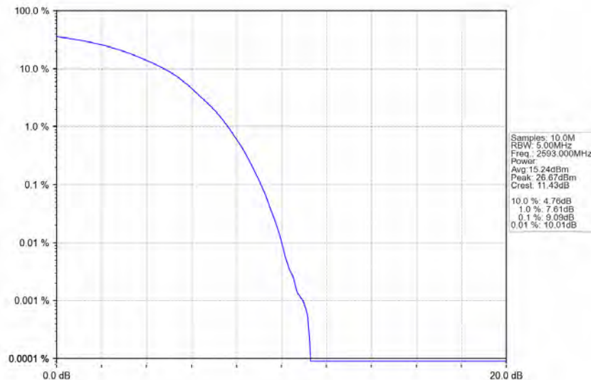
Band41_15MHz_16QAM_MCH_2593MHz_RB_75_0_NTNV
