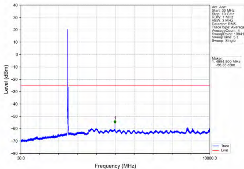
Band41_20MHz_16QAM_LCH_2506MHz_RB_1_0_NTNV
