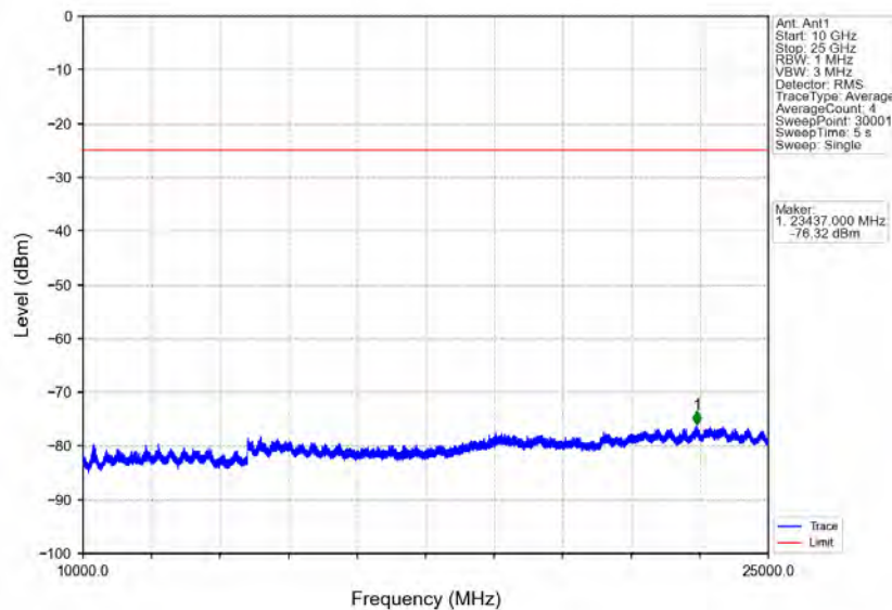
Band41_15MHz_16QAM_MCH_2593MHz_RB_1_0_NTNV
