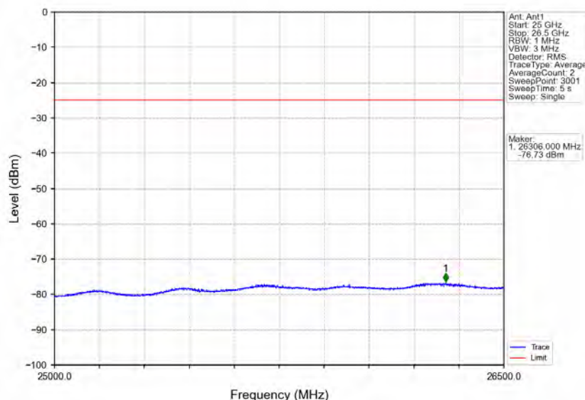
Band41_15MHz_64QAM_MCH_2593MHz_RB_1_0_NTNV
