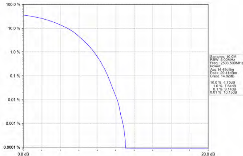
Band41_15MHz_64QAM_LCH_2503.5MHz_RB_75_0_NTNV
