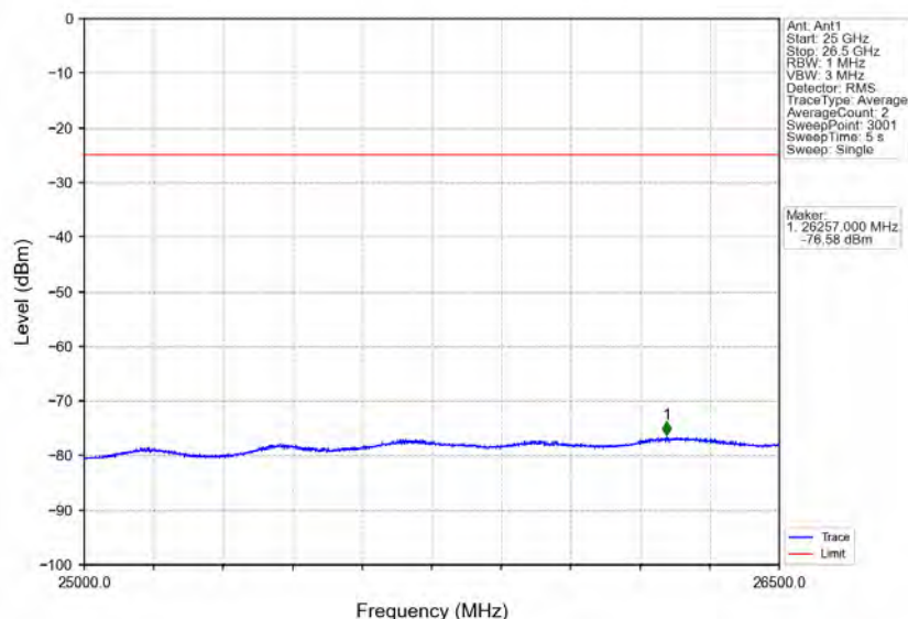
Band41_20MHz_64QAM_LCH_2506MHz_RB_1_0_NTNV
