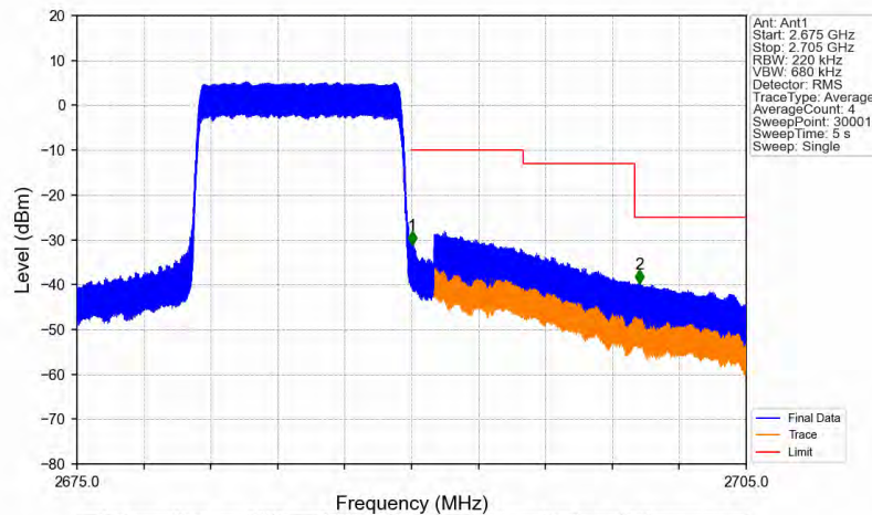
Band41_10MHz_64QAM_HCH_2685MHz_RB_50_0_NTNV
