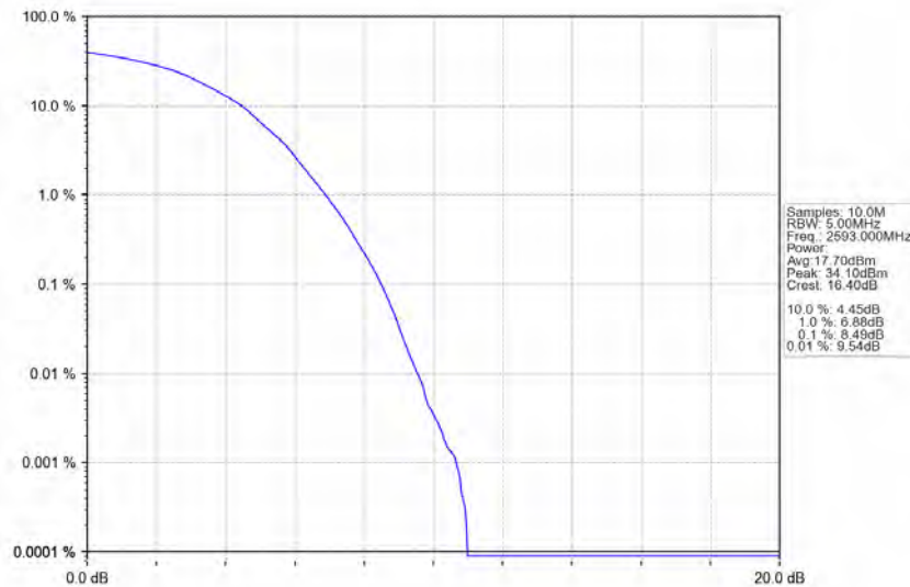
Band41_5MHz_64QAM_MCH_2593MHz_RB_25_0_NTNV
