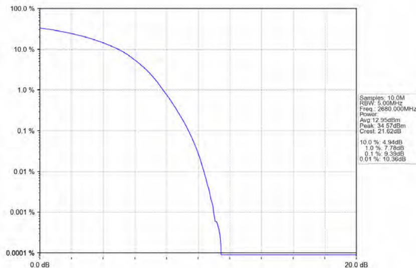
Band41_20MHz_64QAM_HCH_2680MHz_RB_100_0_NTNV
