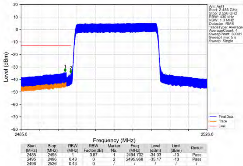
Band41_20MHz_64QAM_LCH_2506MHz_RB_100_0_NTNV
