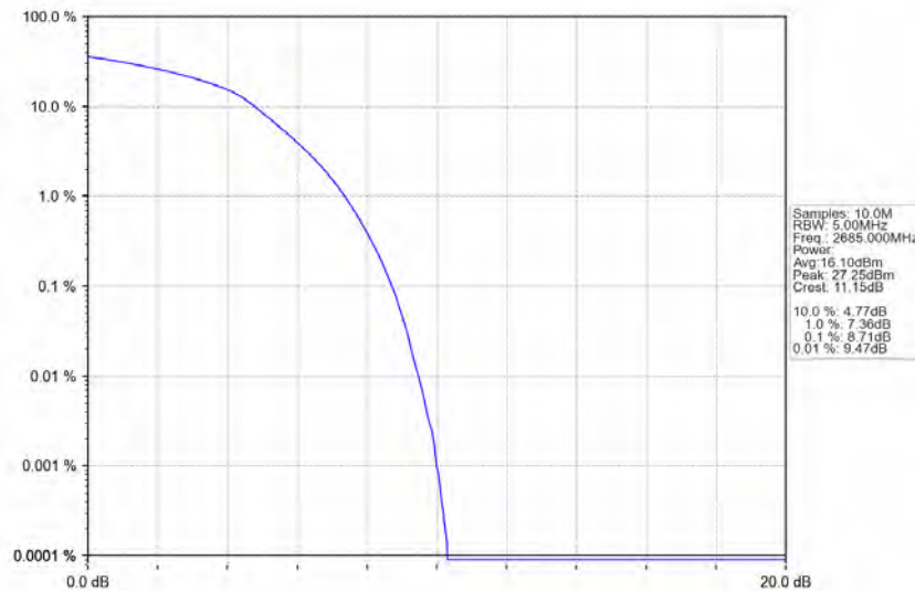
Band41_10MHz_64QAM_HCH_2685MHz_RB_50_0_NTNV
