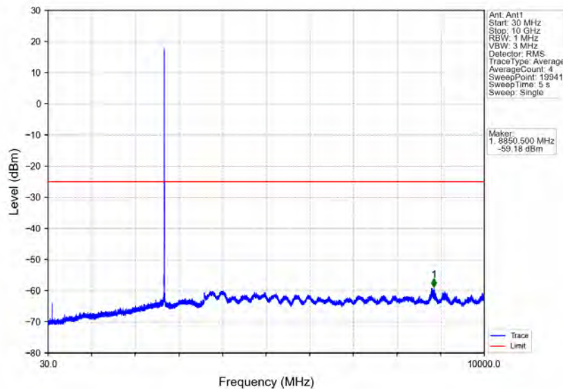
Band41_5MHz_64QAM_HCH_2687.5MHz_RB_1_0_NTNV
