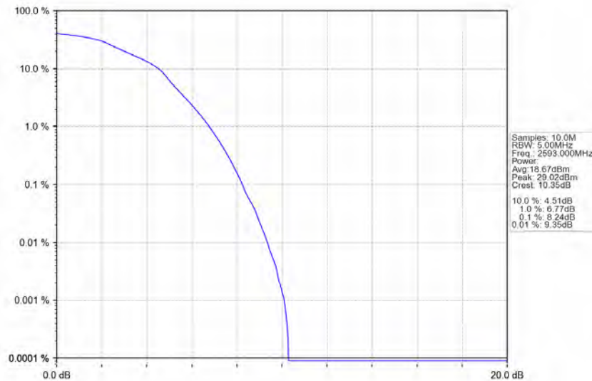
Band41_5MHz_16QAM_MCH_2593MHz_RB_25_0_NTNV
