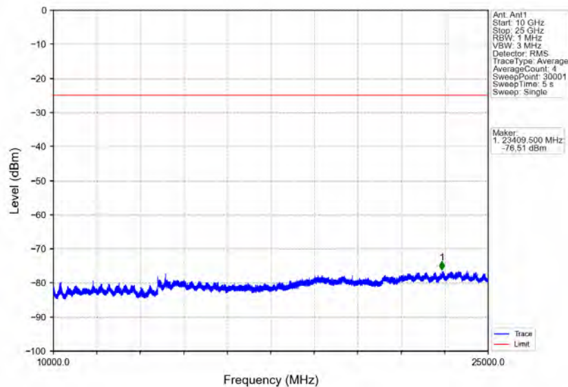
Band41_20MHz_16QAM_HCH_2680MHz_RB_1_0_NTNV
