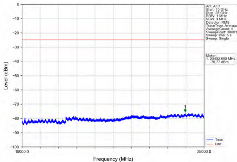
Band41_15MHz_16QAM_LCH_2503.5MHz_RB_1_0_NTNV
