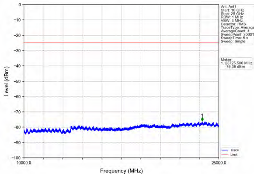
Band41_5MHz_16QAM_MCH_2593MHz_RB_1_0_NTNV
