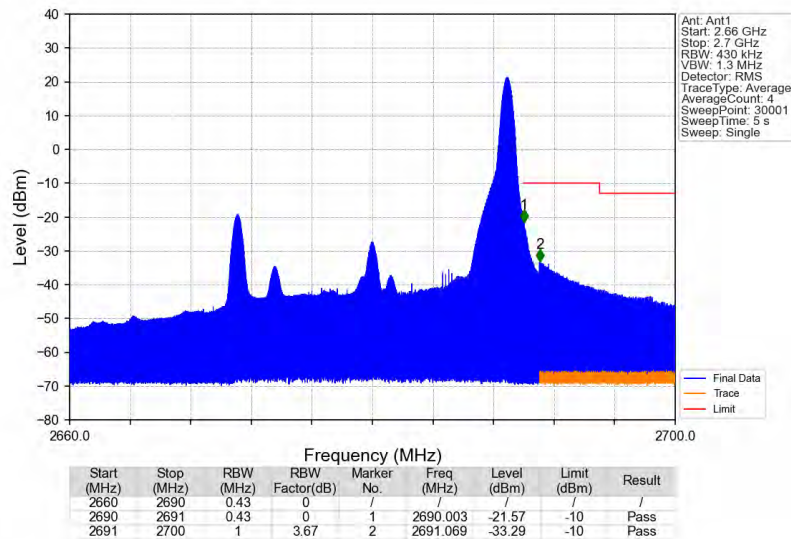
Band41_20MHz_64QAM_HCH_2680MHz_RB_1_99_NTNV
