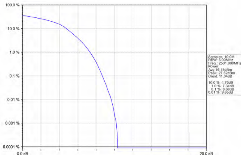
Band41_10MHz_64QAM_LCH_2501MHz_RB_50_0_NTNV
