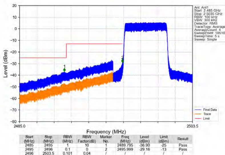
Band41_5MHz_16QAM_LCH_2498.5MHz_RB_25_0_NTNV
