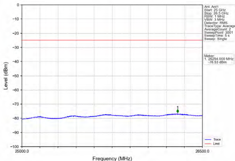
Band41_5MHz_16QAM_LCH_2498.5MHz_RB_25_0_NTNV
