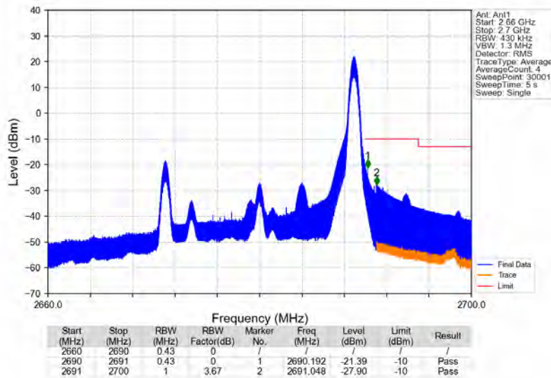
Band41_20MHz_16QAM_HCH_2680MHz_RB_1_99_NTNV
