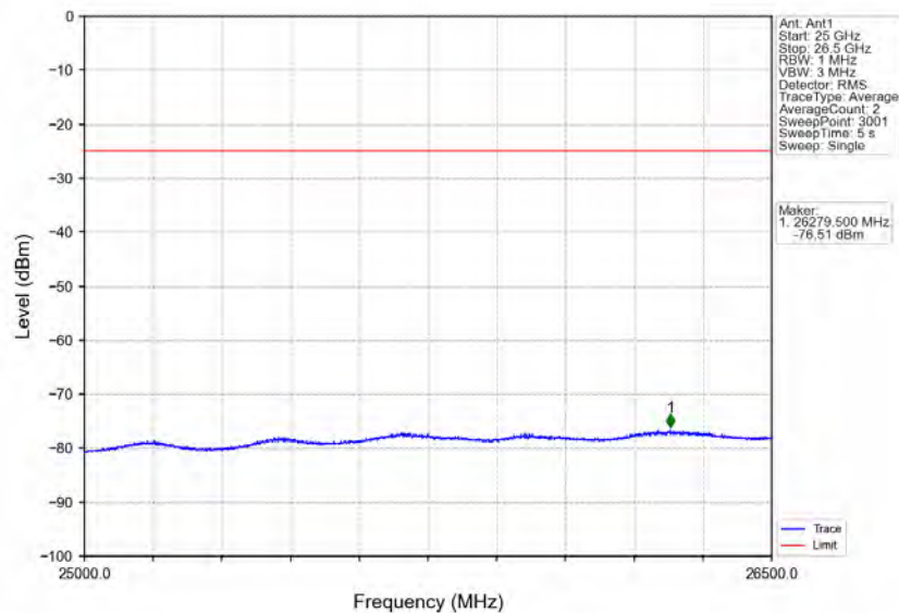
Band41_20MHz_64QAM_MCH_2593MHz_RB_1_0_NTNV
