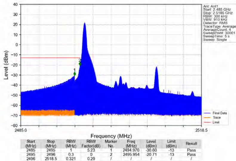
Band41_15MHz_64QAM_LCH_2503.5MHz_RB_1_0_NTNV
