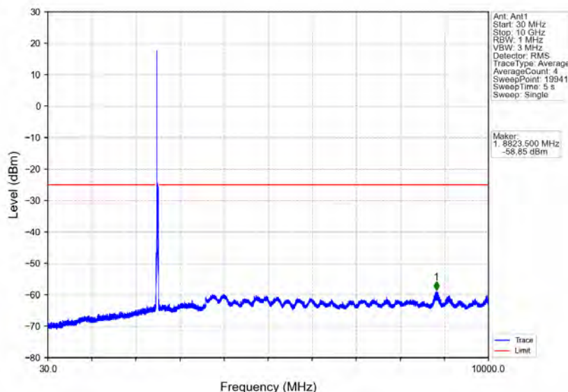
Band41_20MHz_64QAM_LCH_2506MHz_RB_1_0_NTNV
