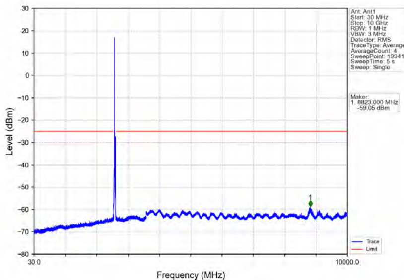
Band41_20MHz_64QAM_MCH_2593MHz_RB_1_0_NTNV
