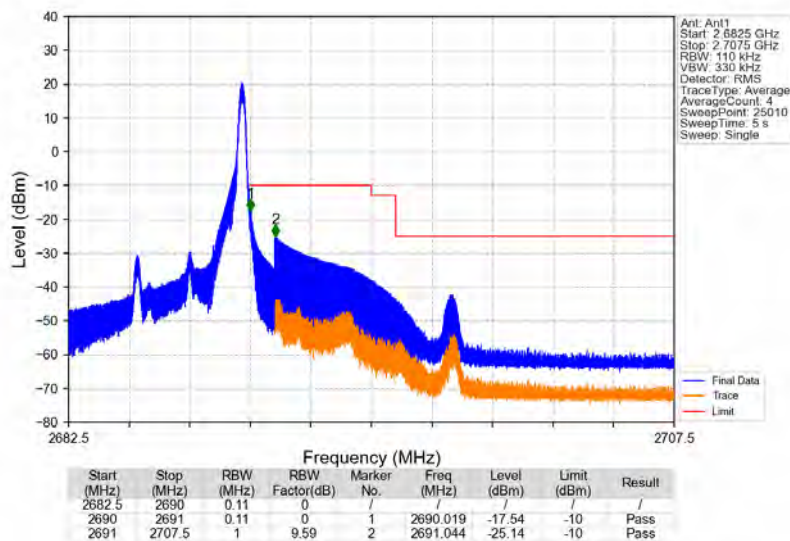
Band41_5MHz_16QAM_HCH_2687.5MHz_RB_1_24_NTNV
