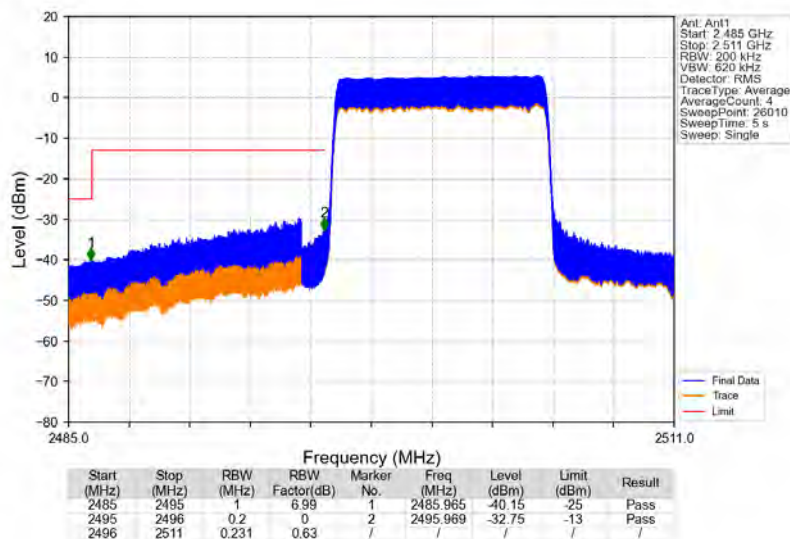
Band41_10MHz_64QAM_LCH_2501MHz_RB_50_0_NTNV
