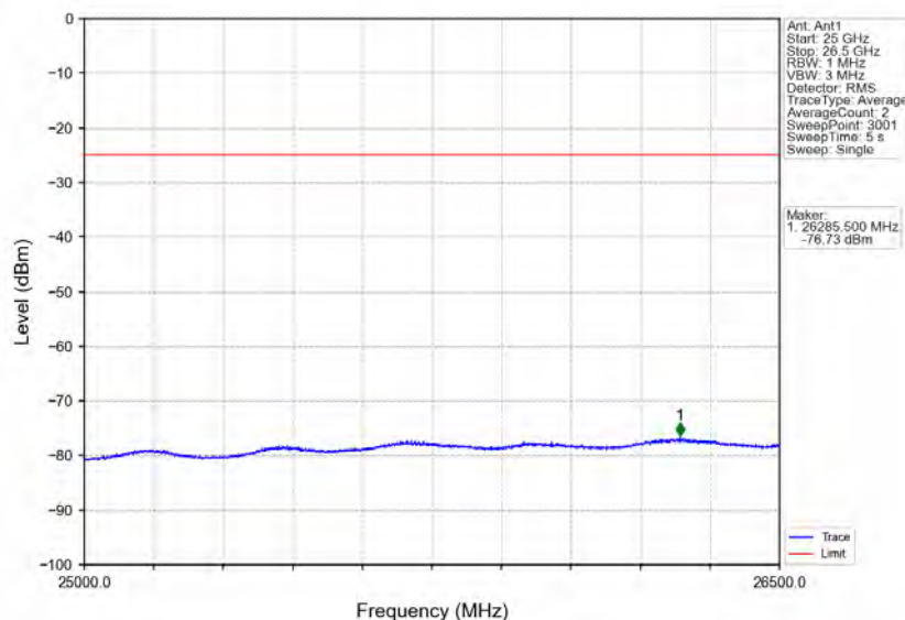
Band41_5MHz_64QAM_HCH_2687.5MHz_RB_1_24_NTNV
