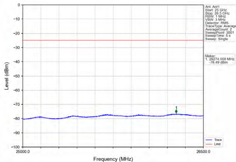
Band41_15MHz_16QAM_LCH_2503.5MHz_RB_75_0_NTNV
