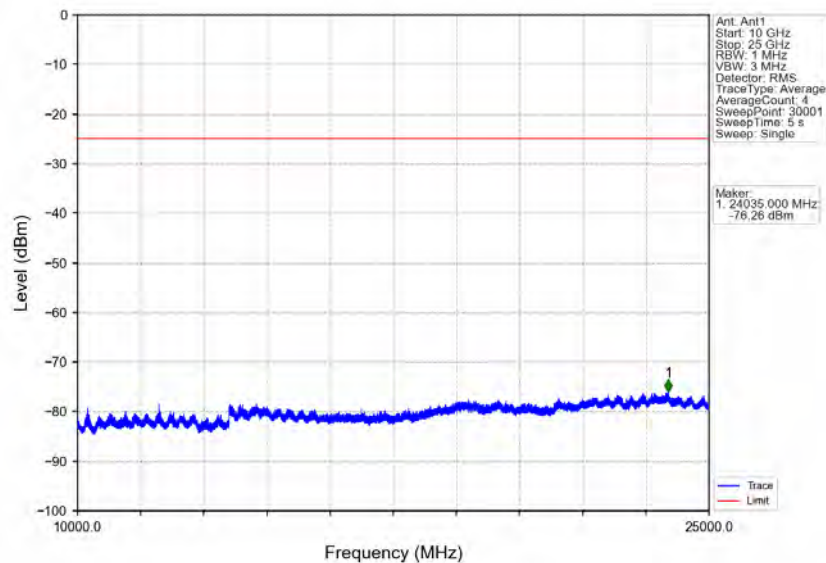
Band41_5MHz_64QAM_LCH_2498.5MHz_RB_1_0_NTNV
