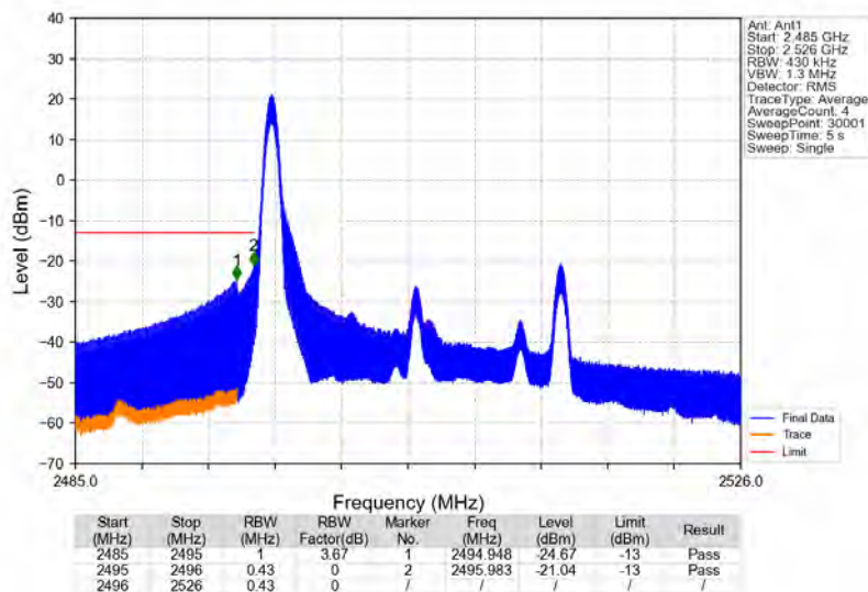
Band41_20MHz_64QAM_LCH_2506MHz_RB_1_0_NTNV
