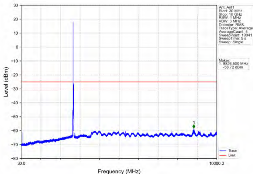
Band41_15MHz_64QAM_HCH_2682.5MHz_RB_1_0_NTNV
