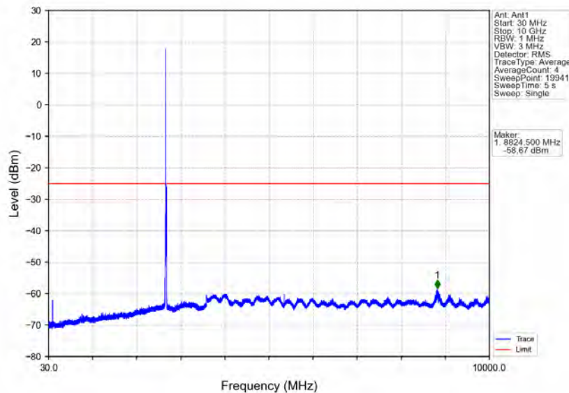
Band41_10MHz_64QAM_HCH_2685MHz_RB_1_0_NTNV
