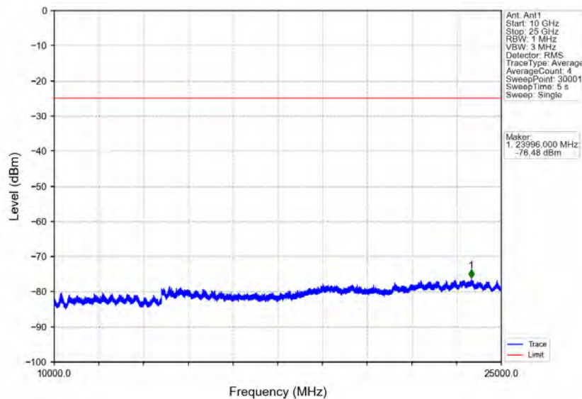
Band41_10MHz_64QAM_HCH_2685MHz_RB_1_0_NTNV
