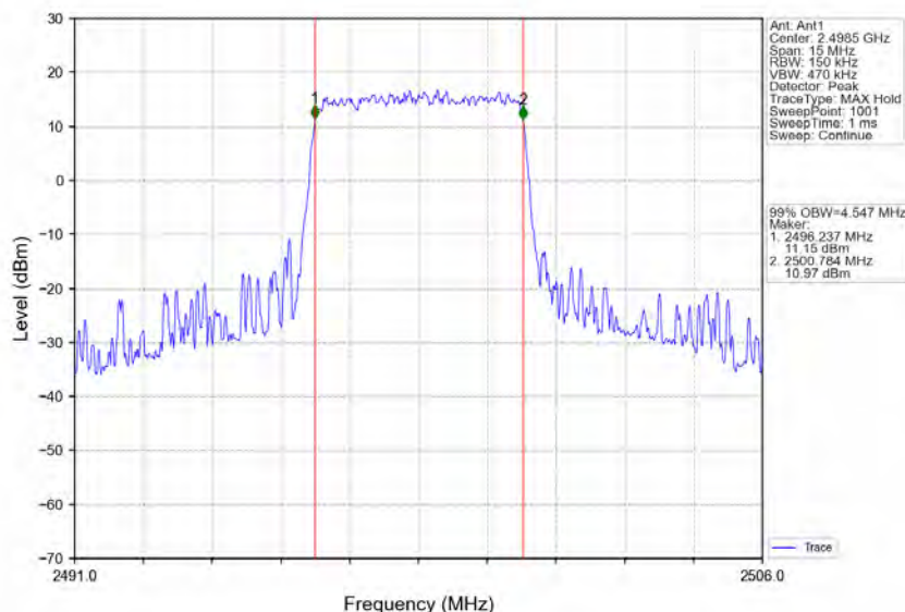
Band41_5MHz_16QAM_LCH_2498.5MHz_RB_25_0_NTNV
