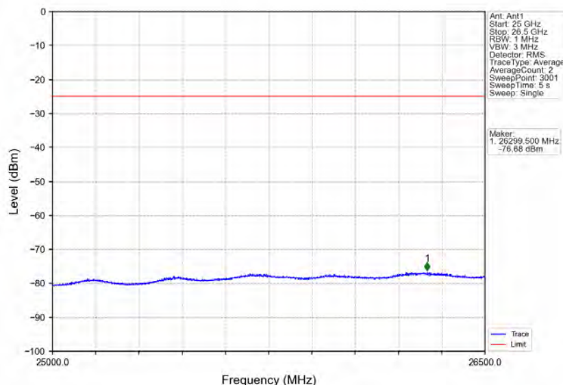
Band41_5MHz_64QAM_MCH_2593MHz_RB_1_0_NTNV
