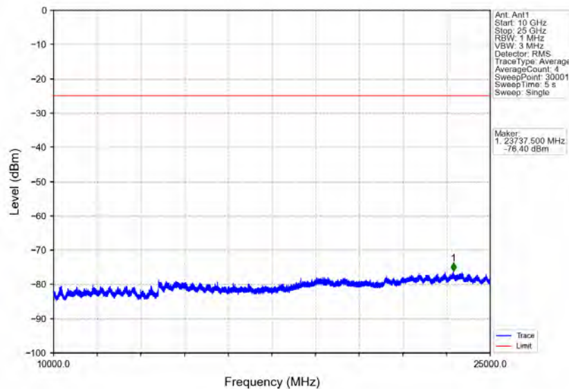
Band41_5MHz_16QAM_HCH_2687.5MHz_RB_1_0_NTNV
