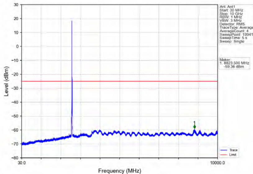
Band41_15MHz_16QAM_MCH_2593MHz_RB_1_0_NTNV
