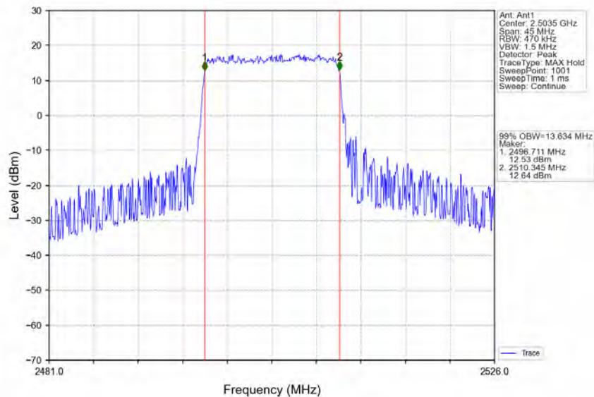
Band41_15MHz_16QAM_LCH_2503.5MHz_RB_75_0_NTNV
