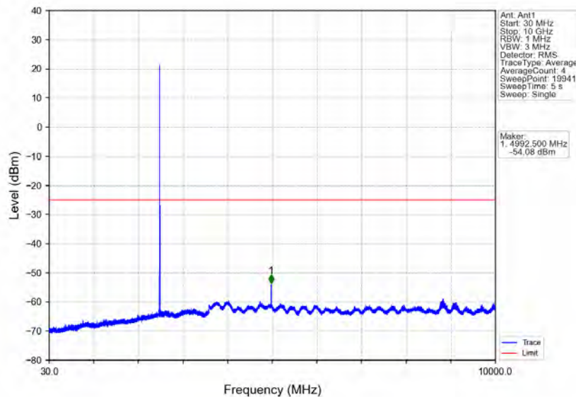
Band41_5MHz_16QAM_LCH_2498.5MHz_RB_1_0_NTNV
