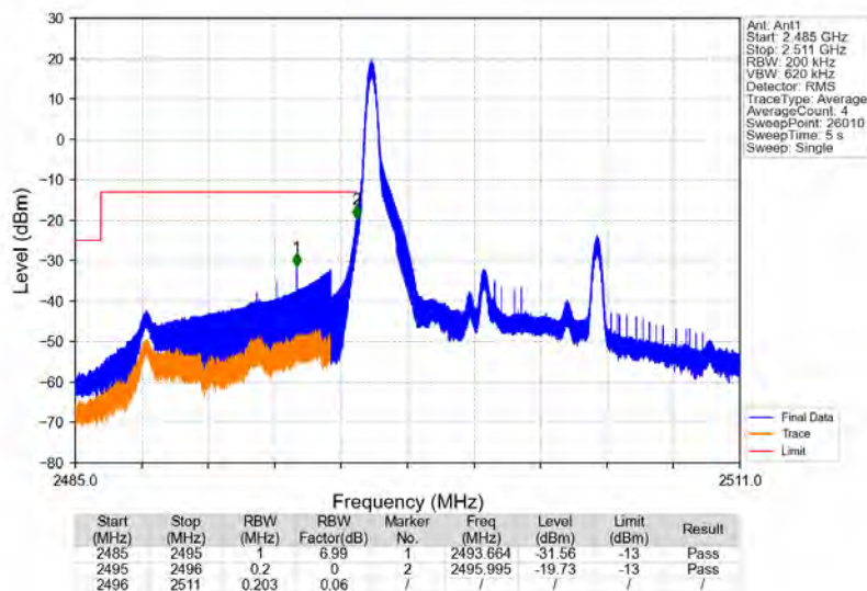
Band41_10MHz_64QAM_LCH_2501MHz_RB_1_0_NTNV
