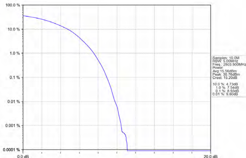
Band41_15MHz_16QAM_LCH_2503.5MHz_RB_75_0_NTNV
