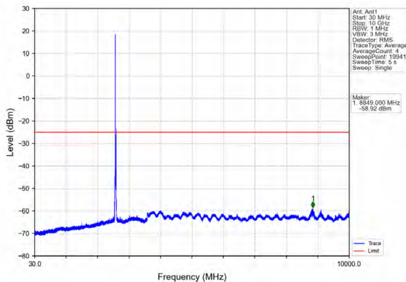
Band41_15MHz_64QAM_MCH_2593MHz_RB_1_0_NTNV
