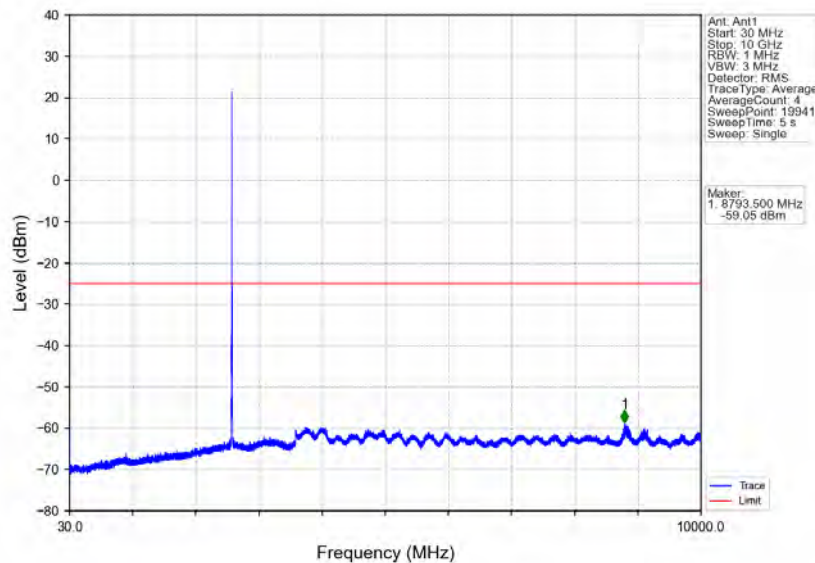
Band41_5MHz_16QAM_MCH_2593MHz_RB_1_0_NTNV
