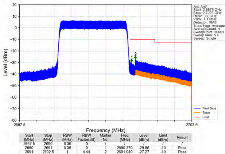
Band41_15MHz_16QAM_HCH_2682.5MHz_RB_75_0_NTNV
