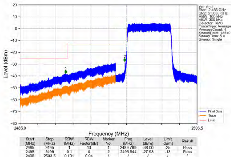
Band41_5MHz_64QAM_LCH_2498.5MHz_RB_25_0_NTNV
