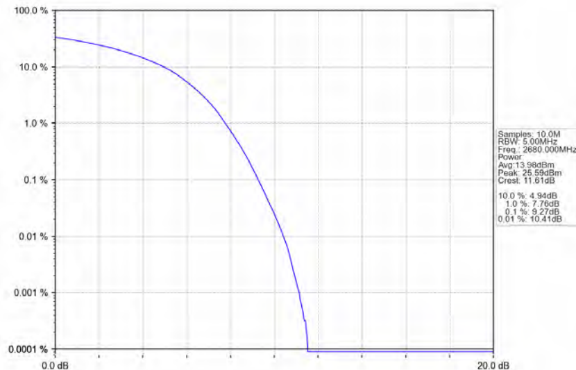
Band41_20MHz_16QAM_HCH_2680MHz_RB_100_0_NTNV
