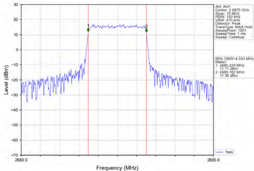
Band41_5MHz_16QAM_HCH_2687.5MHz_RB_25_0_NTNV
