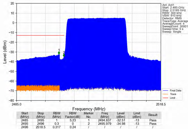
Band41_15MHz_64QAM_LCH_2503.5MHz_RB_75_0_NTNV
