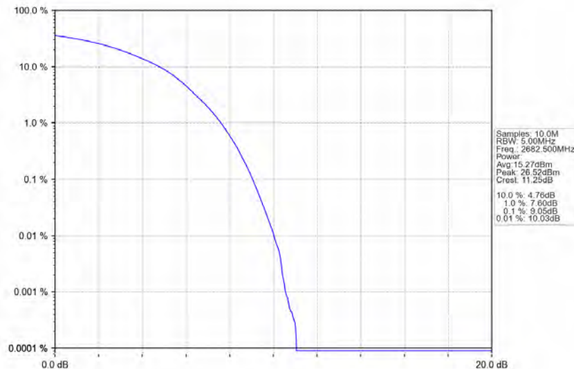
Band41_15MHz_16QAM_HCH_2682.5MHz_RB_75_0_NTNV
