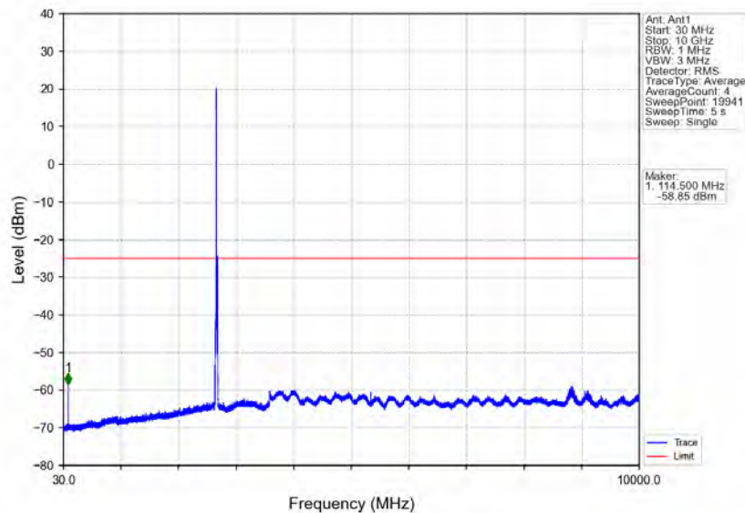
Band41_15MHz_16QAM_HCH_2682.5MHz_RB_1_0_NTNV
