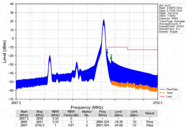
Band41_15MHz_16QAM_HCH_2682.5MHz_RB_1_74_NTNV
