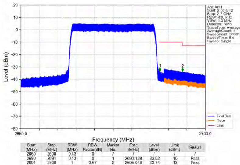
Band41_20MHz_16QAM_HCH_2680MHz_RB_100_0_NTNV
