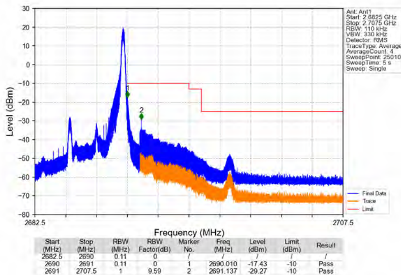
Band41_5MHz_64QAM_HCH_2687.5MHz_RB_1_24_NTNV
