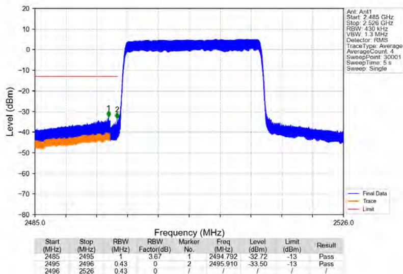
Band41_20MHz_16QAM_LCH_2506MHz_RB_100_0_NTNV
