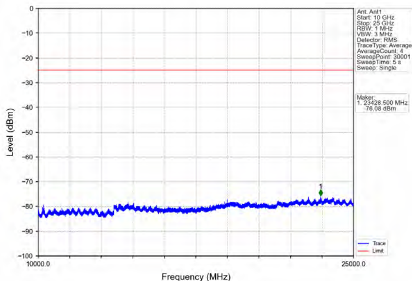
Band41_15MHz_16QAM_HCH_2682.5MHz_RB_1_0_NTNV
