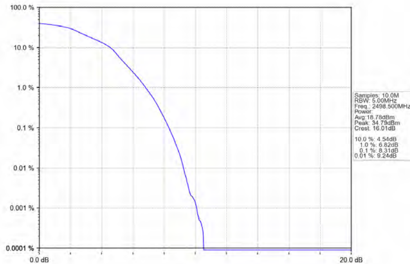
Band41_5MHz_16QAM_LCH_2498.5MHz_RB_25_0_NTNV
