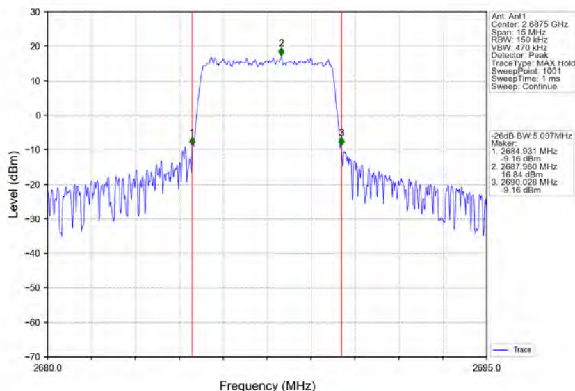
Band41_5MHz_16QAM_HCH_2687.5MHz_RB_25_0_NTNV
