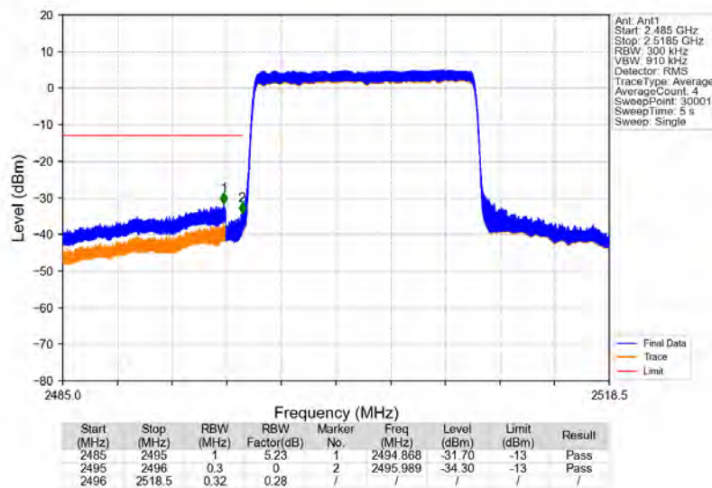
Band41_15MHz_16QAM_LCH_2503.5MHz_RB_75_0_NTNV
