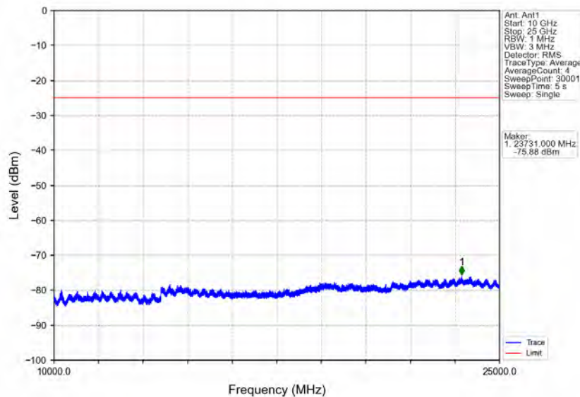
Band41_5MHz_16QAM_LCH_2498.5MHz_RB_1_0_NTNV
