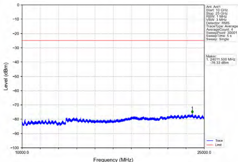
Band41_15MHz_64QAM_HCH_2682.5MHz_RB_1_0_NTNV
