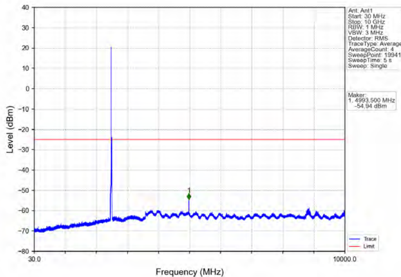
Band41_15MHz_16QAM_LCH_2503.5MHz_RB_1_0_NTNV
