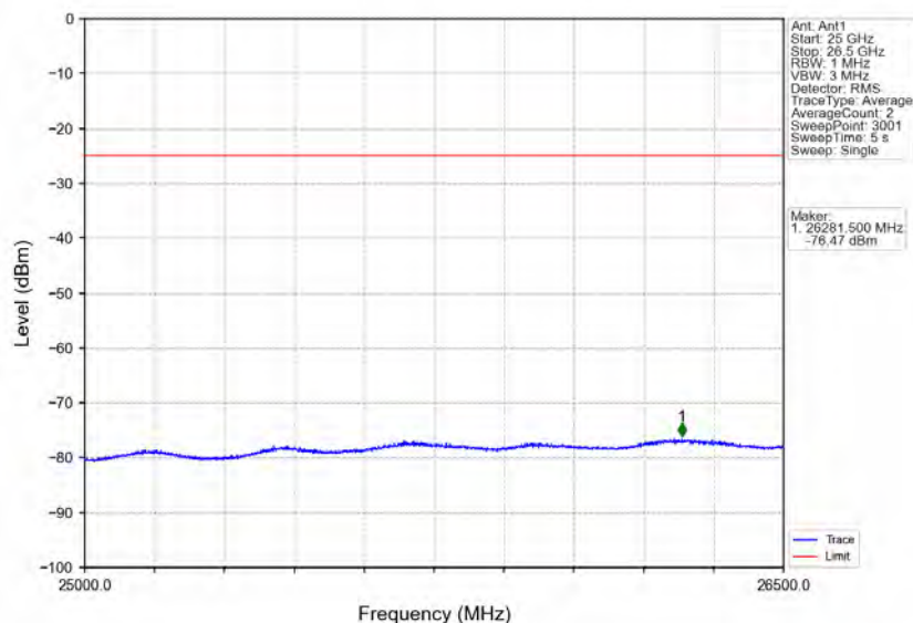
Band41_20MHz_16QAM_LCH_2506MHz_RB_100_0_NTNV
