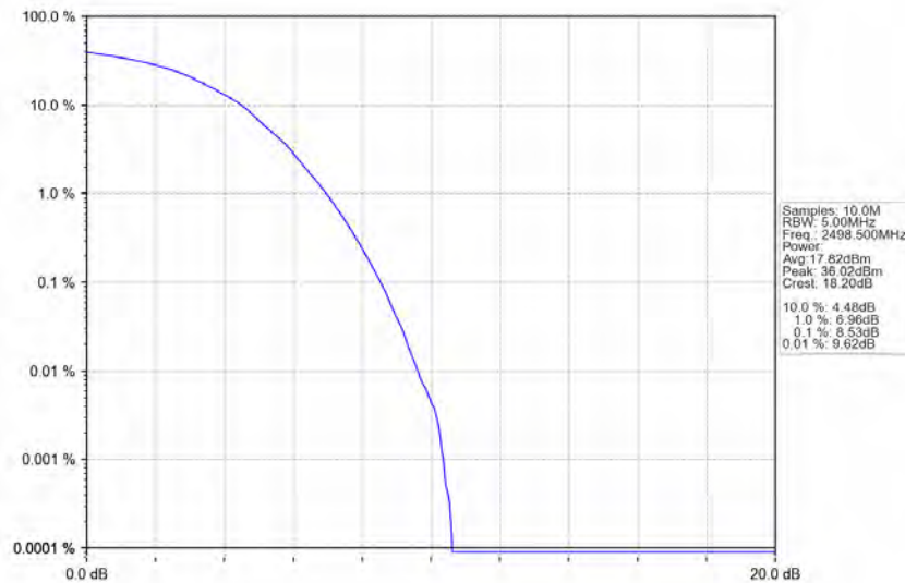
Band41_5MHz_64QAM_LCH_2498.5MHz_RB_25_0_NTNV
