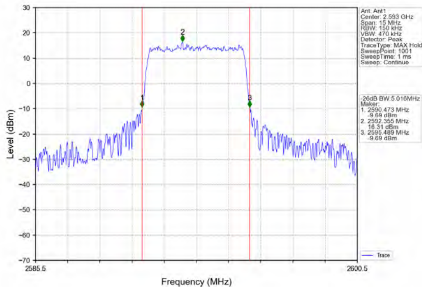
Band41_5MHz_64QAM_MCH_2593MHz_RB_25_0_NTNV
