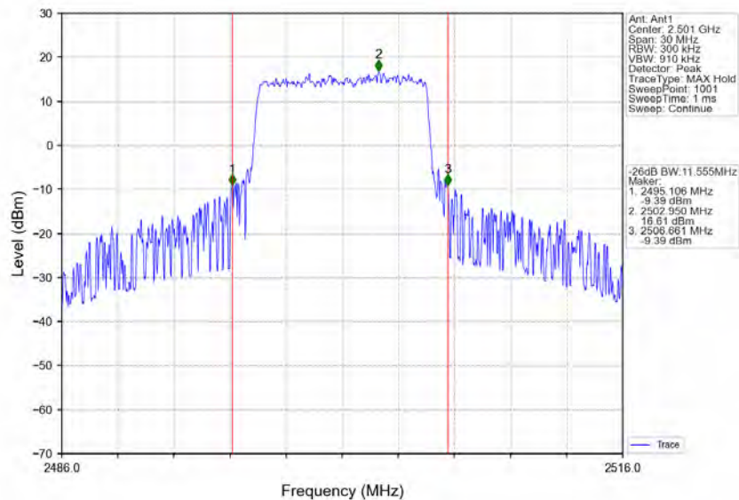
Band41_10MHz_64QAM_LCH_2501MHz_RB_50_0_NTNV
