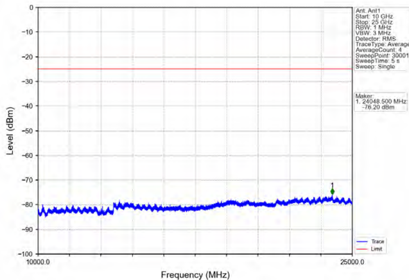
Band41_5MHz_64QAM_HCH_2687.5MHz_RB_1_0_NTNV
