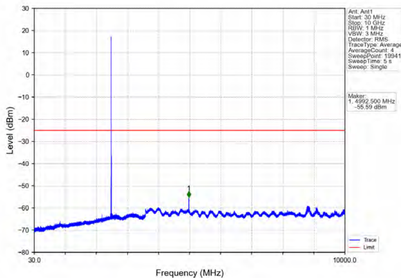
Band41_5MHz_64QAM_LCH_2498.5MHz_RB_1_0_NTNV
