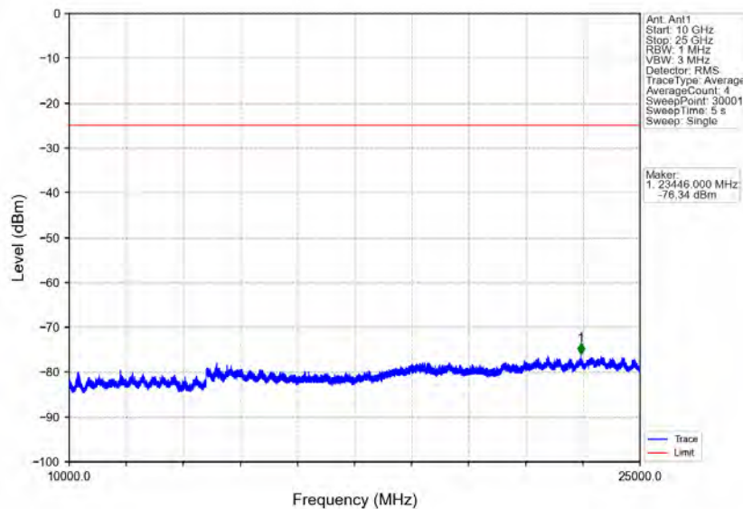
Band41_20MHz_64QAM_HCH_2680MHz_RB_1_0_NTNV
