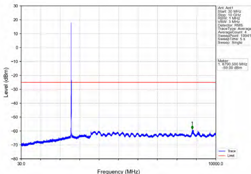
Band41_10MHz_64QAM_MCH_2593MHz_RB_1_0_NTNV
