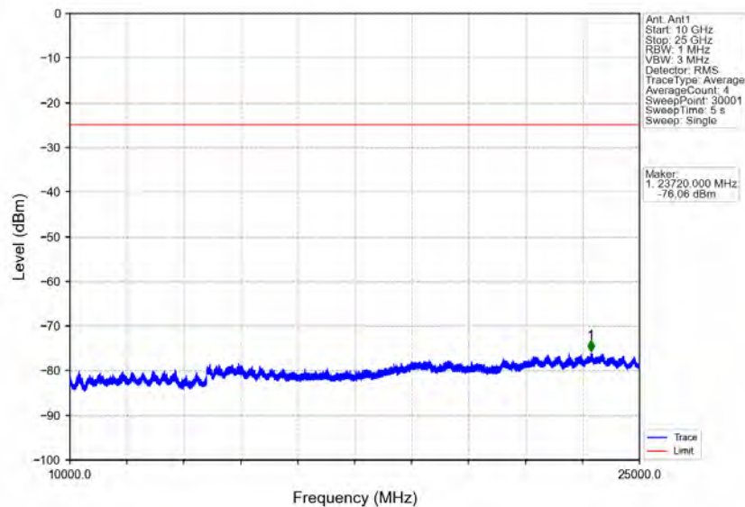
Band41_15MHz_64QAM_LCH_2503.5MHz_RB_1_0_NTNV
