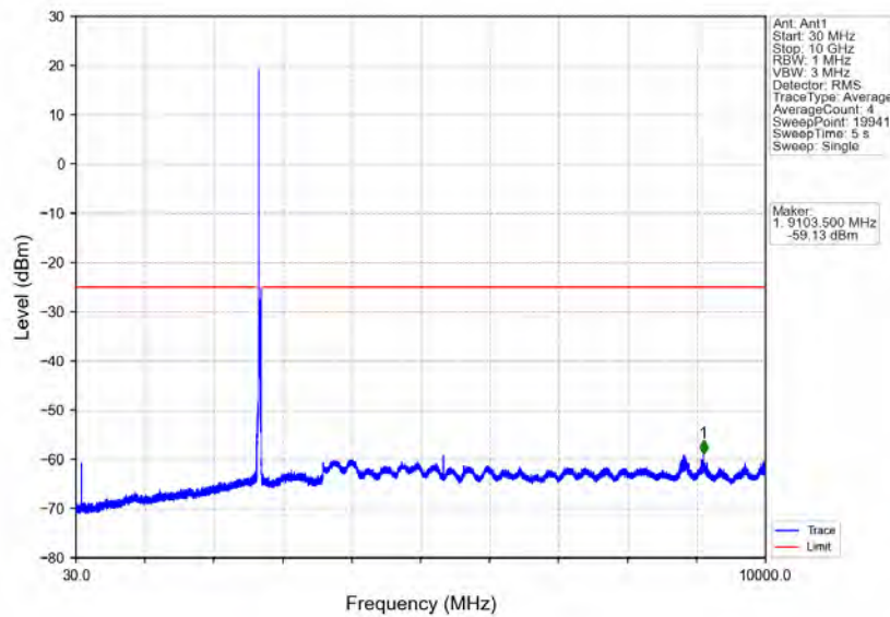
Band41_20MHz_64QAM_HCH_2680MHz_RB_1_0_NTNV
