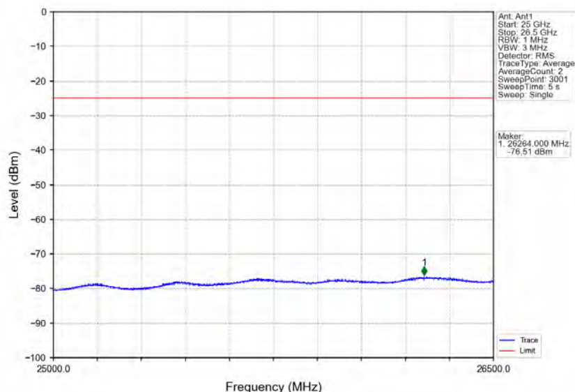
Band41_10MHz_64QAM_LCH_2501MHz_RB_1_0_NTNV
