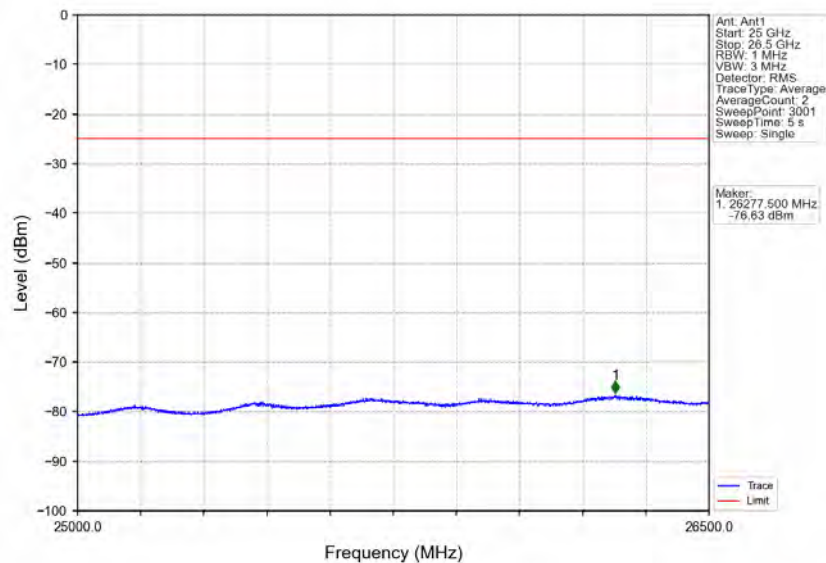
Band41_20MHz_64QAM_HCH_2680MHz_RB_1_99_NTNV
