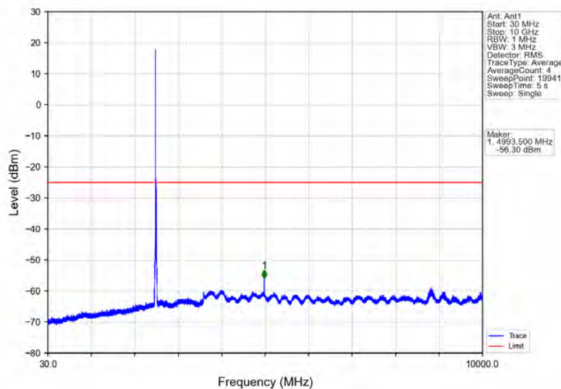
Band41_15MHz_64QAM_LCH_2503.5MHz_RB_1_0_NTNV
