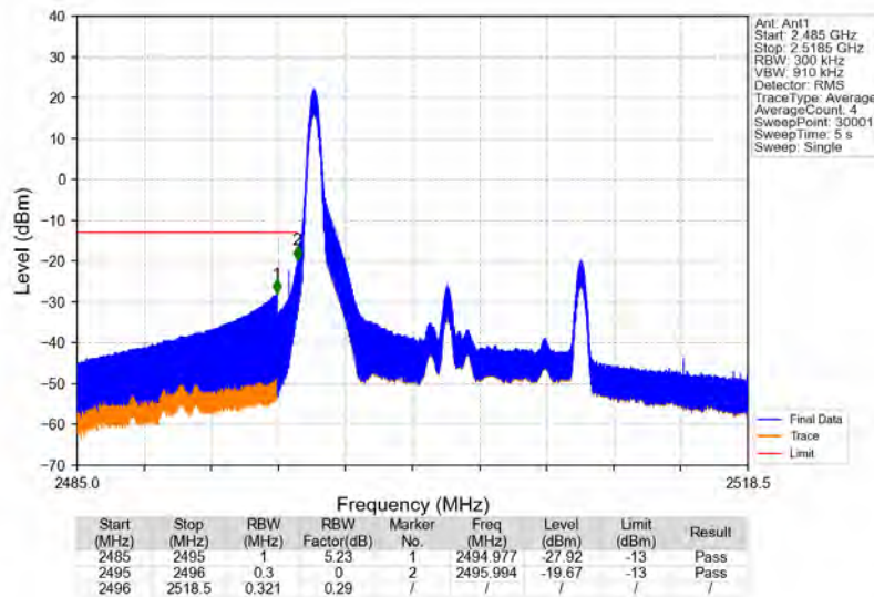
Band41_15MHz_16QAM_LCH_2503.5MHz_RB_1_0_NTNV
