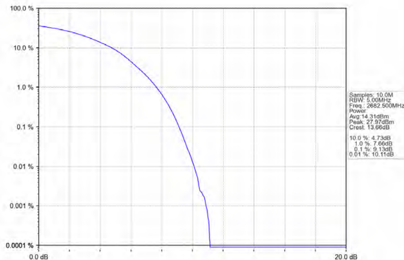
Band41_15MHz_64QAM_HCH_2682.5MHz_RB_75_0_NTNV
