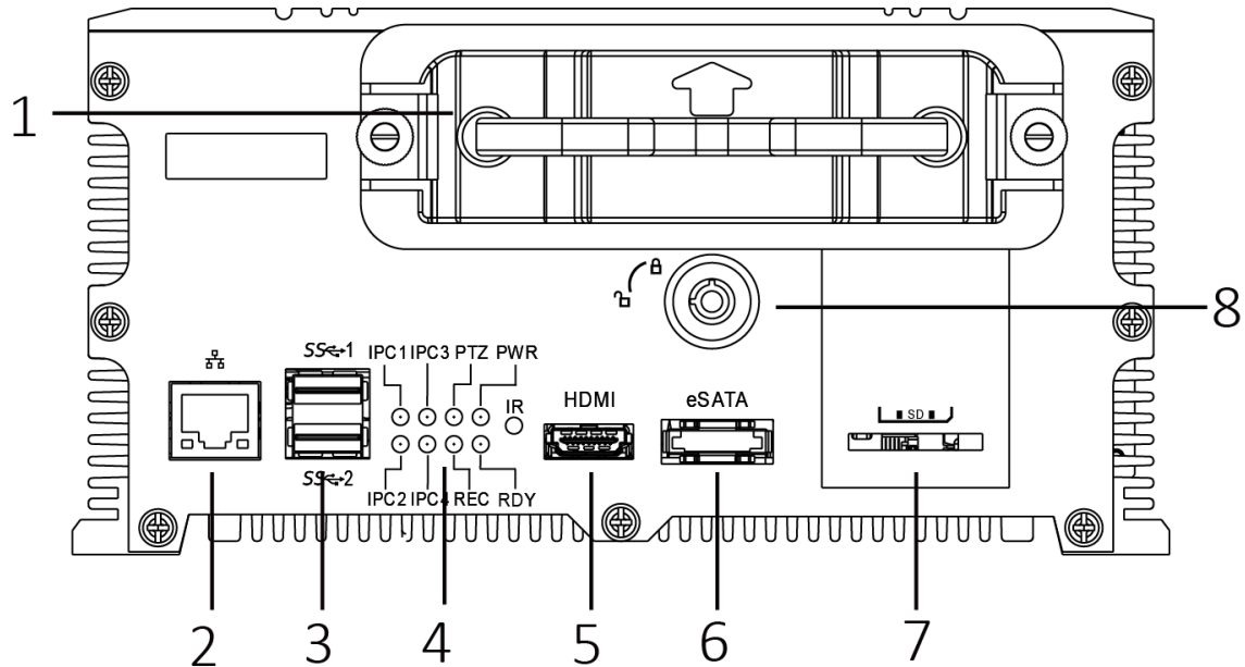
Figure 2-1 Front Panel
