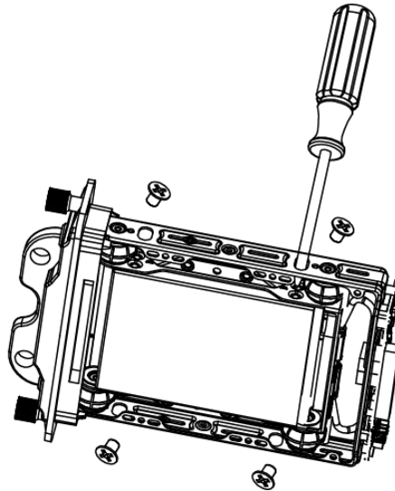
Figure 3-5 Fix HDD
