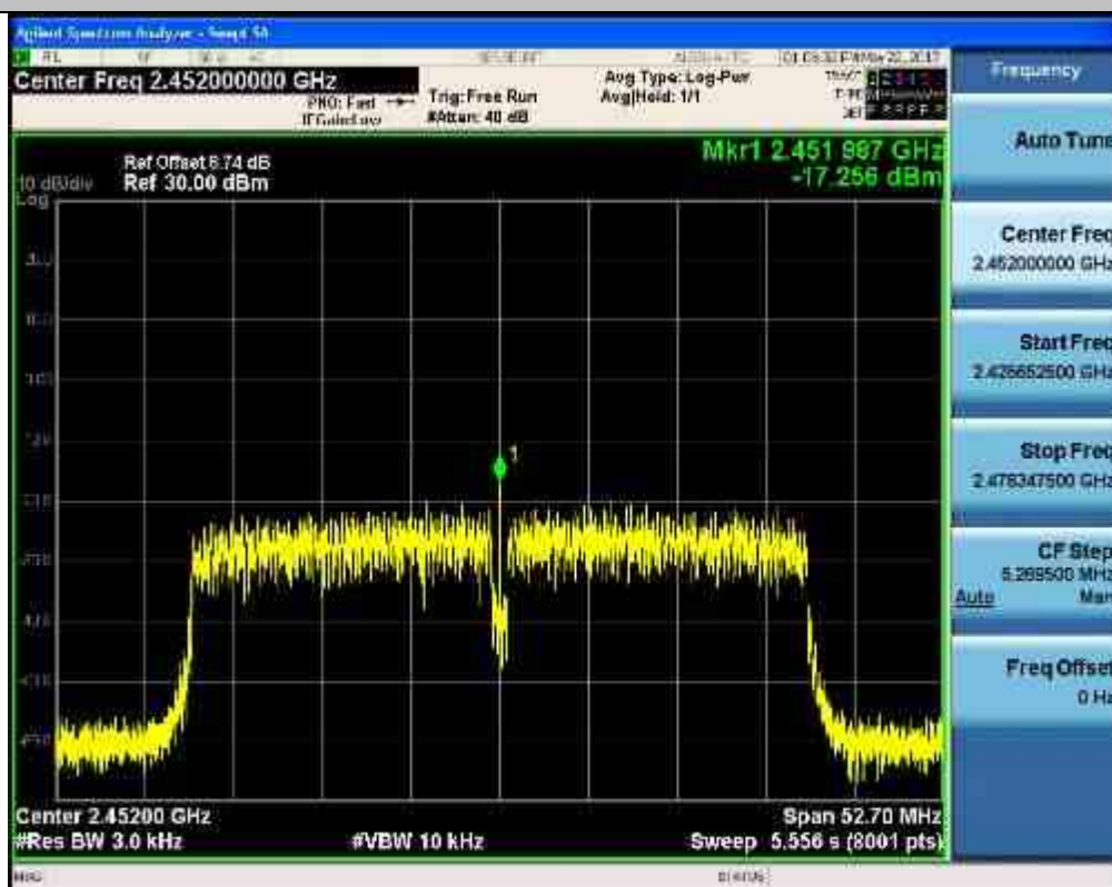
Maximum Peak power spectral density_11N40SISO_2452_ANT0
