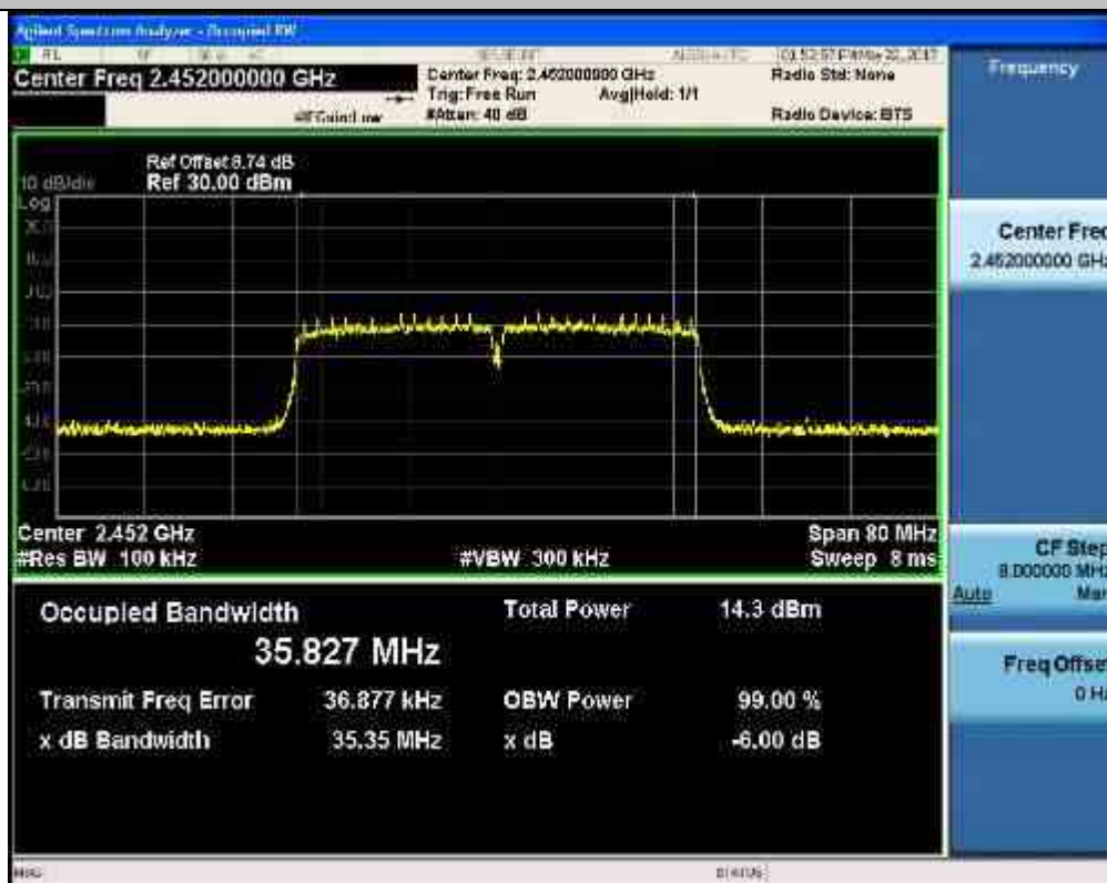
6dB Bandwidth_11N40SISO_2452_ANT1
