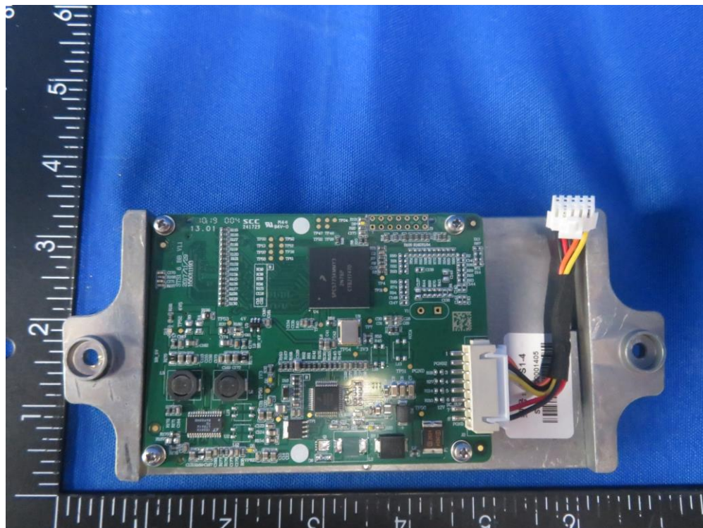
(6) EUT Photo (Radar Module)
