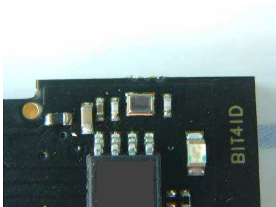
Oscillator view
