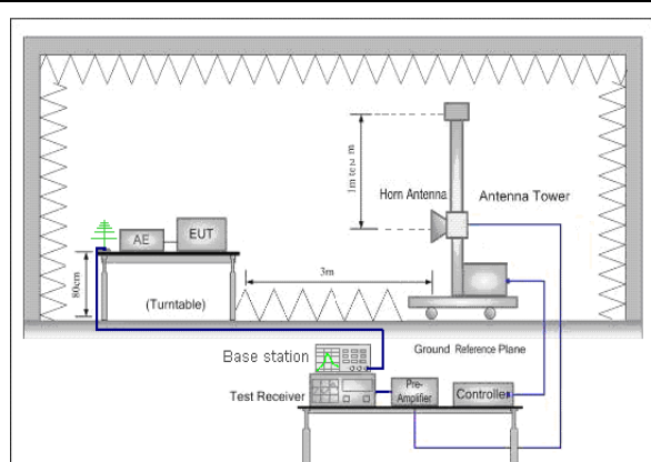
Figure 2. above 1GHz
