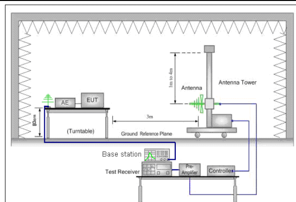
Figure 1. 30MHz to 1GHz
