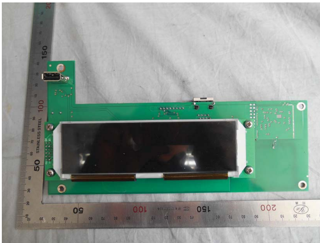
FIGURE 7 COFFEE DISPENSER (M/N: EC/USCUL120V-I) PANEL BOARD (COMPONENT SIDE)
