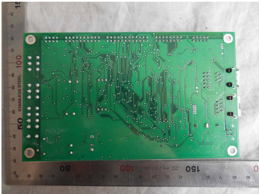
FIGURE 16 COFFEE DISPENSER (M/N: EC/USCUL120V-I) MAIN BOARD (SOLDERED SIDE)
