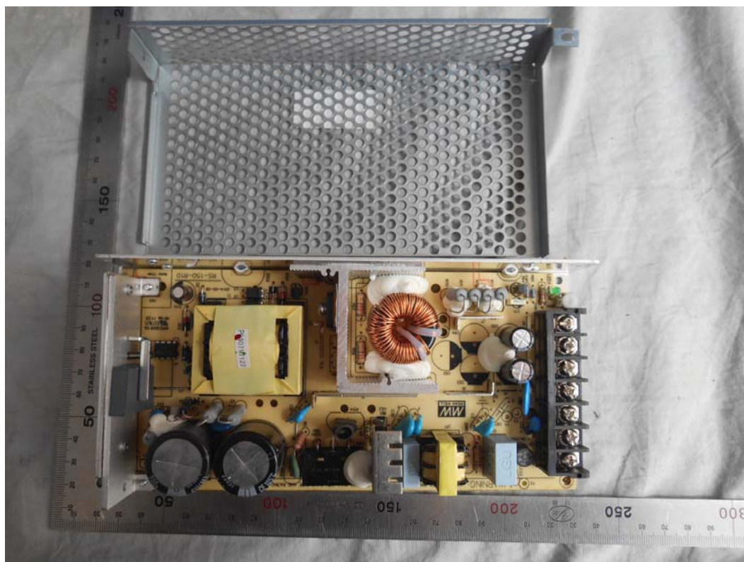
FIGURE 21 COFFEE DISPENSER (M/N: EC/USCUL120V-I) POWER SUPPLY COVER REMOVED
