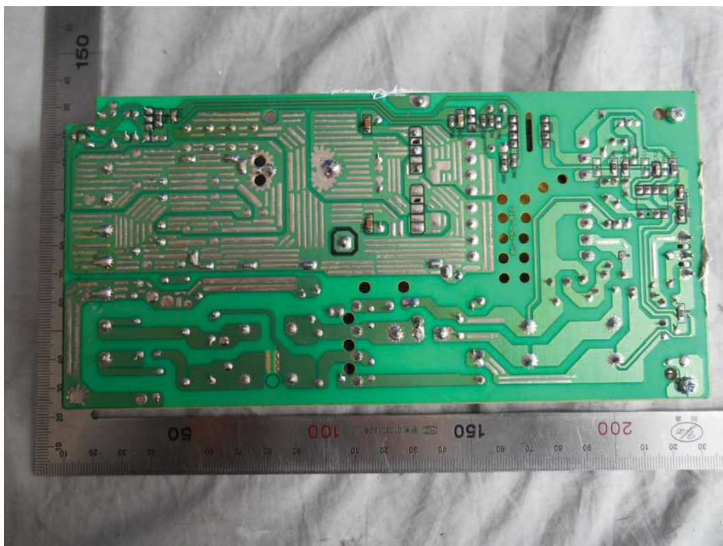
FIGURE 23 COFFEE DISPENSER (M/N: EC/USCUL120V-I) POWER SUPPLY (SOLDERED SIDE)
