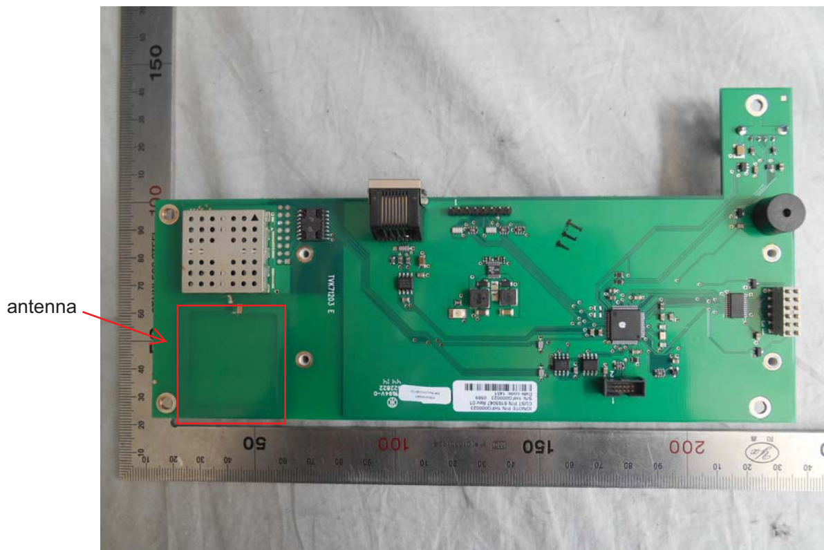
FIGURE 8 COFFEE DISPENSER (M/N: EC/USCUL120V-I) PANEL BOARD (SOLDERED SIDE)
