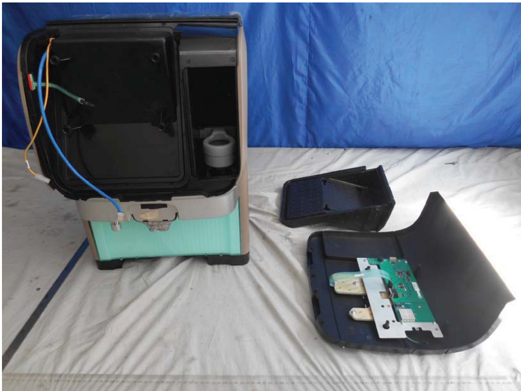
FIGURE 6 COFFEE DISPENSER (M/N: EC/UScUL120V-I) COVER REMOVED #1
