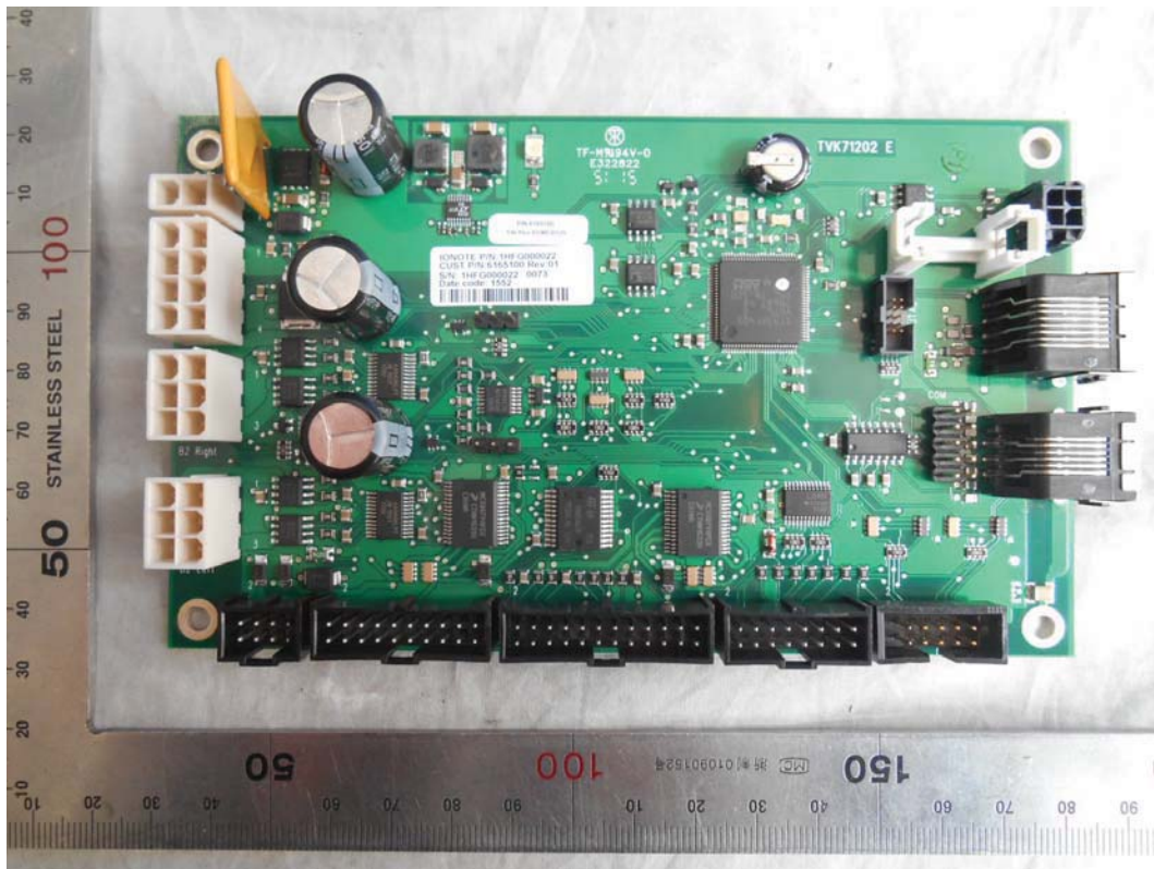
FIGURE 15 COFFEE DISPENSER (M/N: EC/USCUL120V-I) MAIN BOARD (COMPONENT SIDE)
