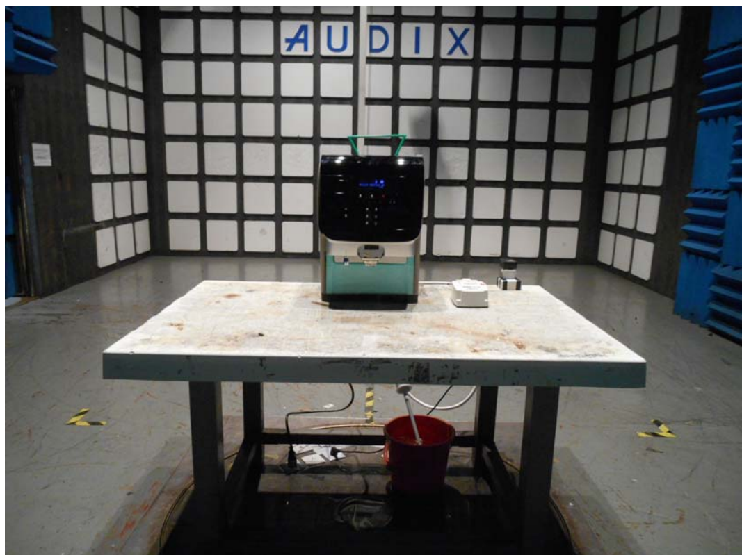
BACK VIEW OF RADIATED EMISSION TEST (ABOVE 30MHz)
