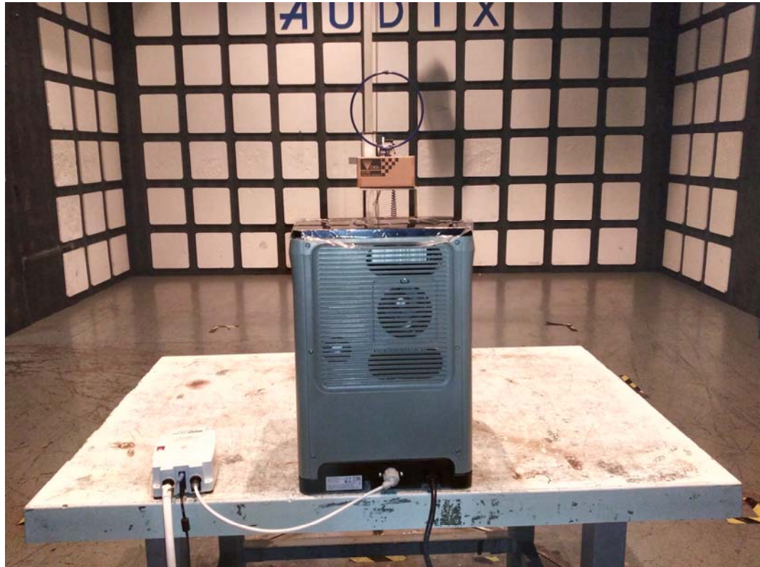
FRONT VIEW OF RADIATED EMISSION TEST (BELOW 30MHz)
