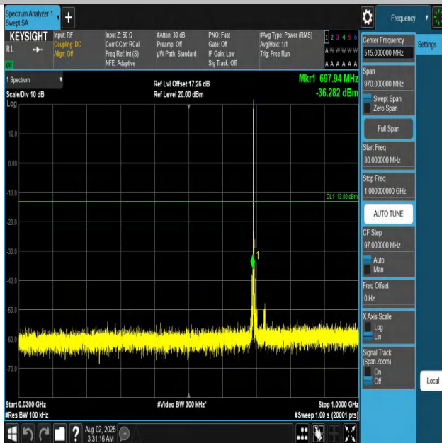
Band12-5MHz-QPSK-23035-1RB#0-30~1000-PASS
