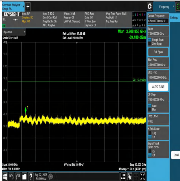
Band12-1.4MHz-QPSK-23017-1RB#0-3000~10000-PASS
