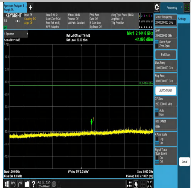
Band12-1.4MHz-QPSK-23173-1RB#0-1000~3000-PASS
