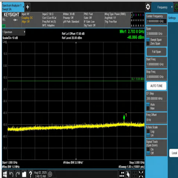
Band12-10MHz-QPSK-23130-1RB#0-1000~3000-PASS
