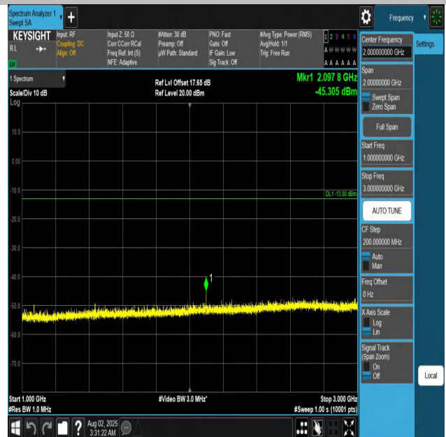
Band12-5MHz-QPSK-23035-1RB#0-1000~3000-PASS
