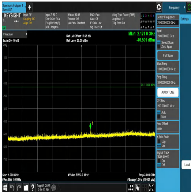
Band12-1.4MHz-QPSK-23095-1RB#0-1000~3000-PASS
