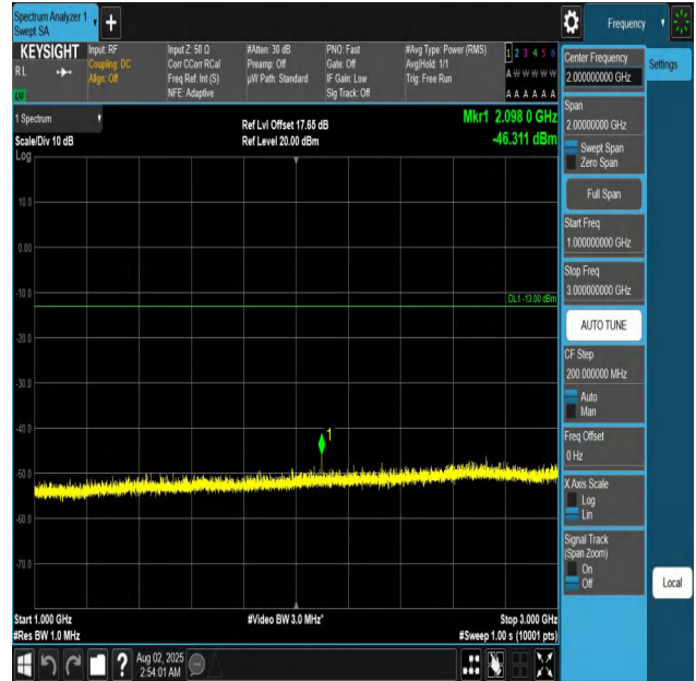
Band12-1.4MHz-QPSK-23017-1RB#0-1000~3000-PASS
