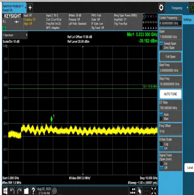
Band12-3MHz-QPSK-23095-1RB#0-3000~10000-PASS
