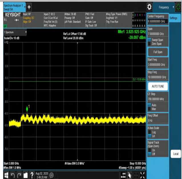
Band12-10MHz-QPSK-23130-1RB#0-3000~10000-PASS
