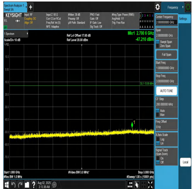
Band12-3MHz-QPSK-23095-1RB#0-1000~3000-PASS
