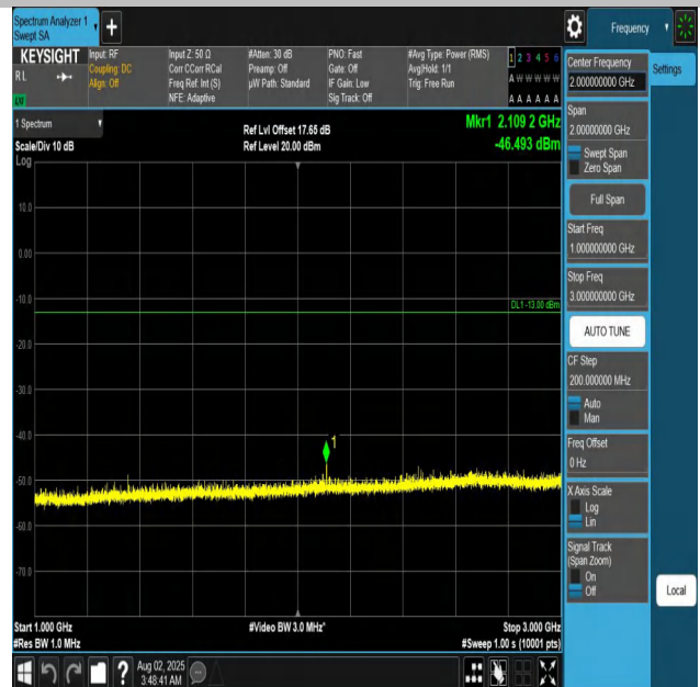
Band12-10MHz-QPSK-23095-1RB#0-1000~3000-PASS
