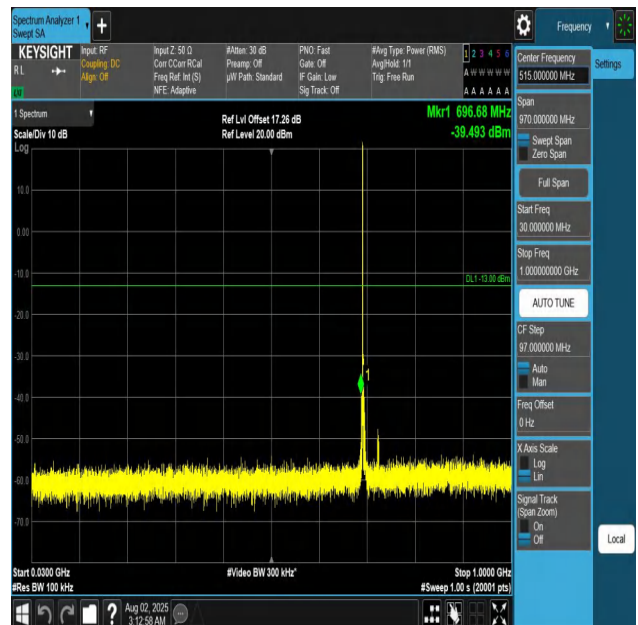
Band12-3MHz-QPSK-23025-1RB#0-30~1000-PASS
