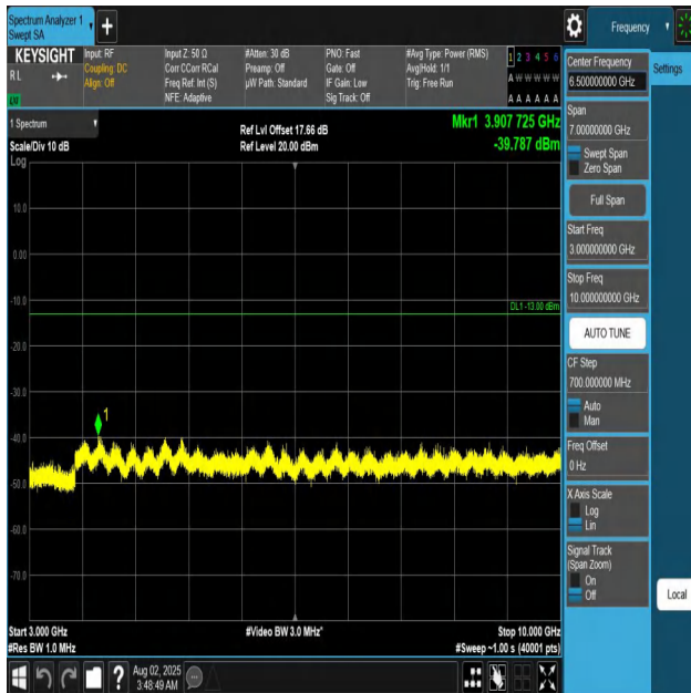
Band12-10MHz-QPSK-23095-1RB#0-3000~10000-PASS
