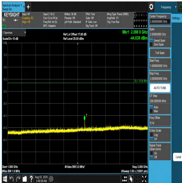
Band12-10MHz-QPSK-23060-1RB#0-1000~3000-PASS
