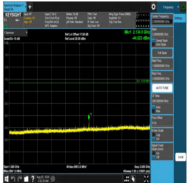
Band12-5MHz-QPSK-23155-1RB#0-1000~3000-PASS
