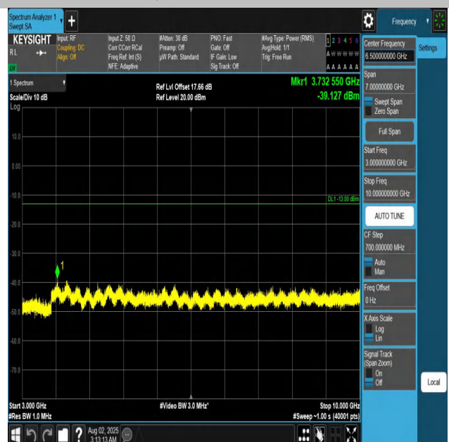
Band12-3MHz-QPSK-23025-1RB#0-3000~10000-PASS
