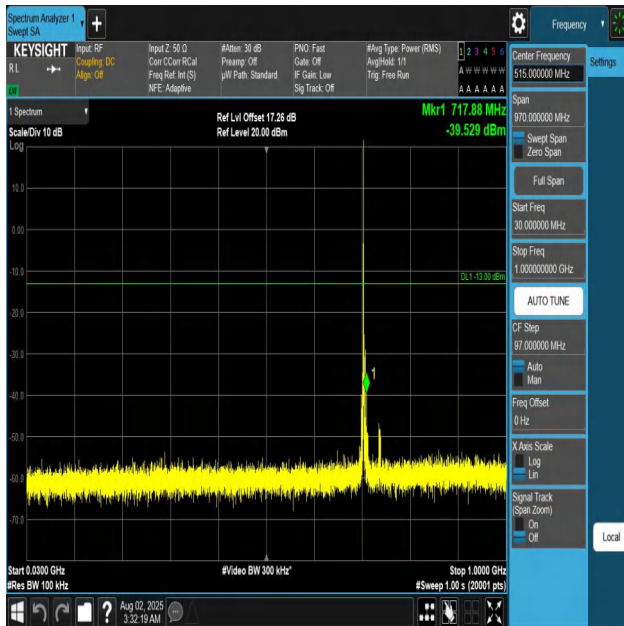
Band12-5MHz-QPSK-23155-1RB#0-30~1000-PASS
