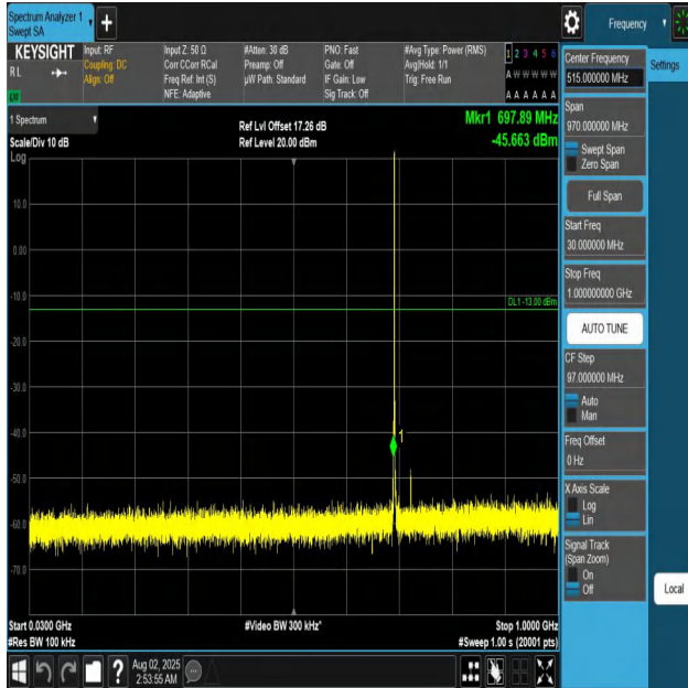
Band12-1.4MHz-QPSK-23017-1RB#0-30~1000-PASS
