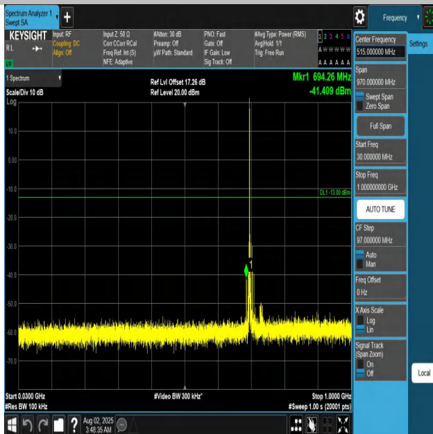
Band12-10MHz-QPSK-23095-1RB#0-30~1000-PASS
