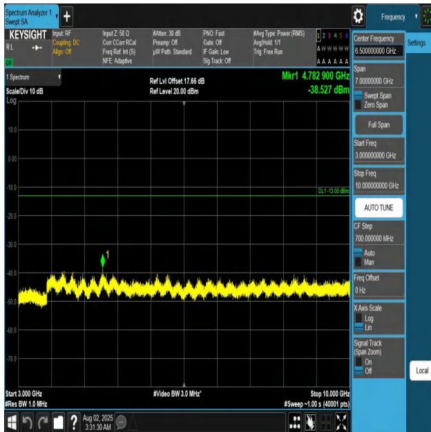
Band12-5MHz-QPSK-23035-1RB#0-3000~10000-PASS
