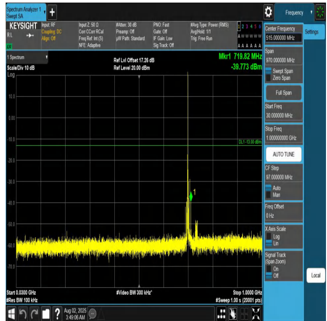
Band12-10MHz-QPSK-23130-1RB#0-30~1000-PASS
