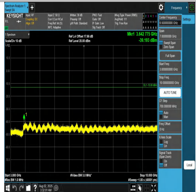
Band12-5MHz-QPSK-23095-1RB#0-3000~10000-PASS
