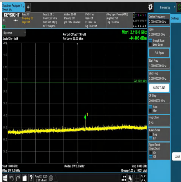
Band12-5MHz-QPSK-23095-1RB#0-1000~3000-PASS
