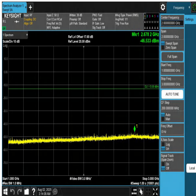
Band12-3MHz-QPSK-23165-1RB#0-1000~3000-PASS
