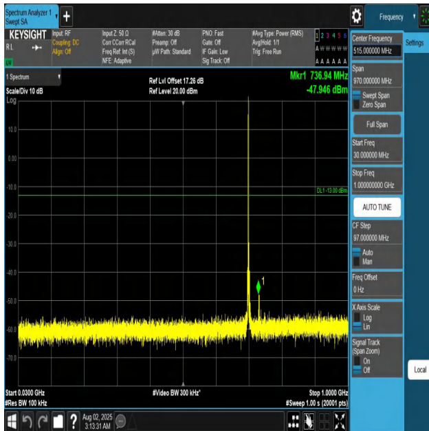
Band12-3MHz-QPSK-23095-1RB#0-30~1000-PASS
