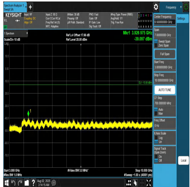
Band12-3MHz-QPSK-23165-1RB#0-3000~10000-PASS
