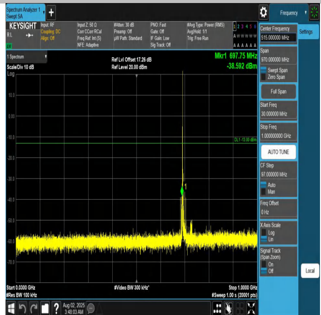
Band12-10MHz-QPSK-23060-1RB#0-30~1000-PASS
