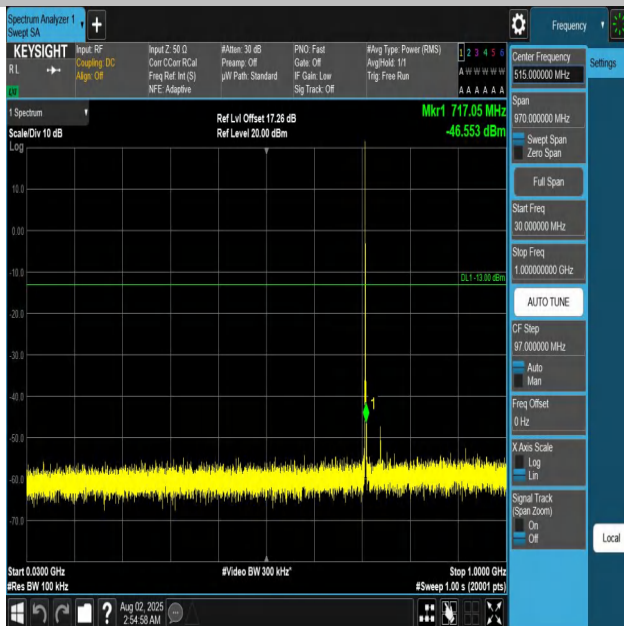
Band12-1.4MHz-QPSK-23173-1RB#0-30~1000-PASS
