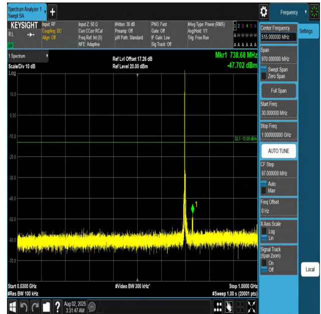
Band12-5MHz-QPSK-23095-1RB#0-30~1000-PASS
