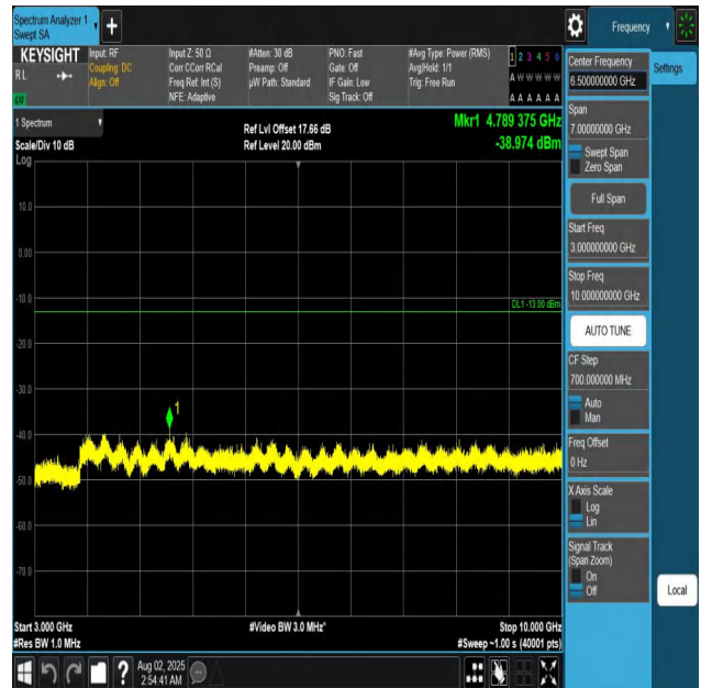
Band12-1.4MHz-QPSK-23095-1RB#0-3000~10000-PASS
