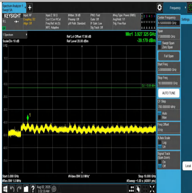
Band12-5MHz-QPSK-23155-1RB#0-3000~10000-PASS
