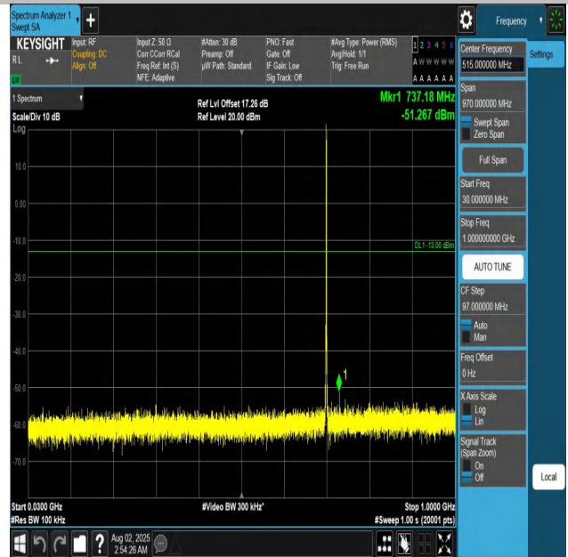
Band12-1.4MHz-QPSK-23095-1RB#0-30~1000-PASS
