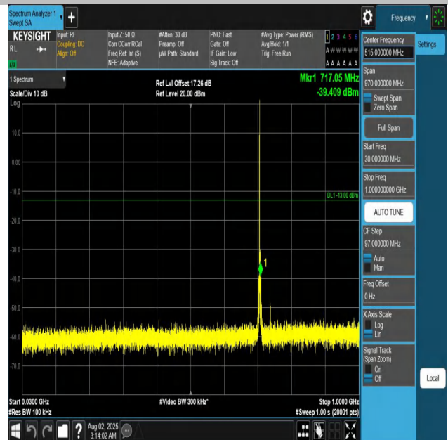
Band12-3MHz-QPSK-23165-1RB#0-30~1000-PASS
