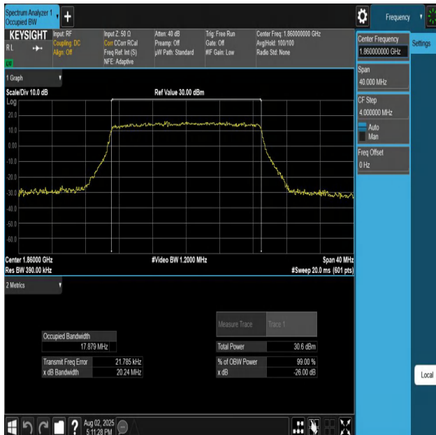
Band25-20MHz-QPSK-26140-100RB#0-PASS
