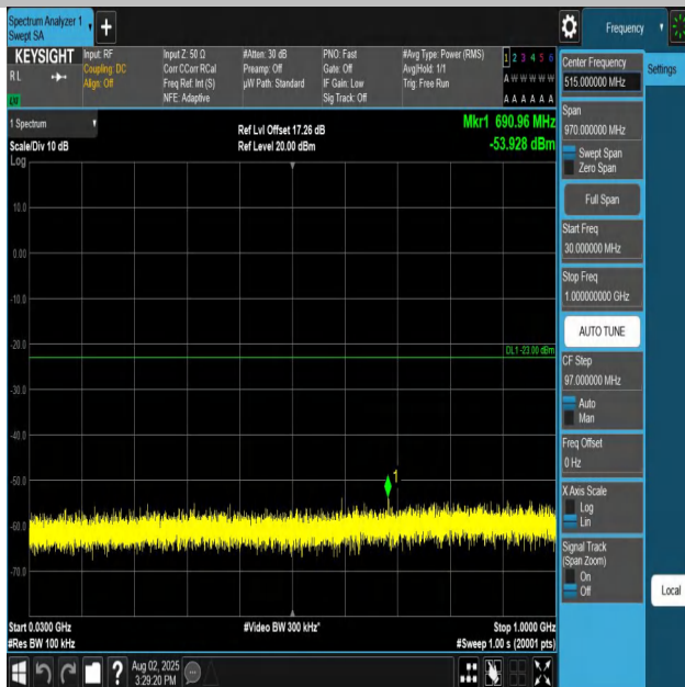
Band25-1.4MHz-QPSK-26683-1RB#0-30~1000-PASS
