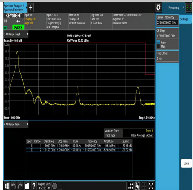
Band25-15MHz-QPSK-26615-1RB#0-PASS
