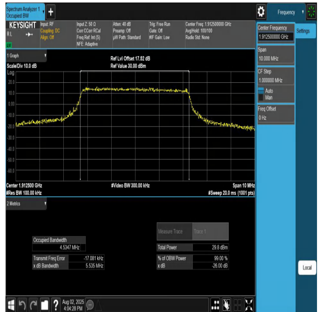
Band25-5MHz-16QAM-26665-25RB#0-PASS
