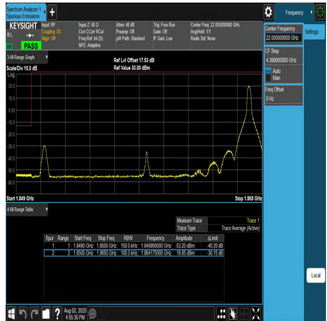
Band25-15MHz-QPSK-26115-1RB#74-PASS
