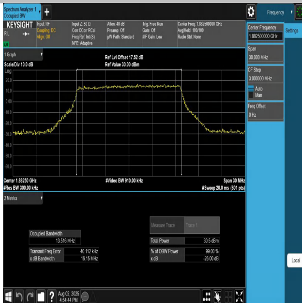
Band25-15MHz-QPSK-26365-75RB#0-PASS
