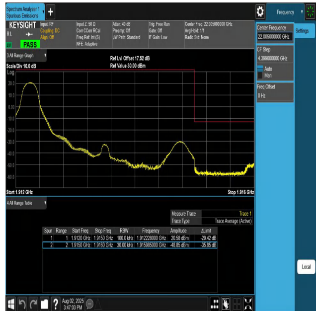
Band25-3MHz-QPSK-26675-1RB#0-PASS
