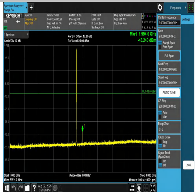
Band25-1.4MHz-QPSK-26683-1RB#0-1000~3000-PASS
