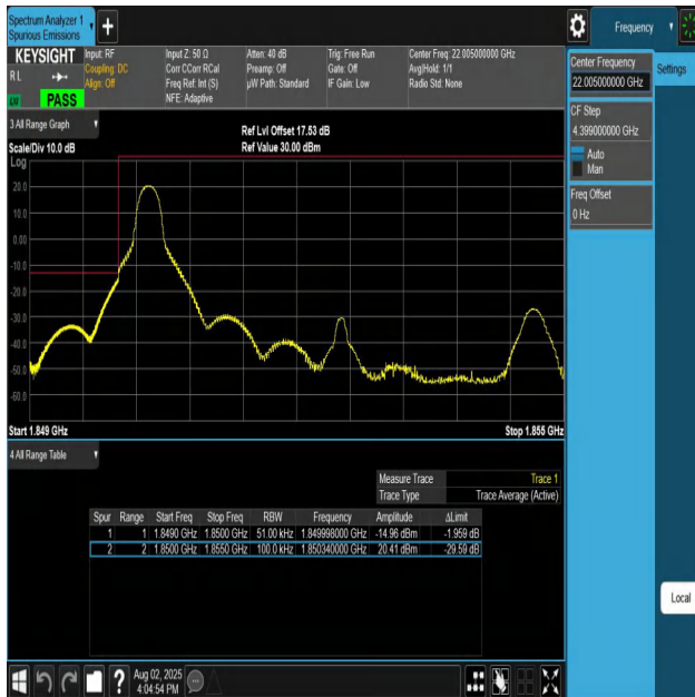
Band25-5MHz-QPSK-26065-1RB#0-PASS
