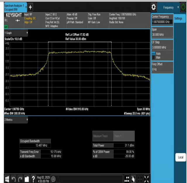
Band25-15MHz-QPSK-26615-75RB#0-PASS
