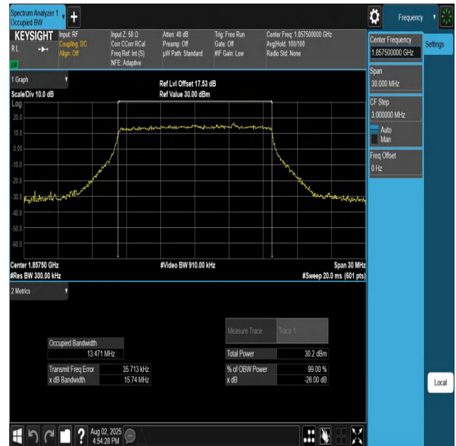
Band25-15MHz-QPSK-26115-75RB#0-PASS
