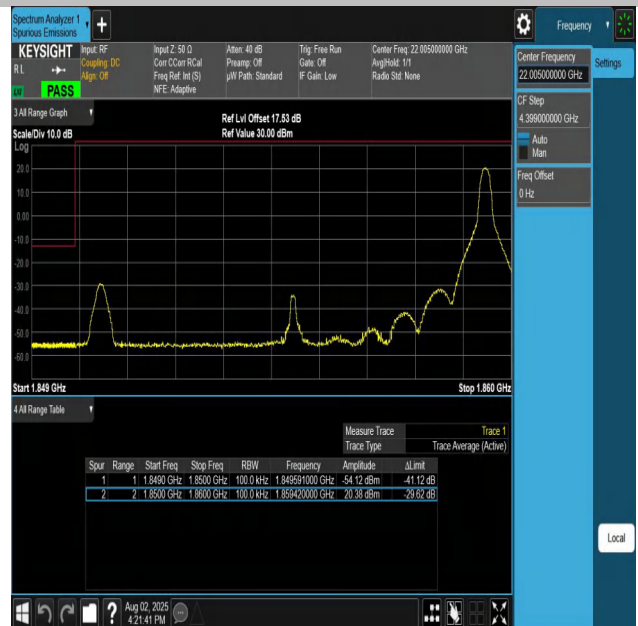
Band25-10MHz-QPSK-26090-1RB#49-PASS
