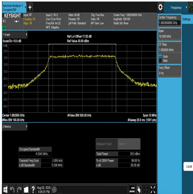
Band25-5MHz-16QAM-26365-25RB#0-PASS
