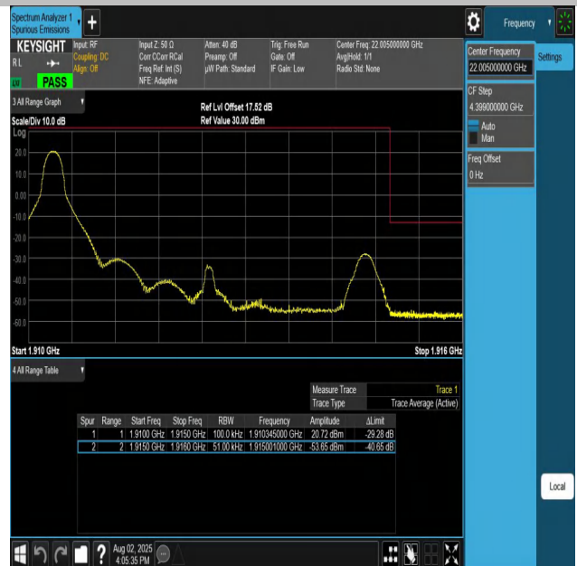
Band25-5MHz-QPSK-26665-1RB#0-PASS
