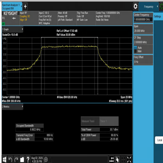
Band25-10MHz-QPSK-26090-50RB#0-PASS
