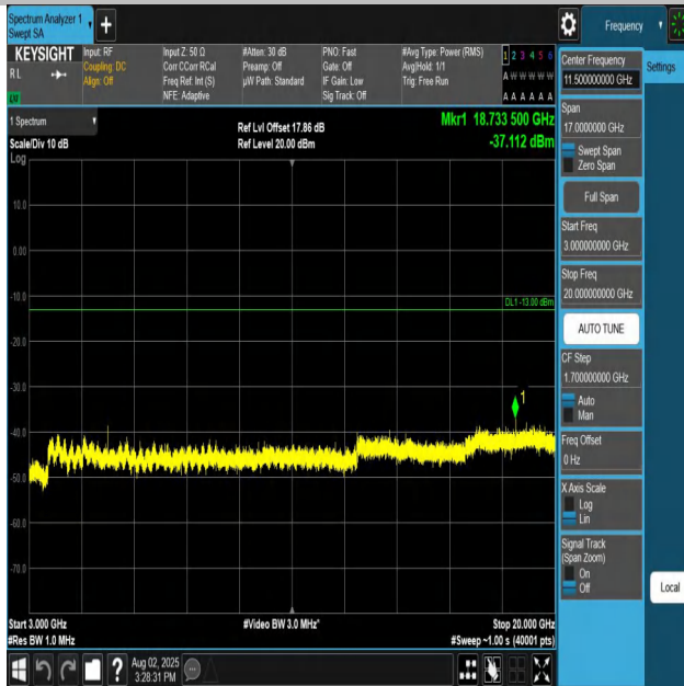
Band25-1.4MHz-QPSK-26047-1RB#0-3000~20000-PASS
