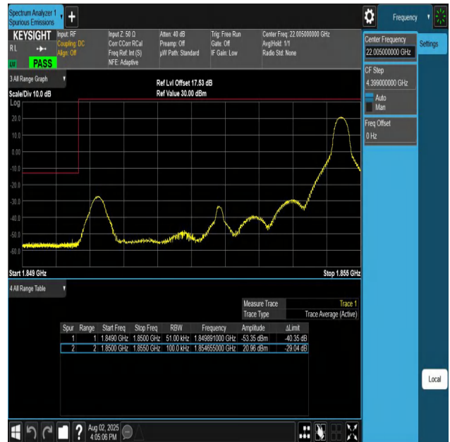
Band25-5MHz-QPSK-26065-1RB#24-PASS
