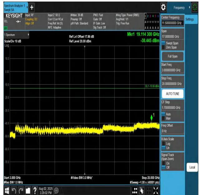
Band25-1.4MHz-QPSK-26365-1RB#0-3000~20000-PASS
