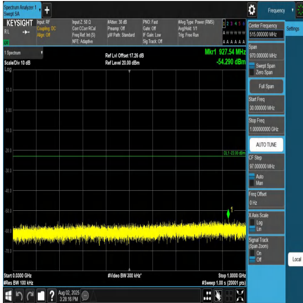
Band25-1.4MHz-QPSK-26047-1RB#0-30~1000-PASS
