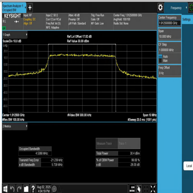
Band25-5MHz-QPSK-26665-25RB#0-PASS
