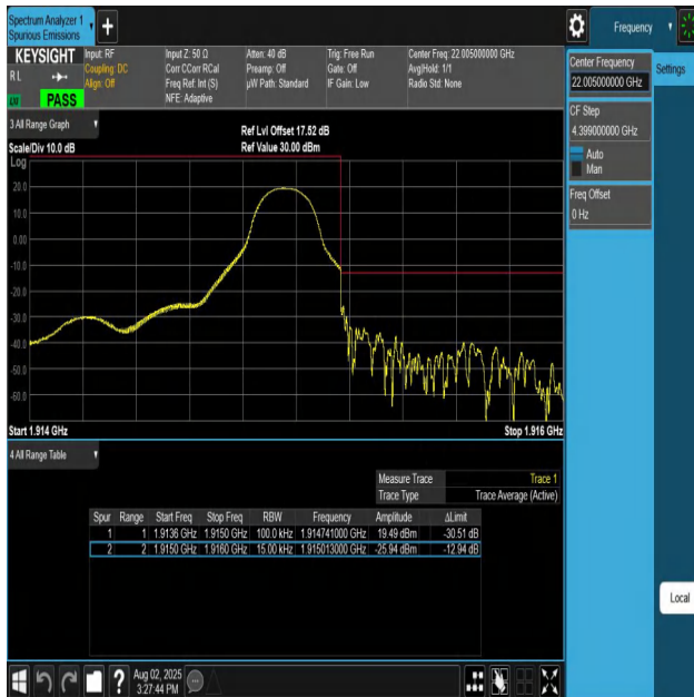
Band25-1.4MHz-QPSK-26683-1RB#5-PASS
