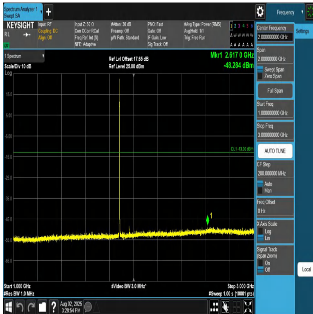
Band25-1.4MHz-QPSK-26365-1RB#0-1000~3000-PASS
