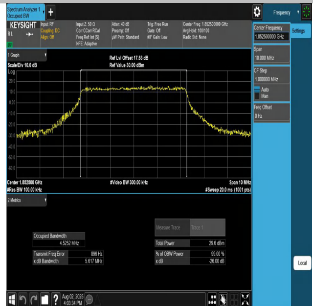
Band25-5MHz-16QAM-26065-25RB#0-PASS
