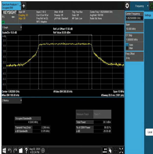
Band25-5MHz-QPSK-26065-25RB#0-PASS
