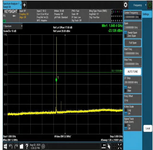
Band25-1.4MHz-QPSK-26047-1RB#0-1000~3000-PASS
