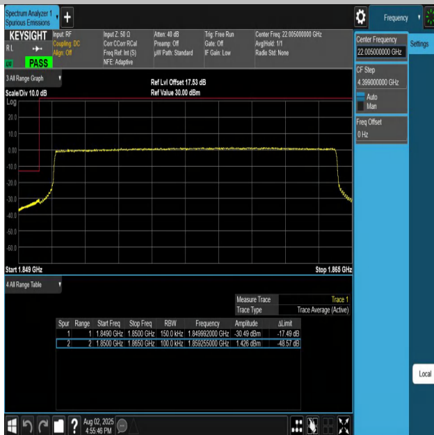
Band25-15MHz-QPSK-26115-75RB#0-PASS
