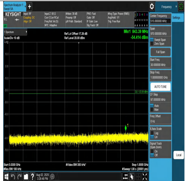
Band25-1.4MHz-QPSK-26365-1RB#0-30~1000-PASS
