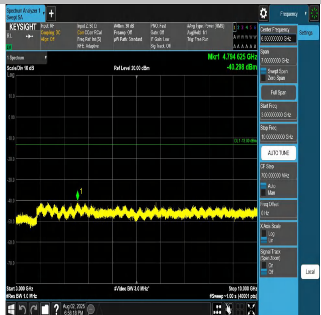
Band26(824-849)-3MHz-QPSK-26805-1RB#0-3000~1000 0-PASS
