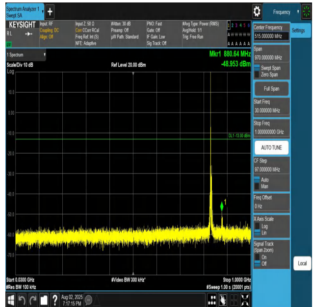
Band26(824-849)-5MHz-QPSK-26915-1RB#0-30~1000-P ASS
