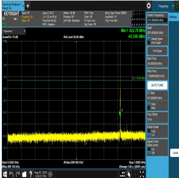
Band26(824-849)-1.4MHz-QPSK-26797-1RB#0-30~1000- PASS
