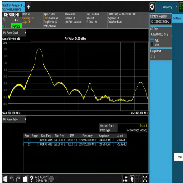
Band26(824-849)-5MHz-QPSK-26815-1RB#0-PASS
