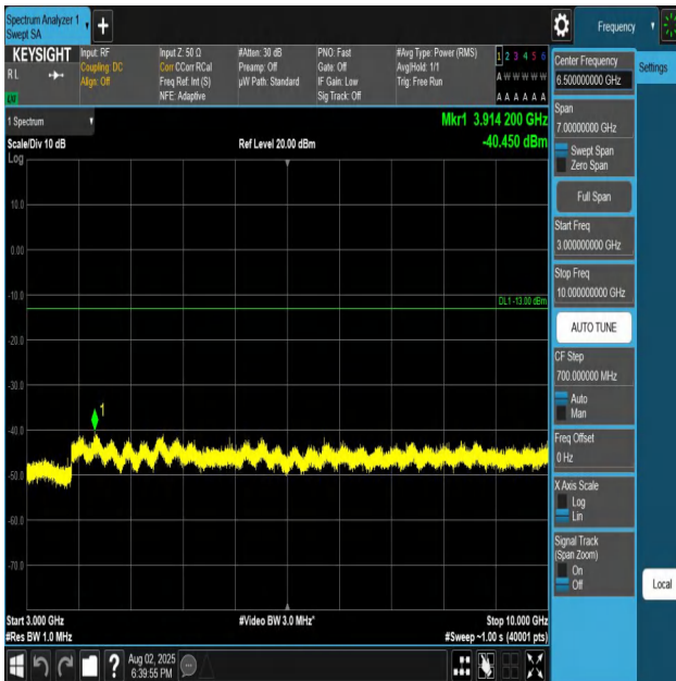
Band26(824-849)-1.4MHz-QPSK-27033-1RB#0-3000~100 00-PASS
