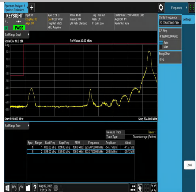
Band26(824-849)-10MHz-QPSK-26840-1RB#49-PASS
