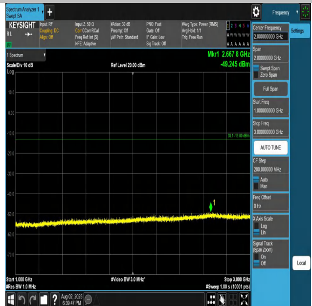
Band26(824-849)-1.4MHz-QPSK-27033-1RB#0-1000~300 0-PASS
