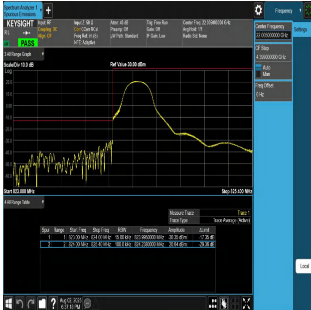
Band26(824-849)-1.4MHz-QPSK-26797-1RB#0-PASS
