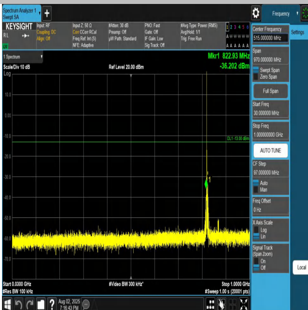
Band26(824-849)-5MHz-QPSK-26815-1RB#0-30~1000-P ASS
