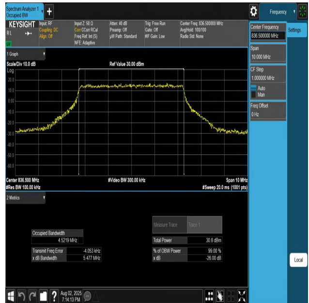
Band26(824-849)-5MHz-QPSK-26915-25RB#0-PASS
