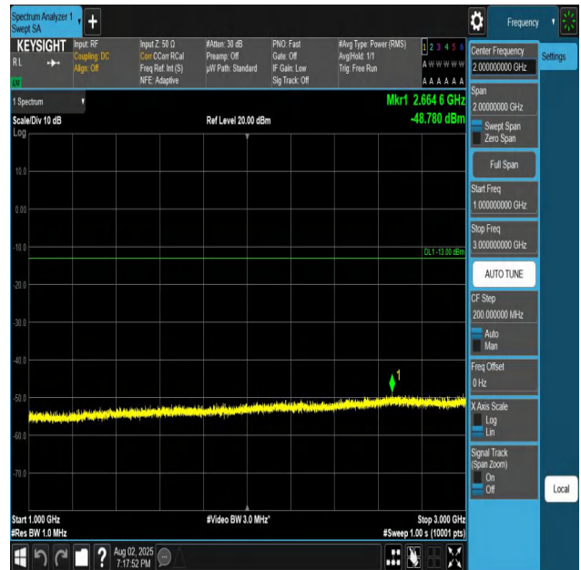
Band26(824-849)-5MHz-QPSK-27015-1RB#0-1000~3000- PASS
