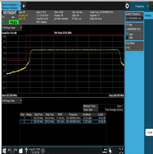
Band26(824-849)-5MHz-QPSK-26815-25RB#0-PASS
