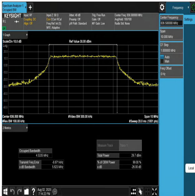
Band26(824-849)-5MHz-16QAM-26915-25RB#0-PASS
