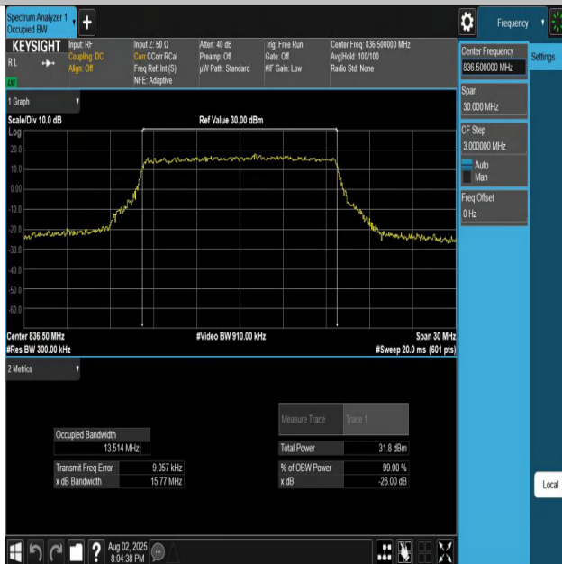
Band26(824-849)-15MHz-QPSK-26915-75RB#0-PASS
