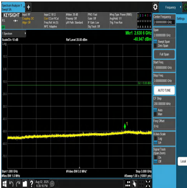
Band26(824-849)-1.4MHz-QPSK-26915-1RB#0-1000~300 0-PASS
