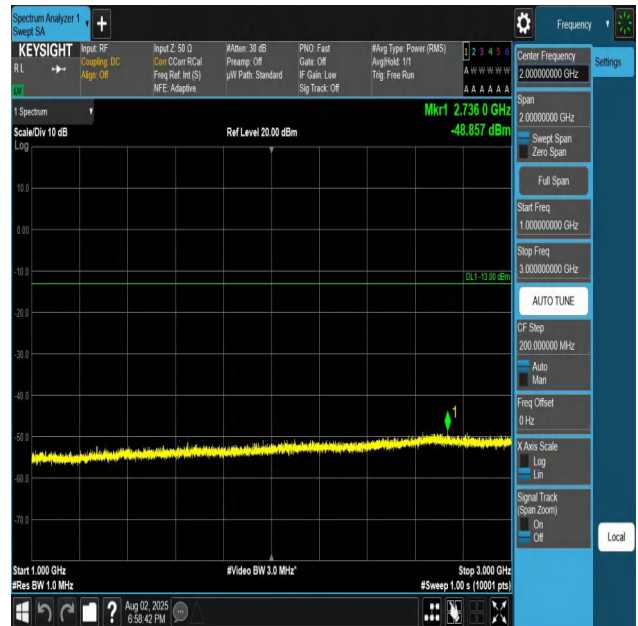
Band26(824-849)-3MHz-QPSK-26915-1RB#0-1000~3000- PASS
