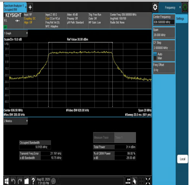
Band26(824-849)-10MHz-QPSK-26915-50RB#0-PASS
