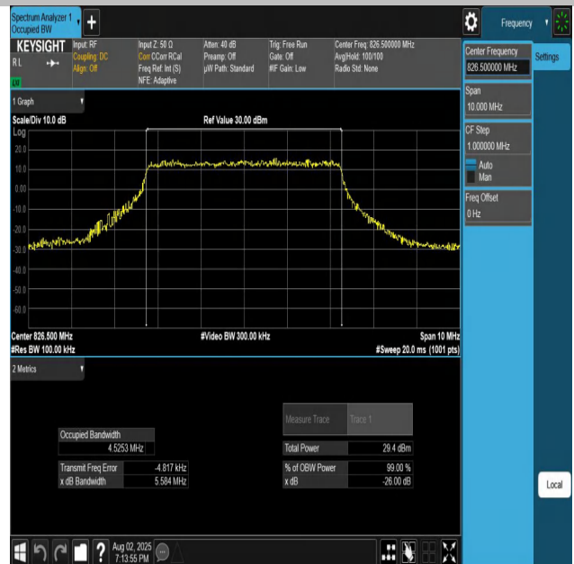
Band26(824-849)-5MHz-16QAM-26815-25RB#0-PASS
