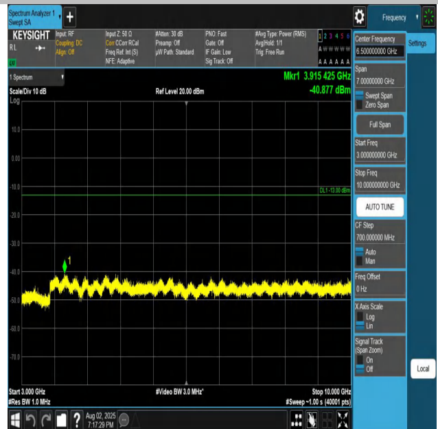
Band26(824-849)-5MHz-QPSK-26915-1RB#0-3000~1000 0-PASS
