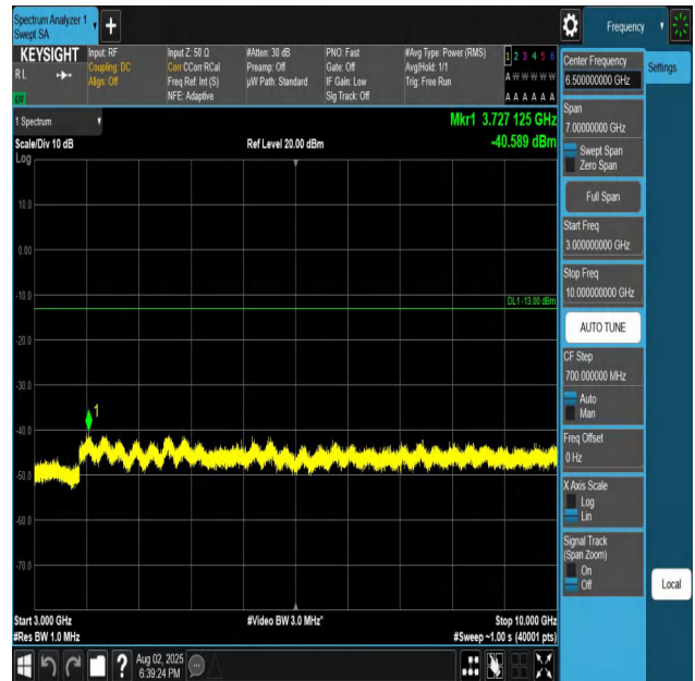
Band26(824-849)-1.4MHz-QPSK-26915-1RB#0-3000~100 00-PASS
