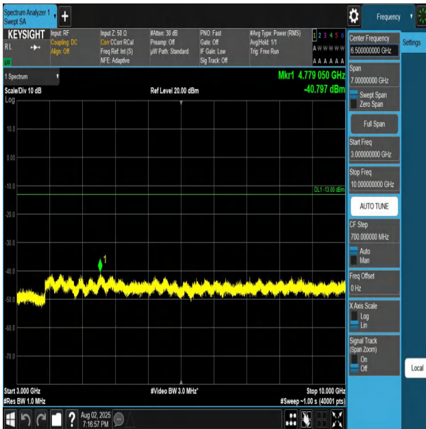
Band26(824-849)-5MHz-QPSK-26815-1RB#0-3000~1000 0-PASS
