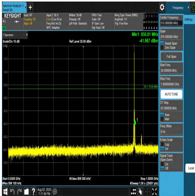
Band26(824-849)-5MHz-QPSK-27015-1RB#0-30~1000-P ASS
