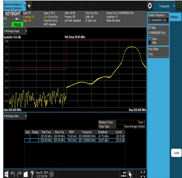
Band26(824-849)-1.4MHz-QPSK-26797-1RB#5-PASS
