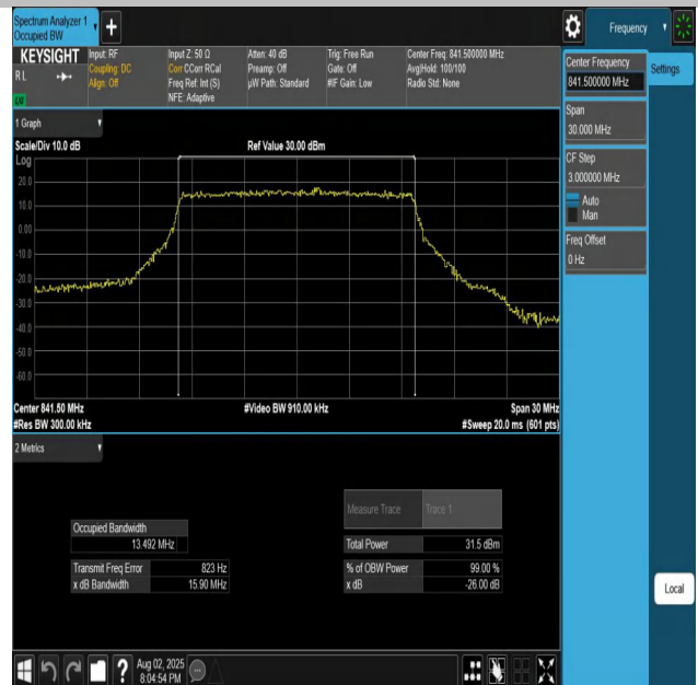
Band26(824-849)-15MHz-QPSK-26965-75RB#0-PASS
