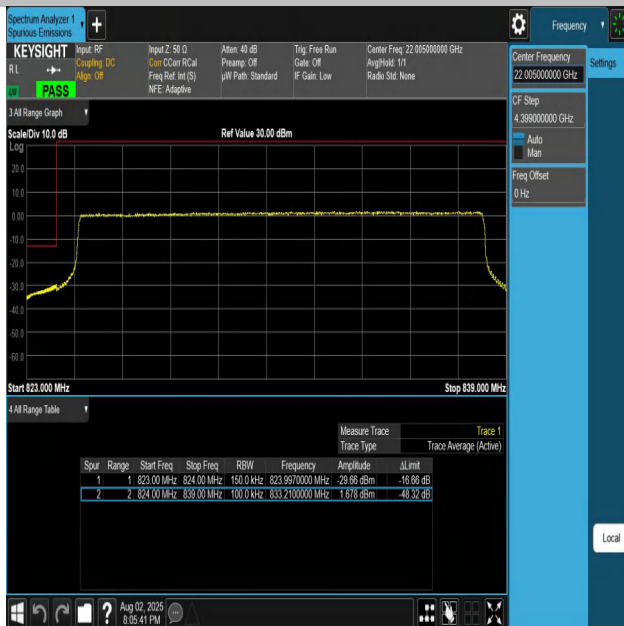
Band26(824-849)-15MHz-QPSK-26865-75RB#0-PASS
