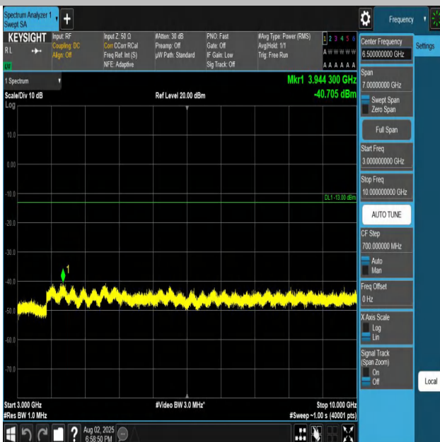
Band26(824-849)-3MHz-QPSK-26915-1RB#0-3000~1000 0-PASS
