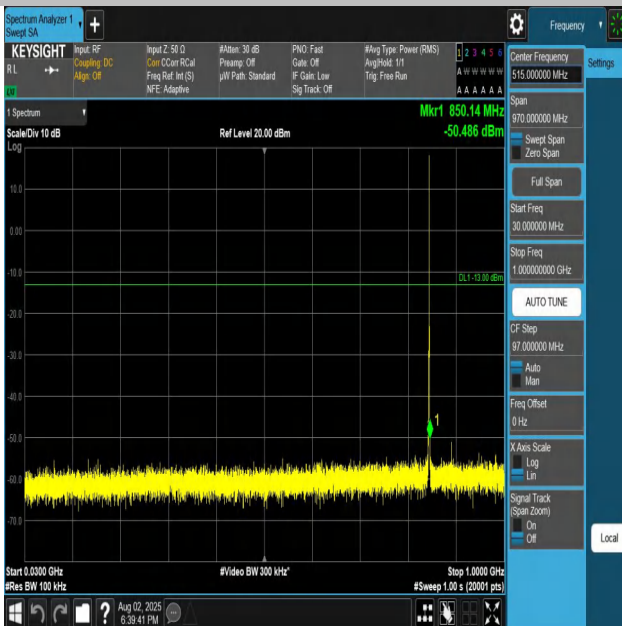
Band26(824-849)-1.4MHz-QPSK-27033-1RB#0-30~1000- PASS
