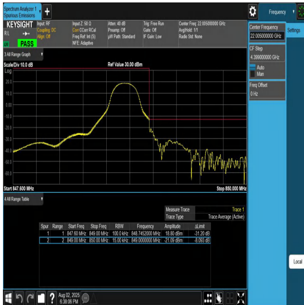
Band26(824-849)-1.4MHz-QPSK-27033-1RB#5-PASS
