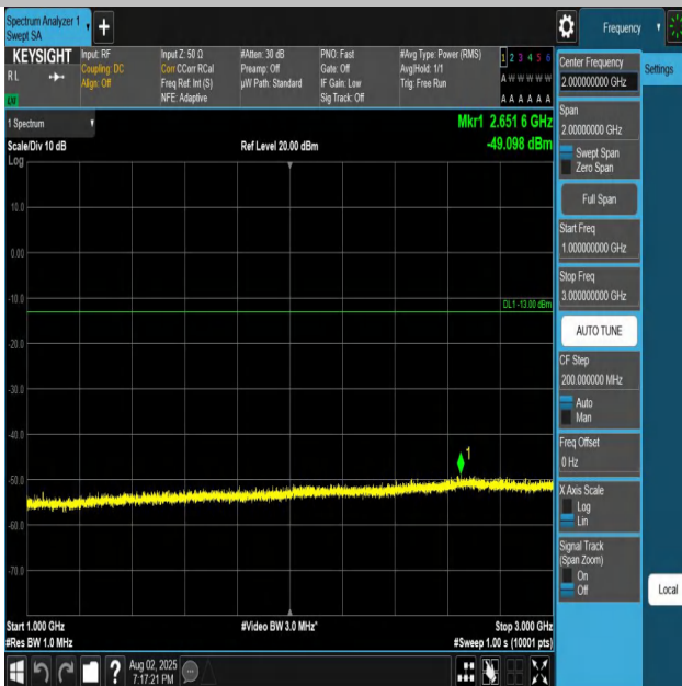
Band26(824-849)-5MHz-QPSK-26915-1RB#0-1000~3000- PASS
