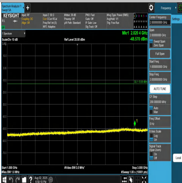
Band26(824-849)-3MHz-QPSK-26805-1RB#0-1000~3000- PASS
