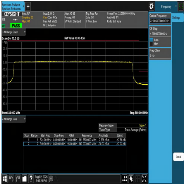
Band26(824-849)-15MHz-QPSK-26965-75RB#0-PASS
