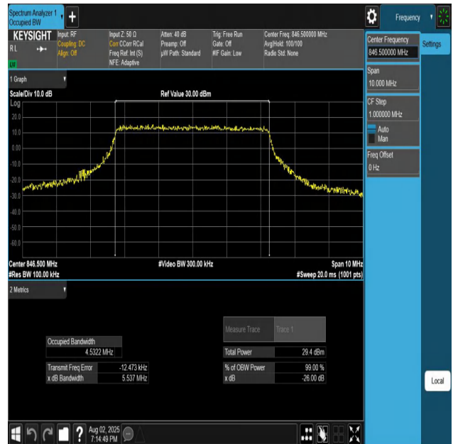
Band26(824-849)-5MHz-16QAM-27015-25RB#0-PASS
