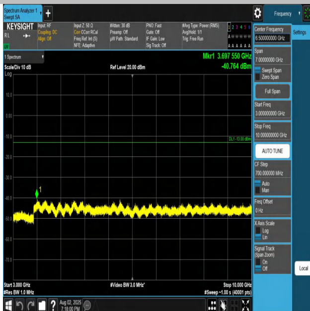
Band26(824-849)-5MHz-QPSK-27015-1RB#0-3000~1000 0-PASS
