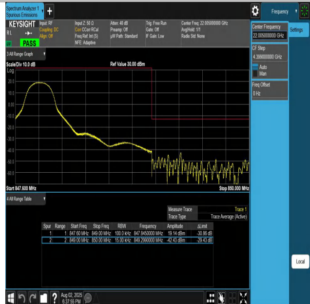
Band26(824-849)-1.4MHz-QPSK-27033-1RB#0-PASS
