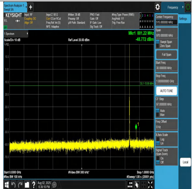
Band26(824-849)-1.4MHz-QPSK-26915-1RB#0-30~1000- PASS
