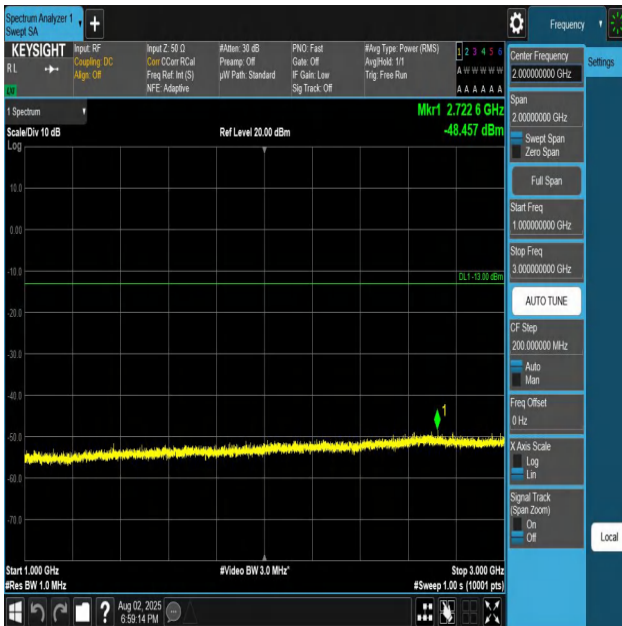
Band26(824-849)-3MHz-QPSK-27025-1RB#0-1000~3000- PASS
