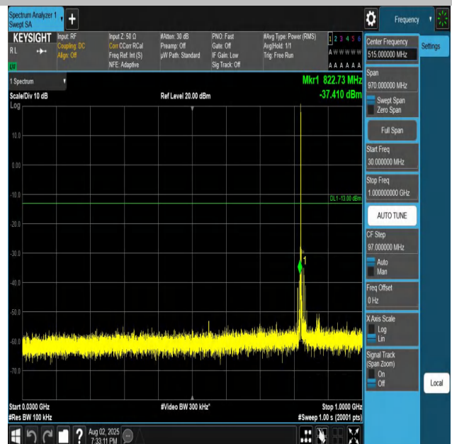
Band26(824-849)-10MHz-QPSK-26840-1RB#0-30~1000-P ASS
