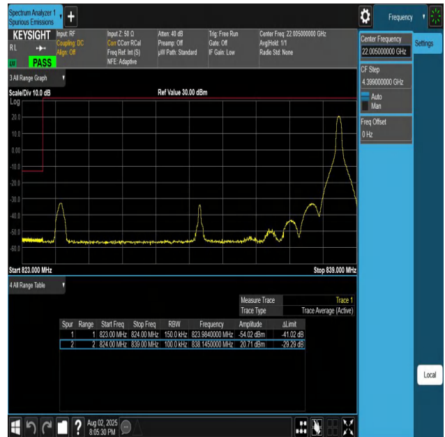
Band26(824-849)-15MHz-QPSK-26865-1RB#74-PASS
