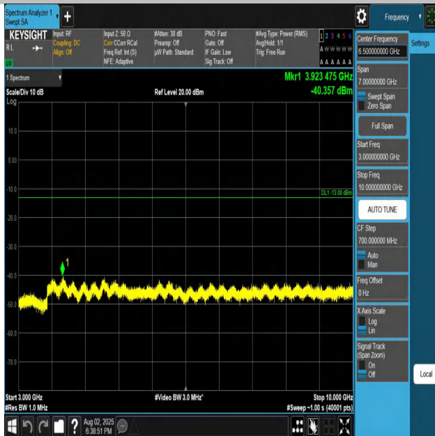
Band26(824-849)-1.4MHz-QPSK-26797-1RB#0-3000~100 00-PASS
