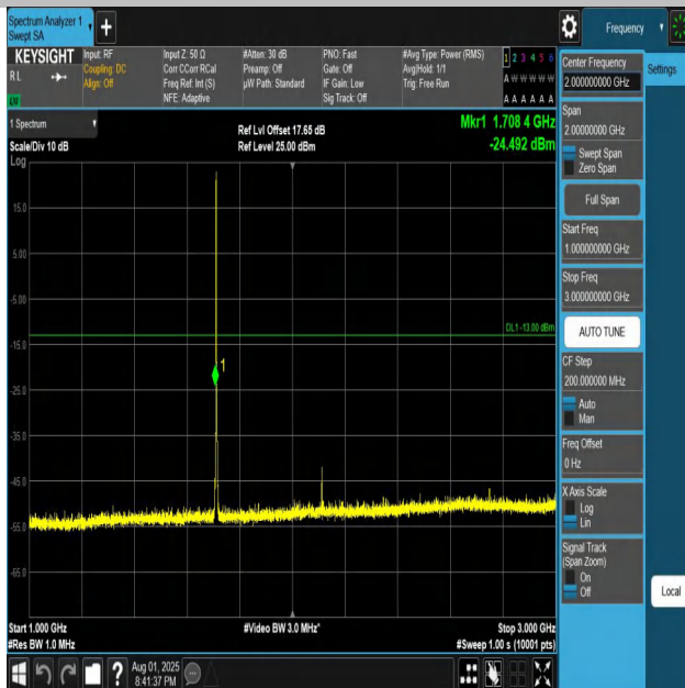
Band4-3MHz-QPSK-19965-1RB#0-1000~3000-PASS
