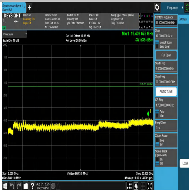
Band4-3MHz-QPSK-20175-1RB#0-3000~20000-PASS
