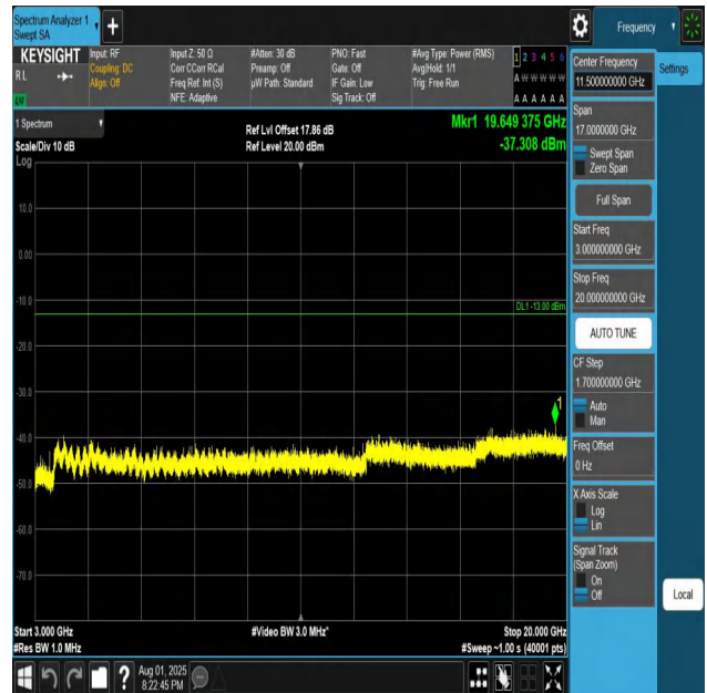
Band4-1.4MHz-QPSK-20175-1RB#0-3000~20000-PASS
