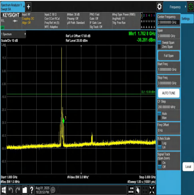
Band4-20MHz-QPSK-20300-1RB#0-1000~3000-PASS
