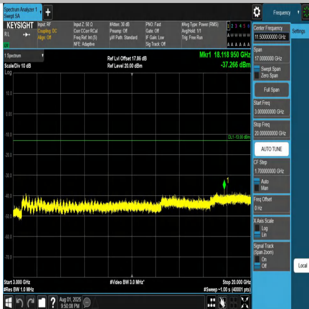
Band4-15MHz-QPSK-20025-1RB#0-3000~20000-PASS
