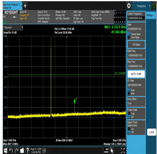
Band4-3MHz-QPSK-20175-1RB#0-1000~3000-PASS
