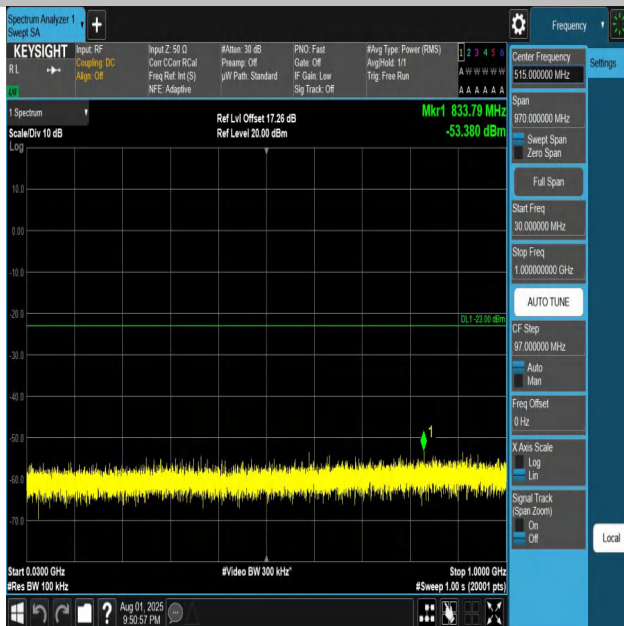
Band4-15MHz-QPSK-20325-1RB#0-30~1000-PASS
