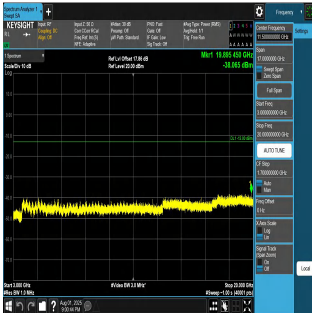
Band4-5MHz-QPSK-19975-1RB#0-3000~20000-PASS
