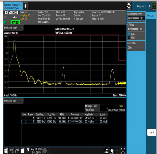
Band4-15MHz-QPSK-20325-1RB#0-PASS
