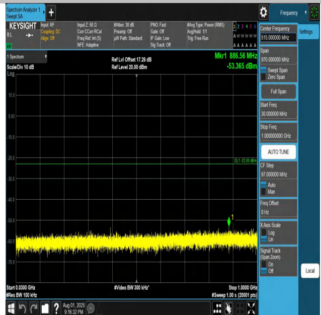
Band4- 10MHz-QPSK-20000-1RB#0-30~1000-PASS
