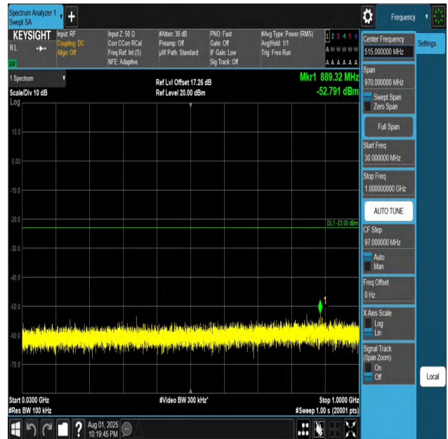
Band4-20MHz-QPSK-20050-1RB#0-30~1000-PASS
