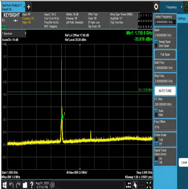
Band4-10MHz-QPSK-20350-1RB#0-1000~3000-PASS
