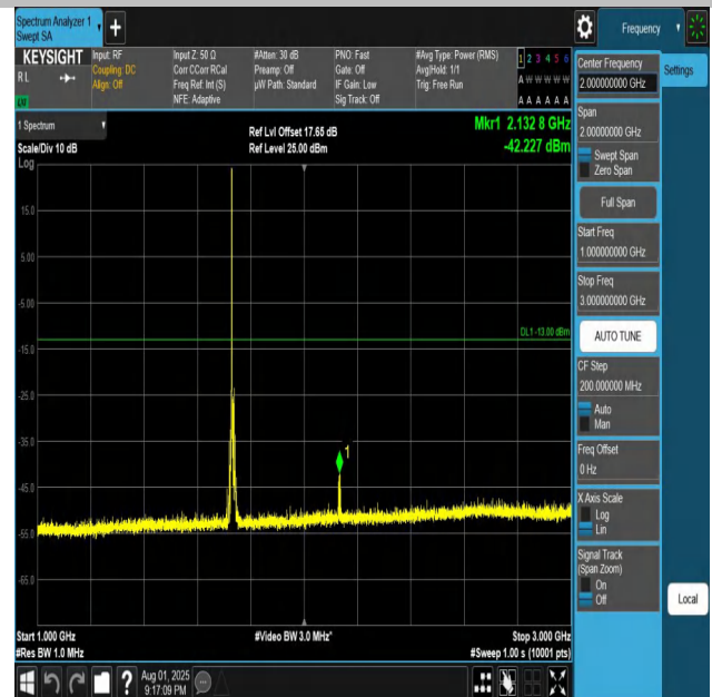
Band4-10MHz-QPSK-20175-1RB#0-1000~3000-PASS
