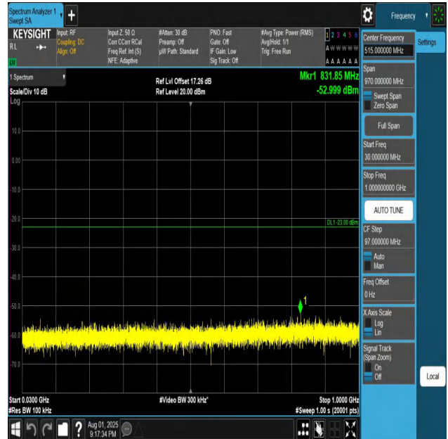
Band4-10MHz-QPSK-20350-1RB#0-30~1000-PASS
