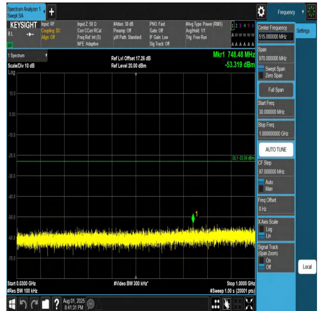
Band4-3MHz-QPSK-19965-1RB#0-30~1000-PASS
