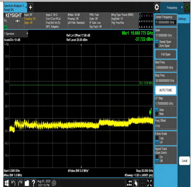
Band4-5MHz-QPSK-20175-1RB#0-3000~20000-PASS
