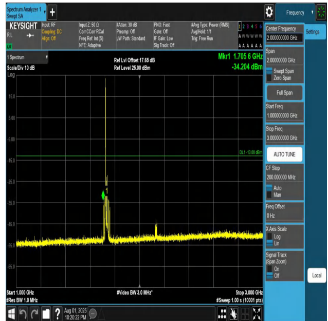
Band4-20MHz-QPSK-20175-1RB#0-1000~3000-PASS
