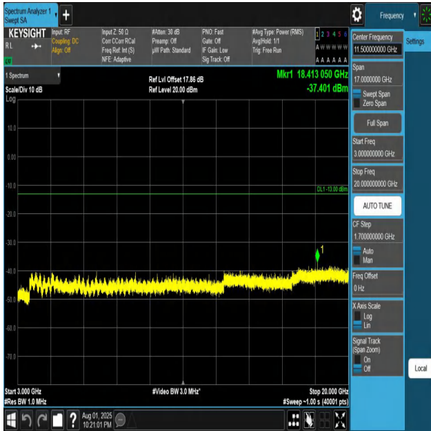
Band4-20MHz-QPSK-20300-1RB#0-3000~20000-PASS
