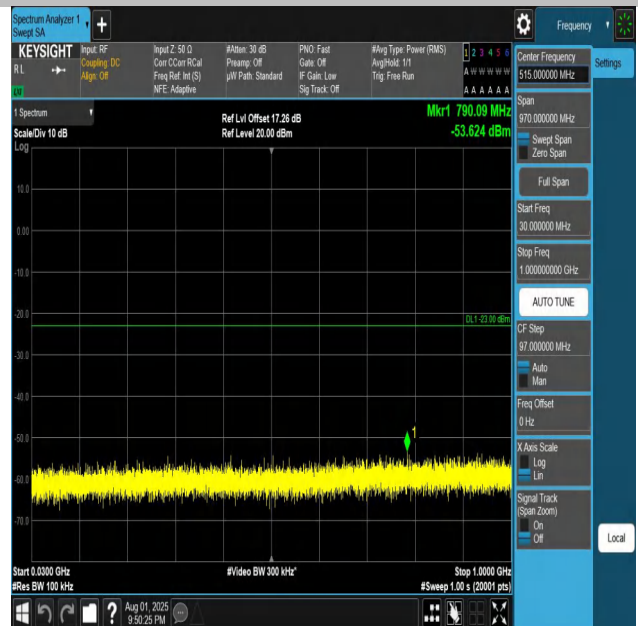
Band4-15MHz-QPSK-20175-1RB#0-30~1000-PASS
