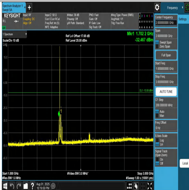
Band4-20MHz-QPSK-20050-1RB#0-1000~3000-PASS
