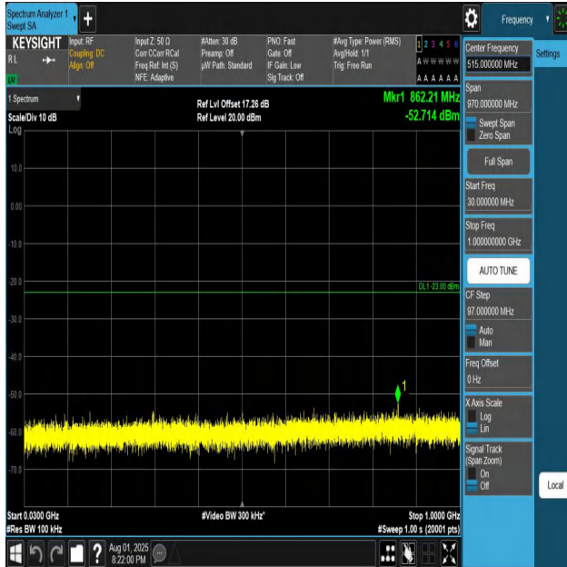
Band4-1.4MHz-QPSK-19957-1RB#0-30~1000-PASS
