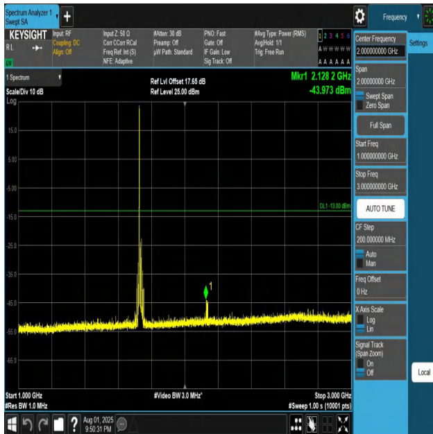
Band4-15MHz-QPSK-20175-1RB#0-1000~3000-PASS
