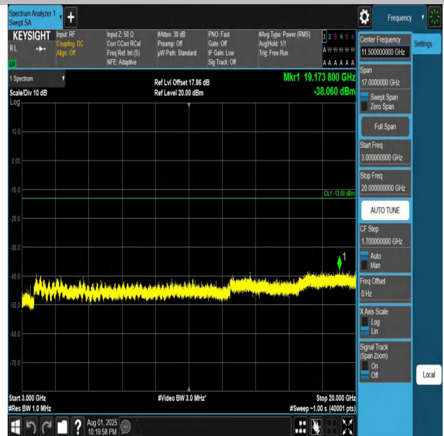
Band4-20MHz-QPSK-20050-1RB#0-3000~20000-PASS
