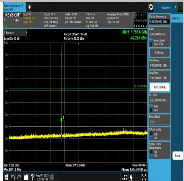
Band4-1.4MHz-QPSK-20393-1RB#0-1000~3000-PASS
