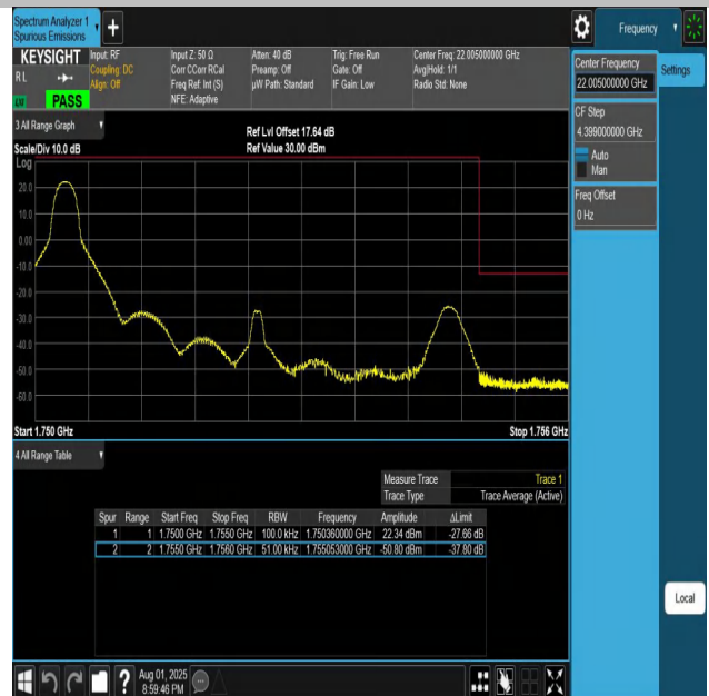
Band4-5MHz-QPSK-20375-1RB#0-PASS
