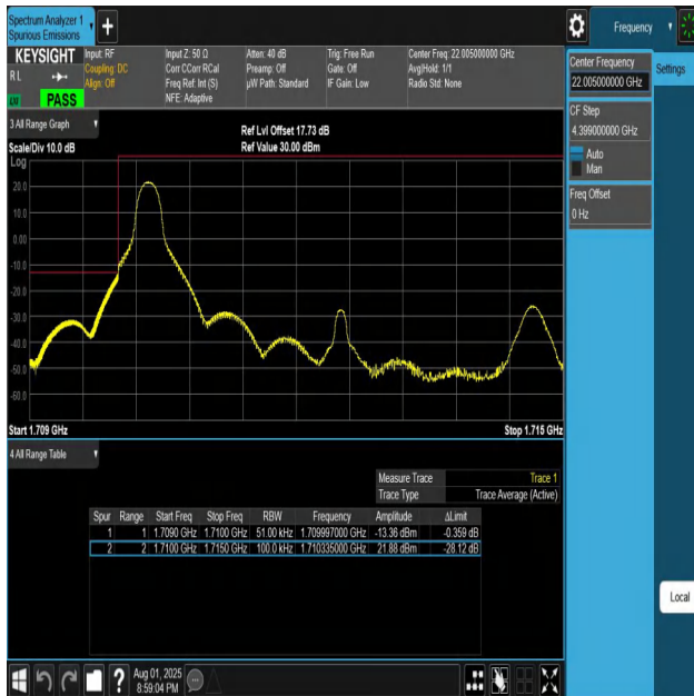
Band4-5MHz-QPSK-19975-1RB#0-PASS
