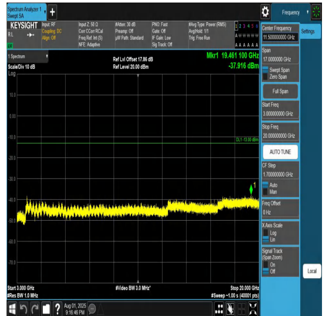
Band4-10MHz-QPSK-20000-1RB#0-3000~20000-PASS
