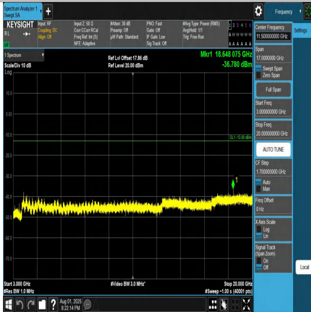
Band4-1.4MHz-QPSK-19957-1RB#0-3000~20000-PASS
