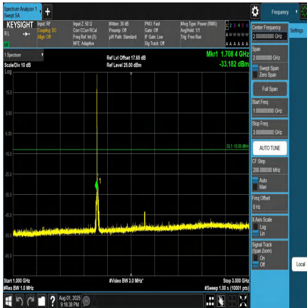
Band4-10MHz-QPSK-20000-1RB#0-1000~3000-PASS
