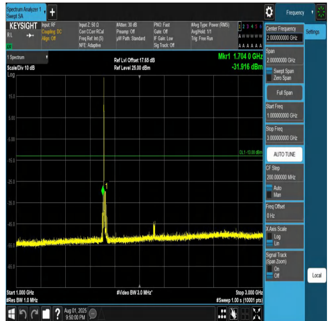
Band4-15MHz-QPSK-20025-1RB#0-1000~3000-PASS
