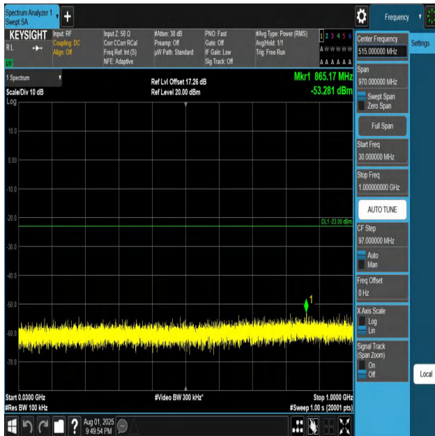
Band4-15MHz-QPSK-20025-1RB#0-30~1000-PASS
