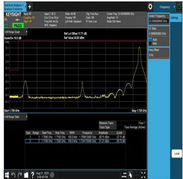
Band4-15MHz-QPSK-20025-1RB#74-PASS
