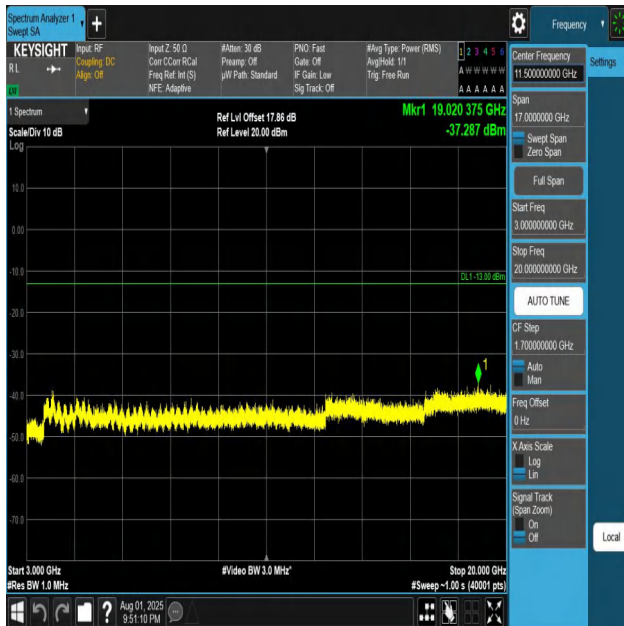
Band4-15MHz-QPSK-20325-1RB#0-3000~20000-PASS
