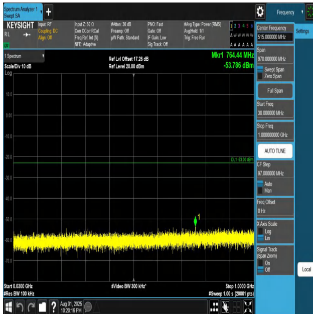
Band4-20MHz-QPSK-20175-1RB#0-30~1000-PASS
