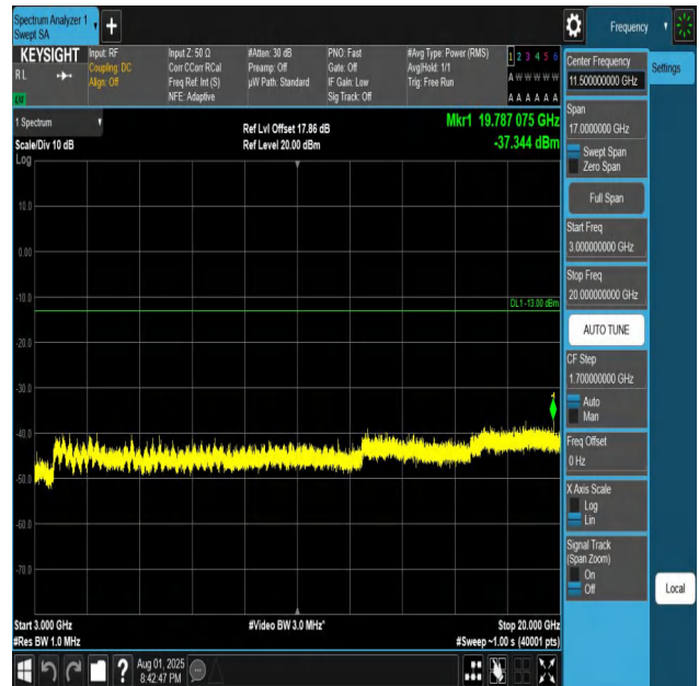
Band4-3MHz-QPSK-20385-1RB#0-3000~20000-PASS
