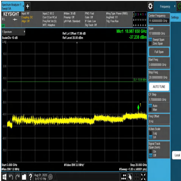
Band4-10MHz-QPSK-20175-1RB#0-3000~20000-PASS
