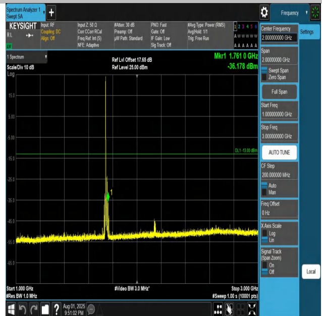
Band4-15MHz-QPSK-20325-1RB#0-1000~3000-PASS
