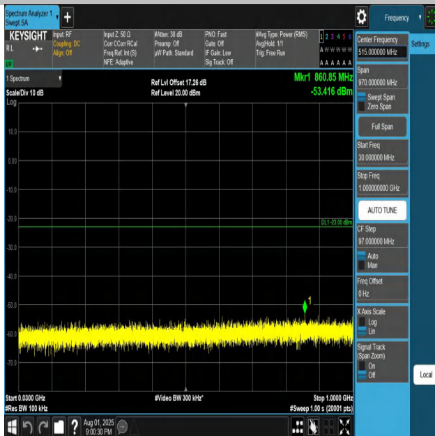
Band4-5MHz-QPSK-19975-1RB#0-30~1000-PASS
