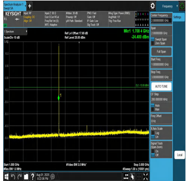
Band4-1.4MHz-QPSK-19957-1RB#0-1000~3000-PASS
