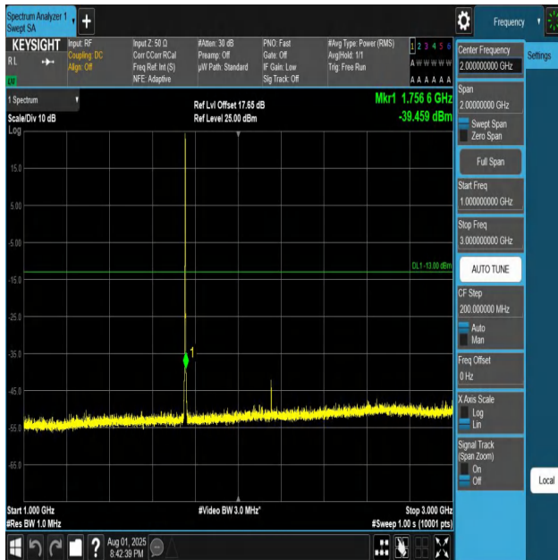
Band4-3MHz-QPSK-20385-1RB#0-1000~3000-PASS
