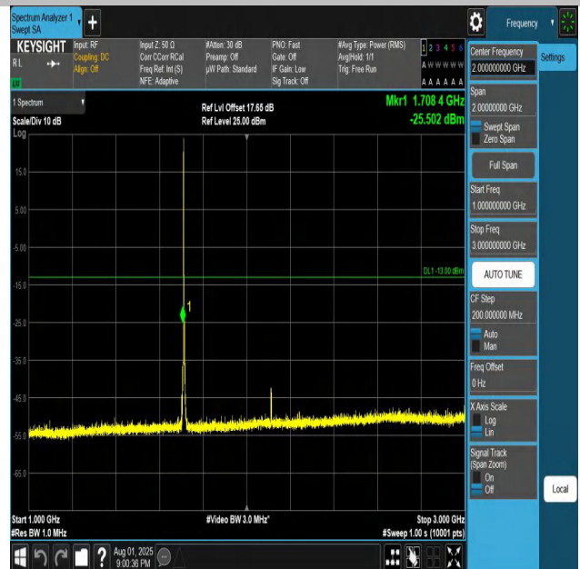
Band4-5MHz-QPSK-19975-1RB#0-1000~3000-PASS
