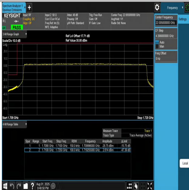
Band4-15MHz-QPSK-20025-75RB#0-PASS
