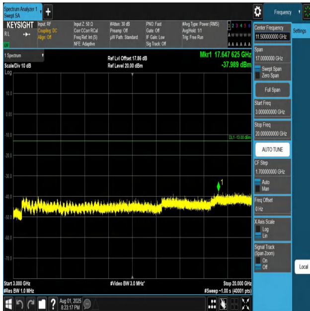
Band4-1.4MHz-QPSK-20393-1RB#0-3000~20000-PASS
