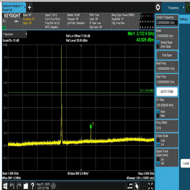
Band4-5MHz-QPSK-20175-1RB#0-1000~3000-PASS
