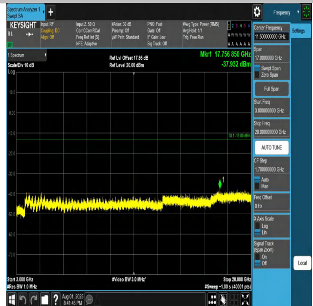
Band4-3MHz-QPSK-19965-1RB#0-3000~20000-PASS
