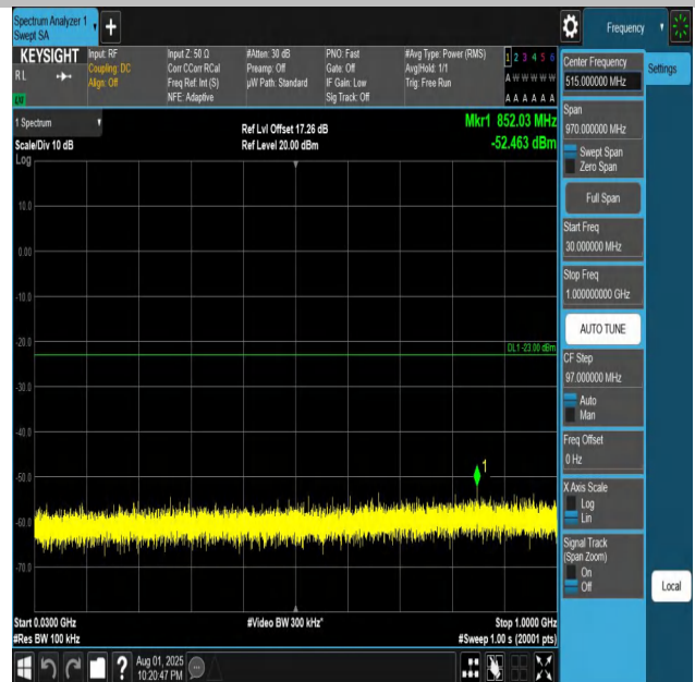
Band4-20MHz-QPSK-20300-1RB#0-30~1000-PASS
