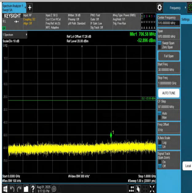
Band4-10MHz-QPSK-20175-1RB#0-30~1000-PASS
