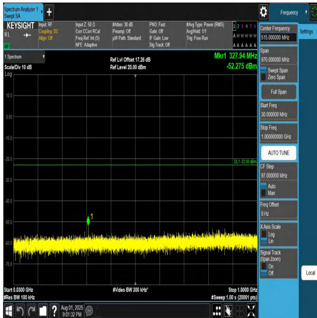
Band4-5MHz-QPSK-20375-1RB#0-30~1000-PASS
