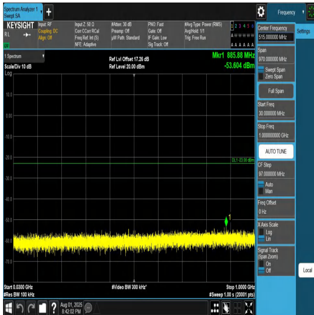
Band4-3MHz-QPSK-20175-1RB#0-30~1000-PASS
