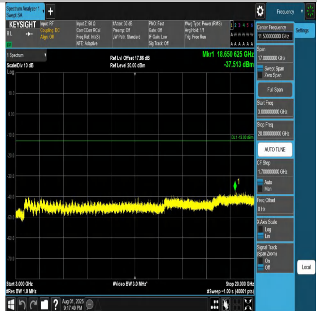
Band4-10MHz-QPSK-20350-1RB#0-3000~20000-PASS
