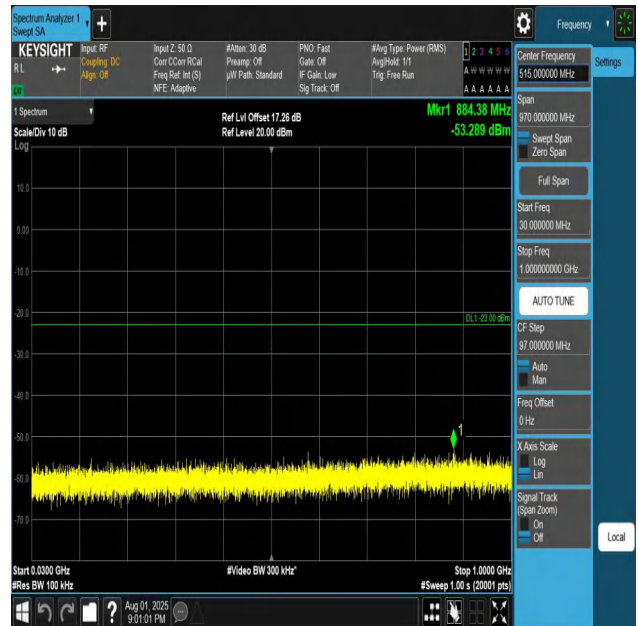
Band4-5MHz-QPSK-20175-1RB#0-30~1000-PASS
