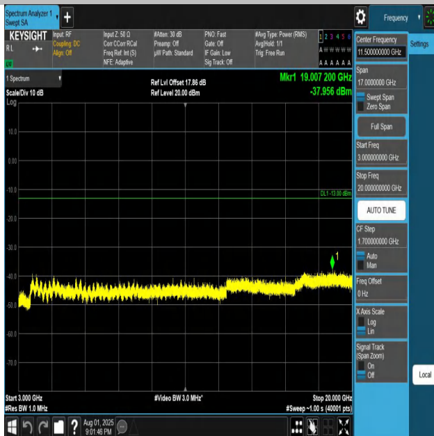
Band4-5MHz-QPSK-20375-1RB#0-3000~20000-PASS
