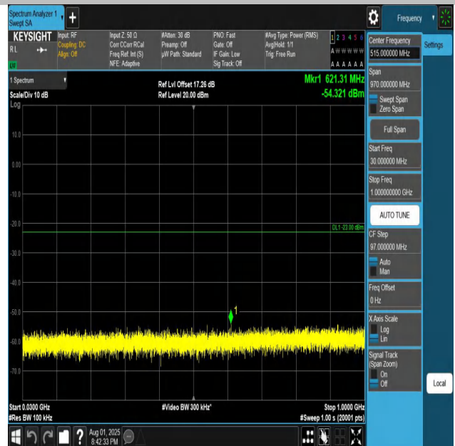
Band4-3MHz-QPSK-20385-1RB#0-30~1000-PASS
