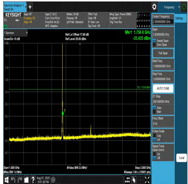
Band4-5MHz-QPSK-20375-1RB#0-1000~3000-PASS
