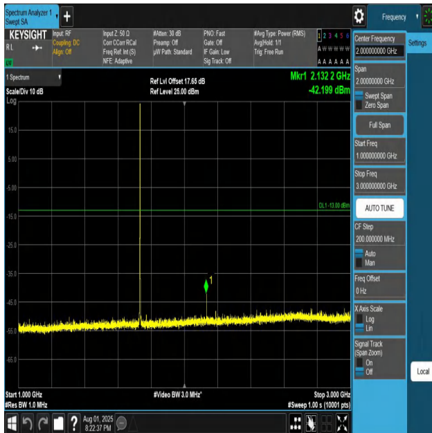
Band4-1.4MHz-QPSK-20175-1RB#0-1000~3000-PASS
