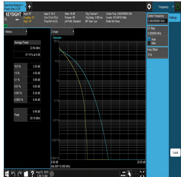
Band41-15MHz-QPSK-41515-75RB#0-PASS
