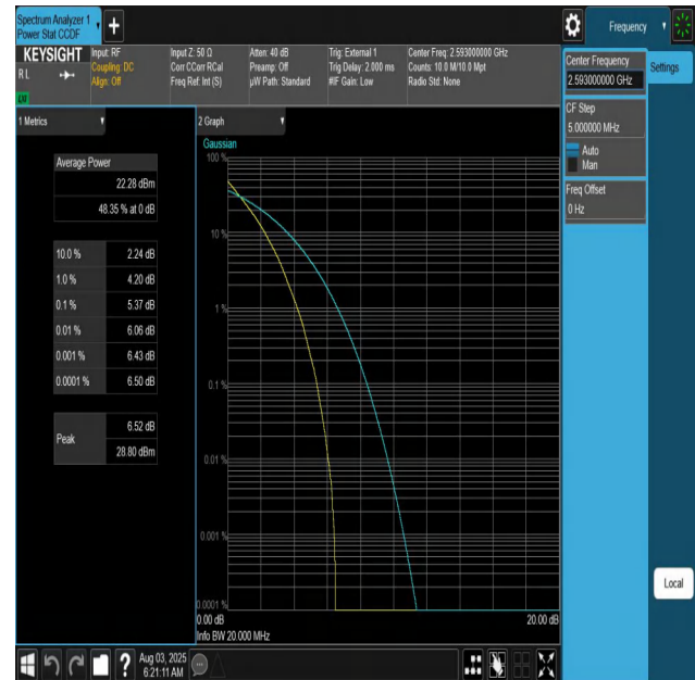
Band41-20MHz-QPSK-40620-100RB#0-PASS
