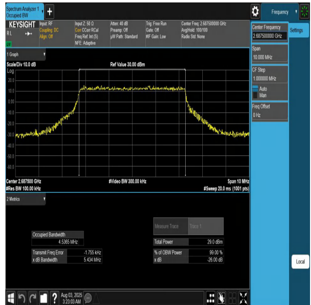
Band41-5MHz-16QAM-41565-25RB#0-PASS
