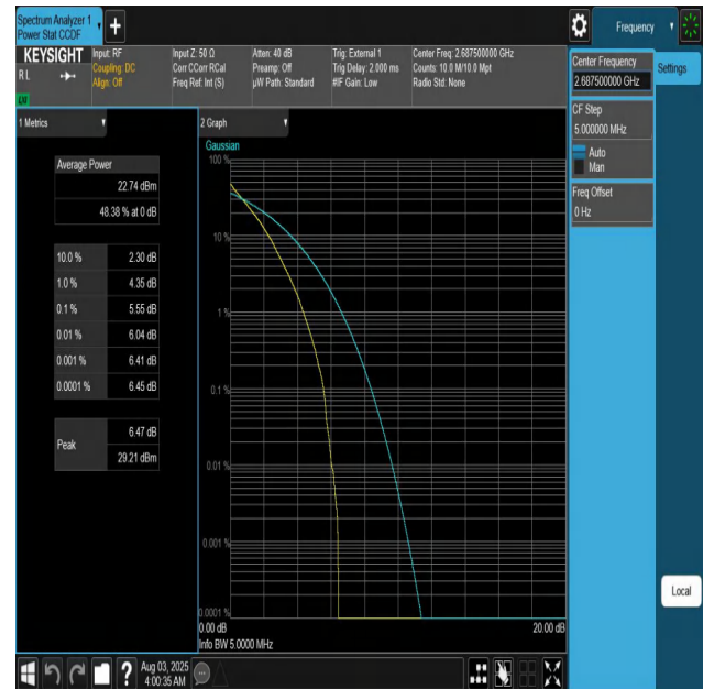
Band41-5MHz-QPSK-41565-25RB#0-PASS
