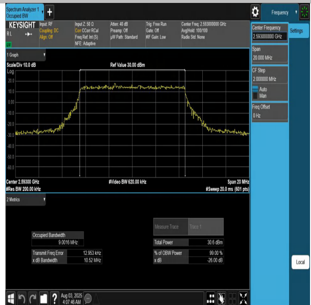
Band41-10MHz-QPSK-40620-50RB#0-PASS
