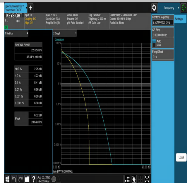
Band41-10MHz-QPSK-39700-50RB#0-PASS
