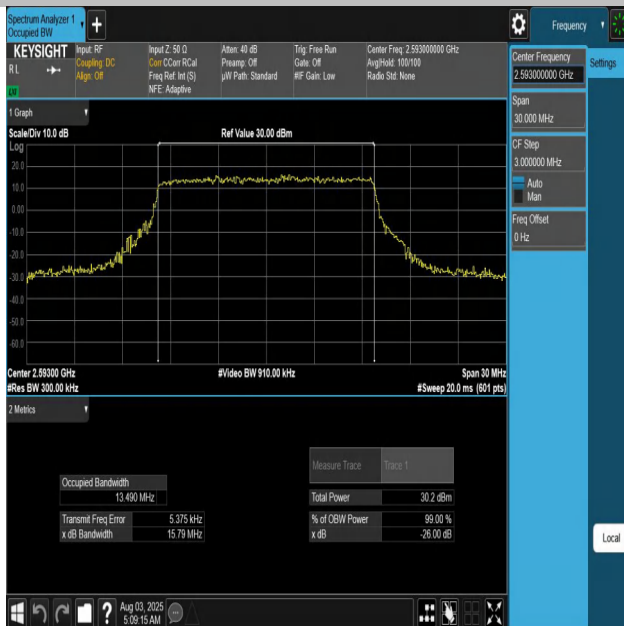
Band41-15MHz-QPSK-40620-75RB#0-PASS
