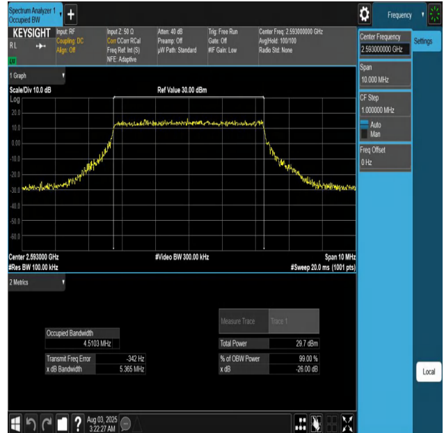
Band41-5MHz-QPSK-40620-25RB#0-PASS
