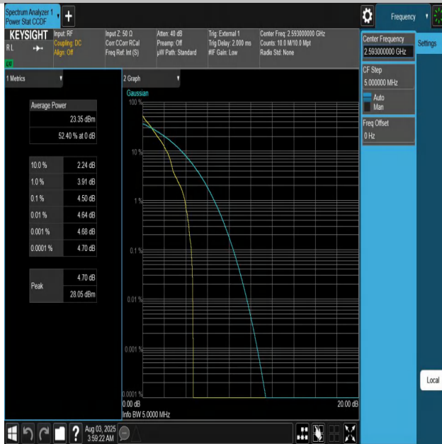
Band41-5MHz-QPSK-40620-1RB#0-PASS
