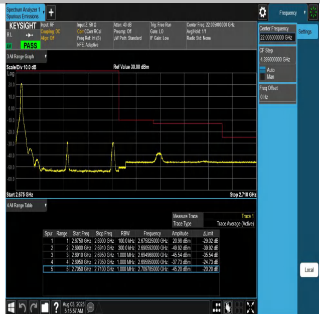
Band41-15MHz-QPSK-41515-1RB#0-PASS
