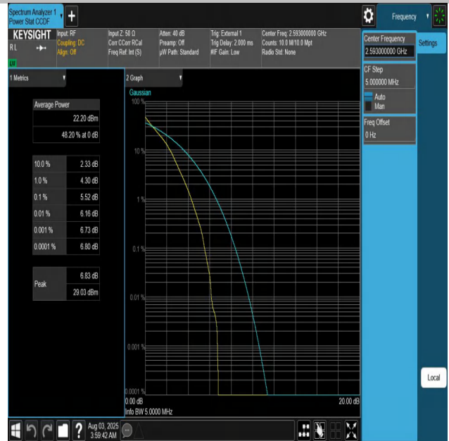
Band41-5MHz-QPSK-40620-25RB#0-PASS
