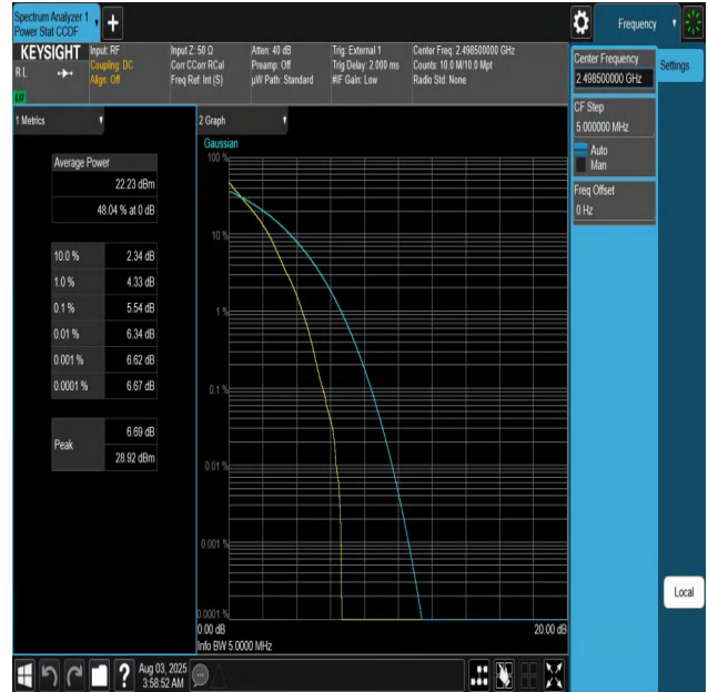
Band41-5MHz-QPSK-39675-25RB#0-PASS
