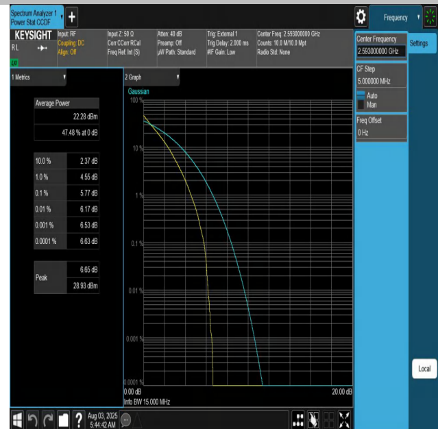
Band41-15MHz-QPSK-40620-75RB#0-PASS
