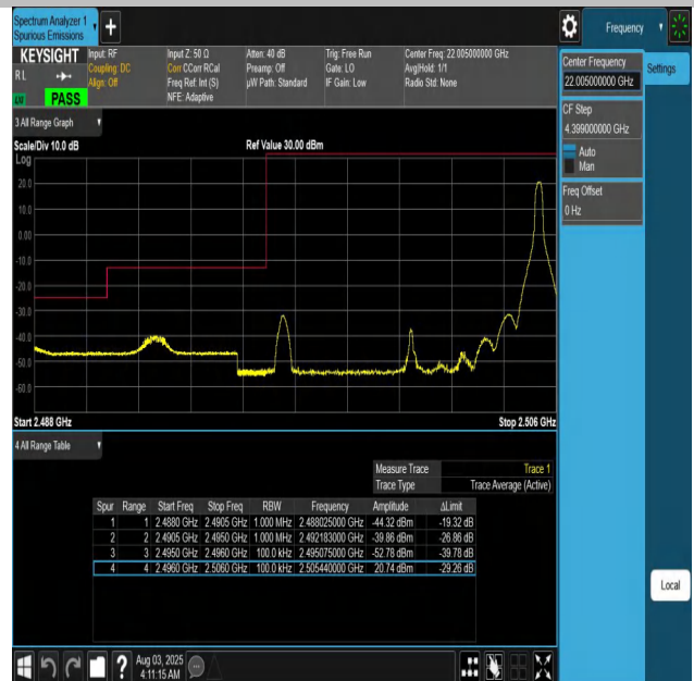
Band41-10MHz-QPSK-39700-1RB#49-PASS
