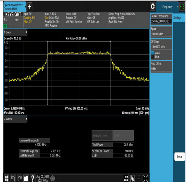
Band41-5MHz-16QAM-39675-25RB#0-PASS
