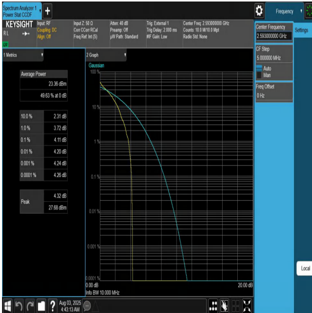
Band41-10MHz-QPSK-40620-1RB#0-PASS
