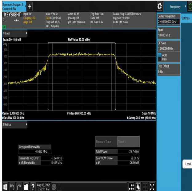
Band41-5MHz-QPSK-39675-25RB#0-PASS
