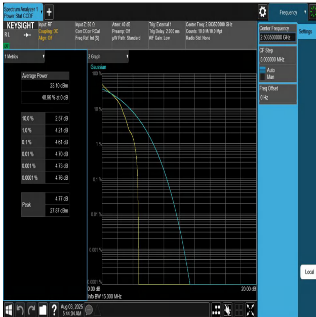
Band41-15MHz-QPSK-39725-1RB#0-PASS
