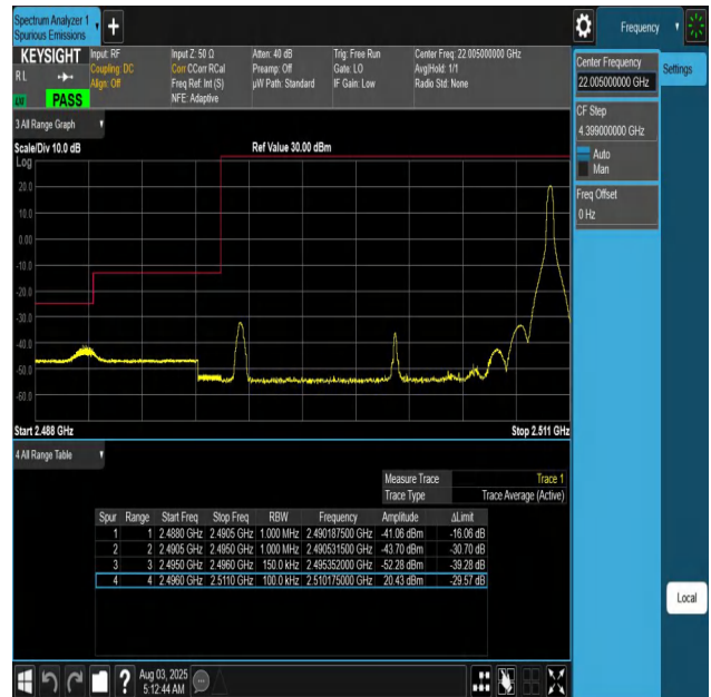
Band41-15MHz-QPSK-39725-1RB#74-PASS
