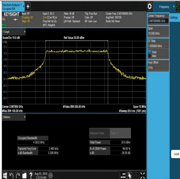
Band41-5MHz-QPSK-41565-25RB#0-PASS
