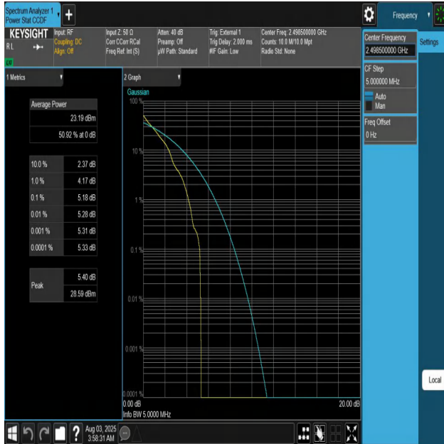
Band41-5MHz-QPSK-39675-1RB#0-PASS
