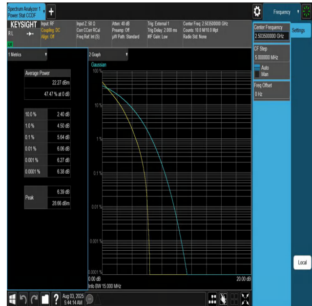
Band41-15MHz-QPSK-39725-75RB#0-PASS
