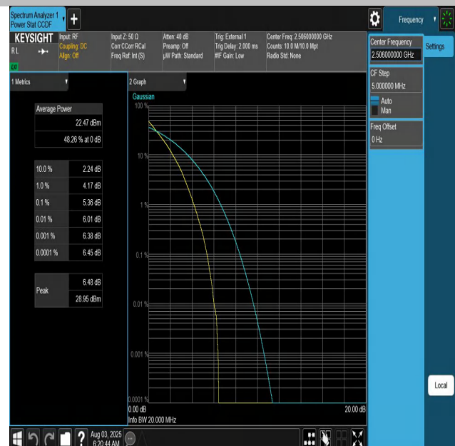
Band41-20MHz-QPSK-39750-100RB#0-PASS
