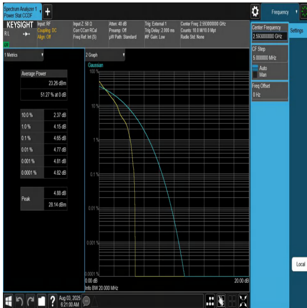
Band41-20MHz-QPSK-40620-1RB#0-PASS
