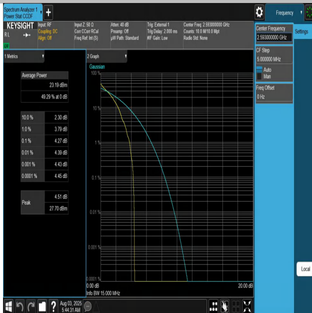
Band41-15MHz-QPSK-40620-1RB#0-PASS
