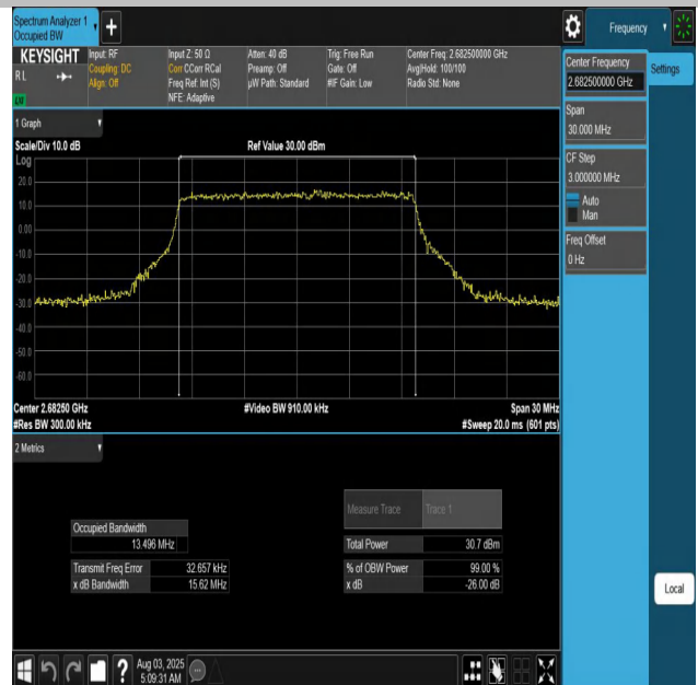
Band41-15MHz-QPSK-41515-75RB#0-PASS
