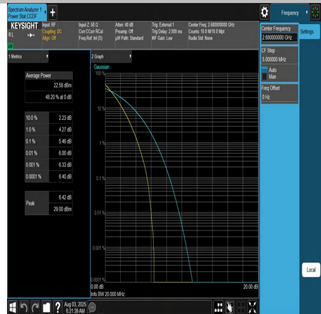
Band41-20MHz-QPSK-41490-100RB#0-PASS
