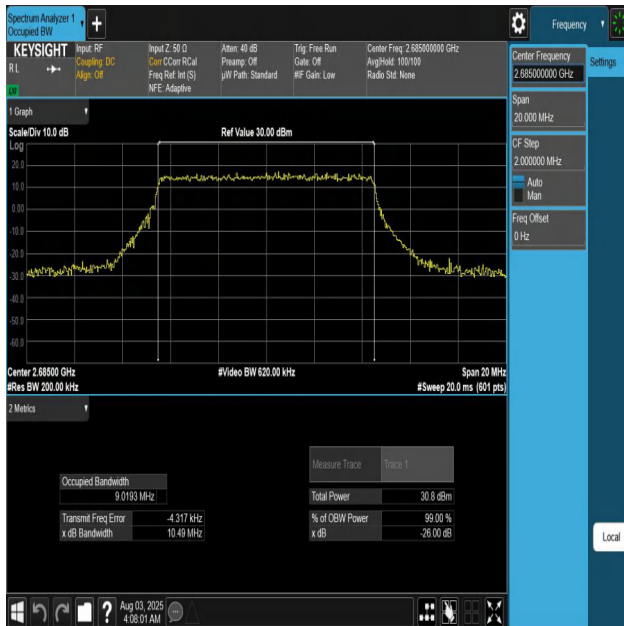
Band41-10MHz-QPSK-41540-50RB#0-PASS
