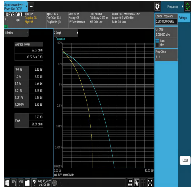
Band41-10MHz-QPSK-40620-50RB#0-PASS
