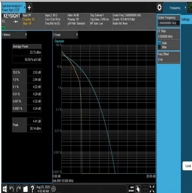
Band41-10MHz-QPSK-41540-1RB#0-PASS
