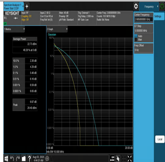
Band41-10MHz-QPSK-41540-50RB#0-PASS
