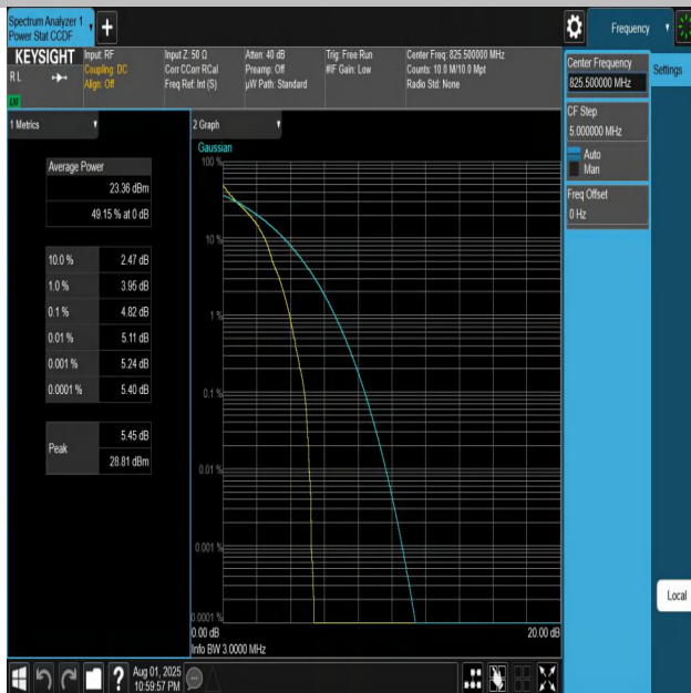
Band5-3MHz-QPSK-20415-1RB#0-PASS
