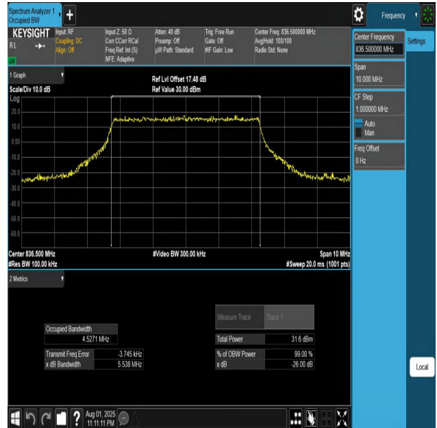
Band5-5MHz-QPSK-20525-25RB#0-PASS
