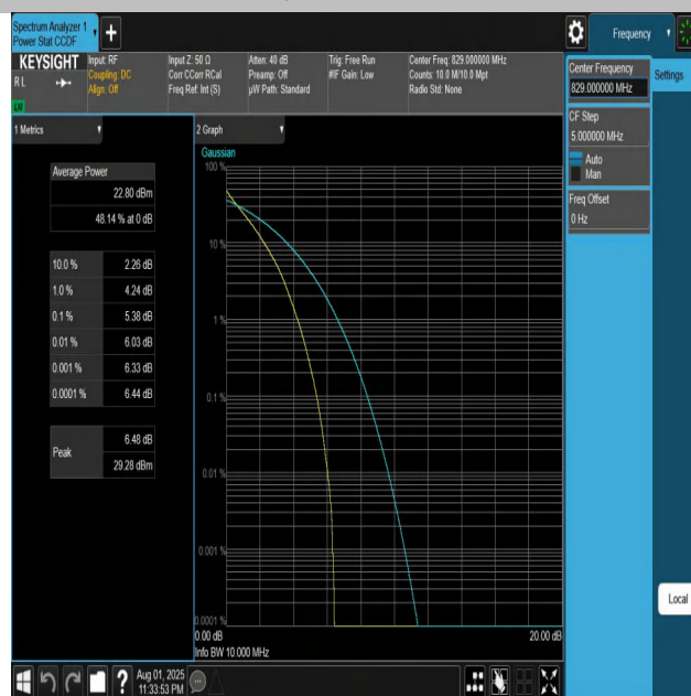
Band5-10MHz-QPSK-20450-50RB#0-PASS
