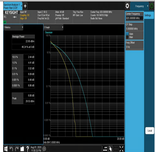
Band5-3MHz-QPSK-20415-15RB#0-PASS
