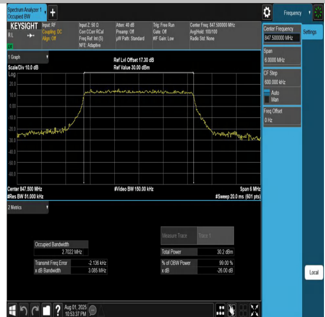
Band5-3MHz-16QAM-20635-15RB#0-PASS
