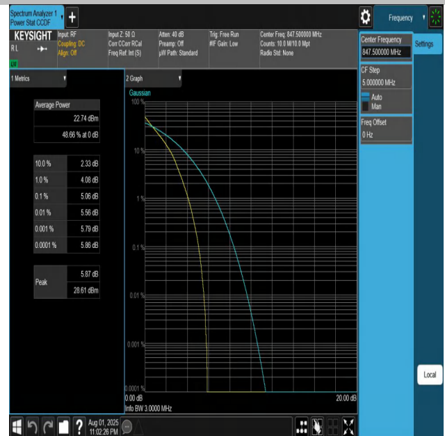
Band5-3MHz-QPSK-20635-15RB#0-PASS
