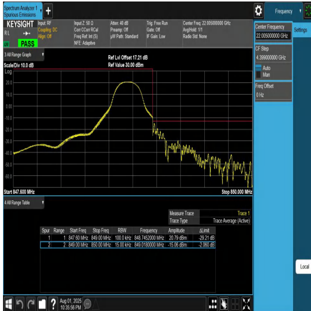
Band5-1.4MHz-QPSK-20643-1RB#5-PASS
