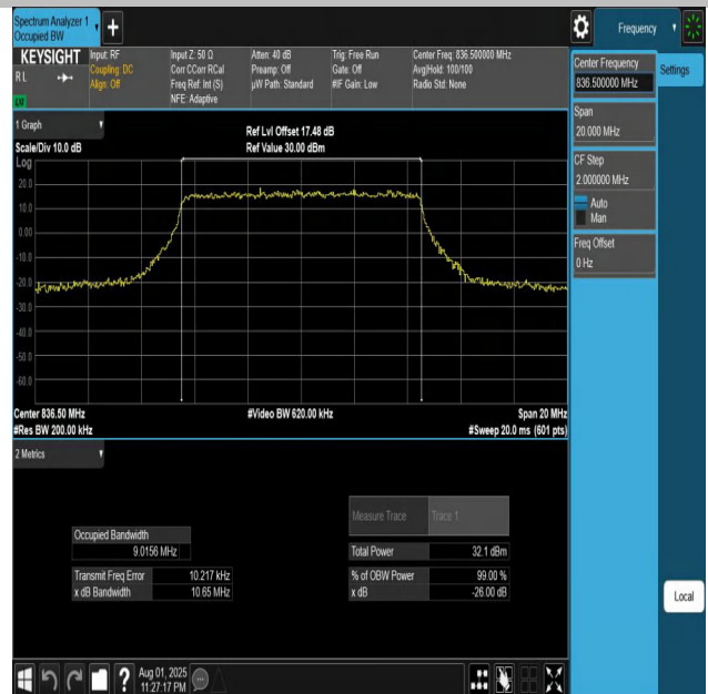
Band5-10MHz-QPSK-20525-50RB#0-PASS
