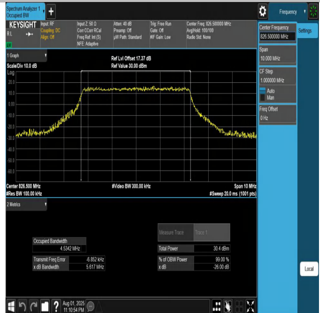
Band5-5MHz-16QAM-20425-25RB#0-PASS
