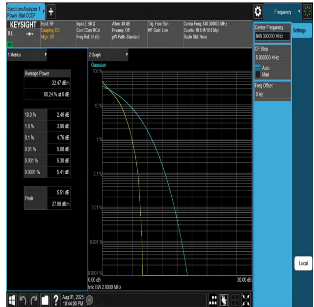
Band5-1.4MHz-QPSK-20643-6RB#0-PASS
