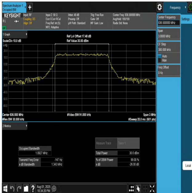
Band5-1.4MHz-16QAM-20525-6RB#0-PASS
