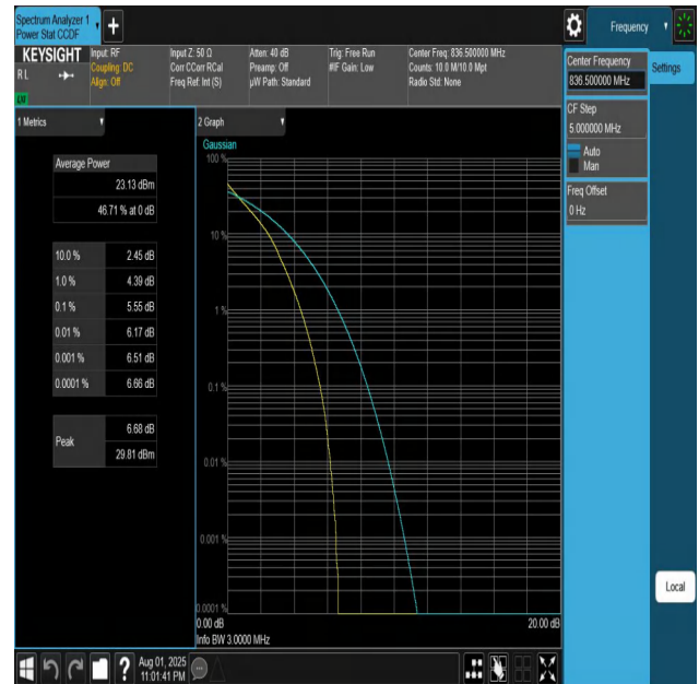
Band5-3MHz-QPSK-20525-15RB#0-PASS
