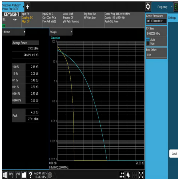
Band5-1.4MHz-QPSK-20643-1RB#0-PASS
