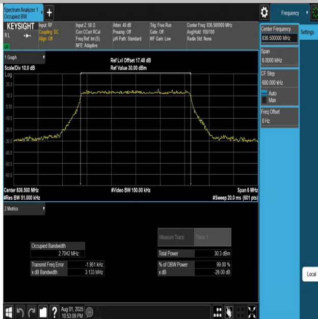
Band5-3MHz-16QAM-20525-15RB#0-PASS
