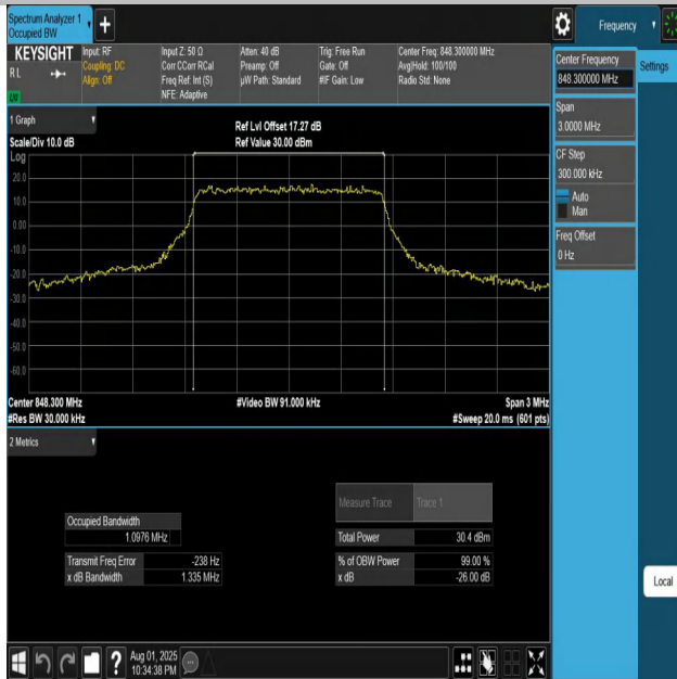
Band5-1.4MHz-QPSK-20643-6RB#0-PASS
