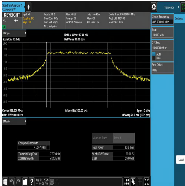
Band5-5MHz-16QAM-20525-25RB#0-PASS
