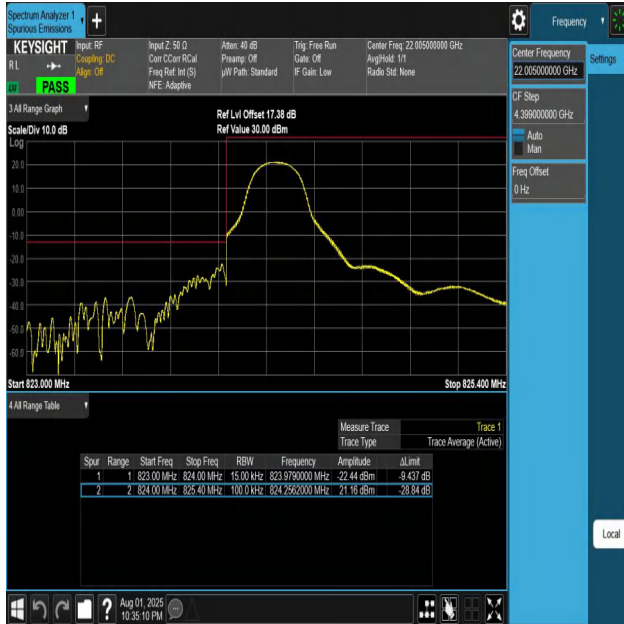
Band5-1.4MHz-QPSK-20407-1RB#0-PASS
