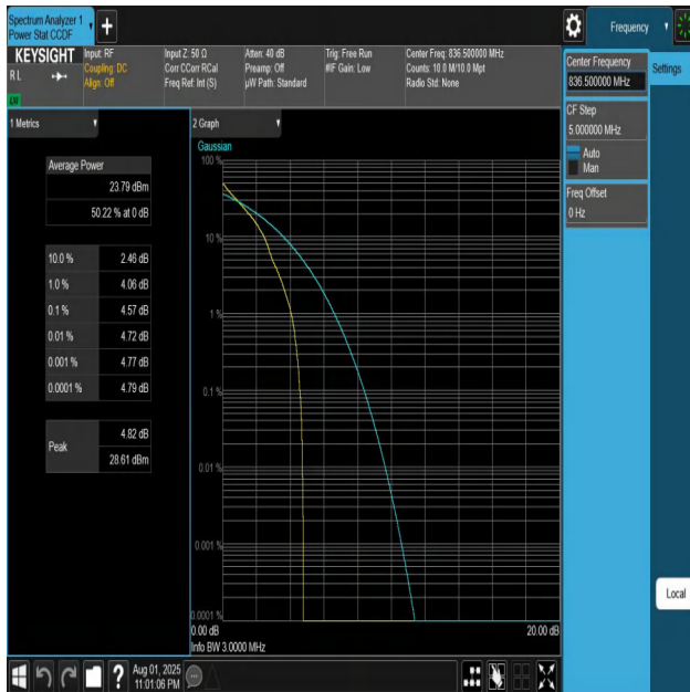
Band5-3MHz-QPSK-20525-1RB#0-PASS
