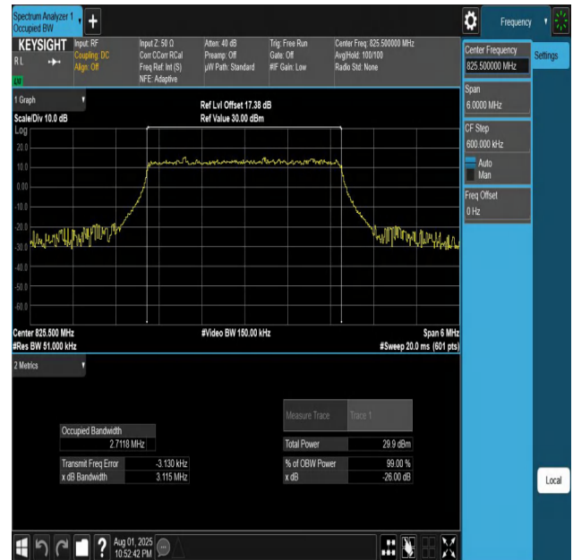
Band5-3MHz-16QAM-20415-15RB#0-PASS
