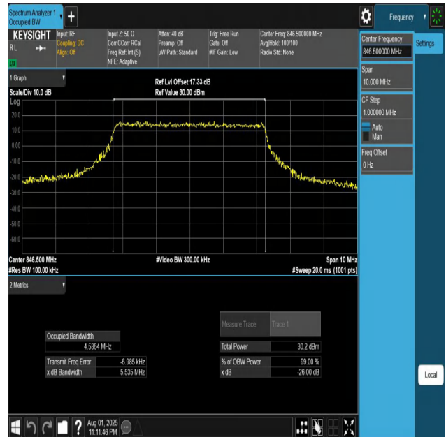
Band5-5MHz-16QAM-20625-25RB#0-PASS
