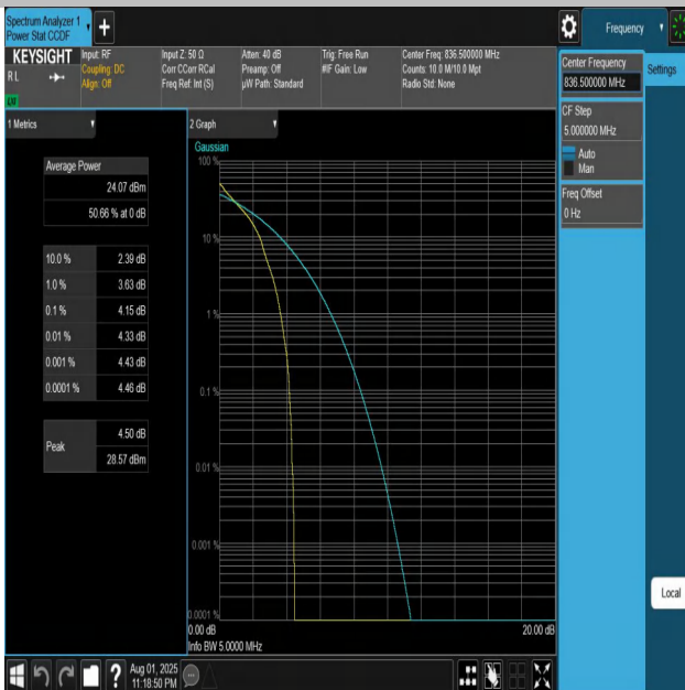
Band5-5MHz-QPSK-20525-1RB#0-PASS
