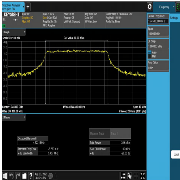
Band66-5MHz-16QAM-132322-25RB#0-PASS
