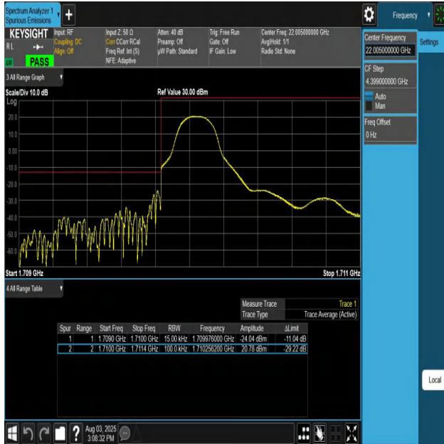
Band66-1.4MHz-QPSK-131979-1RB#0-PASS
