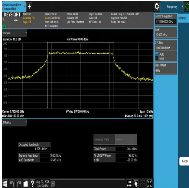
Band66-5MHz-QPSK-131997-25RB#0-PASS
