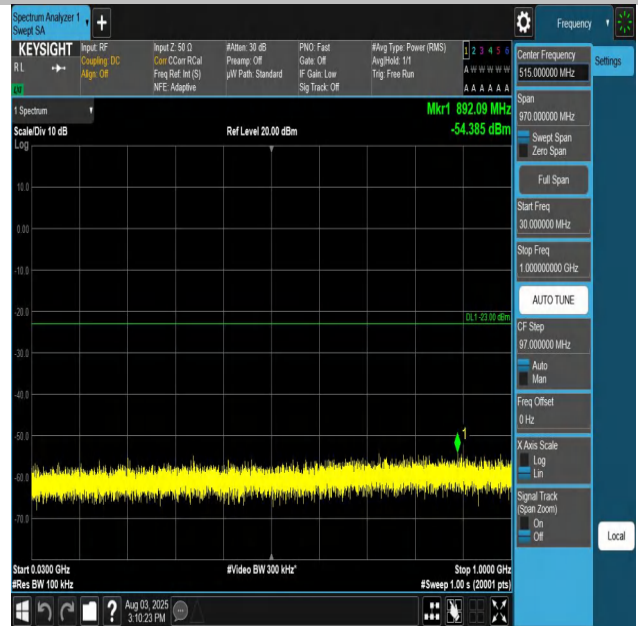
Band66-1.4MHz-QPSK-132322-1RB#0-30~1000-PASS
