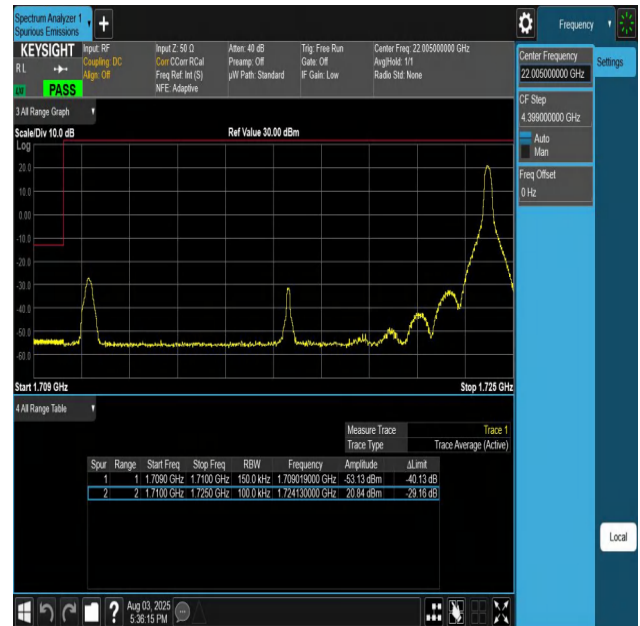
Band66-15MHz-QPSK-132047-1RB#74-PASS
