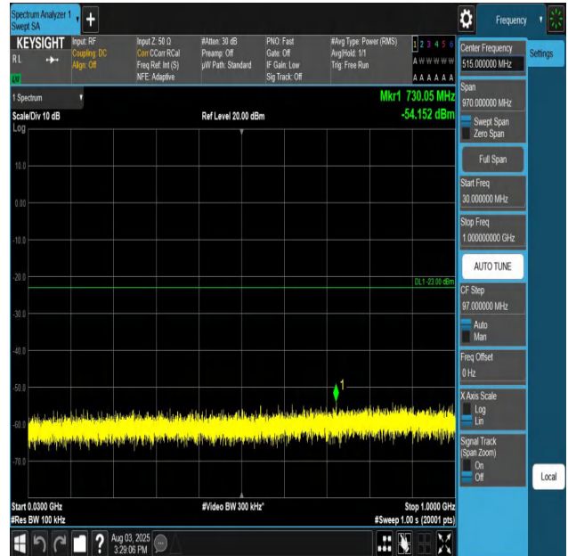
Band66-3MHz-QPSK-131987-1RB#0-30~1000-PASS
