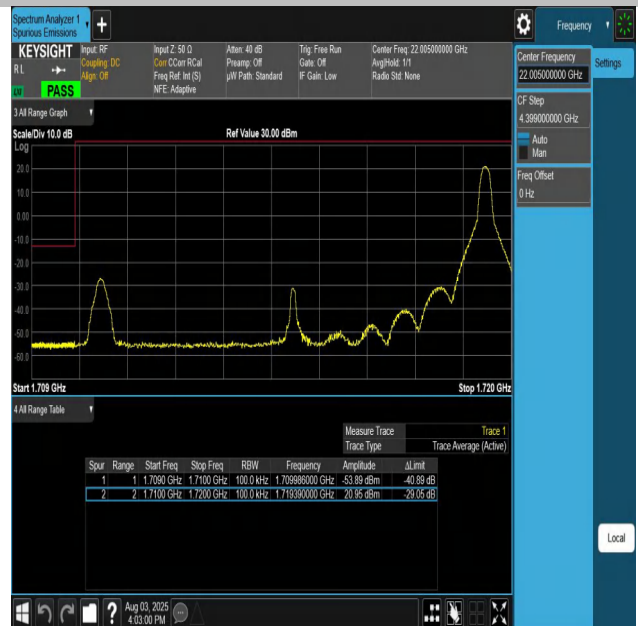
Band66-10MHz-QPSK-132022-1RB#49-PASS
