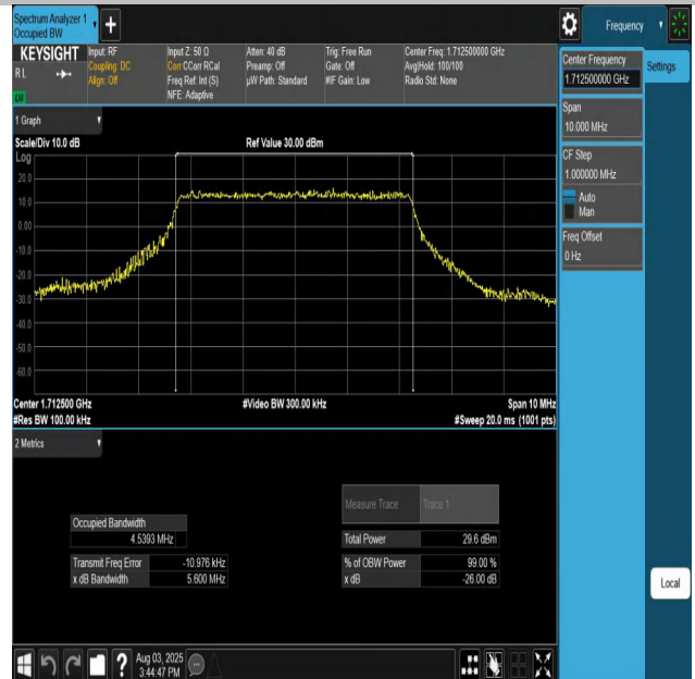
Band66-5MHz-16QAM-131997-25RB#0-PASS
