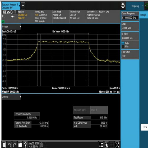
Band66-10MHz-QPSK-132022-50RB#0-PASS
