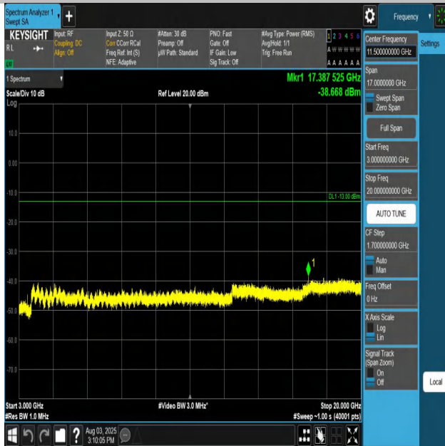
Band66-1.4MHz-QPSK-131979-1RB#0-3000~20000-PAS
