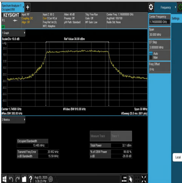
Band66-15MHz-QPSK-132322-75RB#0-PASS
