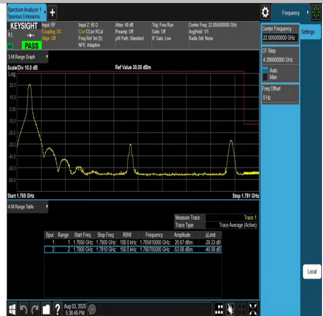
Band66-15MHz-QPSK-132597-1RB#0-PASS
