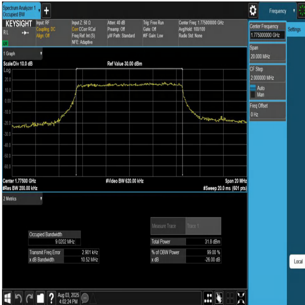
Band66-10MHz-QPSK-132622-50RB#0-PASS
