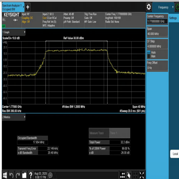
Band66-20MHz-QPSK-132572-100RB#0-PASS
