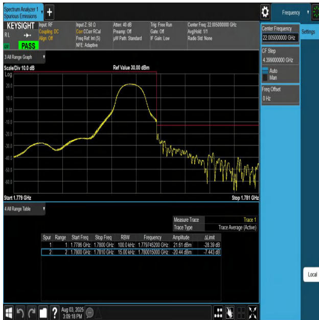
Band66-1.4MHz-QPSK-132665-1RB#5-PASS
