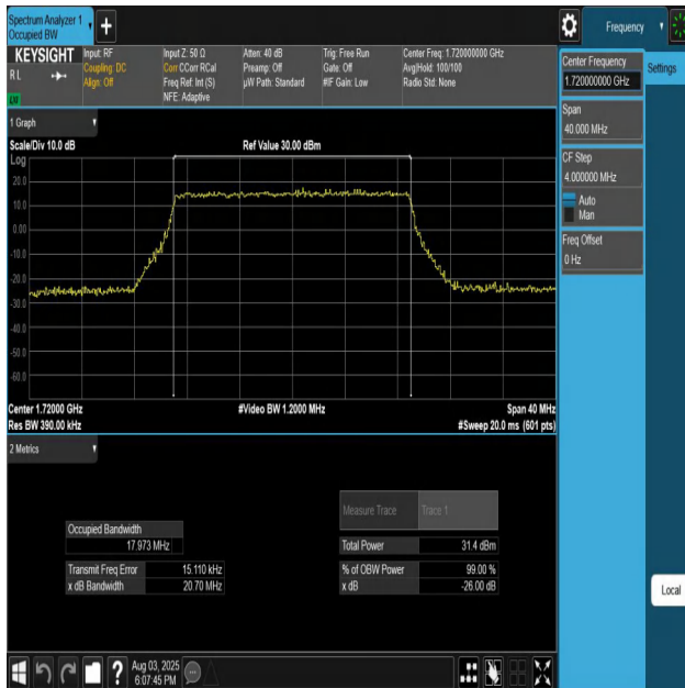
Band66-20MHz-QPSK-132072-100RB#0-PASS
