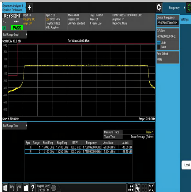
Band66-15MHz-QPSK-132047-75RB#0-PASS
