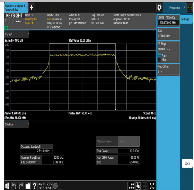
Band66-3MHz-16QAM-132657-15RB#0-PASS
