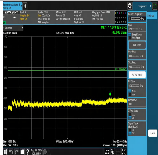
Band66-3MHz-QPSK-131987-1RB#0-3000~20000-PASS
