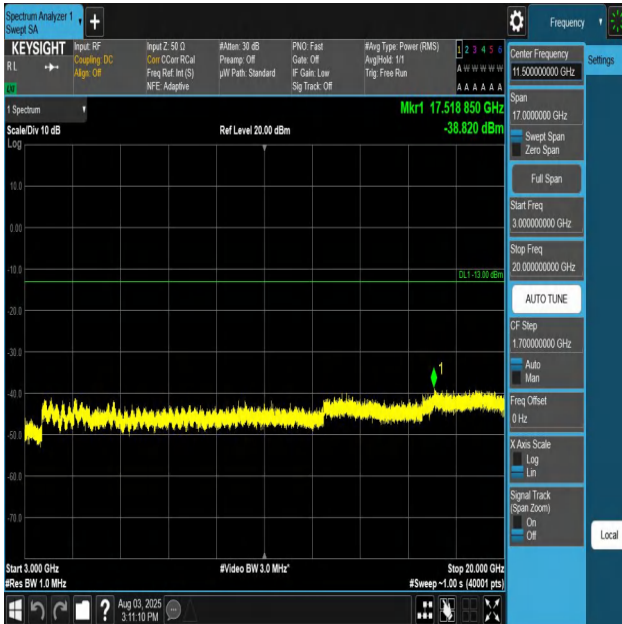
Band66-1.4MHz-QPSK-132665-1RB#0-3000~20000-PAS S
