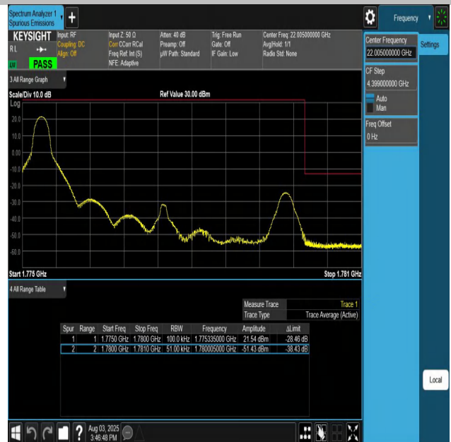
Band66-5MHz-QPSK-132647-1RB#0-PASS
