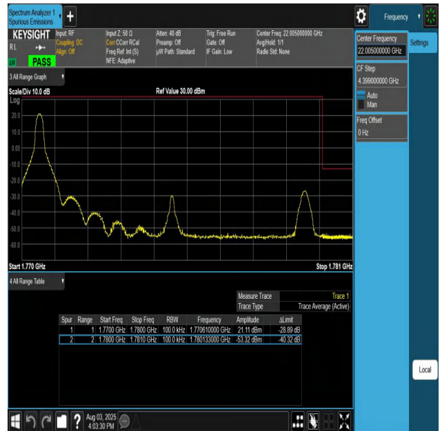
Band66-10MHz-QPSK-132622-1RB#0-PASS
