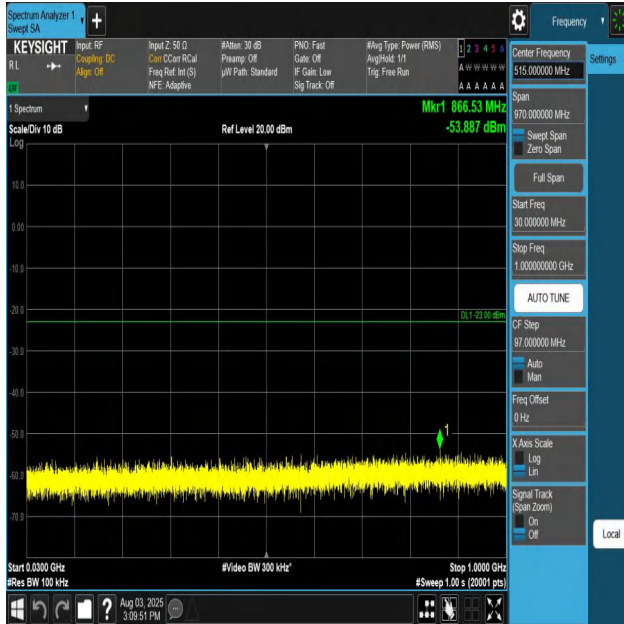
Band66-1.4MHz-QPSK-131979-1RB#0-30~1000-PASS
