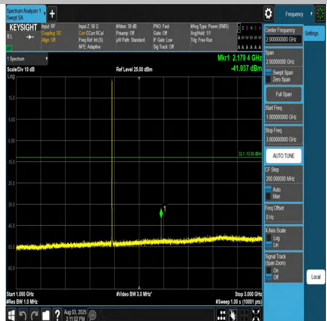
Band66-1.4MHz-QPSK-132665-1RB#0-1000~3000-PASS
