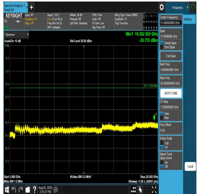
Band66-1.4MHz-QPSK-132322-1RB#0-3000~20000-PASS
