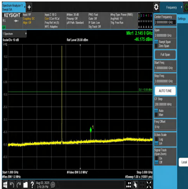
Band66-1.4MHz-QPSK-132322-1RB#0-1000~3000-PASS
