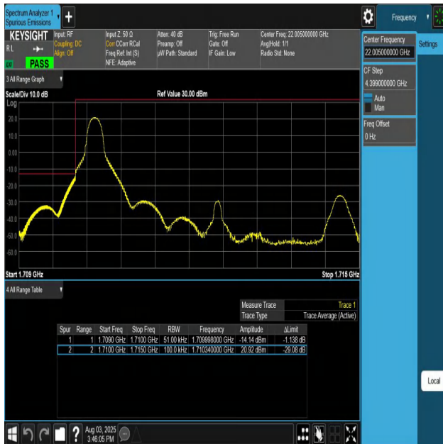
Band66-5MHz-QPSK-131997-1RB#0-PASS
