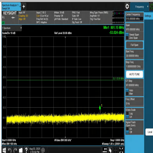
Band66-1.4MHz-QPSK-132665-1RB#0-30~1000-PASS
