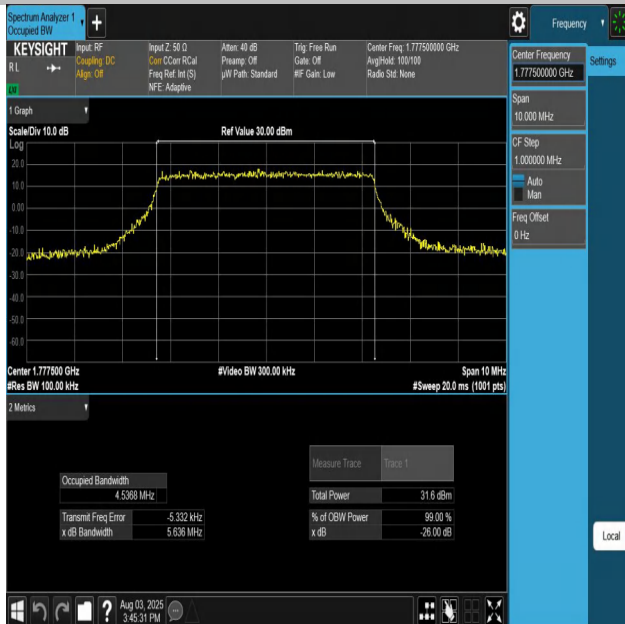
Band66-5MHz-QPSK-132647-25RB#0-PASS
