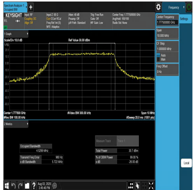
Band66-5MHz-16QAM-132647-25RB#0-PASS
