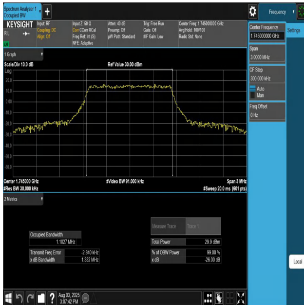
Band66-1.4MHz-16QAM-132322-6RB#0-PASS
