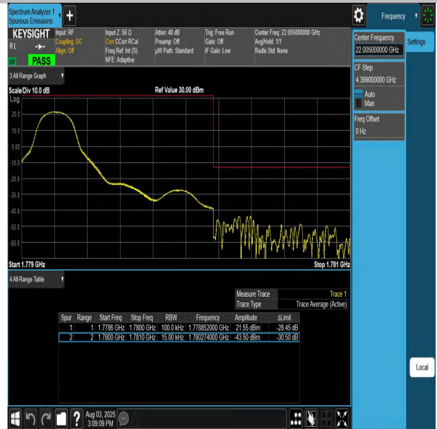
Band66-1.4MHz-QPSK-132665-1RB#0-PASS
