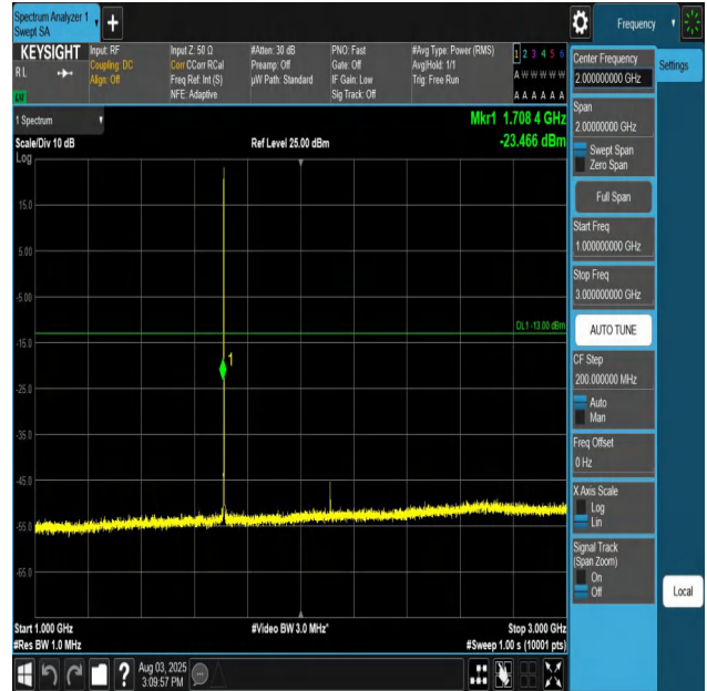
Band66-1.4MHz-QPSK-131979-1RB#0-1000~3000-PASS
