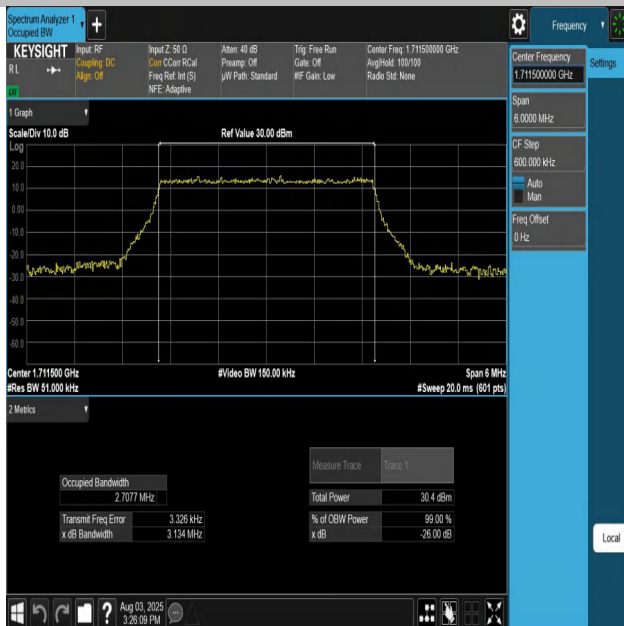
Band66-3MHz-QPSK-131987-15RB#0-PASS
