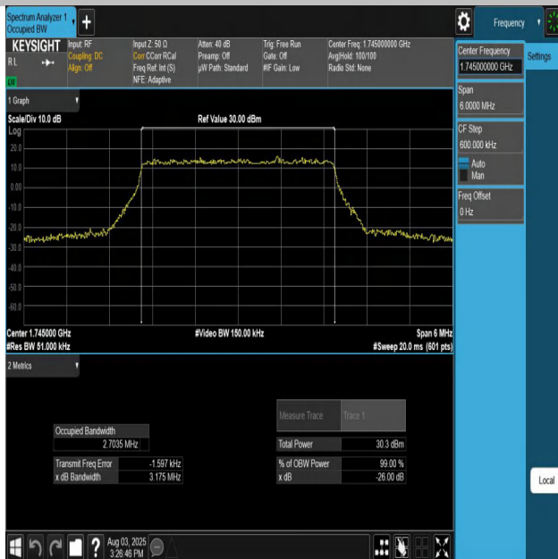
Band66-3MHz-16QAM-132322-15RB#0-PASS
