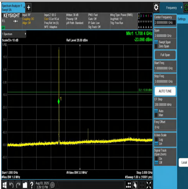
Band66-3MHz-QPSK-131987-1RB#0-1000~3000-PASS
