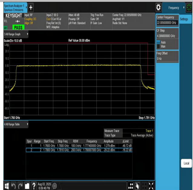
Band66-20MHz-QPSK-132572-100RB#0-PASS
