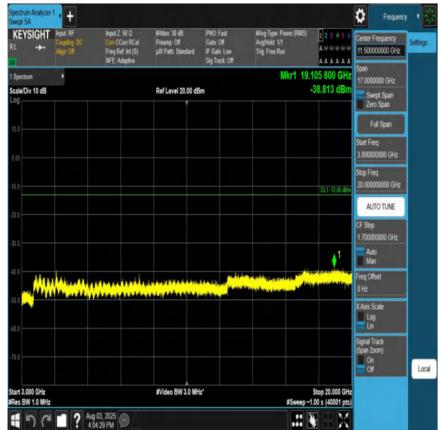
Band66-10MHz-QPSK-132022-1RB#0-3000~20000-PASS
