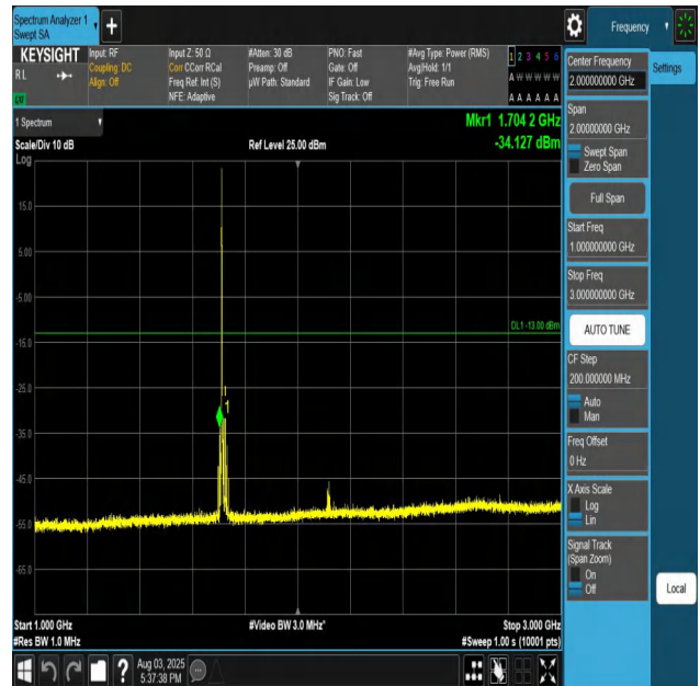
Band66-15MHz-QPSK-132047-1RB#0-1000~3000-PASS
