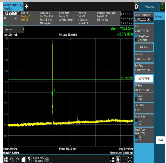
Band66-5MHz-QPSK-131997-1RB#0-1000~3000-PASS
