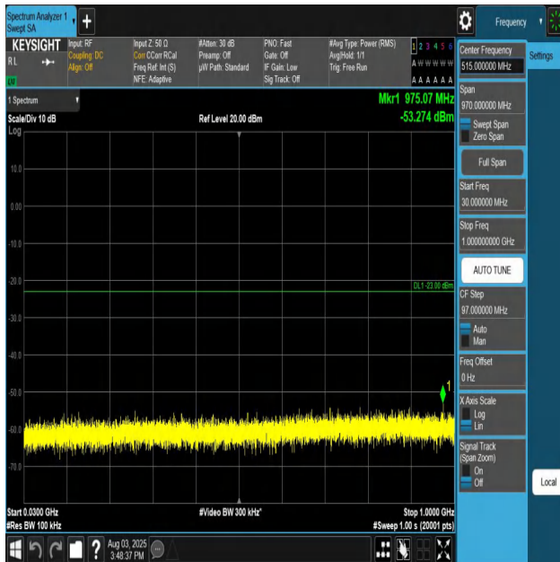
Band66-5MHz-QPSK-132647-1RB#0-30~1000-PASS
