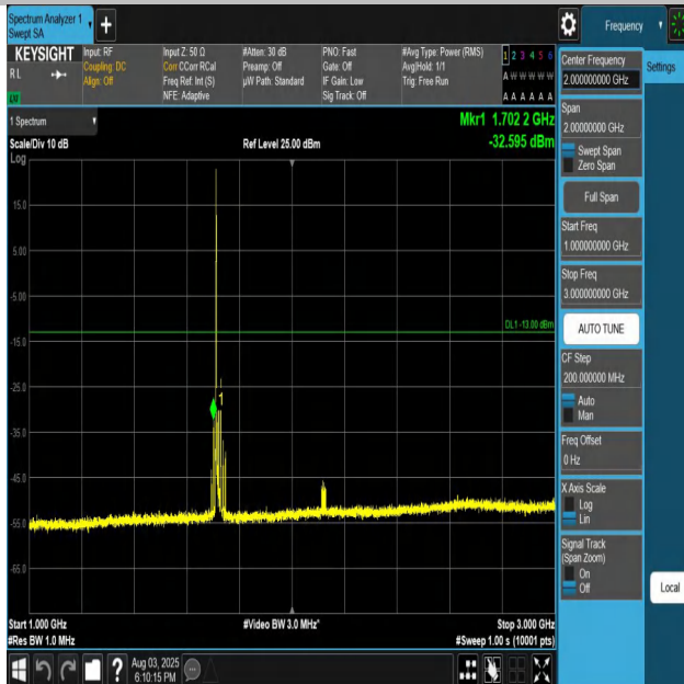
Band66-20MHz-QPSK-132072-1RB#0-1000~3000-PASS
