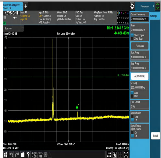
Band66-10MHz-QPSK-132322-1RB#0-1000~3000-PASS
