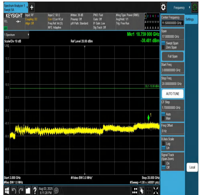
Band66-20MHz-QPSK-132572-1RB#0-3000~20000-PASS
