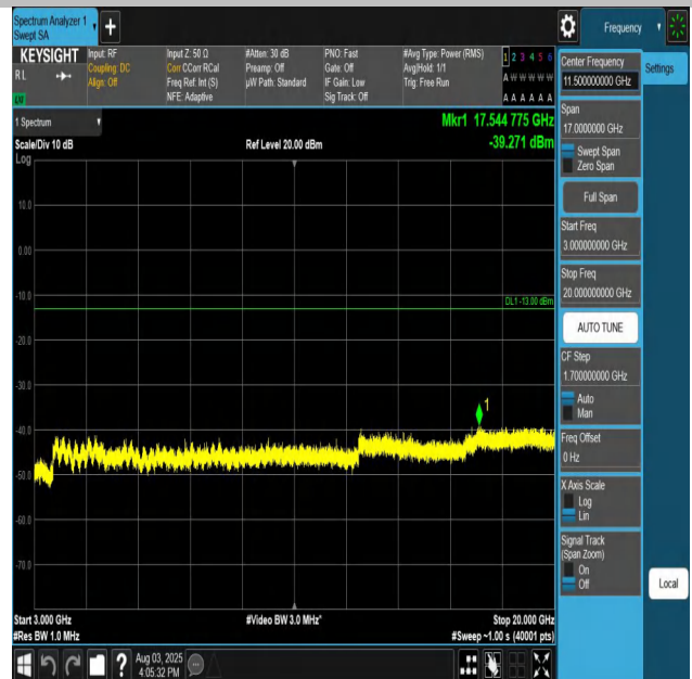
Band66-10MHz-QPSK-132622-1RB#0-3000~20000-PASS
