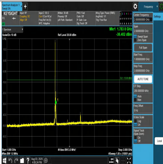
Band66-10MHz-QPSK-132622-1RB#0-1000~3000-PASS
