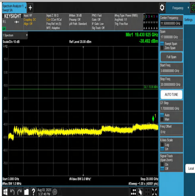
Band66-15MHz-QPSK-132047-1RB#0-3000~20000-PASS
