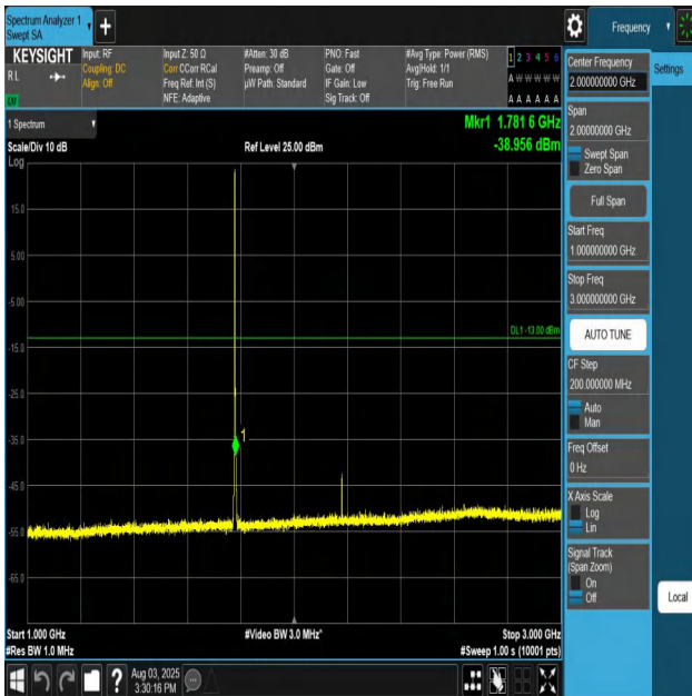
Band66-3MHz-QPSK-132657-1RB#0-1000~3000-PASS
