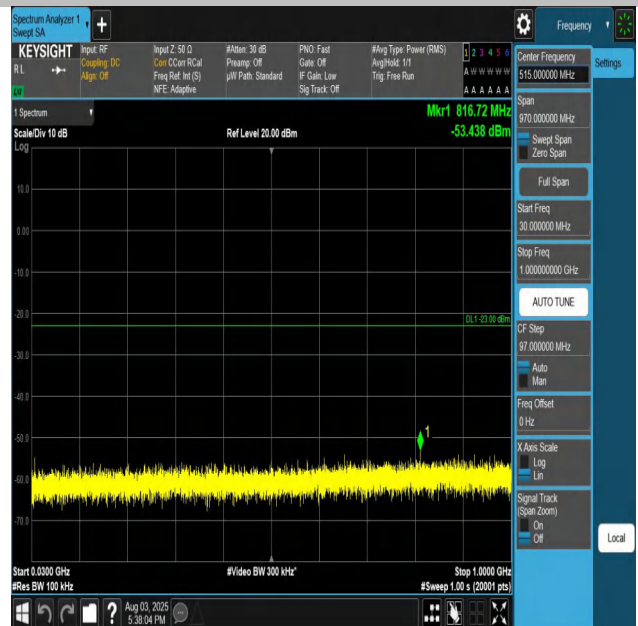
Band66-15MHz-QPSK-132322-1RB#0-30~1000-PASS
