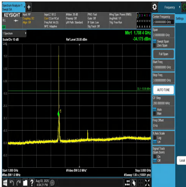
Band66-10MHz-QPSK-132022-1RB#0-1000~3000-PASS
