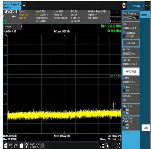
Band66-20MHz-QPSK-132072-1RB#0-30~1000-PASS
