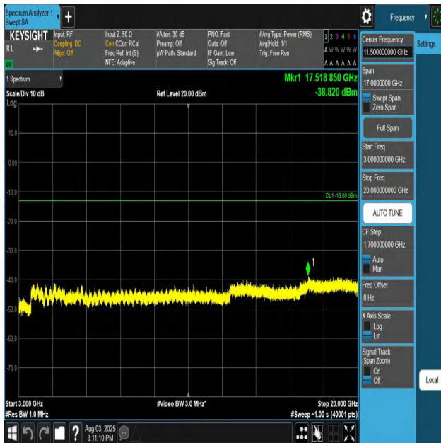
Band66-1.4MHz-QPSK-132665-1RB#0-3000~20000-PAS S
