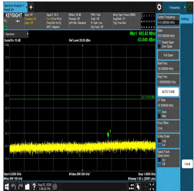
Band66-5MHz-QPSK-132322-1RB#0-30~1000-PASS
