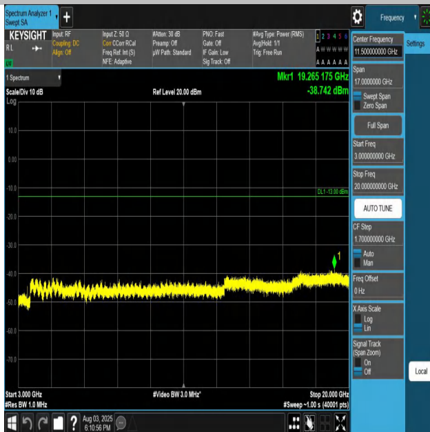
Band66-20MHz-QPSK-132322-1RB#0-3000~20000-PASS
