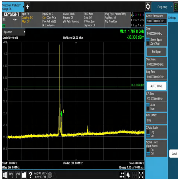
Band66-20MHz-QPSK-132572-1RB#0-1000~3000-PASS
