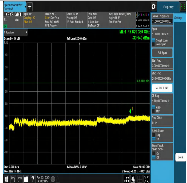
Band66-20MHz-QPSK-132072-1RB#0-3000~20000-PASS
