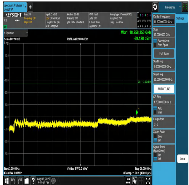
Band66-15MHz-QPSK-132322-1RB#0-3000~20000-PASS
