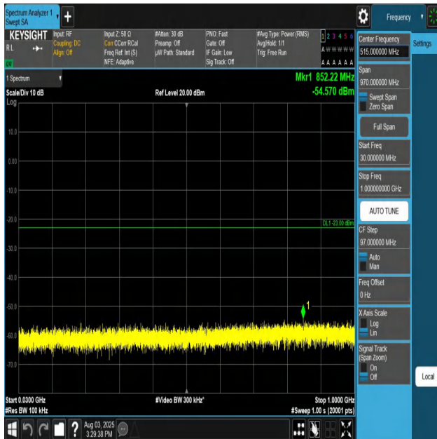
Band66-3MHz-QPSK-132322-1RB#0-30~1000-PASS
