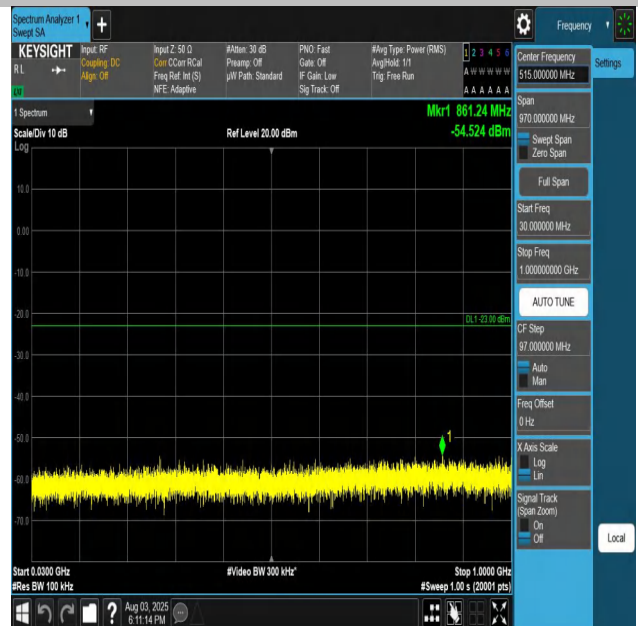
Band66-20MHz-QPSK-132572-1RB#0-30~1000-PASS
