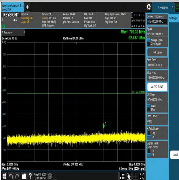
Band66-5MHz-QPSK-131997-1RB#0-30~1000-PASS
