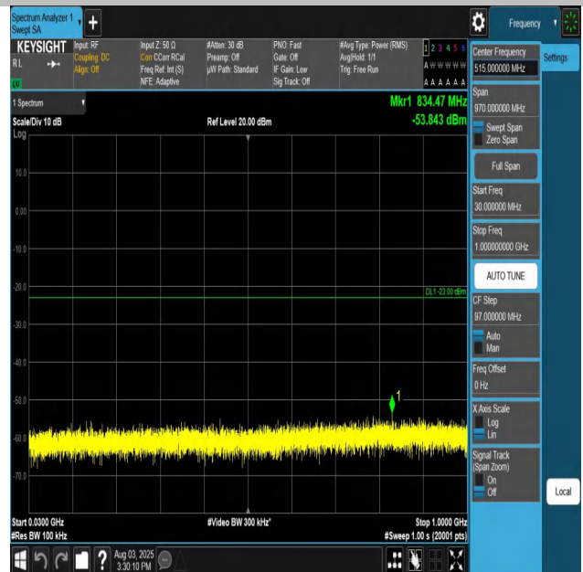
Band66-3MHz-QPSK-132657-1RB#0-30~1000-PASS
