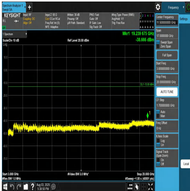
Band66-15MHz-QPSK-132597-1RB#0-3000~20000-PASS
