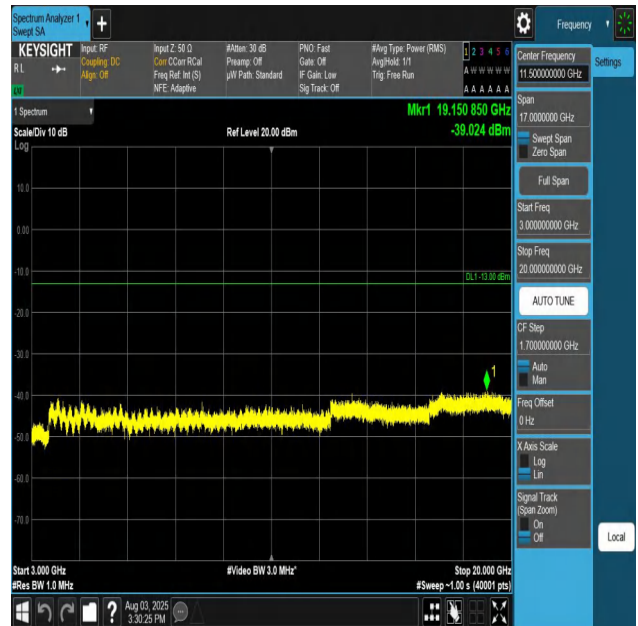
Band66-3MHz-QPSK-132657-1RB#0-3000~20000-PASS
