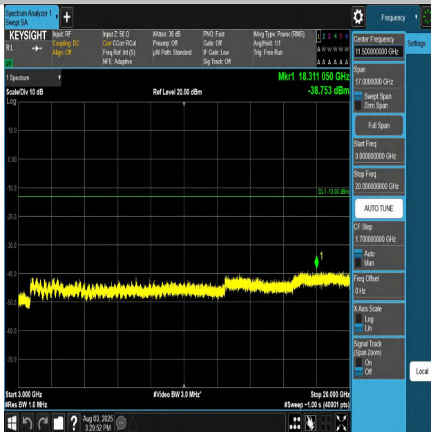
Band66-3MHz-QPSK-132322-1RB#0-3000~20000-PASS
