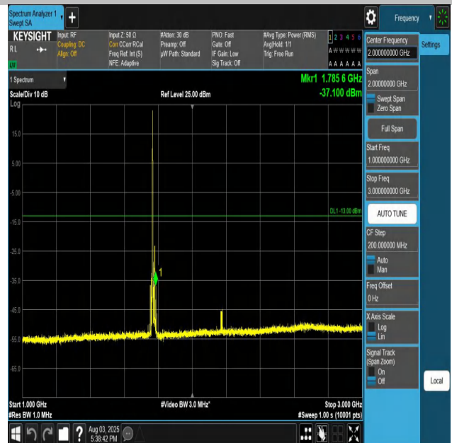
Band66-15MHz-QPSK-132597-1RB#0-1000~3000-PASS
