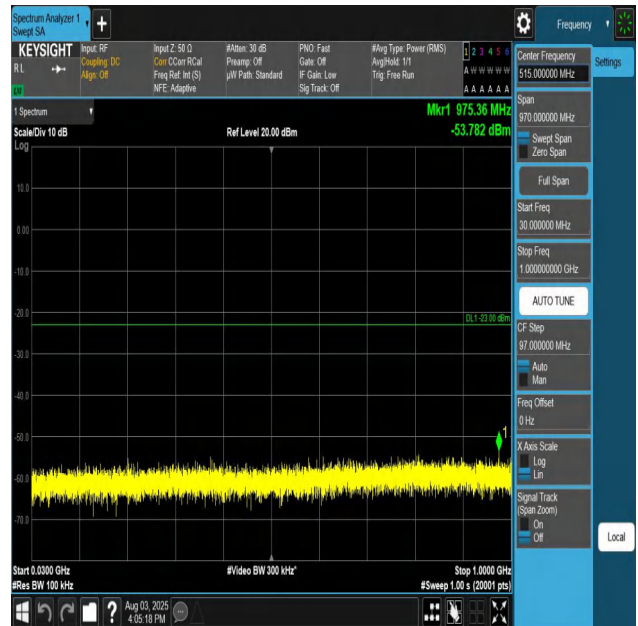
Band66-10MHz-QPSK-132622-1RB#0-30~1000-PASS
