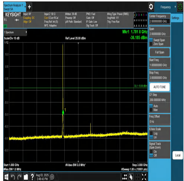
Band66-5MHz-QPSK-132647-1RB#0-1000~3000-PASS
