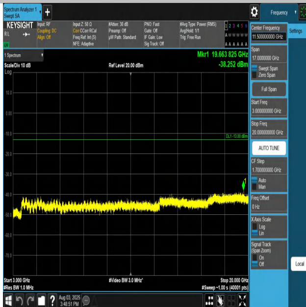
Band66-5MHz-QPSK-132647-1RB#0-3000~20000-PASS
