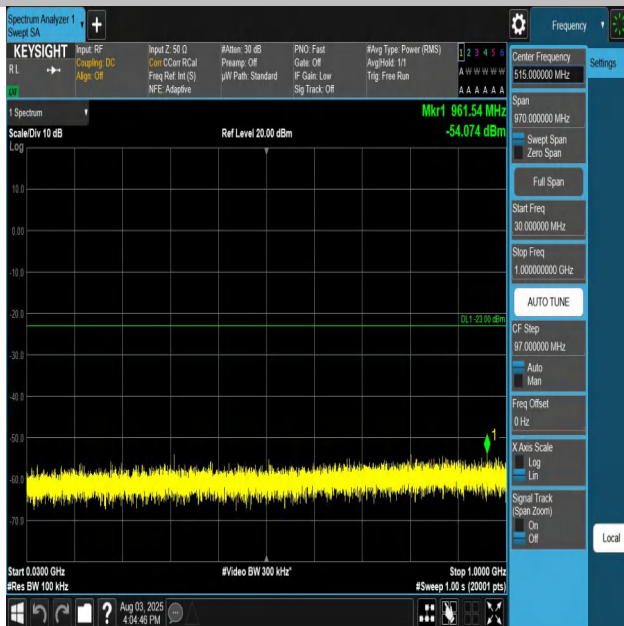
Band66-10MHz-QPSK-132322-1RB#0-30~1000-PASS
