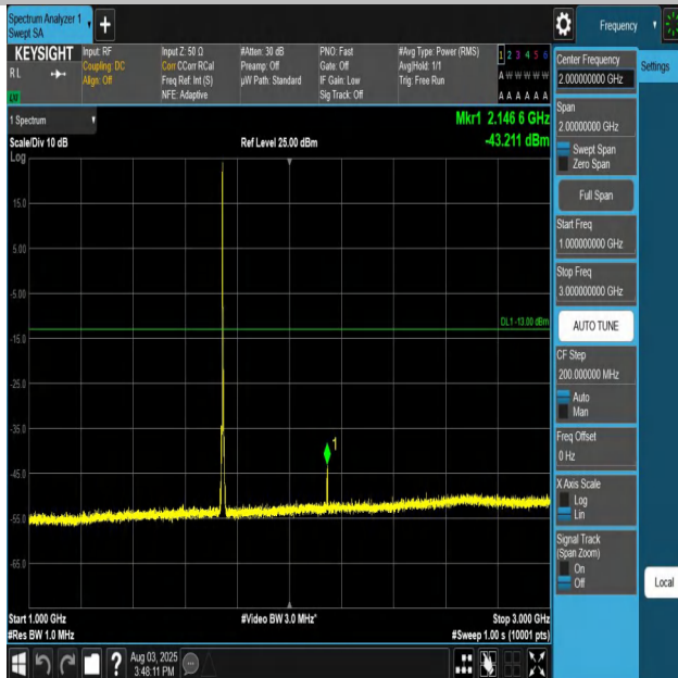
Band66-5MHz-QPSK-132322-1RB#0-1000~3000-PASS
