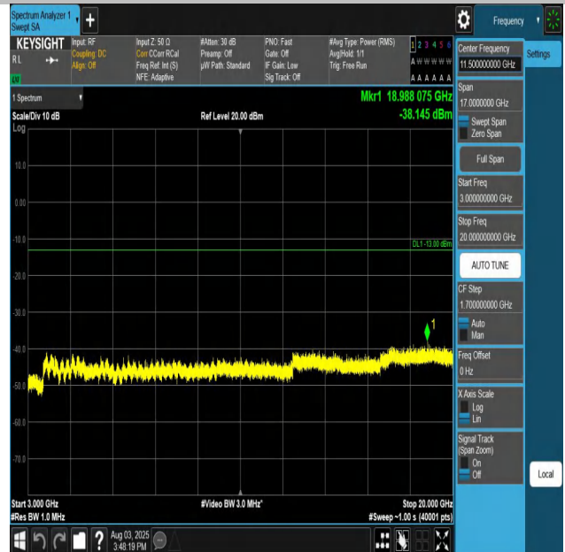
Band66-5MHz-QPSK-132322-1RB#0-3000~20000-PASS
