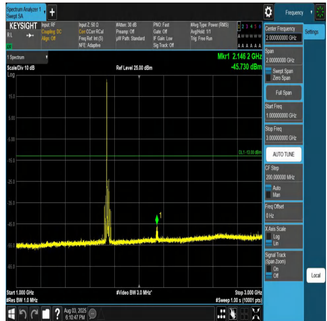
Band66-20MHz-QPSK-132322-1RB#0-1000~3000-PASS
