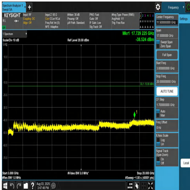
Band66-5MHz-QPSK-131997-1RB#0-3000~20000-PASS
