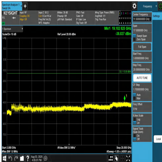
Band66-10MHz-QPSK-132322-1RB#0-3000~20000-PASS
