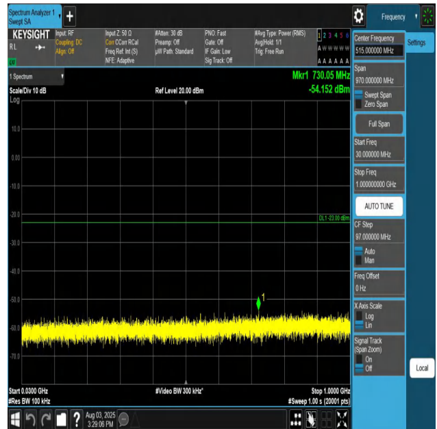
Band66-3MHz-QPSK-131987-1RB#0-30~1000-PASS
