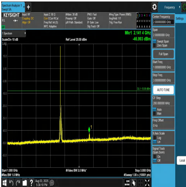
Band66-15MHz-QPSK-132322-1RB#0-1000~3000-PASS
