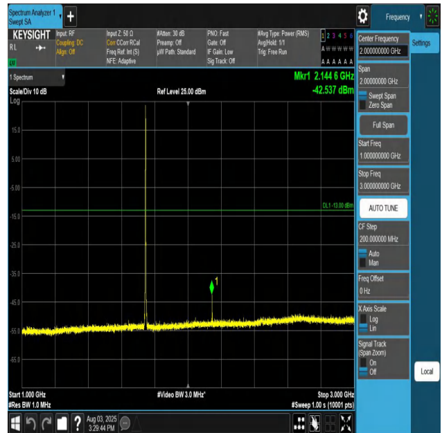
Band66-3MHz-QPSK-132322-1RB#0-1000~3000-PASS
