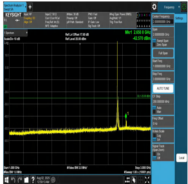
Band7-15MHz-QPSK-21100-1RB#0-1000~3000-PASS
