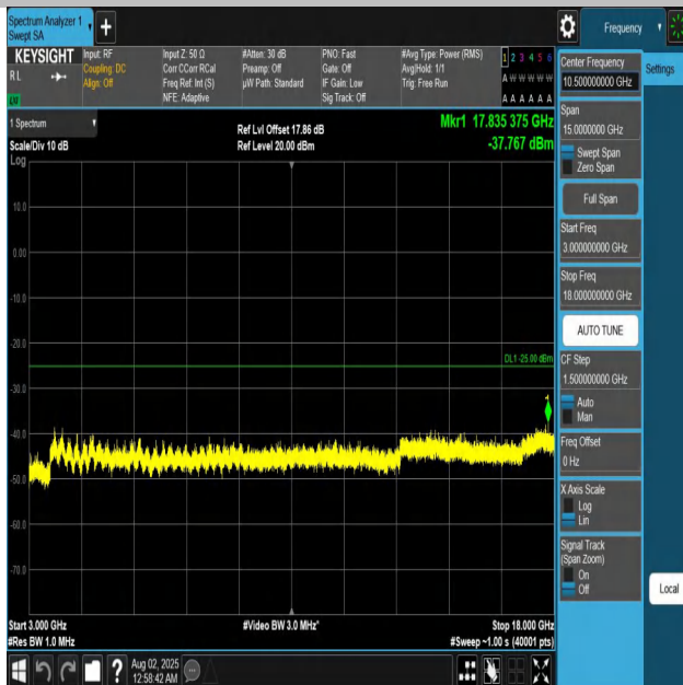
Band7-15MHz-QPSK-20825-1RB#0-3000~18000-PASS
