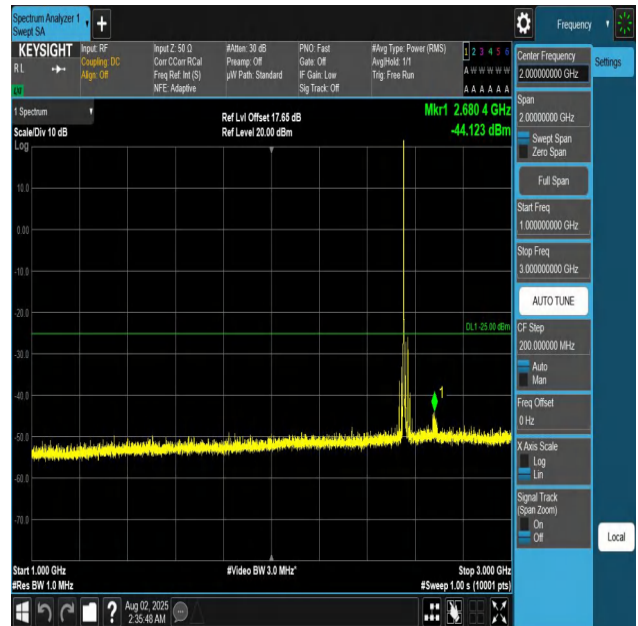
Band7-20MHz-QPSK-21350-1RB#0-1000~3000-PASS
