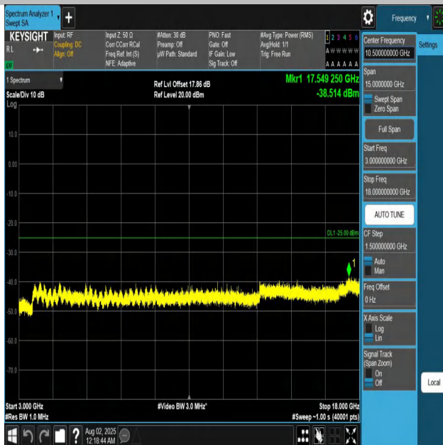
Band7-10MHz-QPSK-21400-1RB#0-3000~18000-PASS
