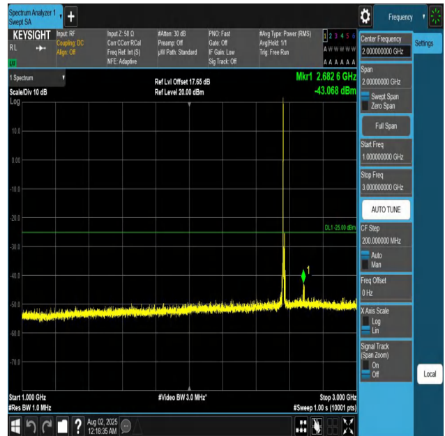
Band7-10MHz-QPSK-21400-1RB#0-1000~3000-PASS
