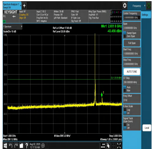
Band7-10MHz-QPSK-21100-1RB#0-1000~3000-PASS
