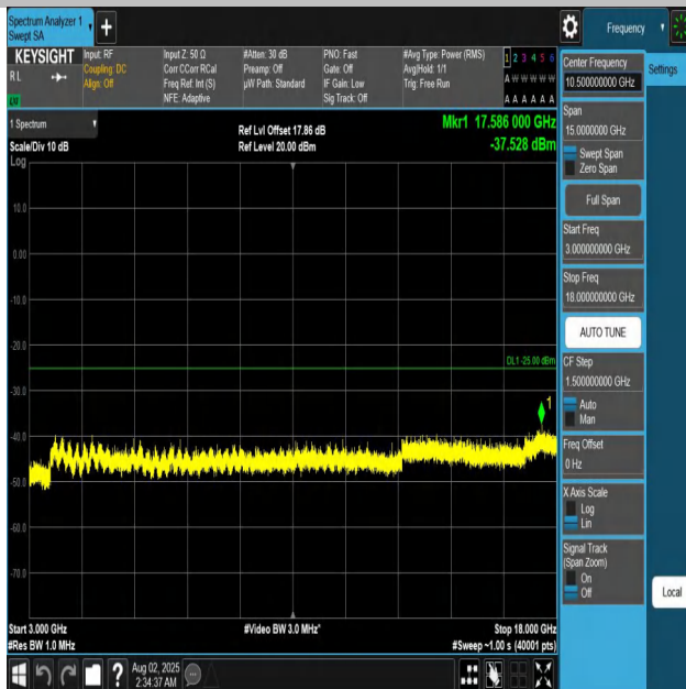
Band7-20MHz-QPSK-20850-1RB#0-3000~18000-PASS
