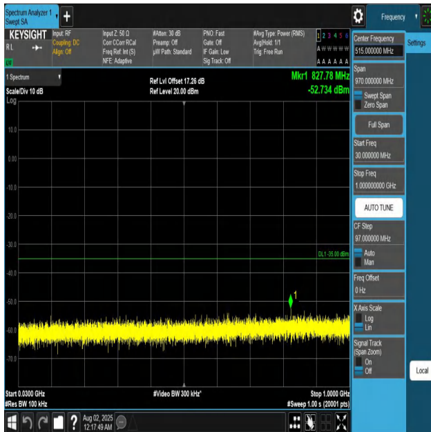
Band7-10MHz-QPSK-21100-1RB#0-30~1000-PASS
