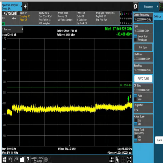
Band7-15MHz-QPSK-21375-1RB#0-3000~18000-PASS
