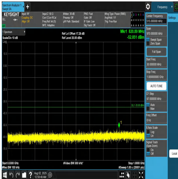
Band7-15MHz-QPSK-21375-1RB#0-30~1000-PASS
