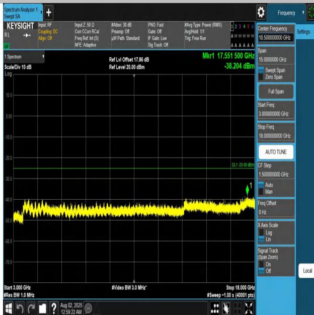
Band7-15MHz-QPSK-21100-1RB#0-3000~18000-PASS
