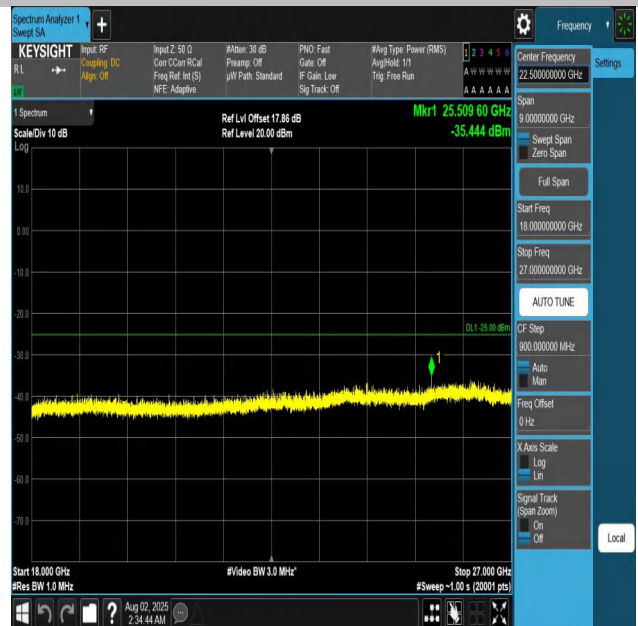
Band7-20MHz-QPSK-20850-1RB#0-18000~27000-PASS
