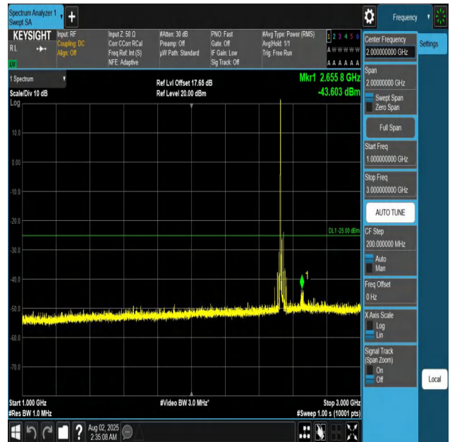
Band7-20MHz-QPSK-21100-1RB#0-1000~3000-PASS
