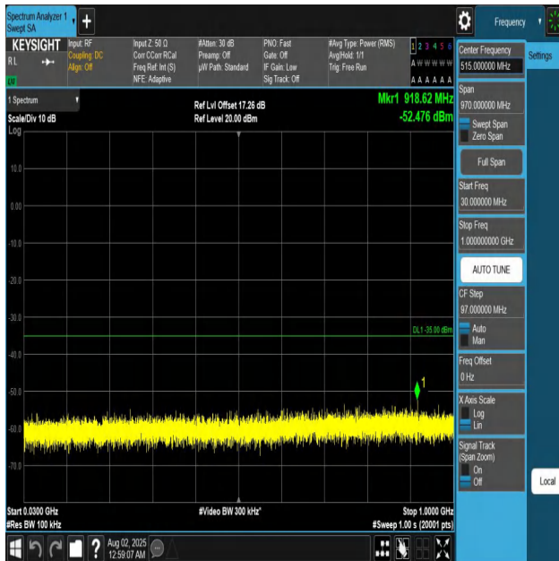
Band7-15MHz-QPSK-21100-1RB#0-30~1000-PASS
