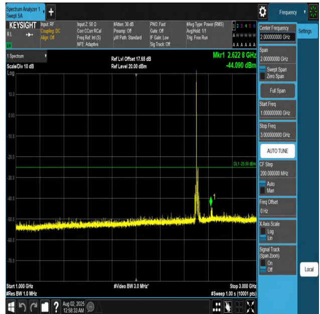
Band7-15MHz-QPSK-20825-1RB#0-1000~3000-PASS
