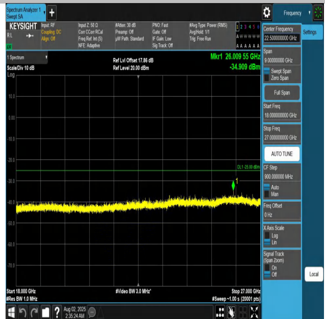
Band7-20MHz-QPSK-21100-1RB#0-18000~27000-PASS
