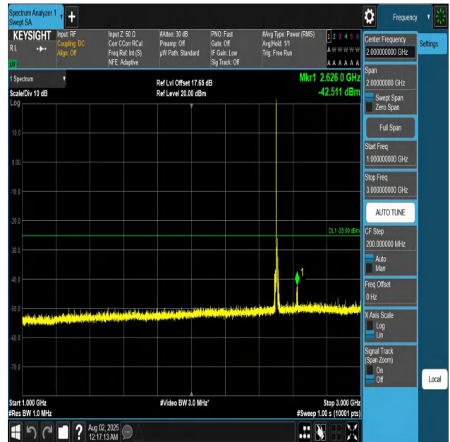
Band7-10MHz-QPSK-20800-1RB#0-1000~3000-PASS
