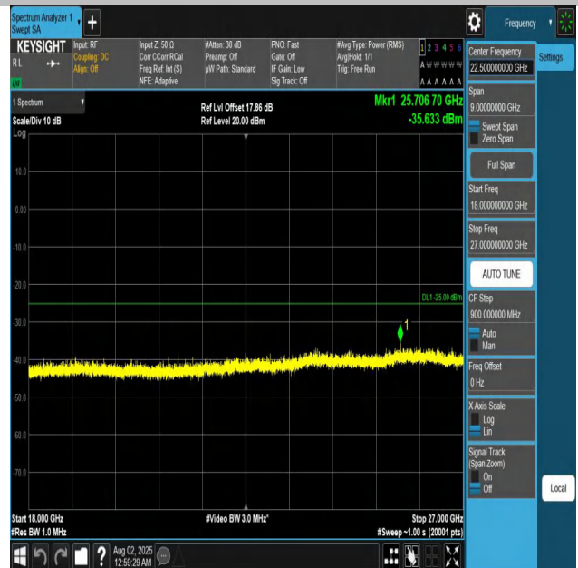
Band7-15MHz-QPSK-21100-1RB#0-18000~27000-PASS
