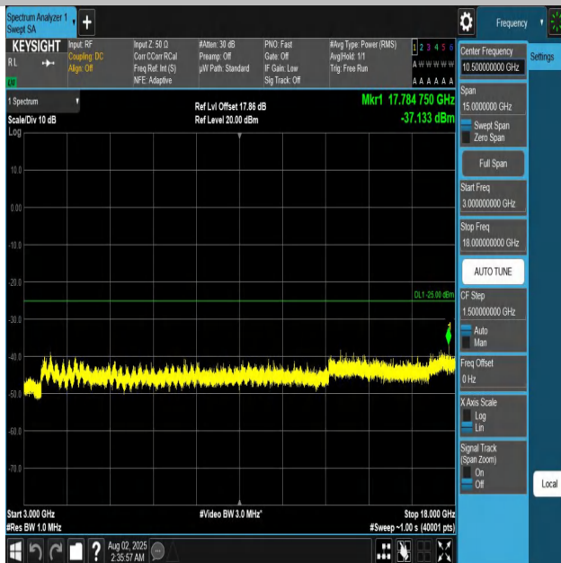
Band7-20MHz-QPSK-21350-1RB#0-3000~18000-PASS
