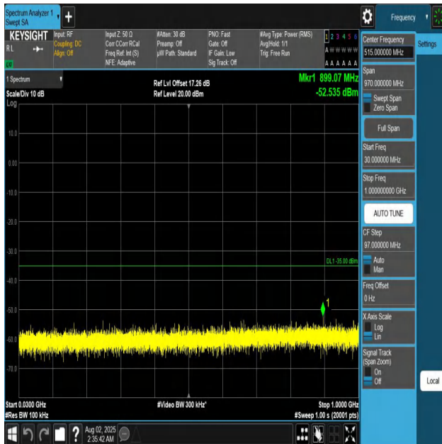
Band7-20MHz-QPSK-21350-1RB#0-30~1000-PASS
