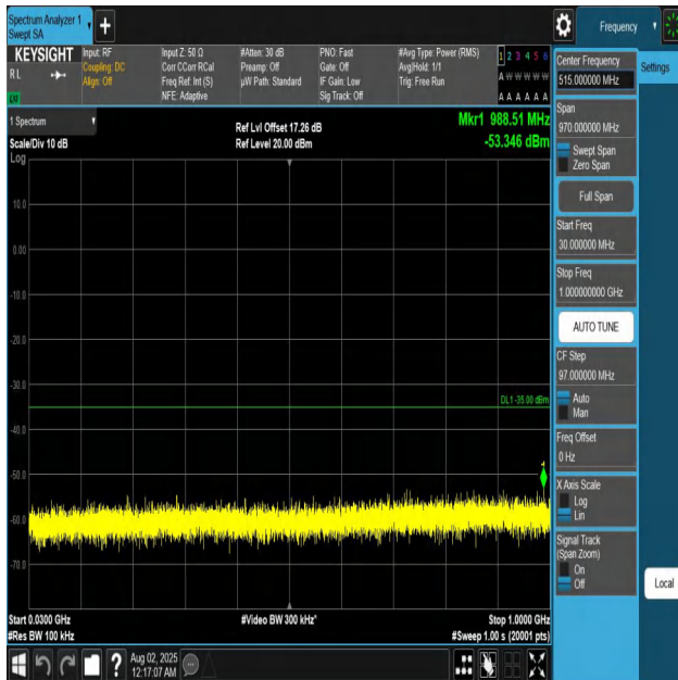
Band7-10MHz-QPSK-20800-1RB#0-30~1000-PASS
