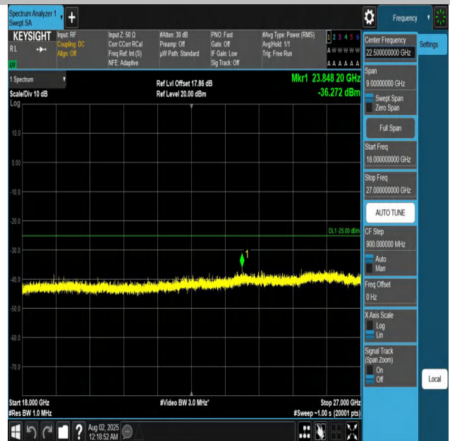
Band7-10MHz-QPSK-21400-1RB#0-18000~27000-PASS
