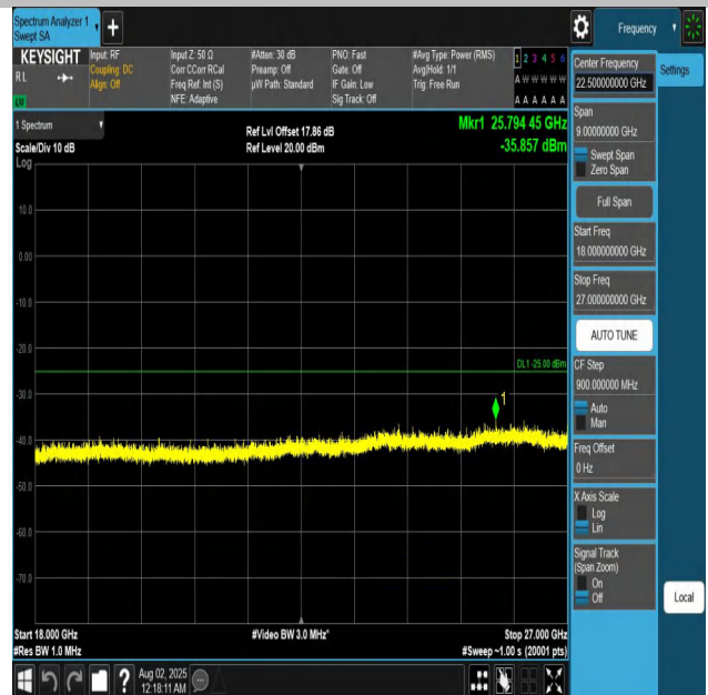
Band7-10MHz-QPSK-21100-1RB#0-18000~27000-PASS
