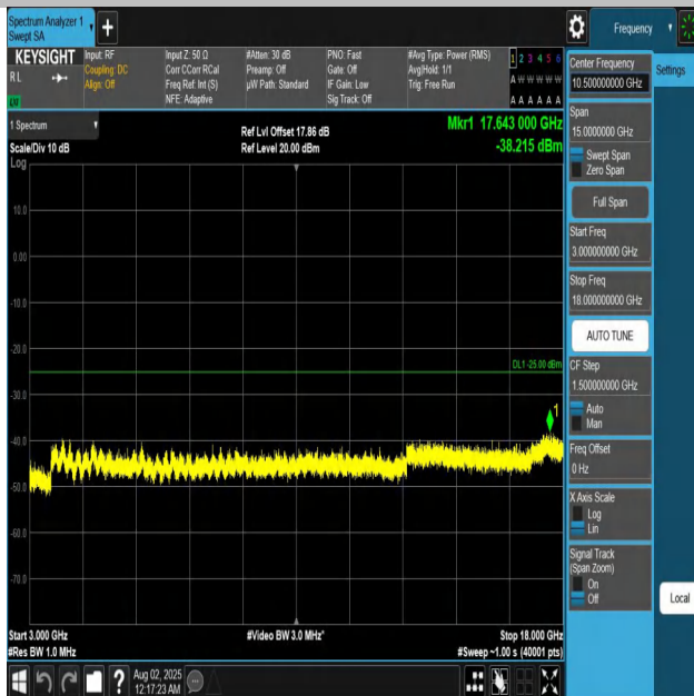
Band7-10MHz-QPSK-20800-1RB#0-3000~18000-PASS
