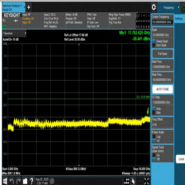
Band7-20MHz-QPSK-21100-1RB#0-3000~18000-PASS
