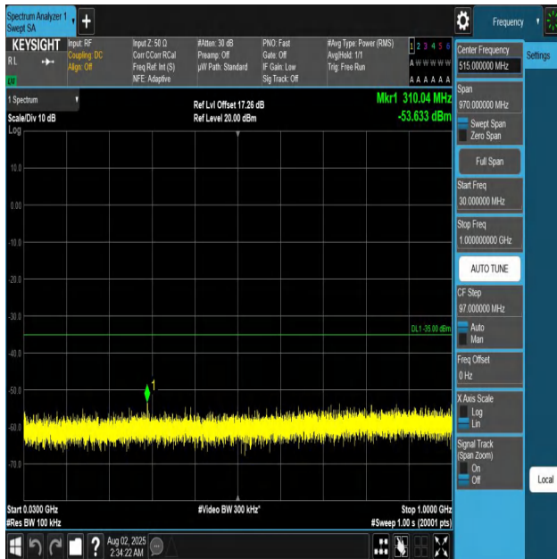
Band7-20MHz-QPSK-20850-1RB#0-30~1000-PASS
