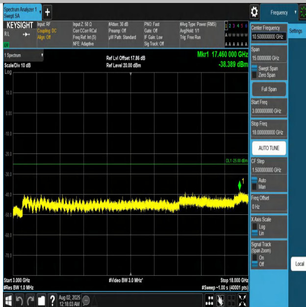
Band7-10MHz-QPSK-21100-1RB#0-3000~18000-PASS
