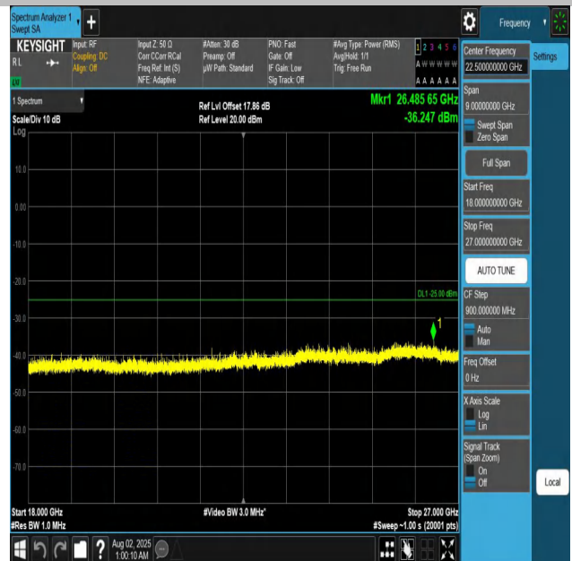
Band7-15MHz-QPSK-21375-1RB#0-18000~27000-PASS
