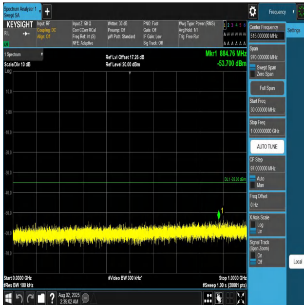
Band7-20MHz-QPSK-21100-1RB#0-30~1000-PASS
