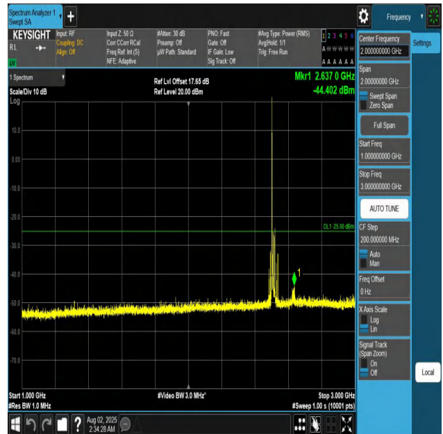
Band7-20MHz-QPSK-20850-1RB#0-1000~3000-PASS
