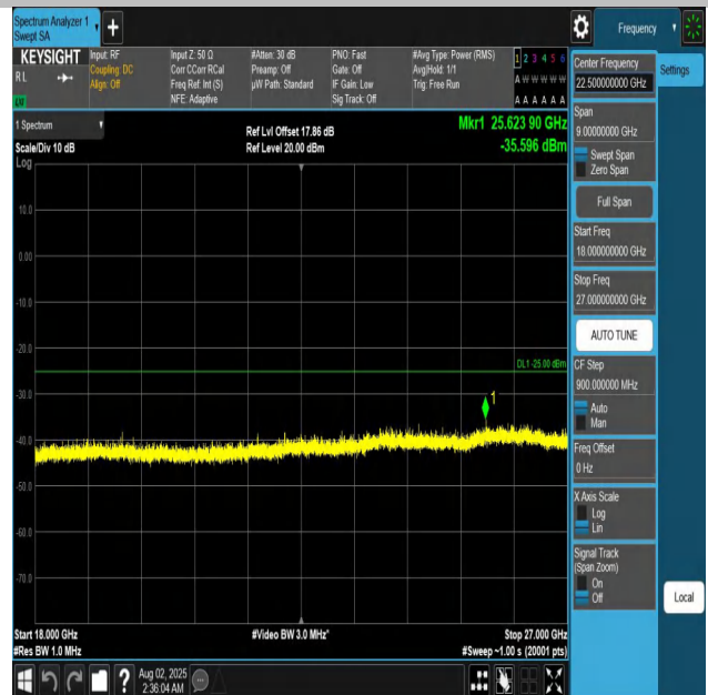
Band7-20MHz-QPSK-21350-1RB#0-18000~27000-PASS
