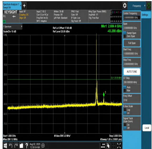
Band7-15MHz-QPSK-21375-1RB#0-1000~3000-PASS
