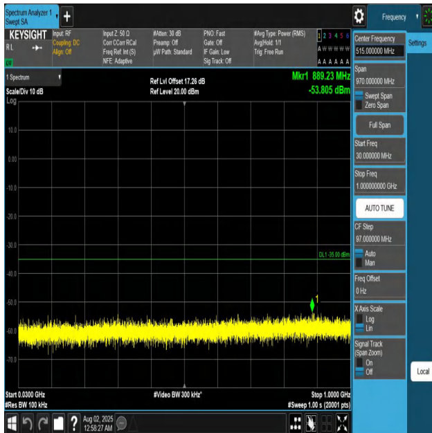
Band7-15MHz-QPSK-20825-1RB#0-30~1000-PASS
