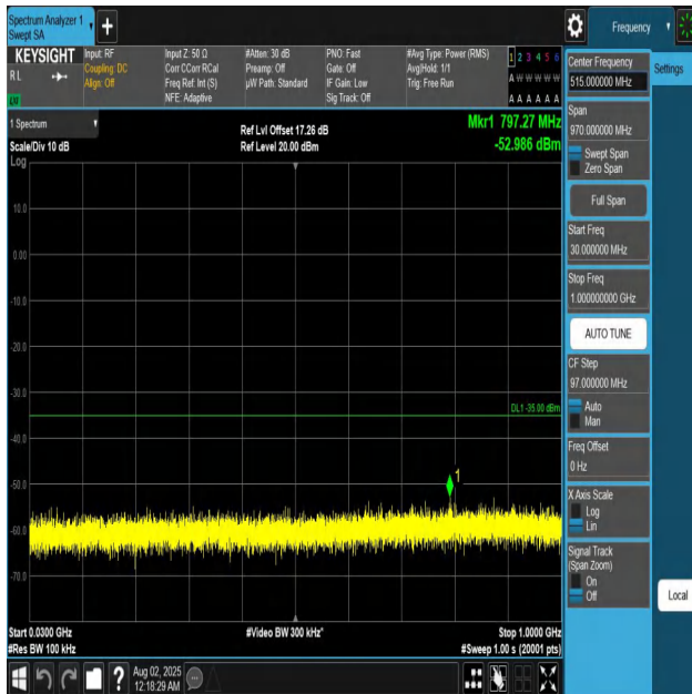
Band7-10MHz-QPSK-21400-1RB#0-30~1000-PASS
