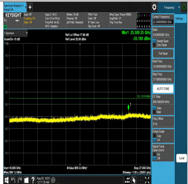
Band7-10MHz-QPSK-20800-1RB#0-18000~27000-PASS
