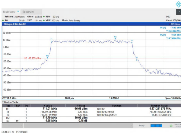
NTNV-n12-PC3-15-5-H-DFT-256QAM-Outer_Full-Ant1-PASS
