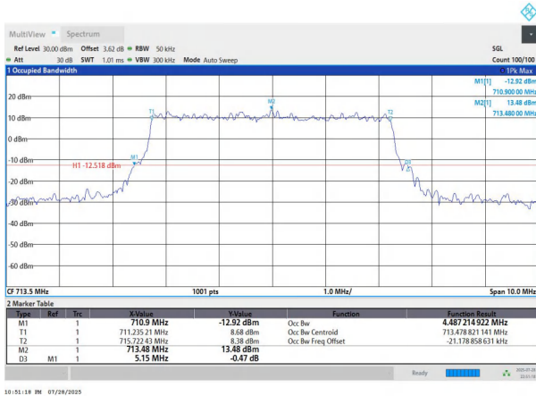
NTNV-n12-PC3-15-5-H-DFT-16QAM-Outer_Full-Ant1-PASS
