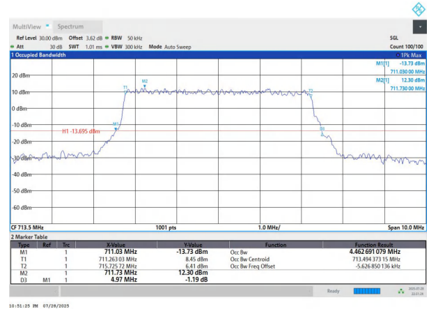
NTNV-n12-PC3-15-5-H-DFT-64QAM-Outer_Full-Ant1-PASS
