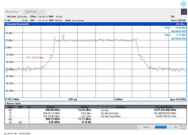
NTNV-n12-PC3-15-5-L-DFT-64QAM-Outer_Full-Ant1-PASS
