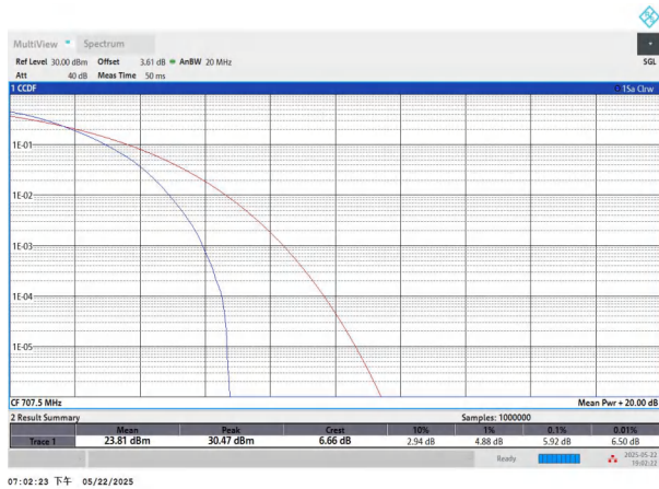
NTNV-n12-PC3-15-15-M-DFT-64QAM-Outer_Full-PASS
