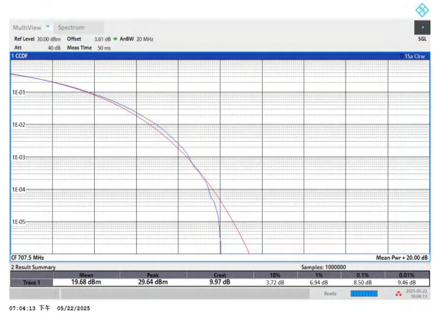
NTNV-n12-PC3-15-15-M-CP-256QAM-Outer_Full-PASS
