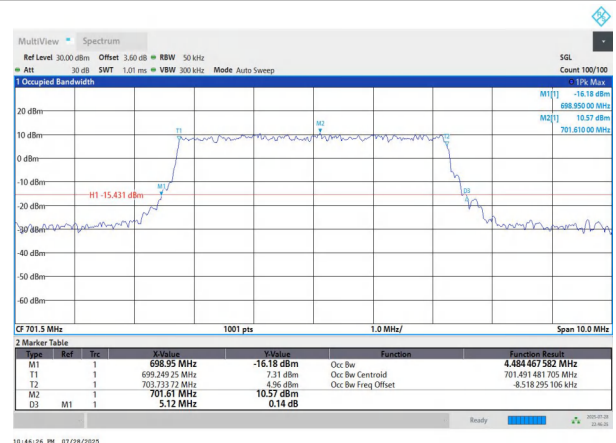
NTNV-n12-PC3-15-5-L-CP-QPSK-Outer_Full-Ant1-PASS
