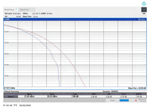
NTNV-n12-PC3-15-15-M-DFT-256QAM-Outer_Full-PASS
