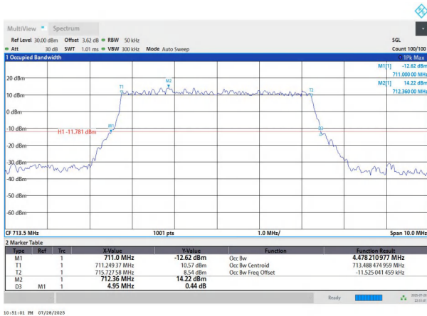
NTNV-n12-PC3-15-5-H-DFT-BPSK-Outer_Full-Ant1-PASS
