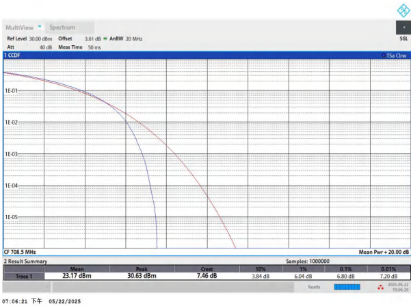
NTNV-n12-PC3-15-15-H-CP-16QAM-Outer_Full-PASS
