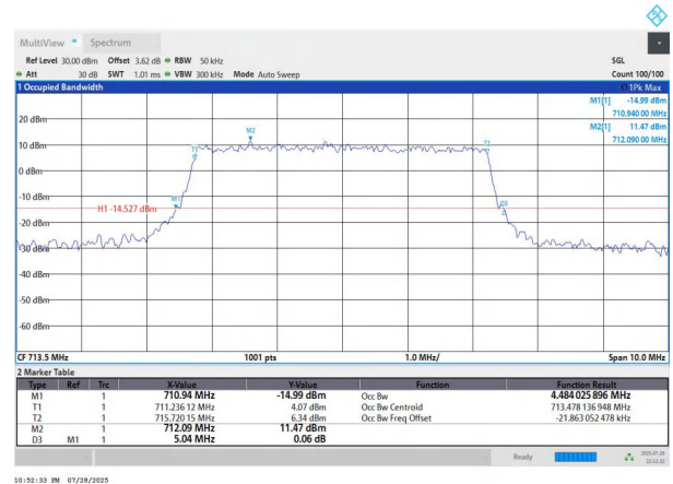
NTNV-n12-PC3-15-5-H-CP-QPSK-Outer_Full-Ant1-PASS
