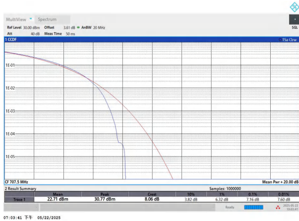
NTNV-n12-PC3-15-15-M-CP-64QAM-Outer_Full-PASS
