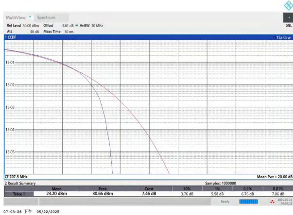
NTNV-n12-PC3-15-15-M-CP-QPSK-Outer_Full-PASS
