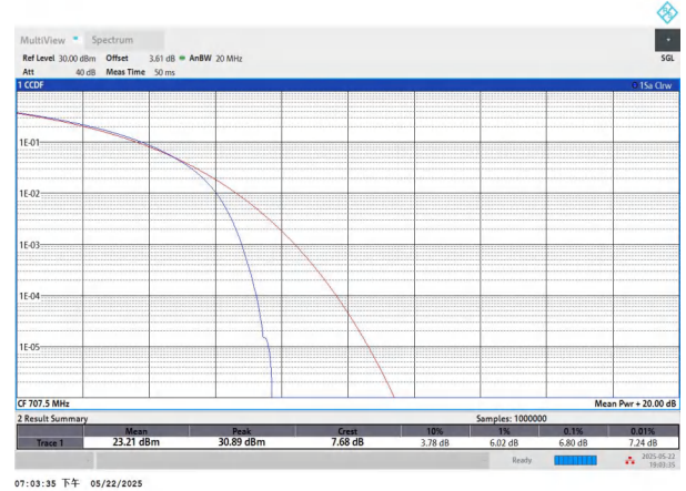
NTNV-n12-PC3-15-15-M-CP-16QAM-Outer_Full-PASS
