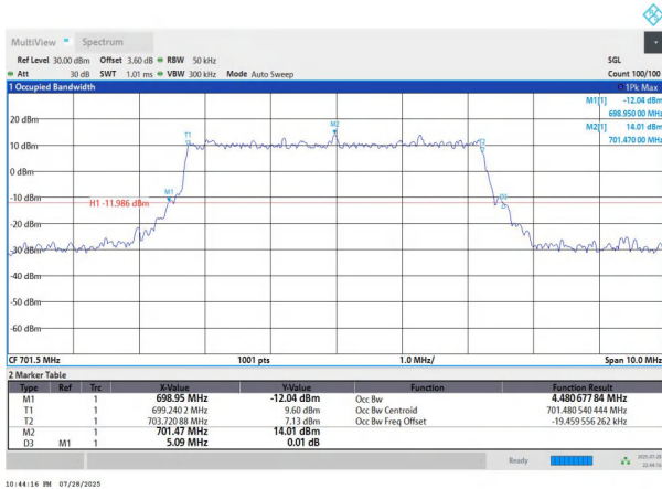
NTNV-n12-PC3-15-5-L-DFT-16QAM-Outer_Full-Ant1-PASS
