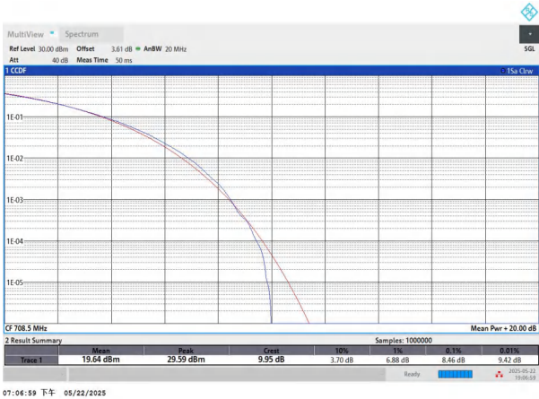
NTNV-n12-PC3-15-15-H-CP-256QAM-Outer_Full-PASS
