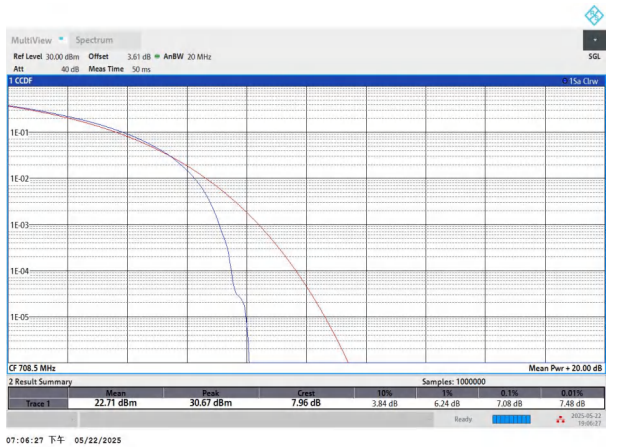
NTNV-n12-PC3-15-15-H-CP-64QAM-Outer_Full-PASS
