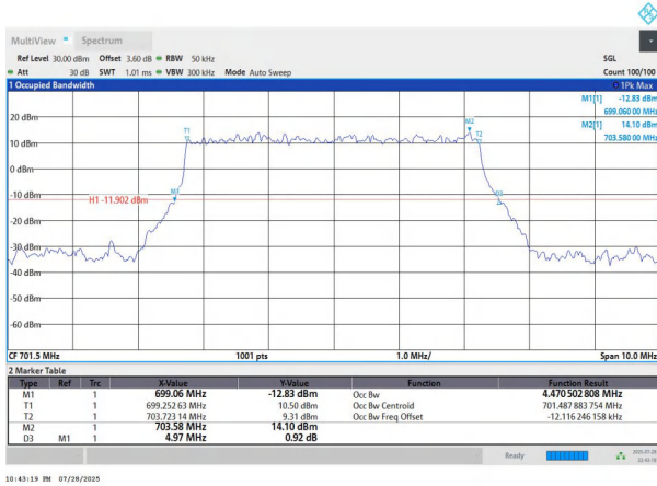
NTNV-n12-PC3-15-5-L-DFT-BPSK-Outer_Full-Ant1-PASS
