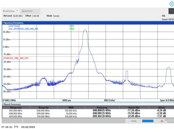
NTNV-n12-PC3-15-5-L-DFT-QPSK-Edge_1RB_Left-PASS
