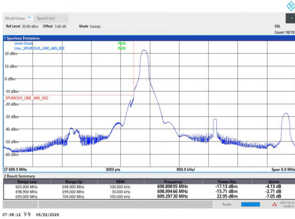
NTNV-n12-PC3-15-5-L-DFT-BPSK-Edge_1RB_Left-PASS
