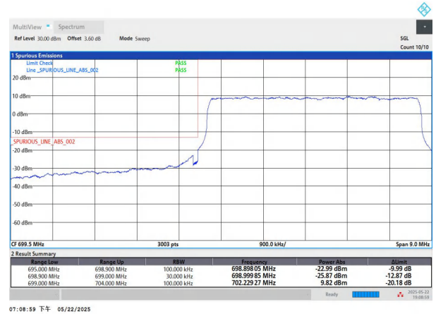
NTNV-n12-PC3-15-5-L-DFT-QPSK-Outer_Full-PASS
