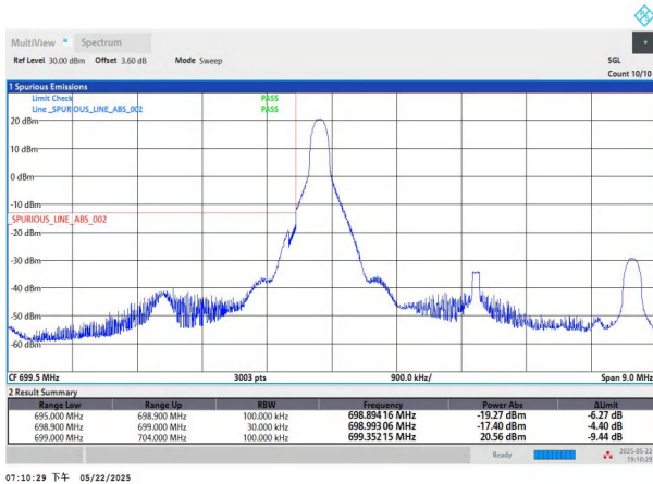
NTNV-n12-PC3-15-5-L-CP-QPSK-Edge_1RB_Left-PASS
