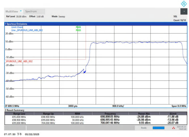
NTNV-n12-PC3-15-5-L-DFT-BPSK-Outer_Full-PASS
