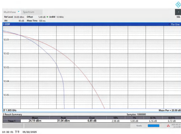
NTNV-n2-PC3-15-10-H-DFT-64QAM-Outer_Full-PASS
