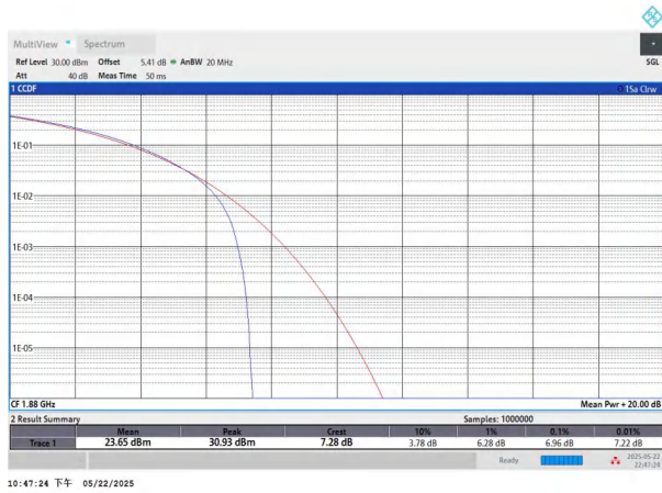
NTNV-n2-PC3-15-20-M-CP-16QAM-Outer_Full-PASS
