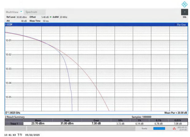
NTNV-n2-PC3-15-15-H-CP-QPSK-Outer_Full-PASS
