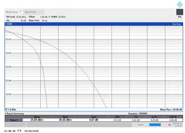
NTNV-n2-PC3-15-20-H-DFT-BPSK-Outer_Full-PASS
