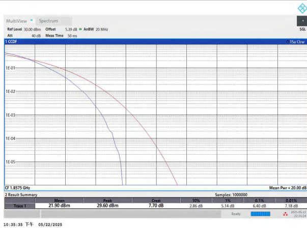
NTNV-n2-PC3-15-15-L-DFT-256QAM-Outer_Full-PASS
