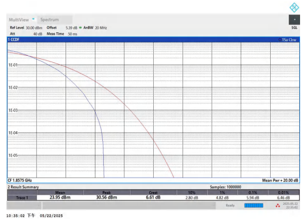
NTNV-n2-PC3-15-15-L-DFT-64QAM-Outer_Full-PASS
