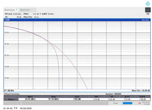
NTNV-n2-PC3-15-15-M-CP-16QAM-Outer_Full-PASS
