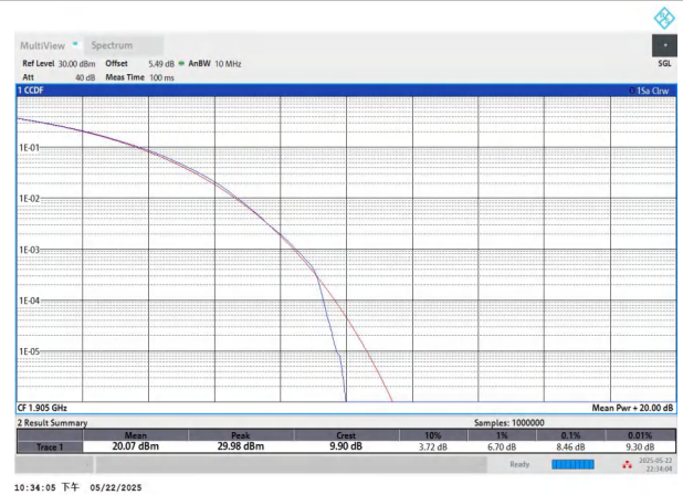
NTNV-n2-PC3-15-10-H-CP-256QAM-Outer_Full-PASS
