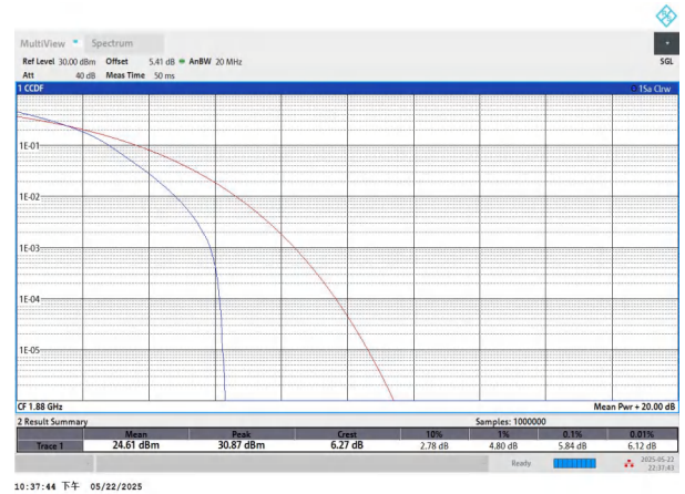
NTNV-n2-PC3-15-15-M-DFT-16QAM-Outer_Full-PASS
