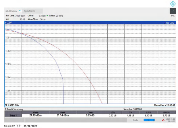
NTNV-n2-PC3-15-15-H-DFT-64QAM-Outer_Full-PASS
