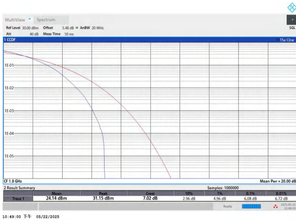
NTNV-n2-PC3-15-20-H-DFT-64QAM-Outer_Full-PASS
