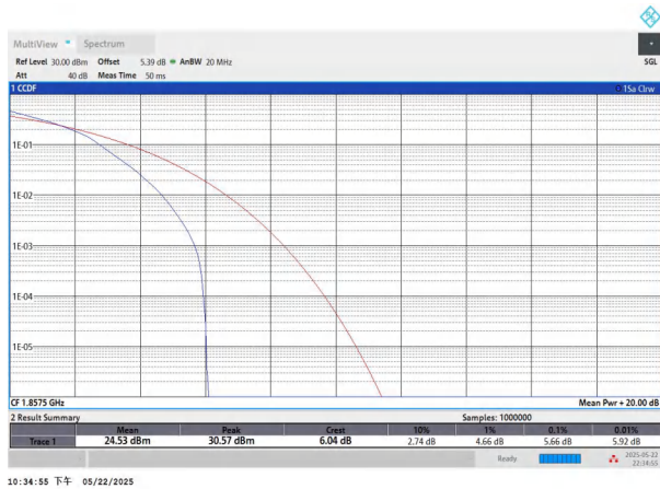
NTNV-n2-PC3-15-15-L-DFT-16QAM-Outer_Full-PASS
