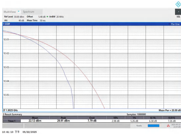
NTNV-n2-PC3-15-15-H-DFT-256QAM-Outer_Full-PASS
