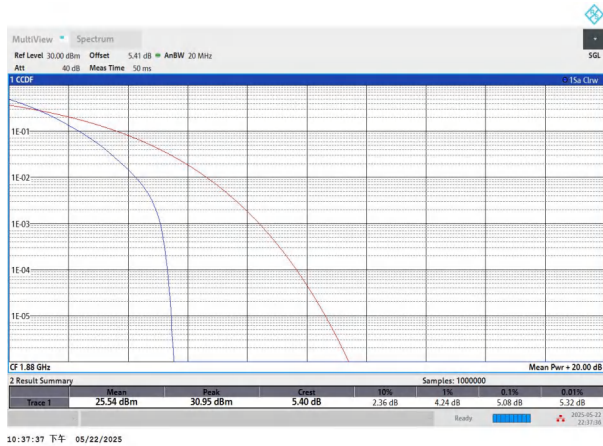
NTNV-n2-PC3-15-15-M-DFT-QPSK-Outer_Full-PASS
