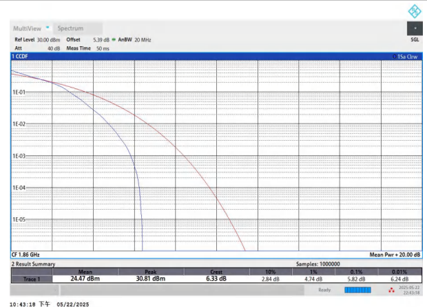
NTNV-n2-PC3-15-20-L-DFT-16QAM-Outer_Full-PASS
