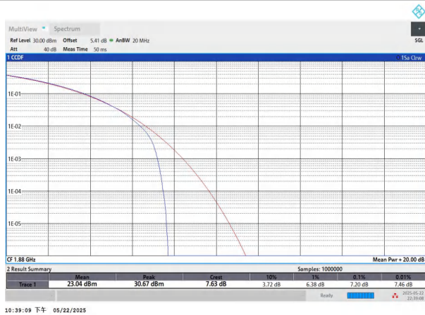
NTNV-n2-PC3-15-15-M-CP-64QAM-Outer_Full-PASS
