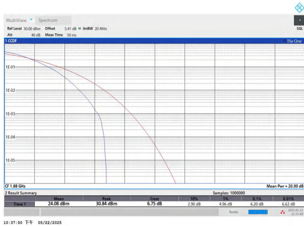
NTNV-n2-PC3-15-15-M-DFT-64QAM-Outer_Full-PASS
