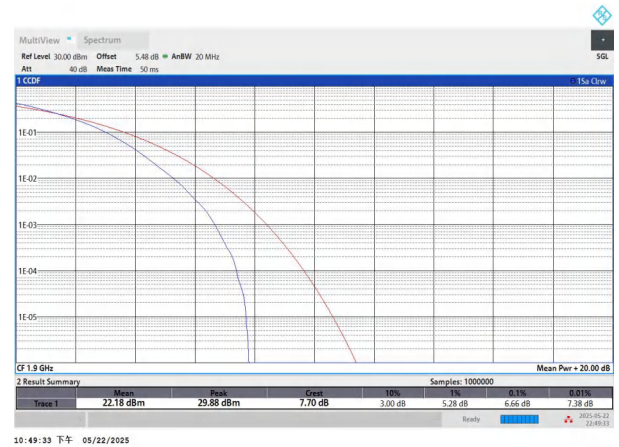
NTNV-n2-PC3-15-20-H-DFT-256QAM-Outer_Full-PASS
