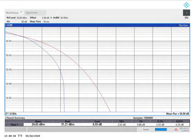
NTNV-n2-PC3-15-20-H-DFT-16QAM-Outer_Full-PASS
