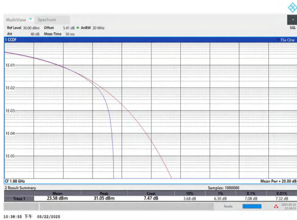
NTNV-n2-PC3-15-15-M-CP-QPSK-Outer_Full-PASS
