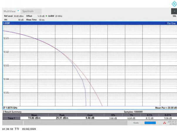
NTNV-n2-PC3-15-15-L-CP-256QAM-Outer_Full-PASS
