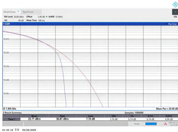
NTNV-n2-PC3-15-10-H-CP-QPSK-Outer_Full-PASS
