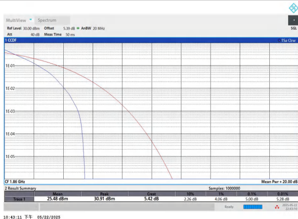
NTNV-n2-PC3-15-20-L-DFT-QPSK-Outer_Full-PASS
