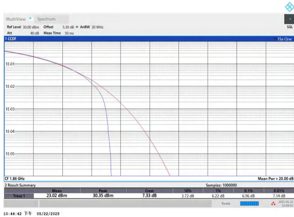
NTNV-n2-PC3-15-20-L-CP-64QAM-Outer_Full-PASS
