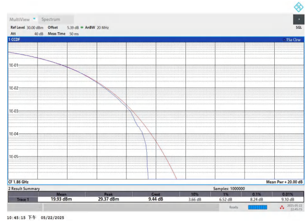
NTNV-n2-PC3-15-20-L-CP-256QAM-Outer_Full-PASS
