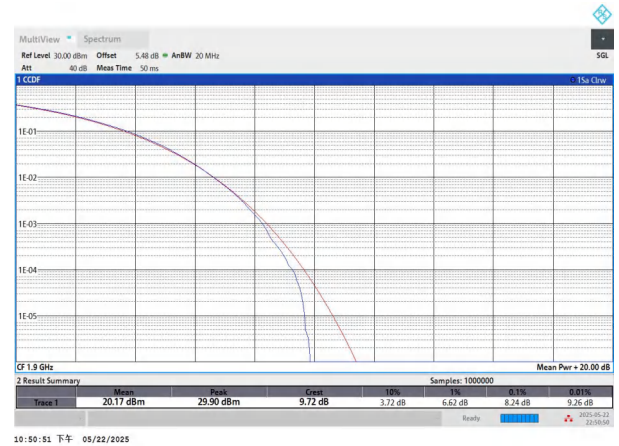
NTNV-n2-PC3-15-20-H-CP-256QAM-Outer_Full-PASS
