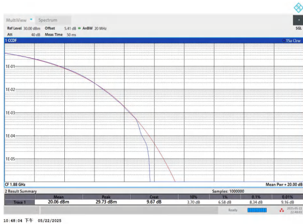
NTNV-n2-PC3-15-20-M-CP-256QAM-Outer_Full-PASS
