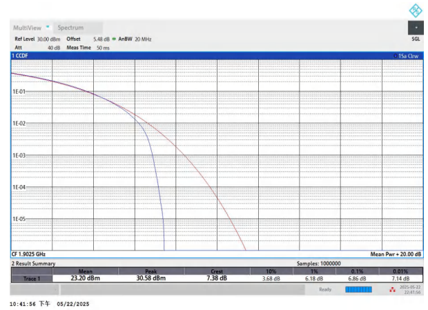
NTNV-n2-PC3-15-15-H-CP-64QAM-Outer_Full-PASS
