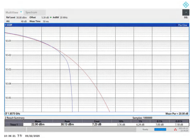
NTNV-n2-PC3-15-15-L-CP-64QAM-Outer_Full-PASS
