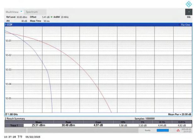
NTNV-n2-PC3-15-15-M-DFT-BPSK-Outer_Full-PASS
