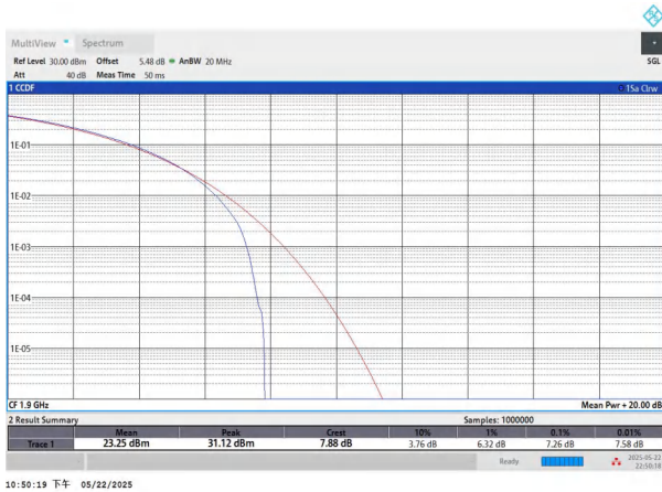
NTNV-n2-PC3-15-20-H-CP-64QAM-Outer_Full-PASS
