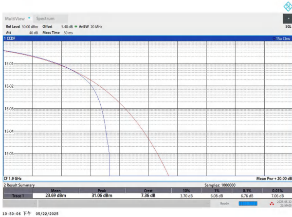
NTNV-n2-PC3-15-20-H-CP-QPSK-Outer_Full-PASS
