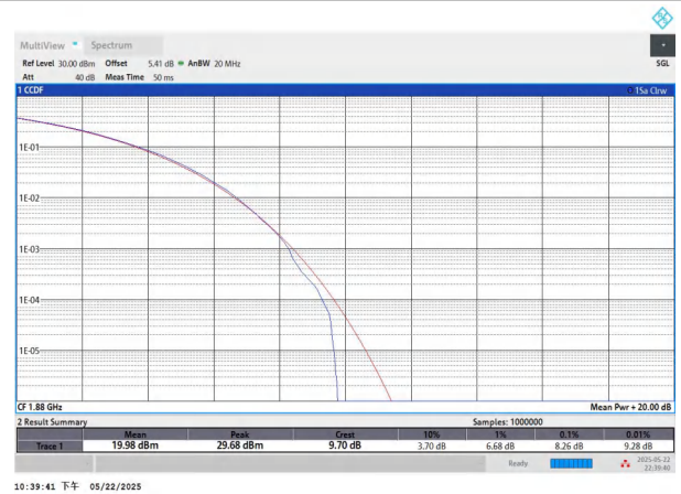
NTNV-n2-PC3-15-15-M-CP-256QAM-Outer_Full-PASS
