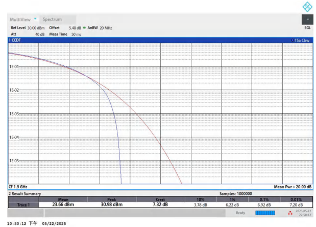
NTNV-n2-PC3-15-20-H-CP-16QAM-Outer_Full-PASS
