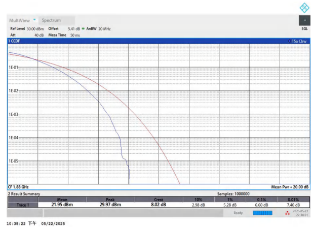
NTNV-n2-PC3-15-15-M-DFT-256QAM-Outer_Full-PASS
