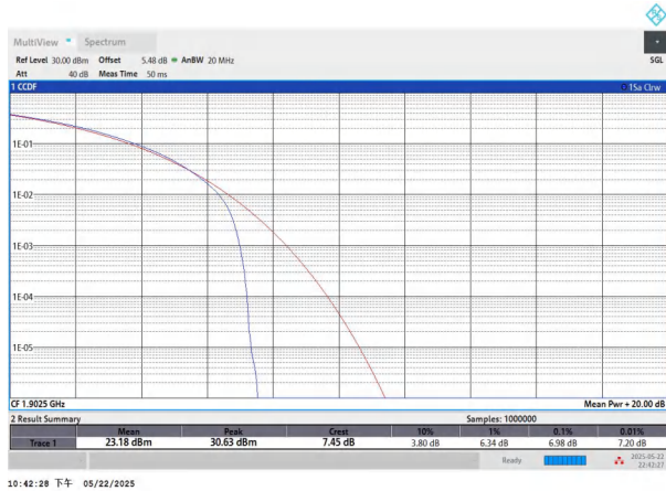
NTNV-n2-PC3-15-15-H-CP-256QAM-Outer_Full-PASS
