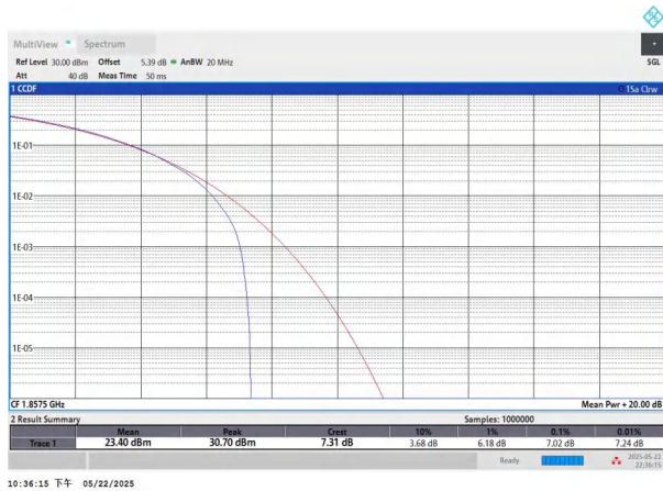
NTNV-n2-PC3-15-15-L-CP-16QAM-Outer_Full-PASS
