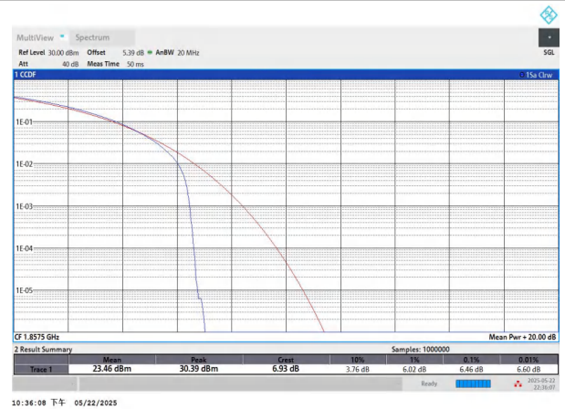
NTNV-n2-PC3-15-15-L-CP-QPSK-Outer_Full-PASS
