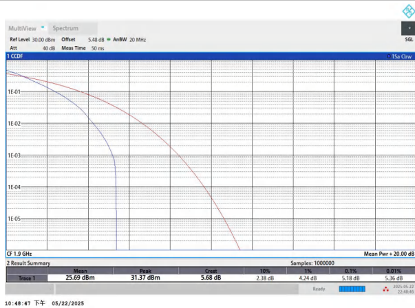
NTNV-n2-PC3-15-20-H-DFT-QPSK-Outer_Full-PASS
