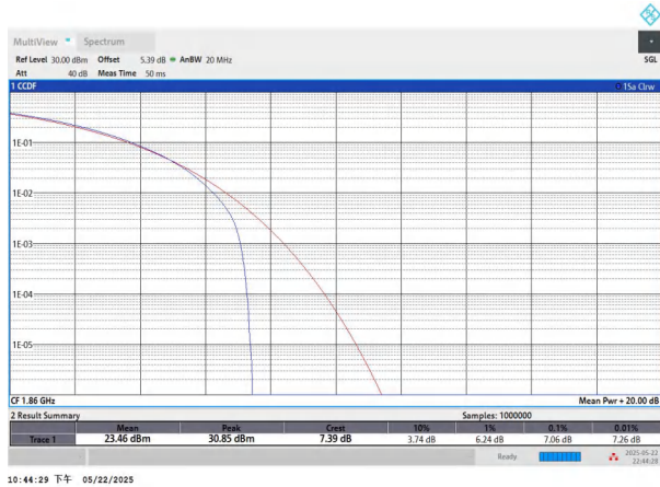
NTNV-n2-PC3-15-20-L-CP-QPSK-Outer_Full-PASS
