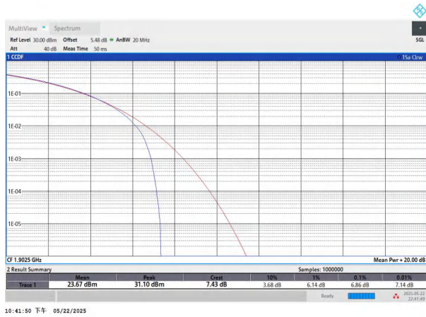
NTNV-n2-PC3-15-15-H-CP-16QAM-Outer_Full-PASS
