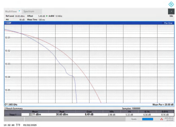
NTNV-n2-PC3-15-10-H-DFT-256QAM-Outer_Full-PASS
