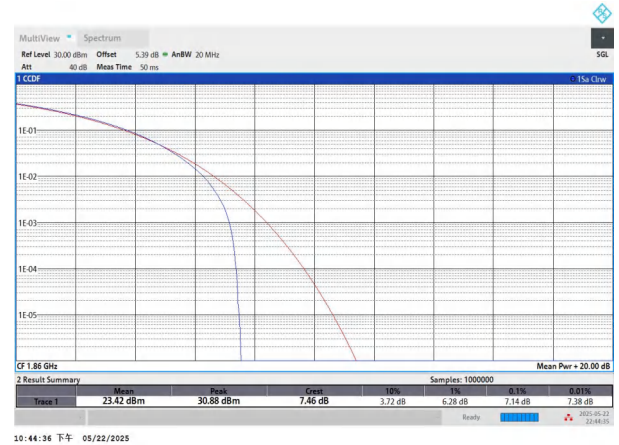
NTNV-n2-PC3-15-20-L-CP-16QAM-Outer_Full-PASS
