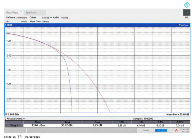
NTNV-n2-PC3-15-10-H-CP-16QAM-Outer_Full-PASS
