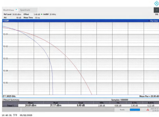
NTNV-n2-PC3-15-15-H-DFT-16QAM-Outer_Full-PASS
