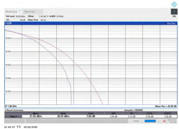
NTNV-n2-PC3-15-20-L-DFT-256QAM-Outer_Full-PASS
