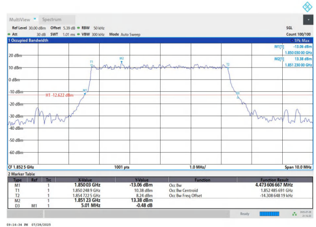
NTNV-n2-PC3-15-5-L-DFT-64QAM-Outer_Full-Ant1-PASS
