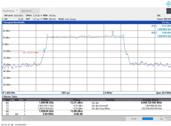
NTNV-n2-PC3-15-10-L-DFT-16QAM-Outer_Full-Ant1-PASS
