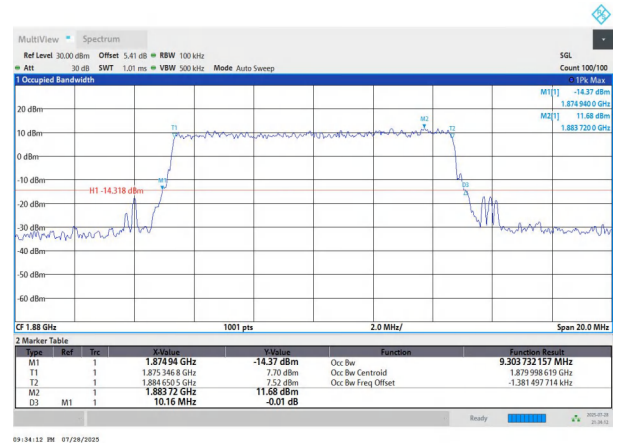
NTNV-n2-PC3-15-10-M-CP-QPSK-Outer_Full-Ant1-PASS
