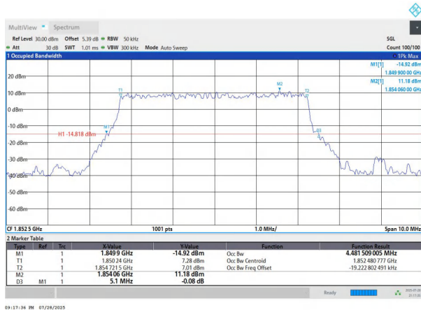
NTNV-n2-PC3-15-5-L-DFT-256QAM-Outer_Full-Ant1-PASS
