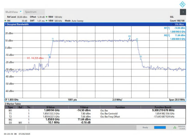
NTNV-n2-PC3-15-10-L-CP-QPSK-Outer_Full-Ant1-PASS
