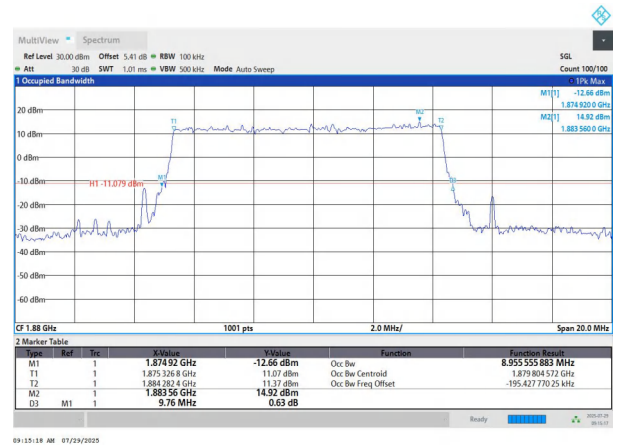
NTNV-n2-PC3-15-10-M-DFT-QPSK-Outer_Full-Ant1-PASS
