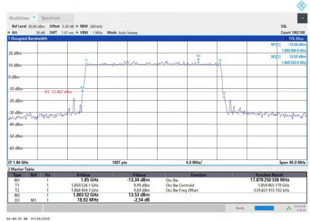
NTNV-n2-PC3-15-20-L-DFT-64QAM-Outet_Full-Ant1-PASS
