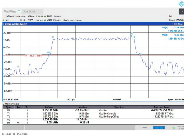
NTNV-n2-PC3-15-5-L-DFT-BPSK-Outer_Full-Ant1-PASS
