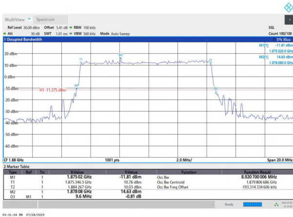
NTNV-n2-PC3-15-10-M-DFT-BPSK-Outer_Full-Ant1-PASS
