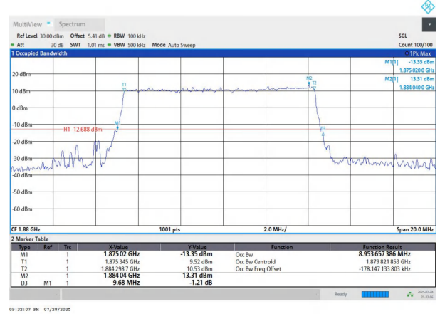
NTNV-n2-PC3-15-10-M-DFT-64QAM-Outer_Full-Ant1-PASS
