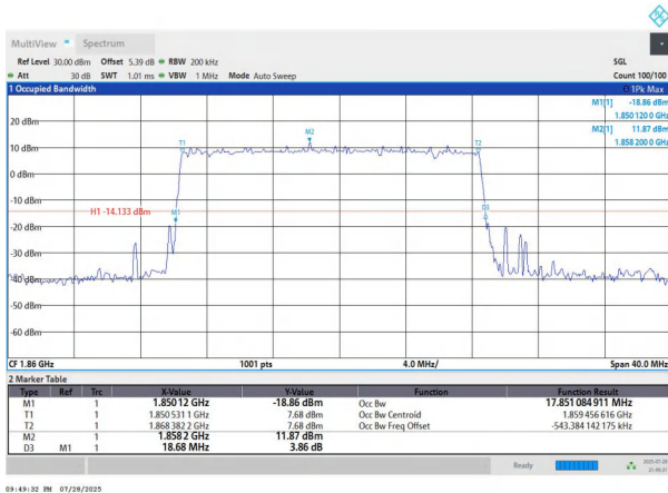
NTNV-n2-PC3-15-20-L-DFT-256QAM-Outet_Full-Ant1-PASS
