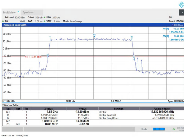
NTNV-n2-PC3-15-20-L-DFT-BPSK-Outet_Full-Ant1-PASS
