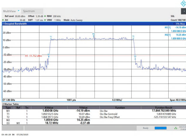
NTNV-n2-PC3-15-20-L-DFT-16QAM-Outet_Full-Ant1-PASS
