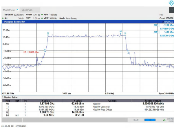
NTNV-n2-PC3-15-10-M-DFT-16QAM-Outer_Full-Ant1-PASS
