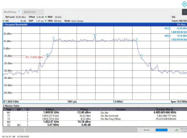
NTNV-n2-PC3-15-5-L-DFT-16QAM-Outer_Full-Ant1-PASS
