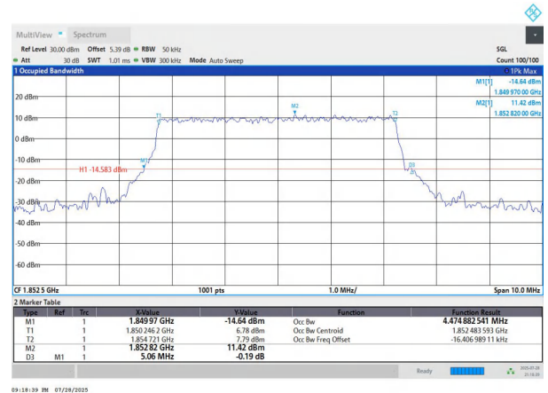
NTNV-n2-PC3-15-5-L-CP-QPSK-Outer_Full-Ant1-PASS
