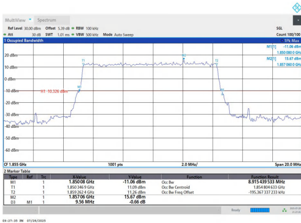
NTNV-n2-PC3-15-10-L-DFT-BPSK-Outer_Full-Ant1-PASS
