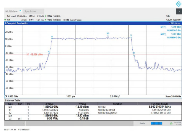
NTNV-n2-PC3-15-10-L-DFT-64QAM-Outer_Full-Ant1-PASS
