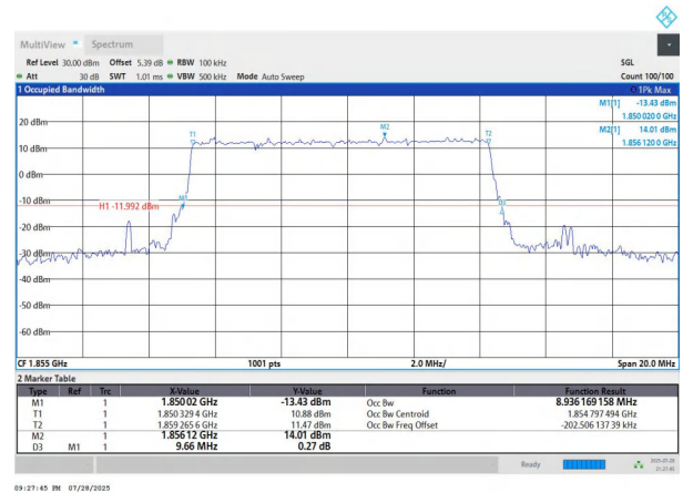
NTNV-n2-PC3-15-10-L-DFT-QPSK-Outer_Full-Ant1-PASS
