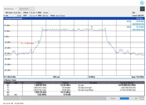
NTNV-n2-PC3-15-5-L-DFT-QPSK-Outer_Full-Ant1-PASS
