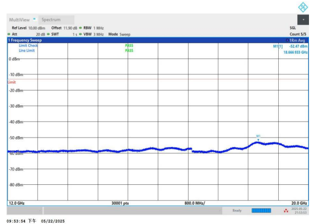
NTNV-n2-PC3-15-15-L-DFT-QPSK-Edge_1RB_Left-12000-20000- PASS
