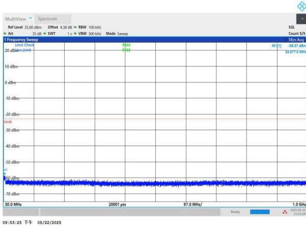
NTNV-n2-PC3-15-15-L-DFT-QPSK-Edge_1RB_Left-30-1000-PA SS
