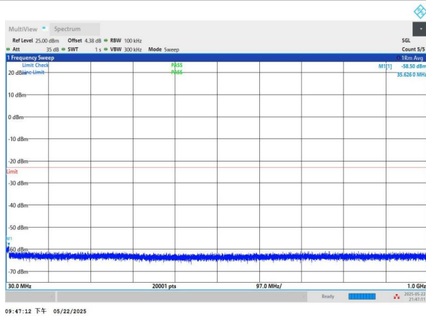
NTNV-n2-PC3-15-10-M-CP-QPSK-Edge_1RB_Left-30-1000-PASS
