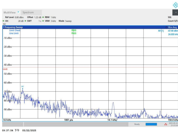
NTNV-n2-PC3-15-5-H-DFT-QPSK-Edge_1RB_Left-0.009-0.15-P ASS
