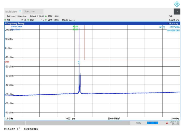
NTNV-n2-PC3-15-15-L-CP-QPSK-Edge_1RB_Left-1000-3000-PASS
