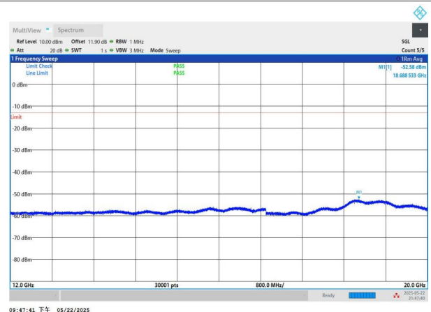
NTNV-n2-PC3-15-10-M-CP-QPSK-Edge_1RB_Left-12000-20000-PASS
