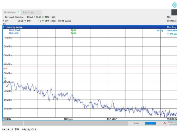
NTNV-n2-PC3-15-5-H-CP-QPSK-Edge_1RB_Left-0.009-0.15-PA SS
