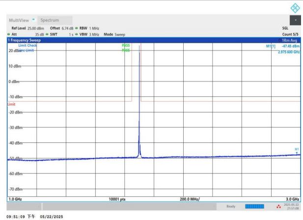
NTNV-n2-PC3-15-10-H-CP-QPSK-Edge_1RB_Left-1000-3000-PASS
