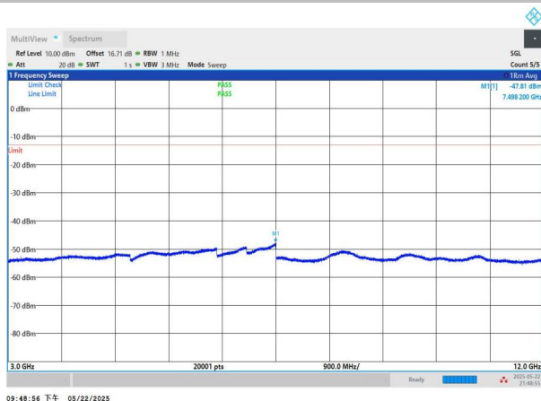
NTNV-n2-PC3-15-10-H-DFT-BPSK-Edge_1RB_Left-3000-12000-
