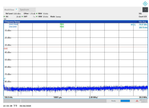
NTNV-n2-PC3-15-15-H-CP-QPSK-Edge_1RB_Left-0.15-30-PASS
