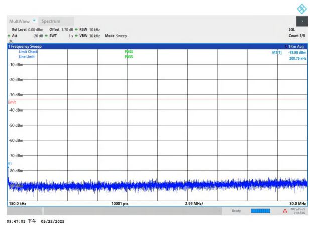
NTNV-n2-PC3-15-10-M-CP-QPSK-Edge_1RB_Left-0.15-30-PASS
