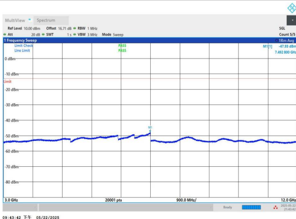
NTNV-n2-PC3-15-10-L-CP-QPSK-Edge_1RB_Left-3000-12000-P ASS
