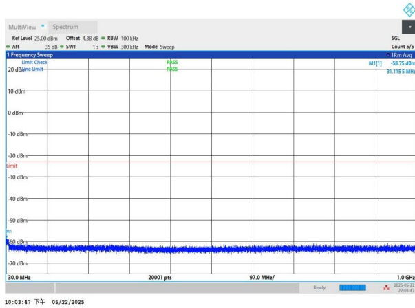
NTNV-n2-PC3-15-15-H-CP-QPSK-Edge_1RB_Left-30-1000-PAS S
