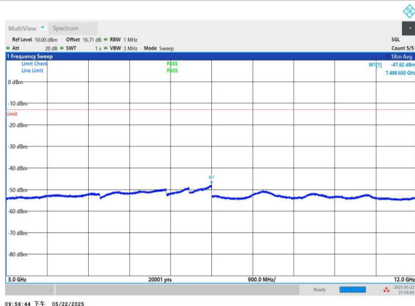
NTNV-n2-PC3-15-15-M-DFT-BPSK-Edge_1RB_Left-3000-12000-PASS
