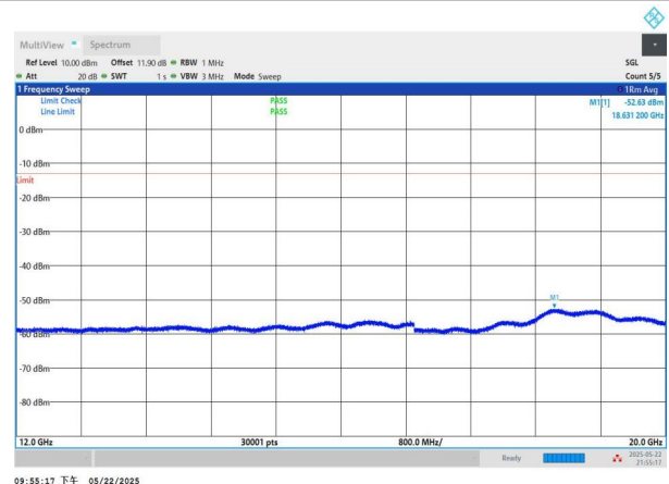
NTNV-n2-PC3-15-15-L-CP-QPSK-Edge_1RB_Left-12000-20000-P ASS
