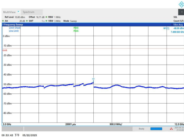
NTNV-n2-PC3-15-15-L-DFT-QPSK-Edge_1RB_Left-3000-12000- PASS
