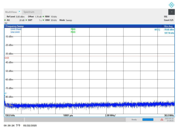
NTNV-n2-PC3-15-5-H-CP-QPSK-Edge_1RB_Left-0.15-30-PASS
