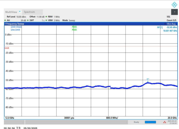
NTNV-n2-PC3-15-15-M-DFT-BPSK-Edge_1RB_Left-12000-20000-PASS
