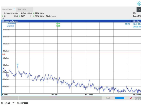
NTNV-n2-PC3-15-10-H-DFT-QPSK-Edge_1RB_Left-0.009-0.15-PASS
