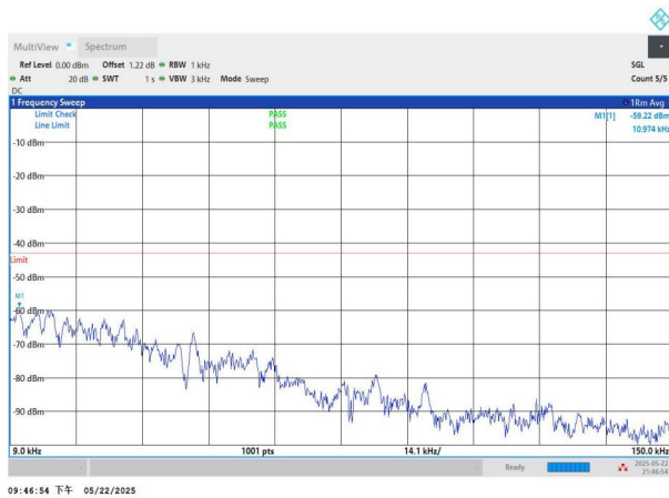
NTNV-n2-PC3-15-10-M-CP-QPSK-Edge_1RB_Left-0.009-0.15-PASS
