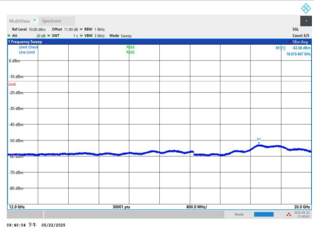
NTNV-n2-PC3-15-5-H-CP-QPSK-Edge_1RB_Left-12000-20000-P ASS
