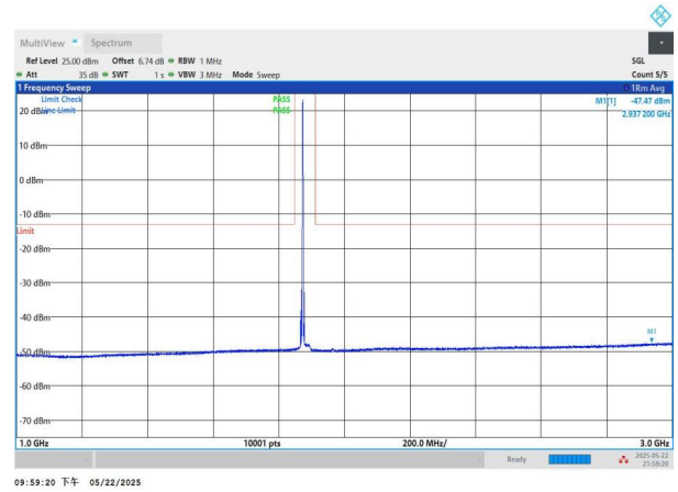
NTNV-n2-PC3-15-15-M-CP-QPSK-Edge_1RB_Left-1000-3000-PASS
