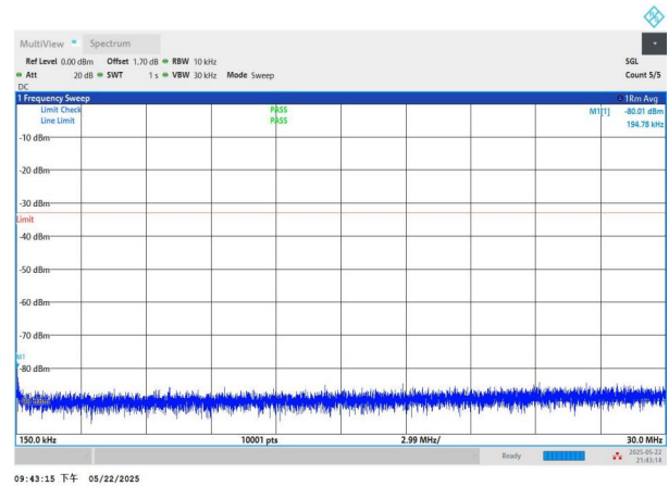
NTNV-n2-PC3-15-10-L-CP-QPSK-Edge_1RB_Left-0.15-30-PASS
