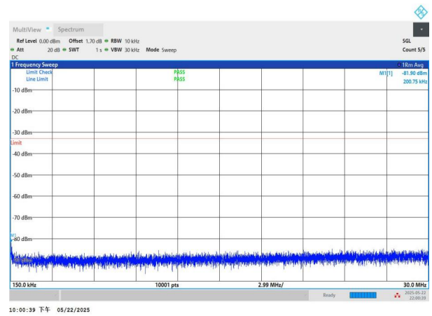
NTNV-n2-PC3-15-15-H-DFT-BPSK-Edge_1RB_Left-0.15-30-PAS
