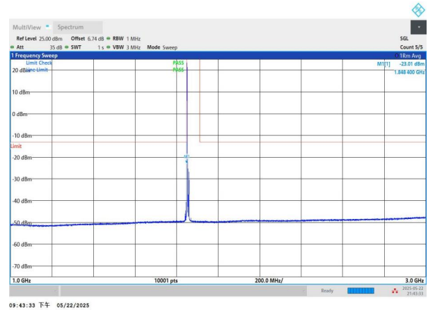
NTNV-n2-PC3-15-10-L-CP-QPSK-Edge_1RB_Left-1000-3000-PA SS
