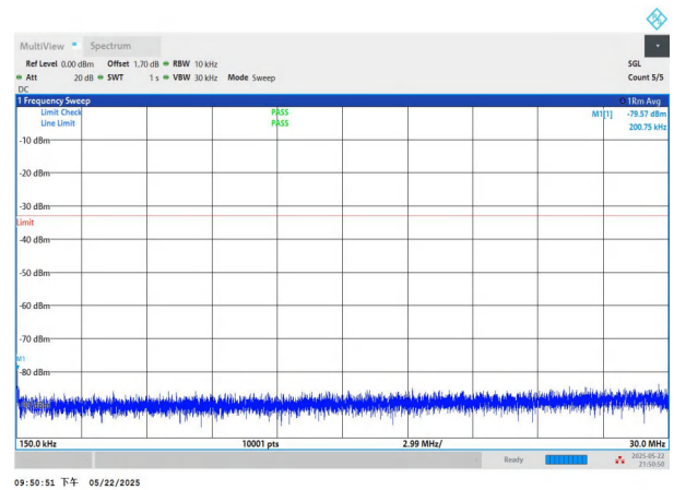
NTNV-n2-PC3-15-10-H-CP-QPSK-Edge_1RB_Left-0.15-30-PASS
