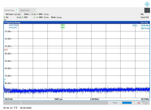
NTNV-n2-PC3-15-15-L-DFT-BPSK-Edge_1RB_Left-0.15-30-PASS
