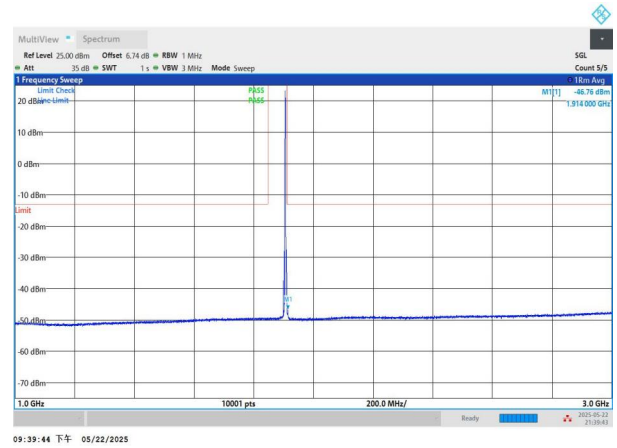
NTNV-n2-PC3-15-5-H-CP-QPSK-Edge_1RB_Left-1000-3000-PASS S
