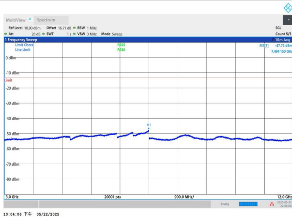
NTNV-n2-PC3-15-15-H-CP-QPSK-Edge_1RB_Left-3000-12000- PASS
