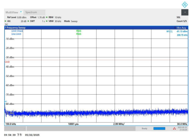
NTNV-n2-PC3-15-15-L-CP-QPSK-Edge_1RB_Left-0.15-30-PASS
