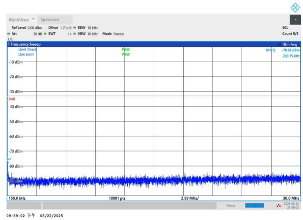
NTNV-n2-PC3-15-15-M-CP-QPSK-Edge_1RB_Left-0.15-30-PASS
