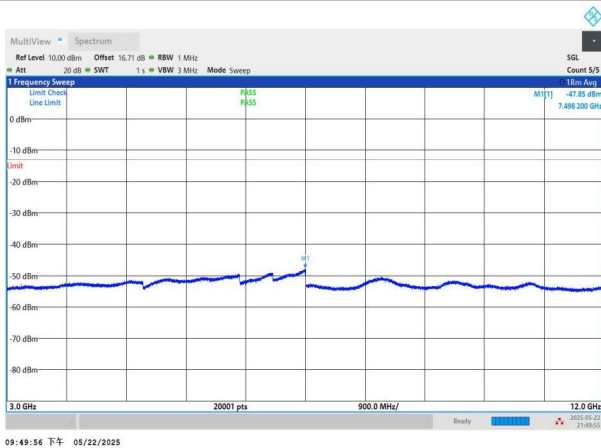
NTNV-n2-PC3-15-10-H-DFT-QPSK-Edge_1RB_Left-3000-12000-PASS
