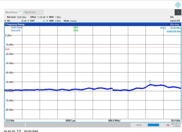
NTNV-n2-PC3-15-10-L-CP-QPSK-Edge_1RB_Left-12000-20000-P ASS
