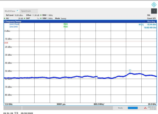
NTNV-n2-PC3-15-10-H-CP-QPSK-Edge_1RB_Left-12000-20000- PASS
