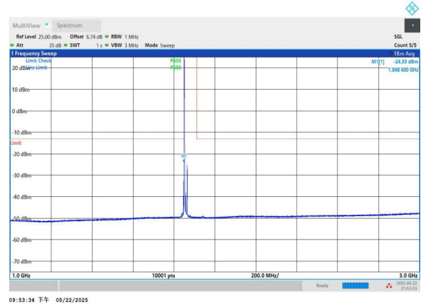
NTNV-n2-PC3-15-15-L-DFT-QPSK-Edge_1RB_Left-1000-3000-P ASS
