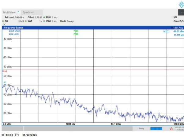
NTNV-n2-PC3-15-10-L-CP-QPSK-Edge_1RB_Left-0.009-0.15-P ASS
