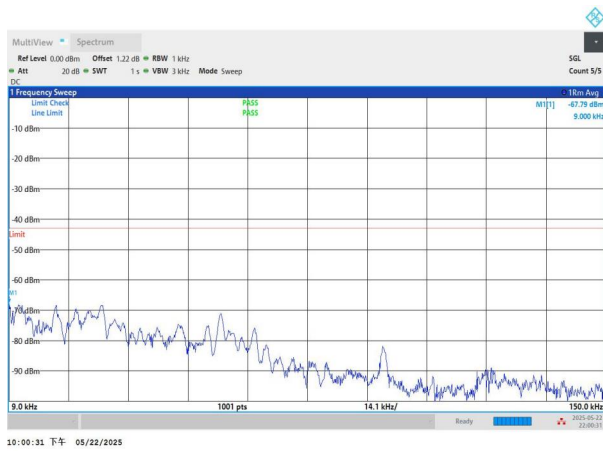
NTNV-n2-PC3-15-15-H-DFT-BPSK-Edge_1RB_Left-0.009-0.15-P
