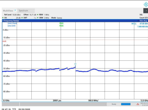
NTNV-n2-PC3-15-10-M-CP-QPSK-Edge_1RB_Left-3000-12000-PASS
