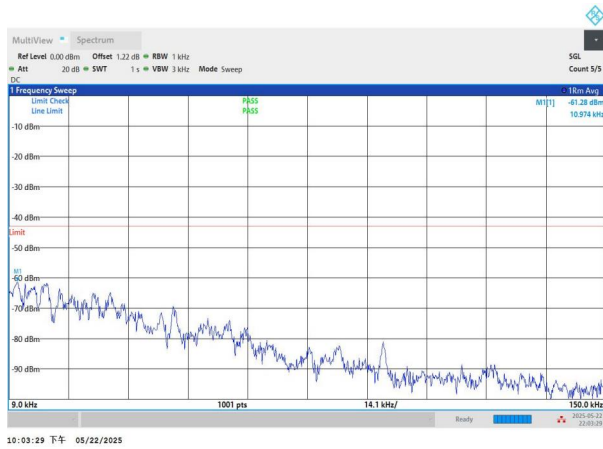
NTNV-n2-PC3-15-15-H-CP-QPSK-Edge_1RB_Left-0.009-0.15-P ASS
