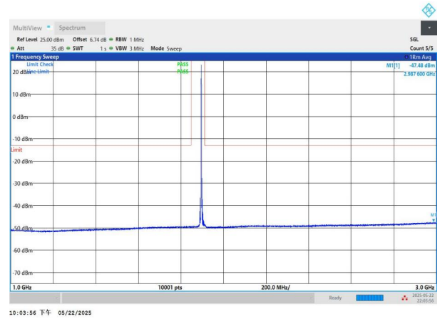
NTNV-n2-PC3-15-15-H-CP-QPSK-Edge_1RB_Left-1000-3000-PASS
