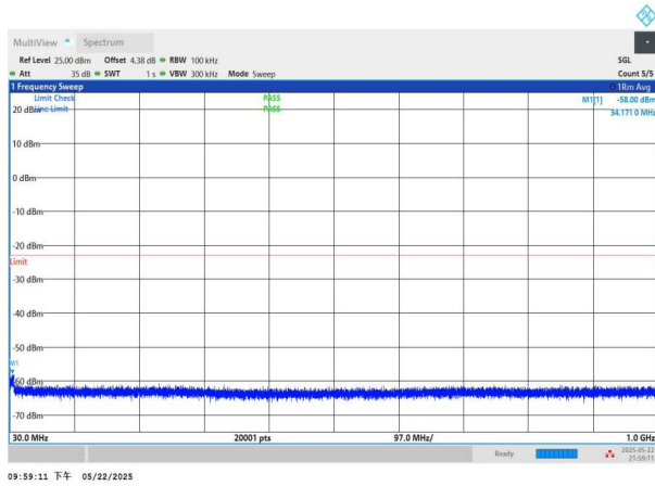
NTNV-n2-PC3-15-15-M-CP-QPSK-Edge_1RB_Left-30-1000-PASS
