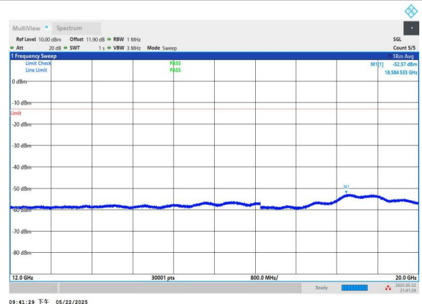
NTNV-n2-PC3-15-10-L-DFT-BPSK-Edge_1RB_Left-12000-20000- PASS
