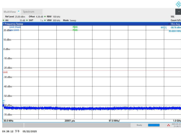
NTNV-n2-PC3-15-5-H-DFT-QPSK-Edge_1RB_Left-30-1000-PAS S
