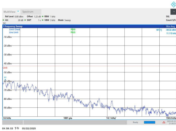
NTNV-n2-PC3-15-15-M-CP-QPSK-Edge_1RB_Left-0.009-0.15-PASS
