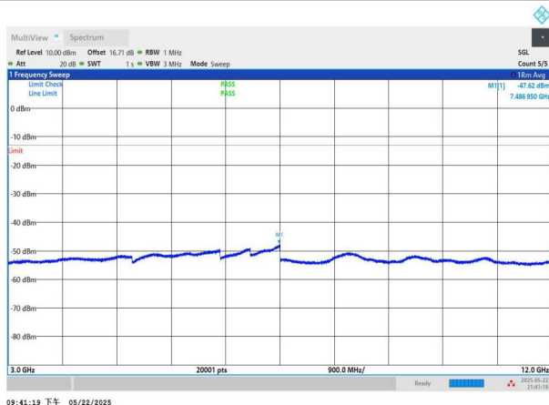
NTNV-n2-PC3-15-10-L-DFT-BPSK-Edge_1RB_Left-3000-12000- PASS
