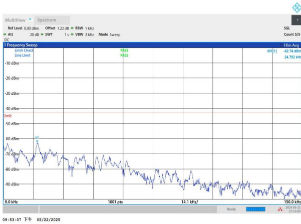
NTNV-n2-PC3-15-15-L-DFT-QPSK-Edge_1RB_Left-0.009-0.15-P ASS
