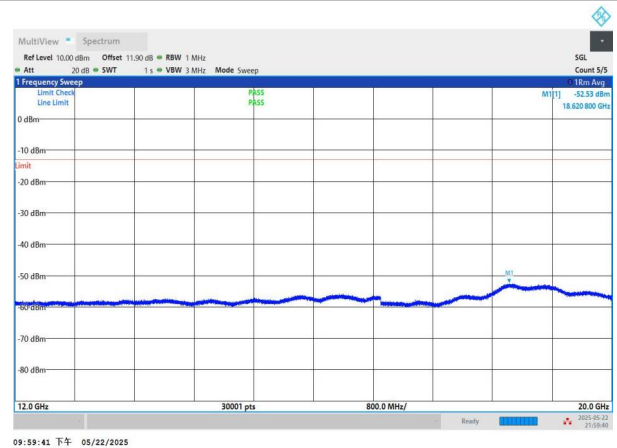
NTNV-n2-PC3-15-15-M-CP-QPSK-Edge_1RB_Left-12000-20000-PASS
