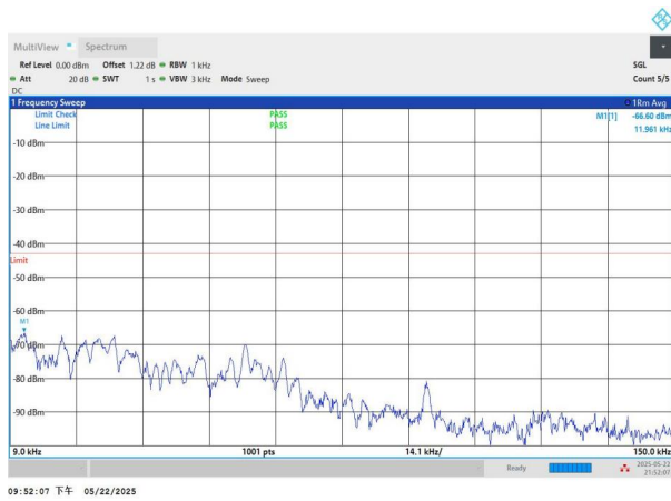
NTNV-n2-PC3-15-15-L-DFT-BPSK-Edge_1RB_Left-0.009-0.15-P ASS
