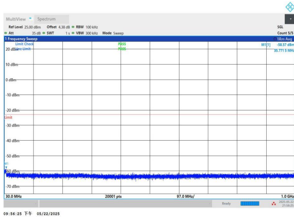
NTNV-n2-PC3-15-15-M-DFT-BPSK-Edge_1RB_Left-30-1000-PASS
