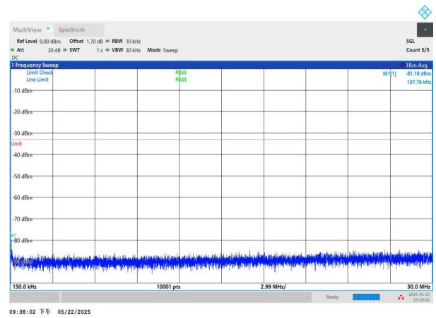
NTNV-n2-PC3-15-5-H-DFT-QPSK-Edge_1RB_Left-0.15-30-PASS
