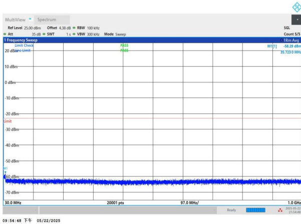
NTNV-n2-PC3-15-15-L-CP-QPSK-Edge_1RB_Left-30-1000-PAS S
