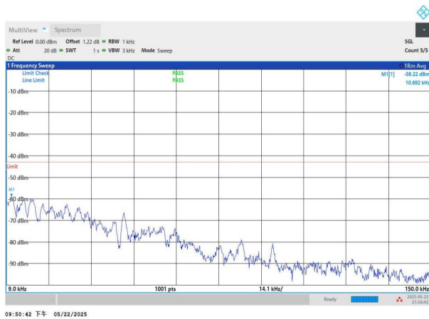
NTNV-n2-PC3-15-10-H-CP-QPSK-Edge_1RB_Left-0.009-0.15-P ASS
