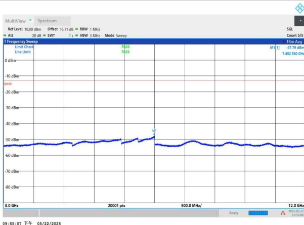
NTNV-n2-PC3-15-15-L-CP-QPSK-Edge_1RB_Left-3000-12000-P ASS
