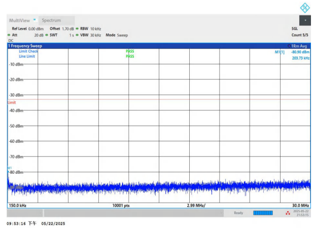
NTNV-n2-PC3-15-15-L-DFT-QPSK-Edge_1RB_Left-0.15-30-PASS
