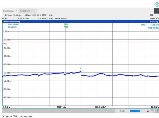
NTNV-n2-PC3-15-5-H-DFT-QPSK-Edge_1RB_Left-3000-12000- PASS
