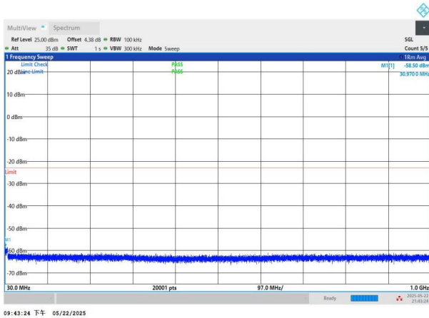
NTNV-n2-PC3-15-10-L-CP-QPSK-Edge_1RB_Left-30-1000-PAS S
