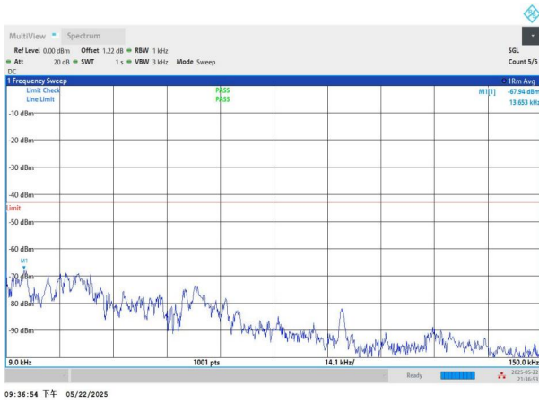
NTNV-n2-PC3-15-5-H-DFT-BPSK-Edge_1RB_Left-0.009-0.15-P ASS
