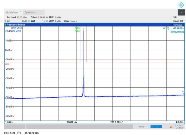
NTNV-n2-PC3-15-10-M-CP-QPSK-Edge_1RB_Left-1000-3000-PASS
