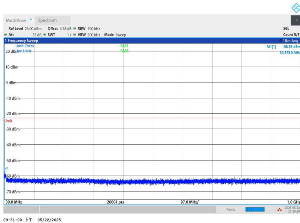
NTNV-n2-PC3-15-10-H-CP-QPSK-Edge_1RB_Left-30-1000-PAS S
