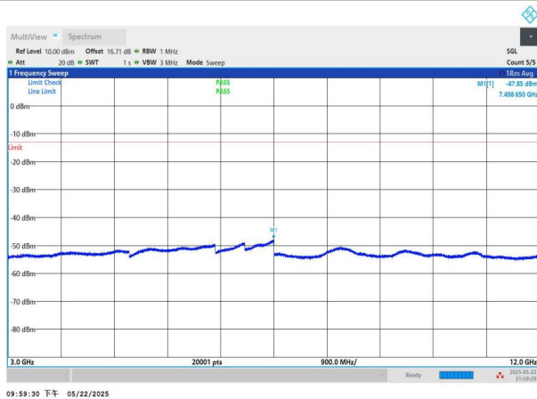
NTNV-n2-PC3-15-15-M-CP-QPSK-Edge_1RB_Left-3000-12000-PASS
