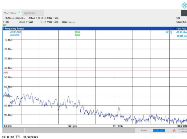
NTNV-n2-PC3-15-10-L-DFT-BPSK-Edge_1RB_Left-0.009-0.15-P ASS
