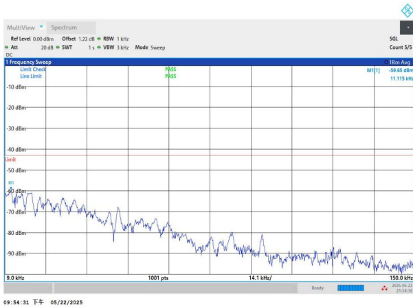
NTNV-n2-PC3-15-15-L-CP-QPSK-Edge_1RB_Left-0.009-0.15-P ASS
