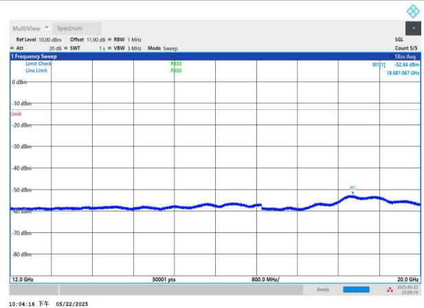
NTNV-n2-PC3-15-15-H-CP-QPSK-Edge_1RB_Left-12000-20000- PASS
