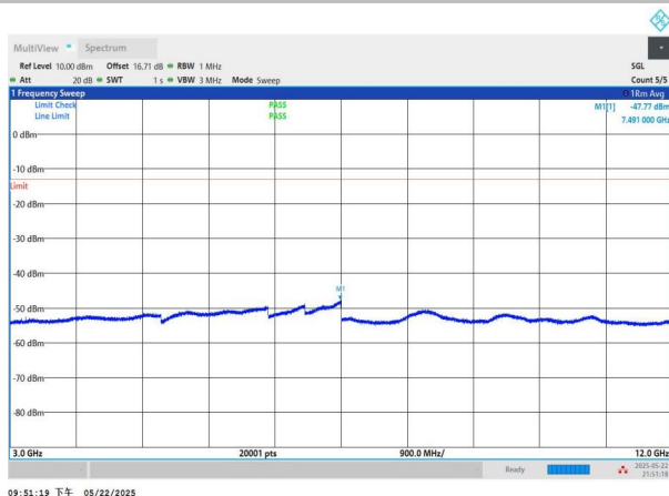
NTNV-n2-PC3-15-10-H-CP-QPSK-Edge_1RB_Left-3000-12000- PASS
