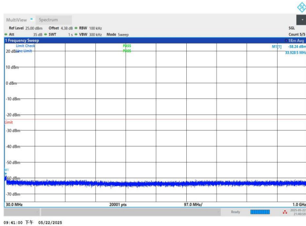
NTNV-n2-PC3-15-10-L-DFT-BPSK-Edge_1RB_Left-30-1000-PAS S
