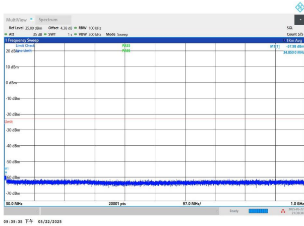
NTNV-n2-PC3-15-5-H-CP-QPSK-Edge_1RB_Left-30-1000-PASS
