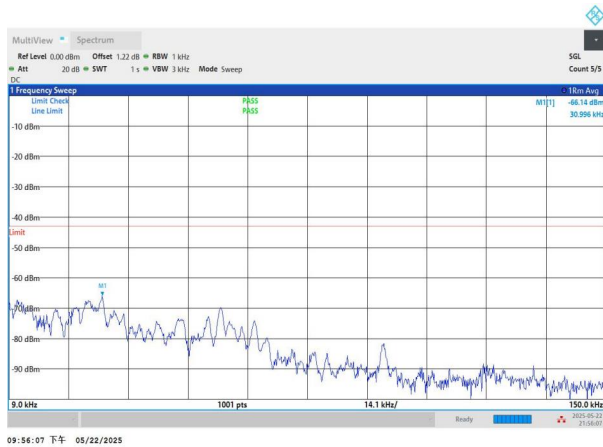
NTNV-n2-PC3-15-15-M-DFT-BPSK-Edge_1RB_Left-0.009-0.15-PASS
