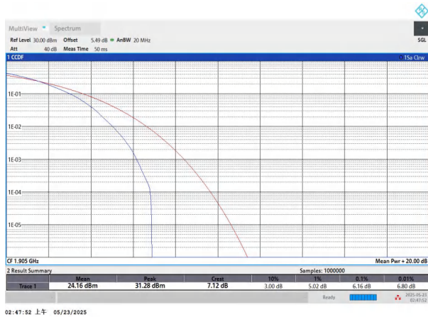
NTNV-n25-PC3-15-20-H-DFT-64QAM-Outer_Full-PASS
