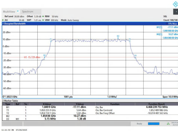
NTNV-n25-PC3-15-5-L-DFT-256QAM-Outter_Full-Ant1-PASS
