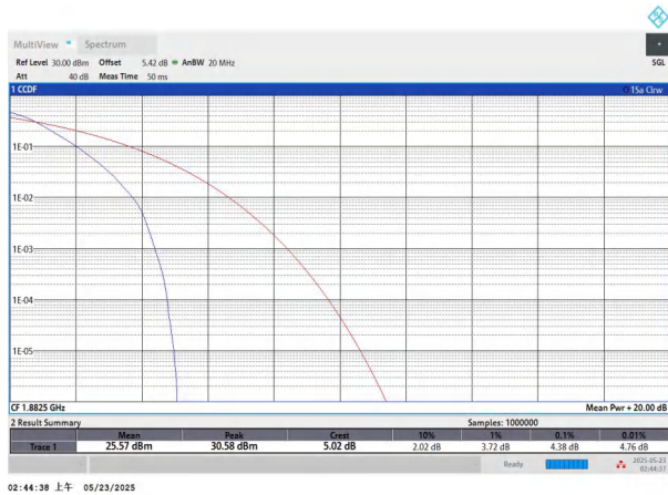
NTNV-n25-PC3-15-20-M-DFT-BPSK-Outer_Full-PASS
