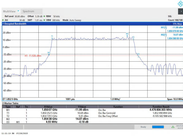
NTNV-n25-PC3-15-5-L-DFT-BPSK-Outter_Full-Ant1-PASS
