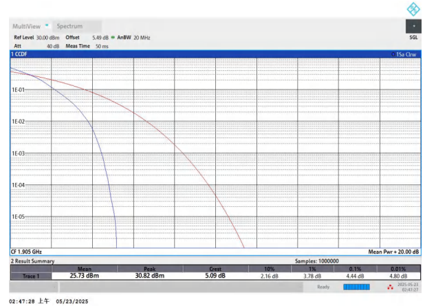
NTNV-n25-PC3-15-20-H-DFT-BPSK-Outer_Full-PASS
