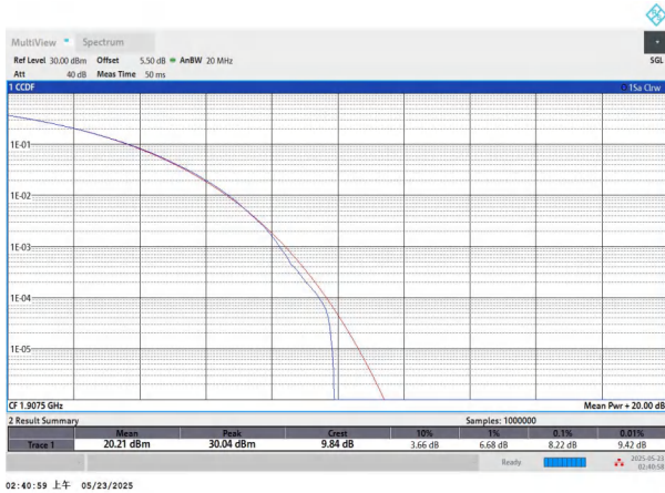
NTNV-n25-PC3-15-15-H-CP-256QAM-Outer_Full-PASS
