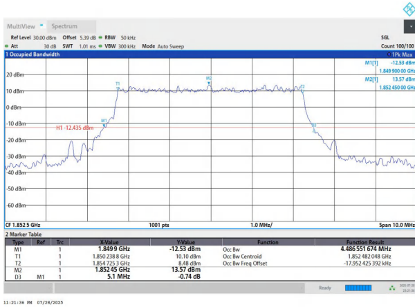
NTNV-n25-PC3-15-5-L-DFT-16QAM-Outter_Full-Ant1-PASS
