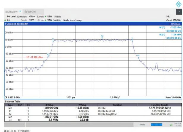
NTNV-n25-PC3-15-5-L-CP-QPSK-Outter_Full-Ant1-PASS
