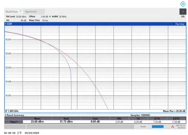
NTNV-n25-PC3-15-20-H-CP-16QAM-Outer_Full-PASS
