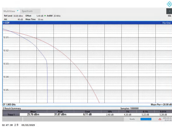
NTNV-n25-PC3-15-20-H-DFT-QPSK-Outer_Full-PASS
