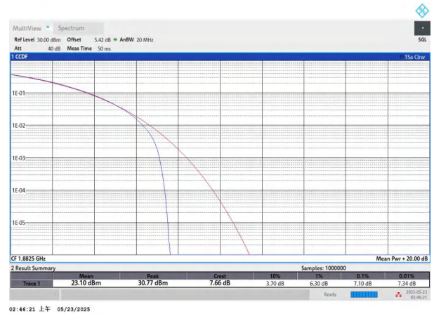
NTNV-n25-PC3-15-20-M-CP-64QAM-Outer_Full-PASS
