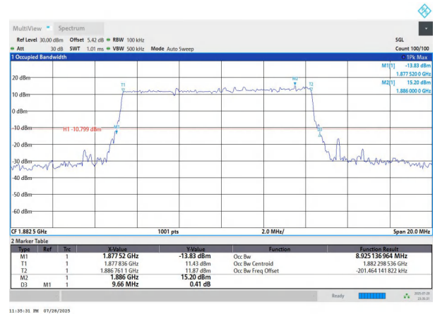
NTVN-n25-PC3-15-10-M-DFT-QPSK-Outet_Full-Ant1-PASS
