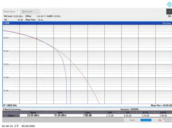
NTNV-n25-PC3-15-20-M-CP-16QAM-Outer_Full-PASS
