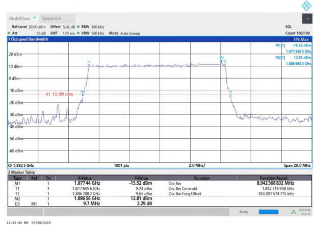
NTVN-n25-PC3-15-10-M-DFT-64QAM-Outet_Full-Ant1-PASS
