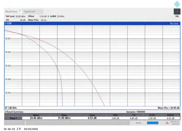
NTNV-n25-PC3-15-20-L-DFT-16QAM-Outer_Full-PASS
