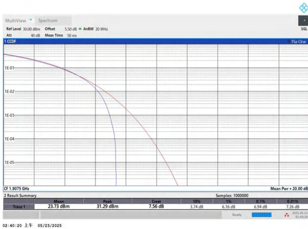
NTNV-n25-PC3-15-15-H-CP-16QAM-Outer_Full-PASS
