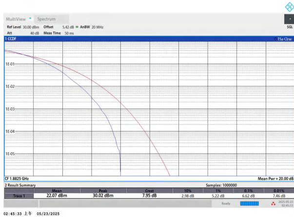
NTNV-n25-PC3-15-20-M-DFT-256QAM-Outer_Full-PASS
