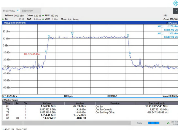
NTNV-n25-PC3-15-15-L-DFT-16QAM-Outet_Full-Ant1-PASS
