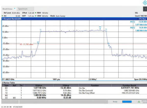
NTVN-n25-PC3-15-10-M-DFT-16QAM-Outet_Full-Ant1-PASS
