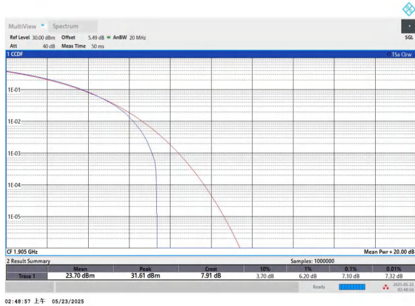
NTNV-n25-PC3-15-20-H-CP-QPSK-Outer_Full-PASS
