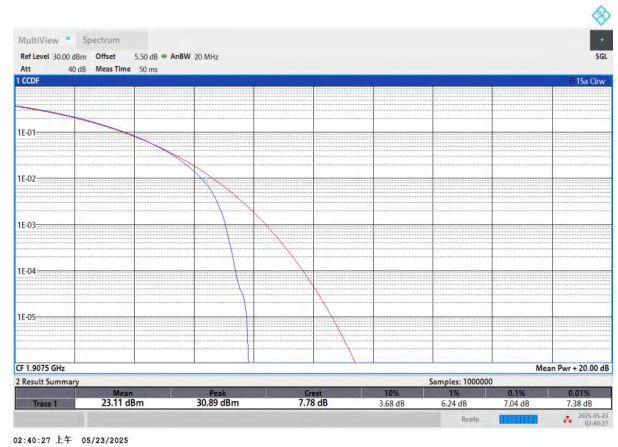
NTNV-n25-PC3-15-15-H-CP-64QAM-Outer_Full-PASS
