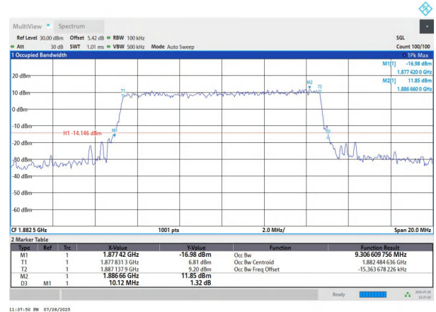
NTVN-n25-PC3-15-10-M-CP-QPSK-Outet_Full-Ant1-PASS
