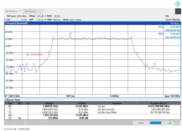
NTNV-n25-PC3-15-5-L-DFT-64QAM-Outter_Full-Ant1-PASS
