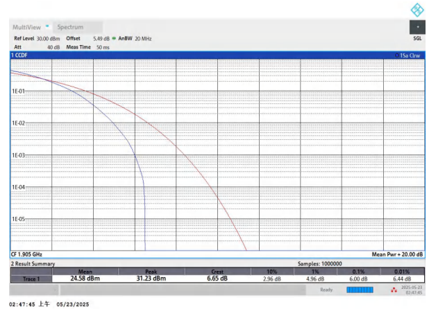
NTNV-n25-PC3-15-20-H-DFT-16QAM-Outer_Full-PASS
