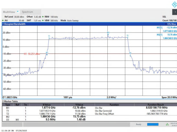
NTVN-n25-PC3-15-10-M-DFT-BPSK-Outet_Full-Ant1-PASS
