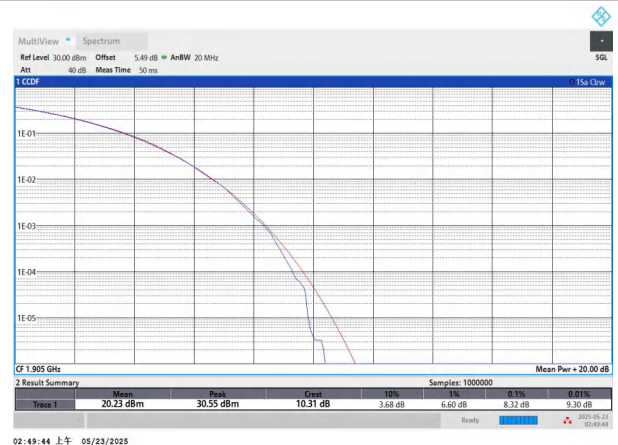
NTNV-n25-PC3-15-20-H-CP-256QAM-Outer_Full-PASS
