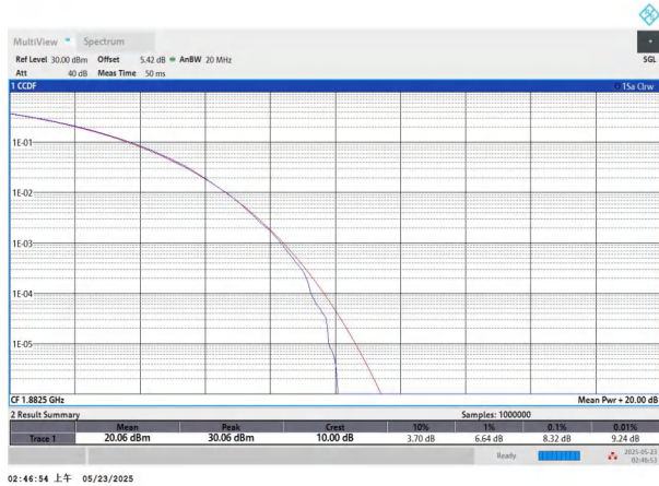
NTNV-n25-PC3-15-20-M-CP-256QAM-Outer_Full-PASS
