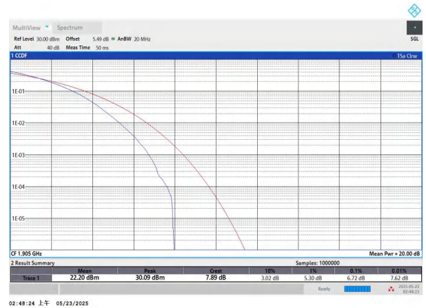
NTNV-n25-PC3-15-20-H-DFT-256QAM-Outer_Full-PASS
