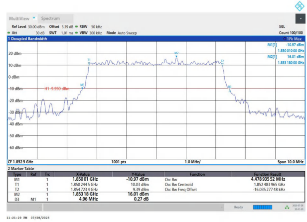
NTNV-n25-PC3-15-5-L-DFT-QPSK-Outter_Full-Ant1-PASS
