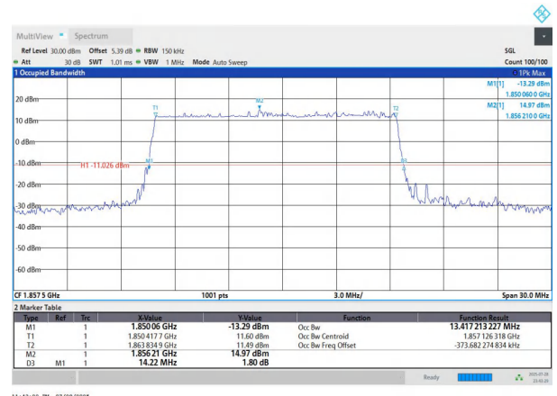
NTNV-n25-PC3-15-15-L-DFT-QPSK-Outet_Full-Ant1-PASS
