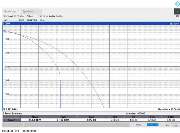
NTNV-n25-PC3-15-20-M-DFT-16QAM-Outer_Full-PASS
