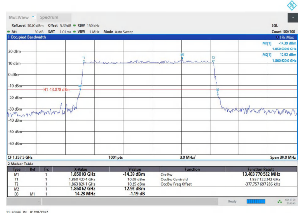
NTNV-n25-PC3-15-15-L-DFT-64QAM-Outet_Full-Ant1-PASS
