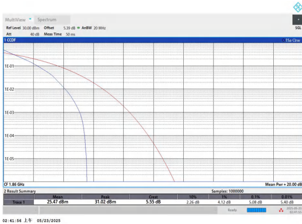
NTNV-n25-PC3-15-20-L-DFT-QPSK-Outer_Full-PASS
