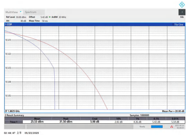
NTNV-n25-PC3-15-20-M-DFT-QPSK-Outer_Full-PASS
