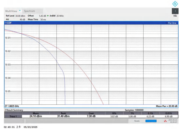
NTNV-n25-PC3-15-20-M-DFT-64QAM-Outer_Full-PASS
