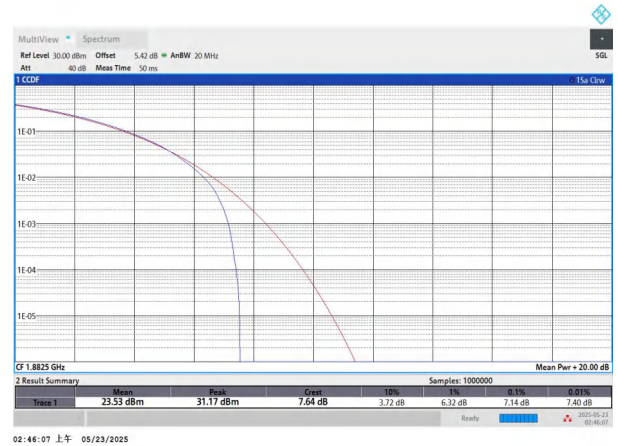
NTNV-n25-PC3-15-20-M-CP-QPSK-Outer_Full-PASS
