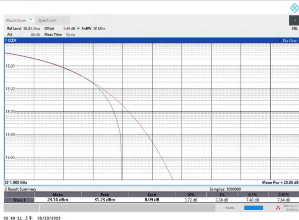
NTNV-n25-PC3-15-20-H-CP-64QAM-Outer_Full-PASS
