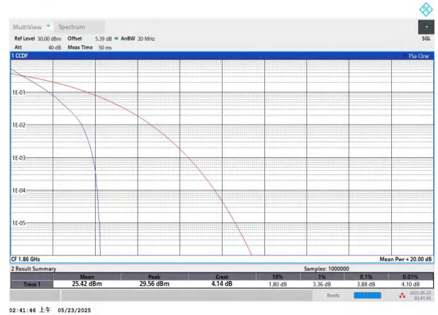
NTNV-n25-PC3-15-20-L-DFT-BPSK-Outer_Full-PASS
