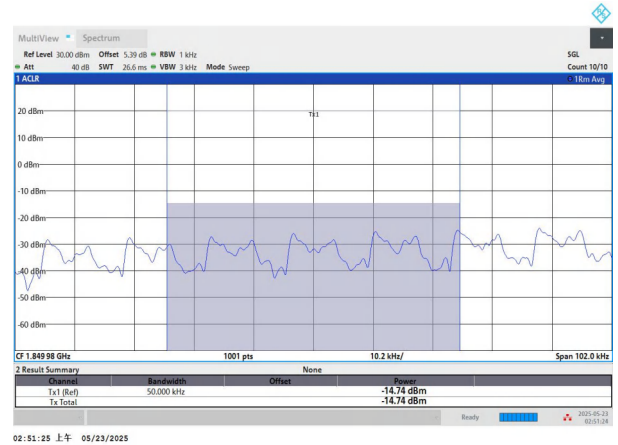
NTNV-n25-PC3-15-5-L-DFT-QPSK-Edge_1RB_Left-PASS_Final1
