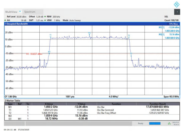
NTNV-n25-PC3-15-20-L-DFT-QPSK-Outet_Full-Ant1-PASS
