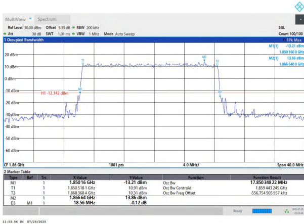
NTNV-n25-PC3-15-20-L-DFT-16QAM-Outet_Full-Ant1-PASS
