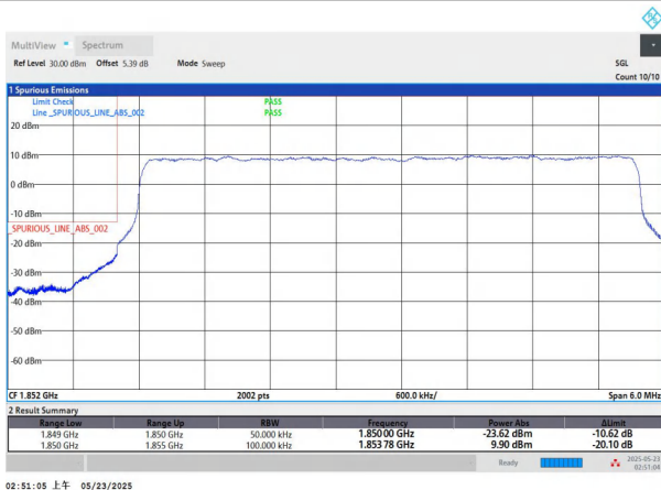
NTNV-n25-PC3-15-5-L-DFT-QPSK-Outer_Full-PASS
