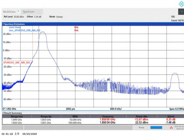
NTNV-n25-PC3-15-5-L-DFT-QPSK-Edge_1RB_Left
