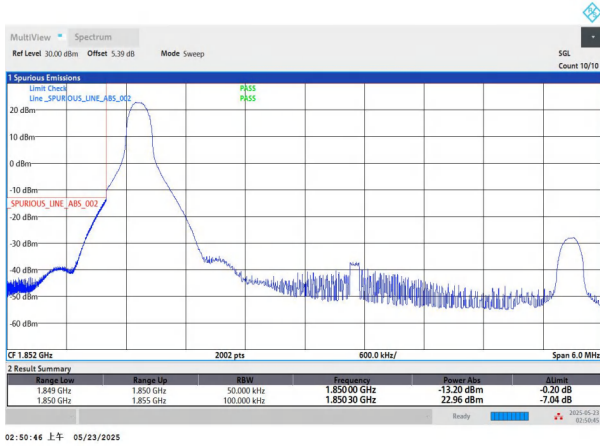
NTNV-n25-PC3-15-5-L-DFT-BPSK-Edge_1RB_Left-PASS
