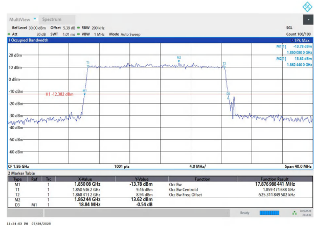
NTNV-n25-PC3-15-20-L-DFT-64QAM-Outet_Full-Ant1-PASS
