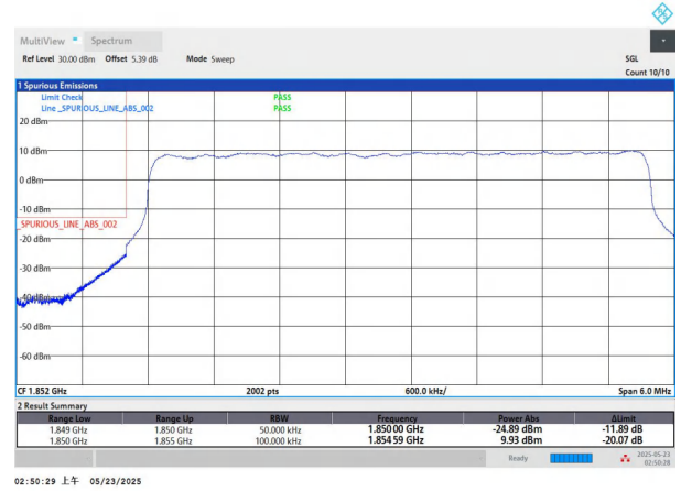
NTNV-n25-PC3-15-5-L-DFT-BPSK-Outer_Full-PASS
