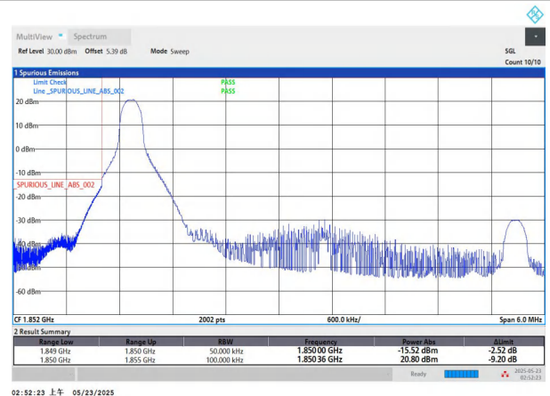
NTNV-n25-PC3-15-5-L-CP-QPSK-Edge_1RB_Left-PASS
