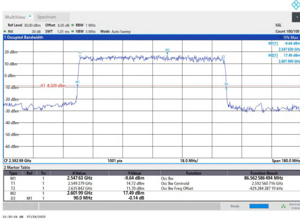
NTNV-n41-PC2-30-90-M-DFT-BPSK-Outer_Full-Ant1-PASS
