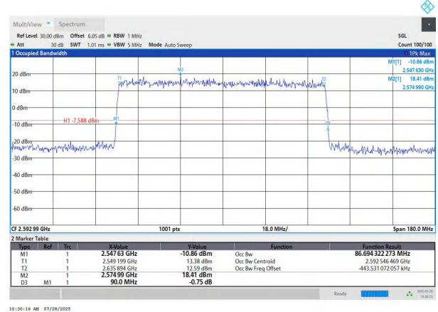
NTNV-n41-PC2-30-90-M-DFT-QPSK-Outer_Full-Ant1-PASS
