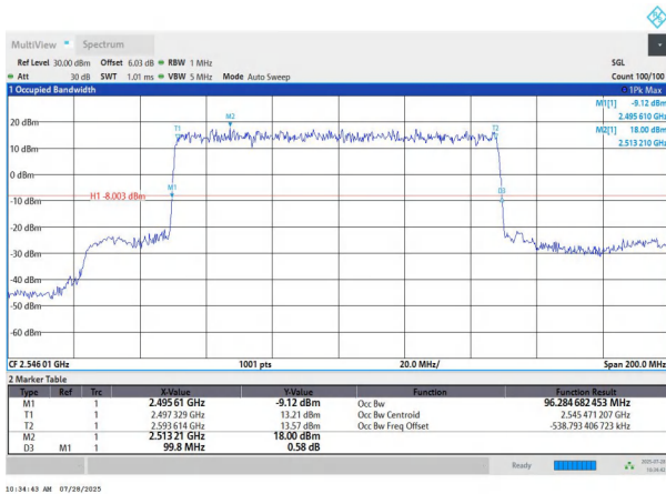
NTNV-n41-PC2-30-100-L-DFT-BPSK-Outer_Full-Ant1-PASS
