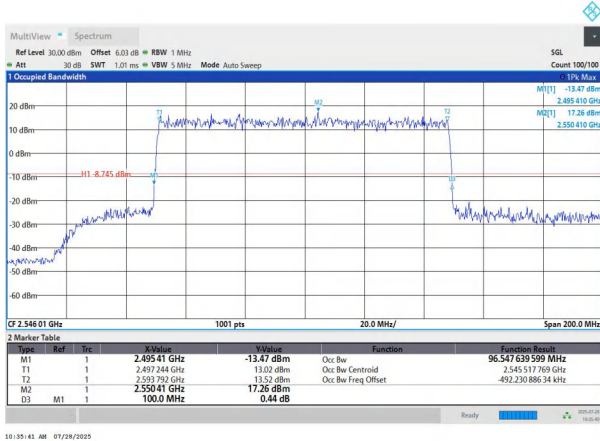
NTNV-n41-PC2-30-100-L-DFT-16QAM-Outer_Full-Ant1-PASS
