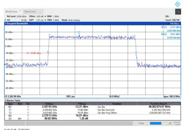
NTNV-n41-PC2-30-90-M-DFT-64QAM-Outer_Full-Ant1-PASS
