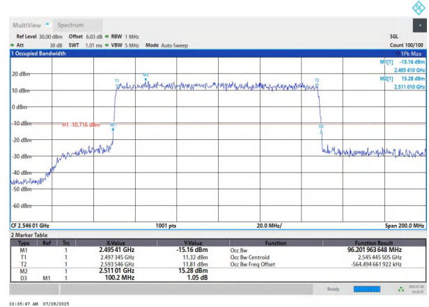
NTNV-n41-PC2-30-100-L-DFT-64QAM-Outer_Full-Ant1-PASS
