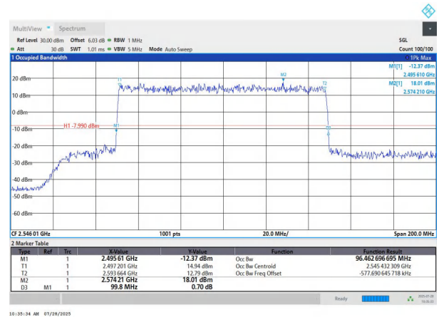
NTNV-n41-PC2-30-100-L-DFT-QPSK-Outer_Full-Ant1-PASS
