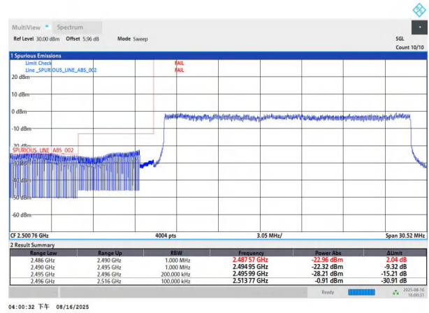
NTVN-n41-PC2-30-20-L-DFT-BPSK-Outer_Full
