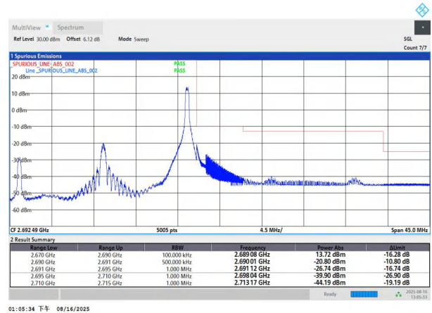
NTVN-n41-PC2-30-20-H-DFT-BPSK-Edge_1RB_Right-PASS
