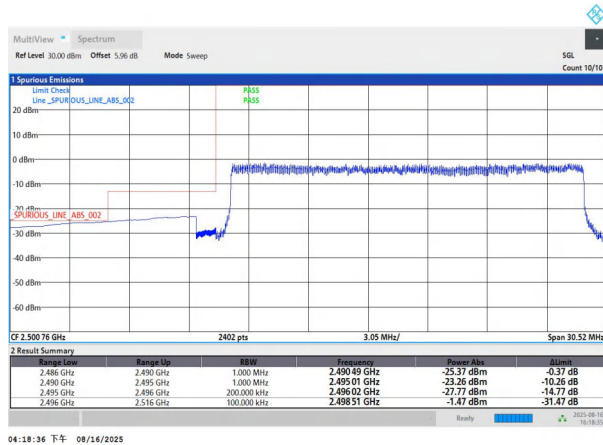
NTVN-n41-PC2-30-20-L-DFT-QPSK-Outer_Full-PASS
