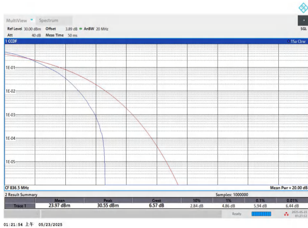
NTNV-n5-PC3-15-15-M-DFT-64QAM-Outer_Full-PASS
