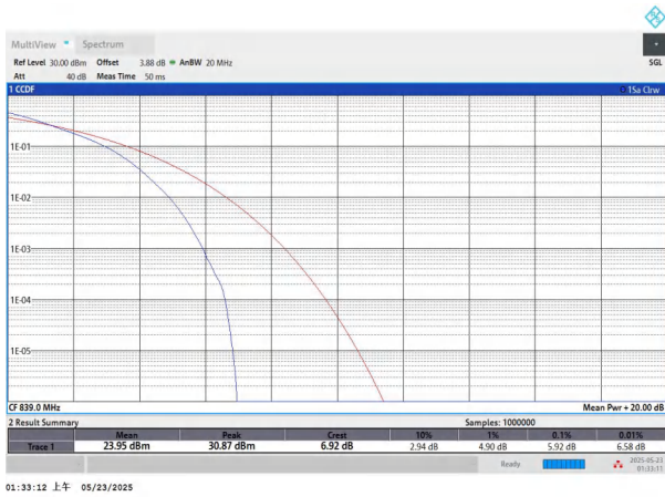
NTNV-n5-PC3-15-20-H-DFT-64QAM-Outer_Full-PASS
