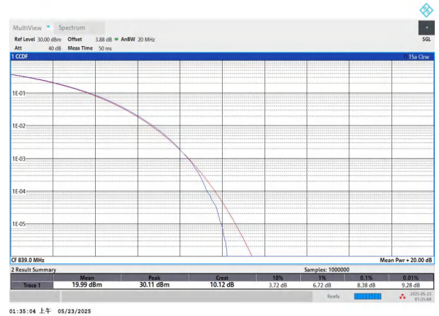
NTNV-n5-PC3-15-20-H-CP-256QAM-Outer_Full-PASS
