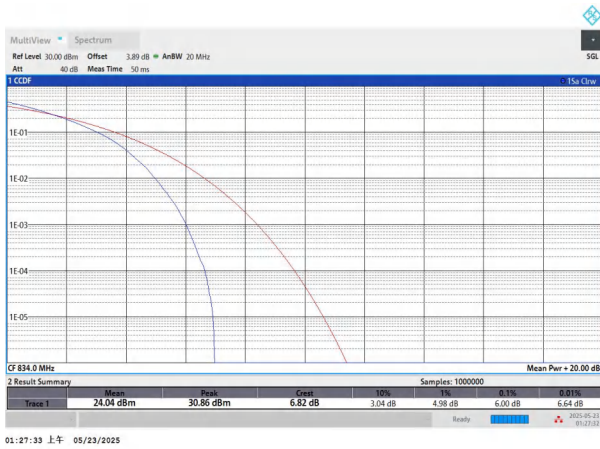
NTNV-n5-PC3-15-20-L-DFT-64QAM-Outer_Full-PASS
