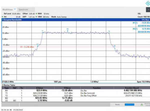
NTNV-n5-PC3-15-5-L-DFT-16QAM-Outer_Full-Ant1-PASS
