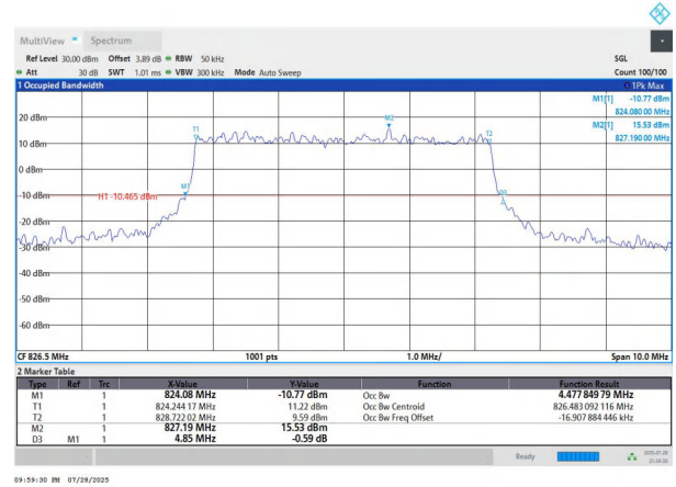
NTNV-n5-PC3-15-5-L-DFT-QPSK-Outer_Full-Ant1-PASS
