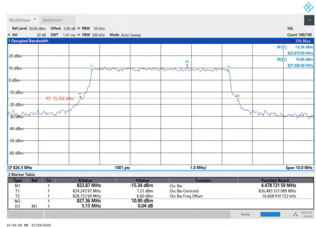
NTNV-n5-PC3-15-5-L-CP-QPSK-Outer_Full-Ant1-PASS
