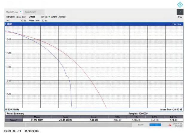
NTNV-n5-PC3-15-15-M-DFT-256QAM-Outer_Full-PASS
