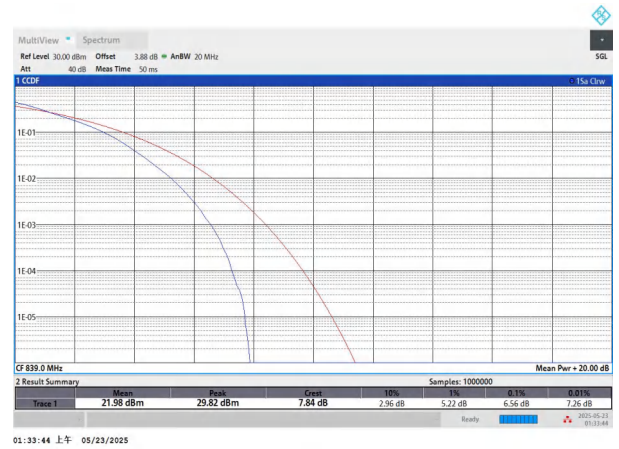
NTNV-n5-PC3-15-20-H-DFT-256QAM-Outer_Full-PASS
