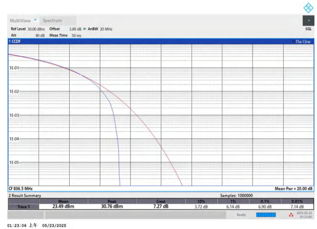
NTNV-n5-PC3-15-15-M-CP-16QAM-Outer_Full-PASS
