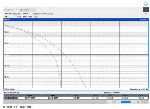
NTNV-n5-PC3-15-20-L-DFT-256QAM-Outer_Full-PASS
