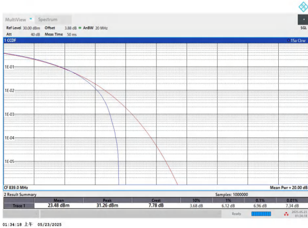
NTNV-n5-PC3-15-20-H-CP-QPSK-Outer_Full-PASS
