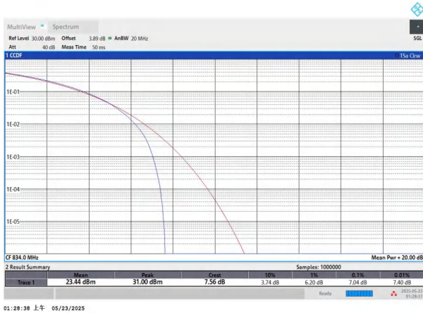
NTNV-n5-PC3-15-20-L-CP-QPSK-Outer_Full-PASS
