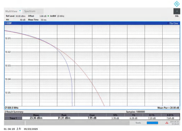
NTNV-n5-PC3-15-20-H-CP-16QAM-Outer_Full-PASS
