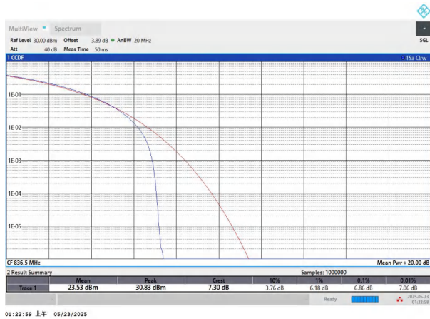
NTNV-n5-PC3-15-15-M-CP-QPSK-Outer_Full-PASS
