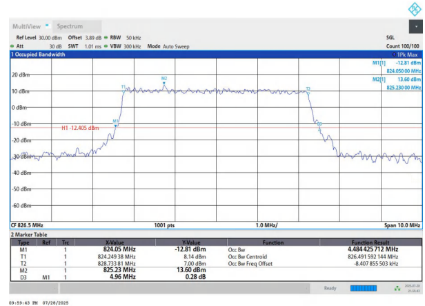
NTNV-n5-PC3-15-5-L-DFT-64QAM-Outer_Full-Ant1-PASS
