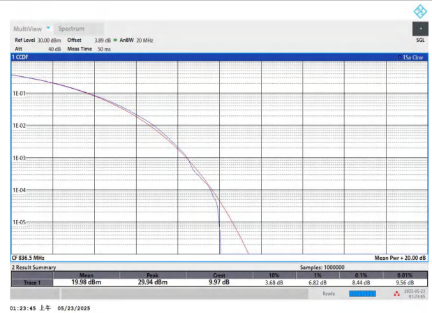
NTNV-n5-PC3-15-15-M-CP-256QAM-Outer_Full-PASS
