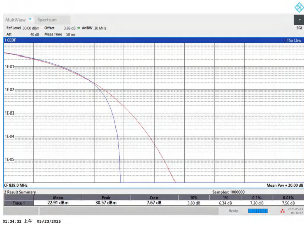
NTNV-n5-PC3-15-20-H-CP-64QAM-Outer_Full-PASS
