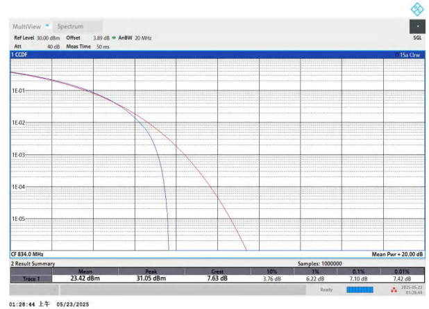
NTNV-n5-PC3-15-20-L-CP-16QAM-Outer_Full-PASS
