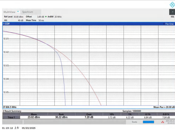
NTNV-n5-PC3-15-15-M-CP-64QAM-Outer_Full-PASS
