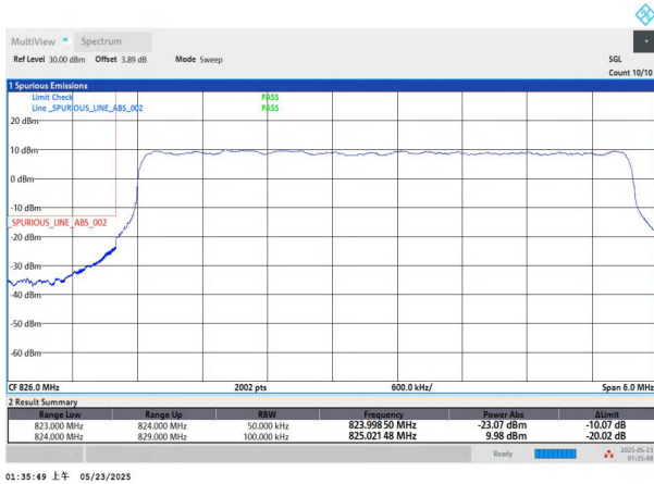
NTNV-n5-PC3-15-5-L-DFT-BPSK-Outer_Full-PASS
