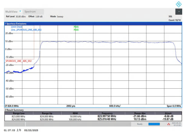
NTNV-n5-PC3-15-5-L-DFT-QPSK-Outer_Full-PASS
