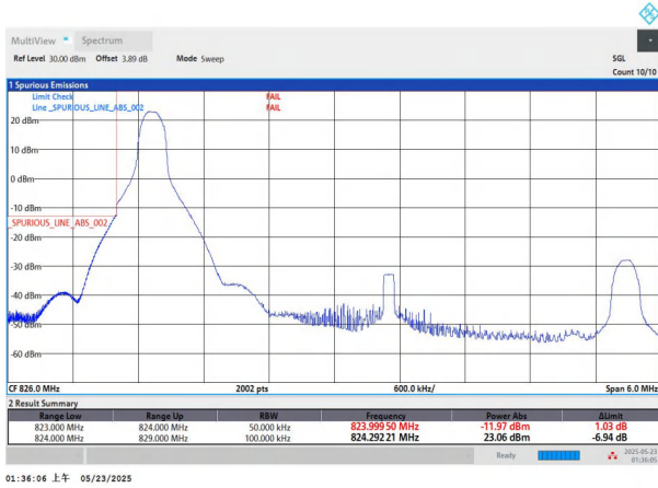
NTNV-n5-PC3-15-5-L-DFT-BPSK-Edge_1RB_Left
