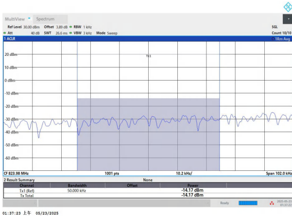
NTNV-n5-PC3-15-5-L-DFT-QPSK-Edge_1RB_Left-PASS_Final1
