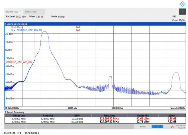
NTNV-n5-PC3-15-5-L-DFT-QPSK-Edge_1RB_Left
