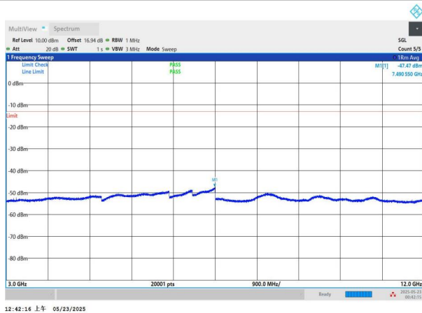
NTNV-n5-PC3-15-15-M-DFT-QPSK-Edge_1RB_Left-3000-12000-PASS
