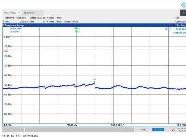
NTNV-n5-PC3-15-10-M-CP-QPSK-Edge_1RB_Left-3000-12000- PASS
