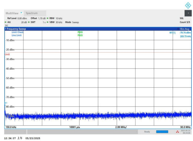
NTNV-n5-PC3-15-10-H-DFT-QPSK-Edge_1RB_Left-0.15-30-PASS
