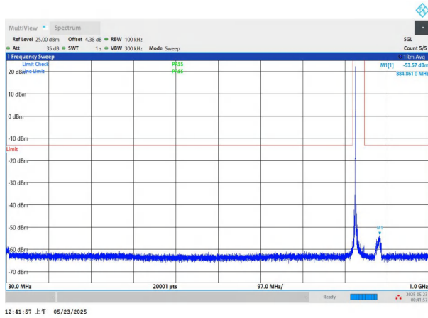
NTNV-n5-PC3-15-15-M-DFT-QPSK-Edge_1RB_Left-30-1000-PASS
