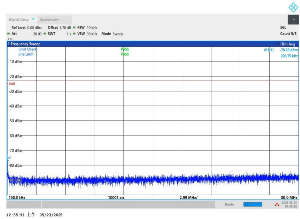
NTNV-n5-PC3-15-10-H-CP-QPSK-Edge_1RB_Left-0.15-30-PASS
