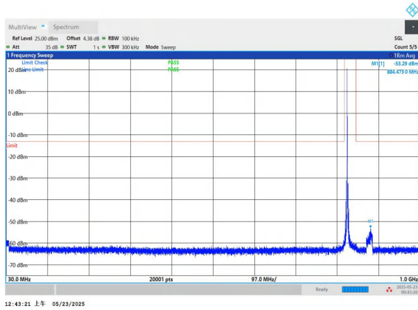
NTNV-n5-PC3-15-15-M-CP-QPSK-Edge_1RB_Left-30-1000-PAS S
