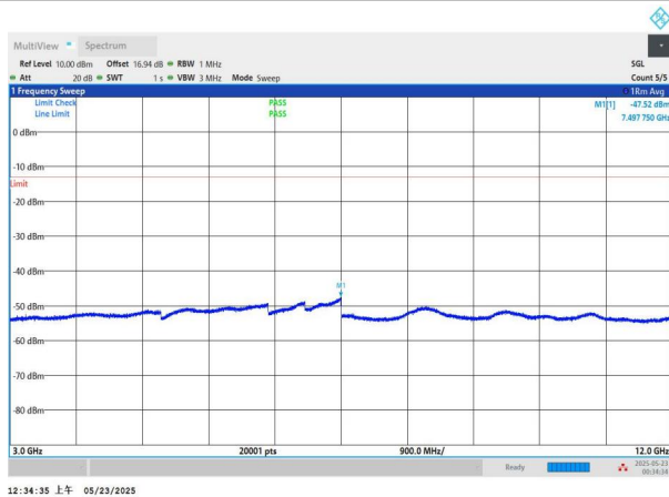
NTNV-n5-PC3-15-10-H-DFT-QPSK-Edge_1RB_Left-3000-12000-PASS
