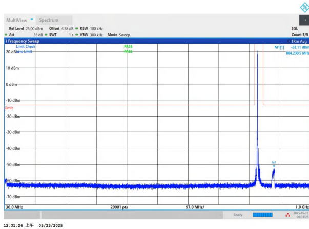
NTNV-n5-PC3-15-10-M-CP-QPSK-Edge_1RB_Left-30-1000-PAS S
