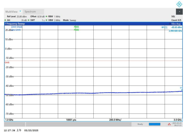
NTNV-n5-PC3-15-10-L-CP-QPSK-Edge_1RB_Left-1000-3000-PA SS
