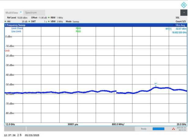
NTNV-n5-PC3-15-15-L-DFT-BPSK-Edge_1RB_Left-12000-20000- PASS
