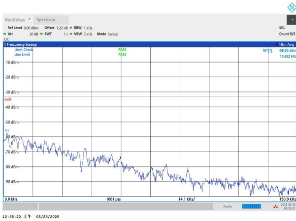
NTNV-n5-PC3-15-10-H-CP-QPSK-Edge_1RB_Left-0.009-0.15-P ASS
