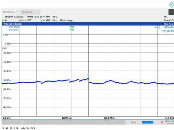
NTNV-n5-PC3-15-15-L-DFT-QPSK-Edge_1RB_Left-3000-12000- PASS
