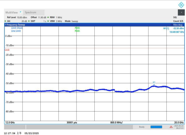
NTNV-n5-PC3-15-10-L-CP-QPSK-Edge_1RB_Left-12000-20000-P ASS
