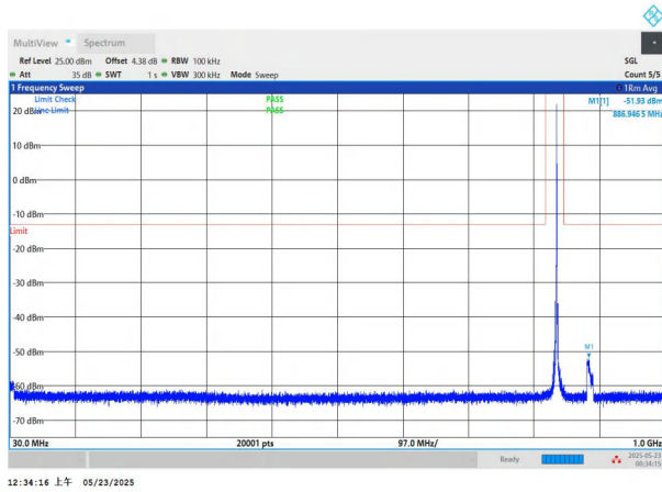
NTNV-n5-PC3-15-10-H-DFT-QPSK-Edge_1RB_Left-30-1000-PA
