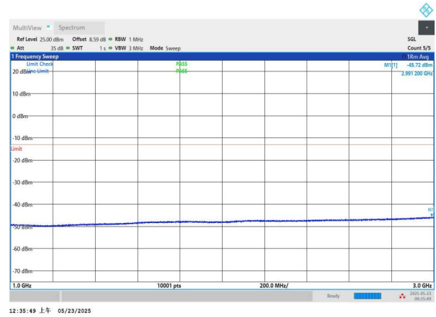
NTNV-n5-PC3-15-10-H-CP-QPSK-Edge_1RB_Left-1000-3000-PASS
