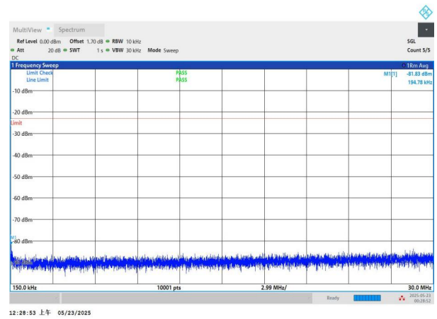
NTNV-n5-PC3-15-10-M-DFT-BPSK-Edge_1RB_Left-0.15-30-PASS
