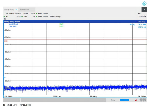
NTNV-n5-PC3-15-15-M-CP-QPSK-Edge_1RB_Left-0.15-30-PASS
