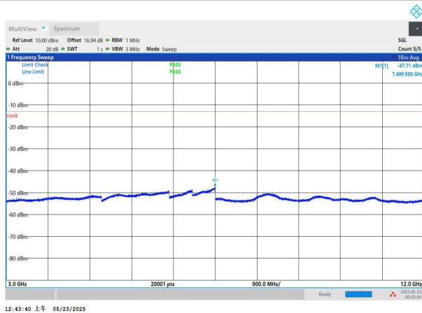
NTNV-n5-PC3-15-15-M-CP-QPSK-Edge_1RB_Left-3000-12000- PASS
