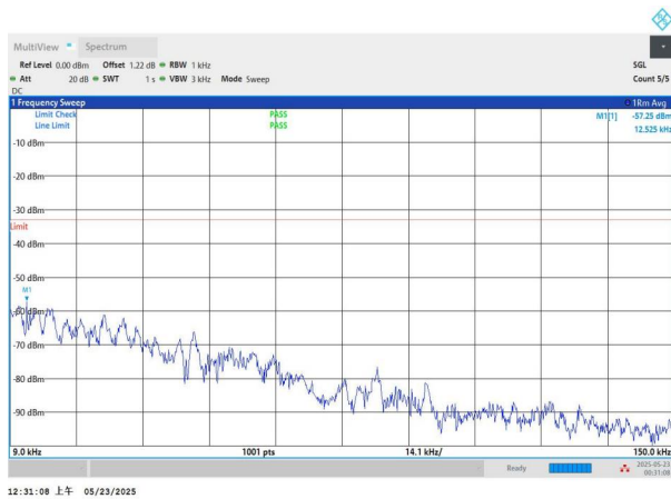
NTNV-n5-PC3-15-10-M-CP-QPSK-Edge_1RB_Left-0.009-0.15-P ASS
