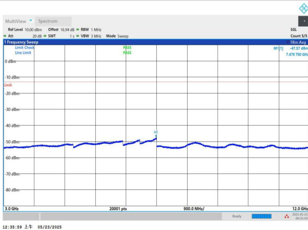
NTNV-n5-PC3-15-10-H-CP-QPSK-Edge_1RB_Left-3000-12000- PASS
