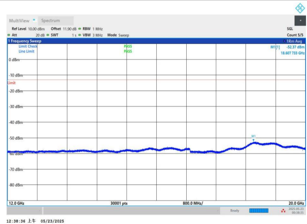
NTNV-n5-PC3-15-15-L-DFT-QPSK-Edge_1RB_Left-12000-20000- PASS
