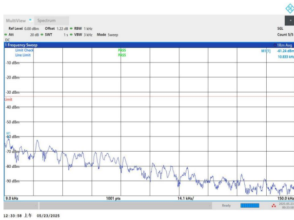
NTNV-n5-PC3-15-10-H-DFT-QPSK-Edge_1RB_Left-0.009-0.15-PASS
