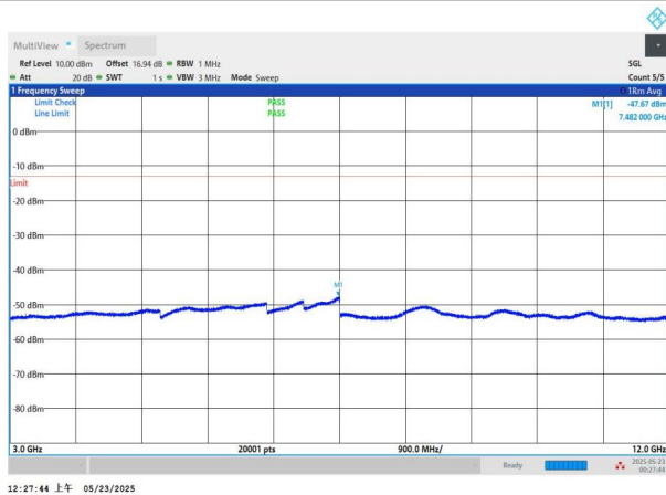
NTNV-n5-PC3-15-10-L-CP-QPSK-Edge_1RB_Left-3000-12000-P ASS
