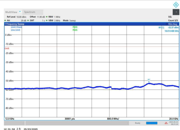
NTNV-n5-PC3-15-10-M-CP-QPSK-Edge_1RB_Left-12000-20000- PASS
