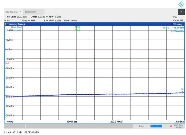
NTNV-n5-PC3-15-15-M-CP-QPSK-Edge_1RB_Left-1000-3000-PASS
