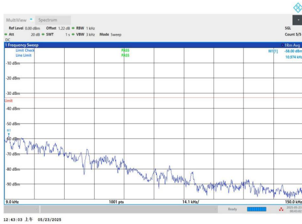
NTNV-n5-PC3-15-15-M-CP-QPSK-Edge_1RB_Left-0.009-0.15-P ASS
