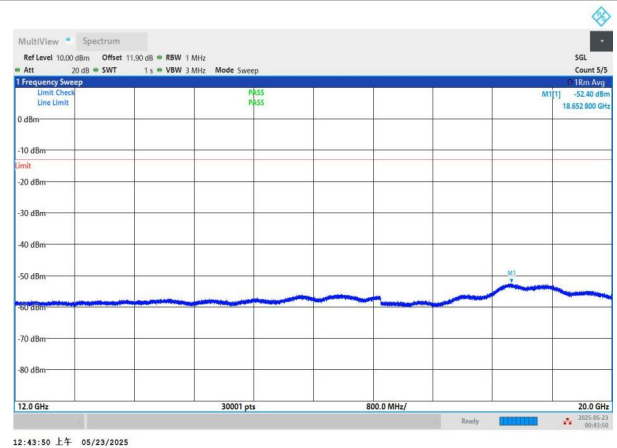
NTNV-n5-PC3-15-15-M-CP-QPSK-Edge_1RB_Left-12000-20000- PASS
