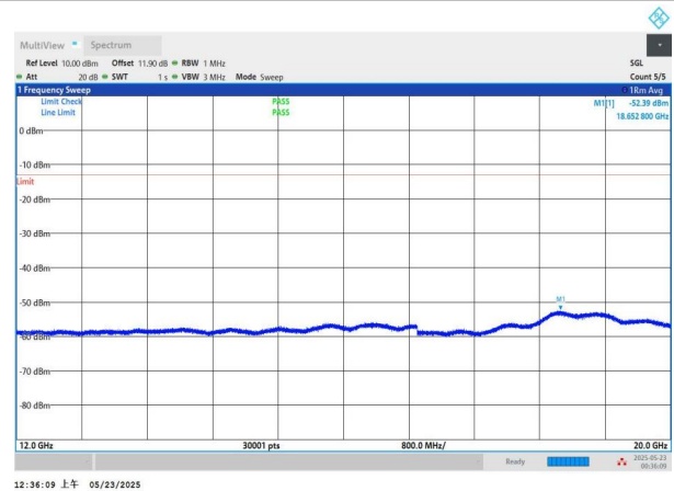
NTNV-n5-PC3-15-10-H-CP-QPSK-Edge_1RB_Left-12000-20000- PASS
