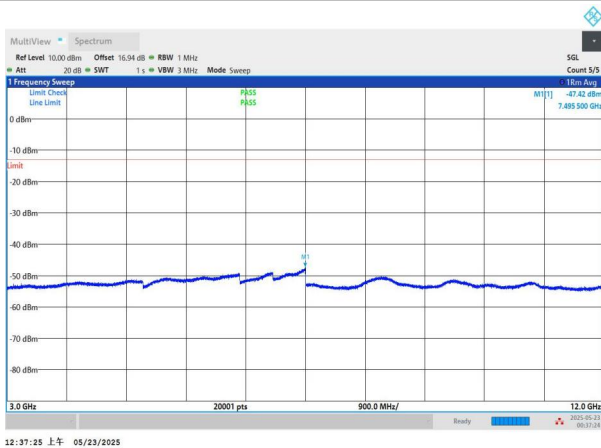
NTNV-n5-PC3-15-15-L-DFT-BPSK-Edge_1RB_Left-3000-12000- PASS
