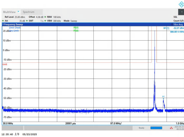
NTNV-n5-PC3-15-10-H-CP-QPSK-Edge_1RB_Left-30-1000-PAS S
