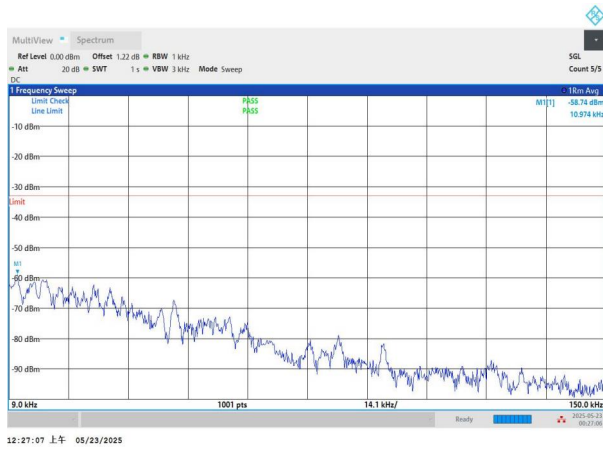
NTNV-n5-PC3-15-10-L-CP-QPSK-Edge_1RB_Left-0.009-0.15-P ASS
