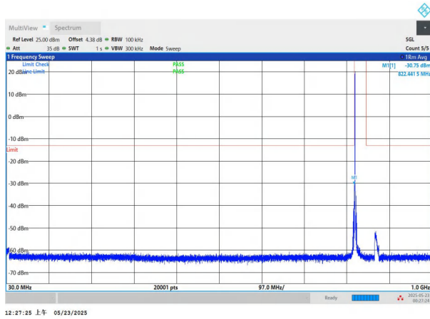
NTNV-n5-PC3-15-10-L-CP-QPSK-Edge_1RB_Left-30-1000-PAS S
