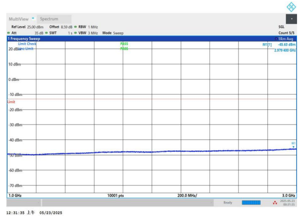
NTNV-n5-PC3-15-10-M-CP-QPSK-Edge_1RB_Left-1000-3000-PASS
