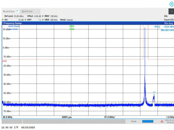
NTNV-n5-PC3-15-10-M-DFT-QPSK-Edge_1RB_Left-30-1000-PA
