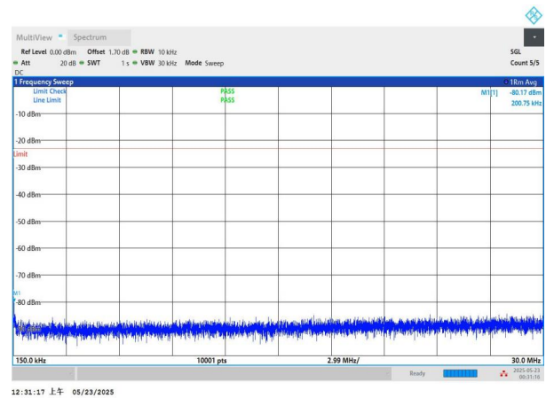
NTNV-n5-PC3-15-10-M-CP-QPSK-Edge_1RB_Left-0.15-30-PASS
