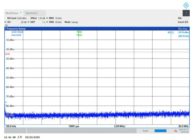
NTNV-n5-PC3-15-15-M-DFT-QPSK-Edge_1RB_Left-0.15-30-PASS
