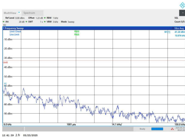
NTNV-n5-PC3-15-15-M-DFT-QPSK-Edge_1RB_Left-0.009-0.15-PASS
