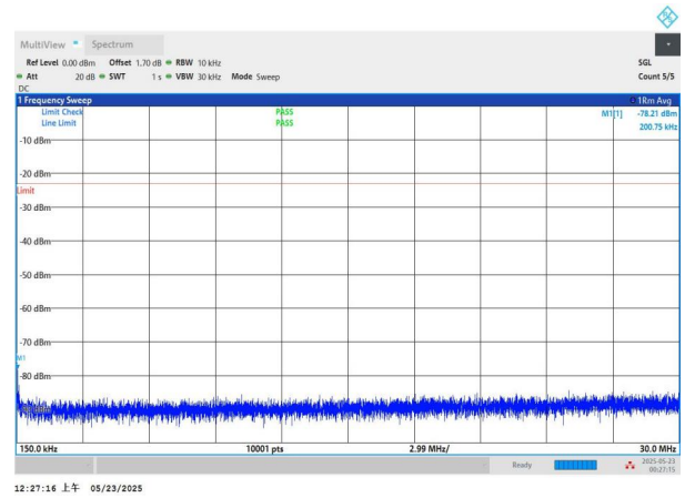
NTNV-n5-PC3-15-10-L-CP-QPSK-Edge_1RB_Left-0.15-30-PASS
