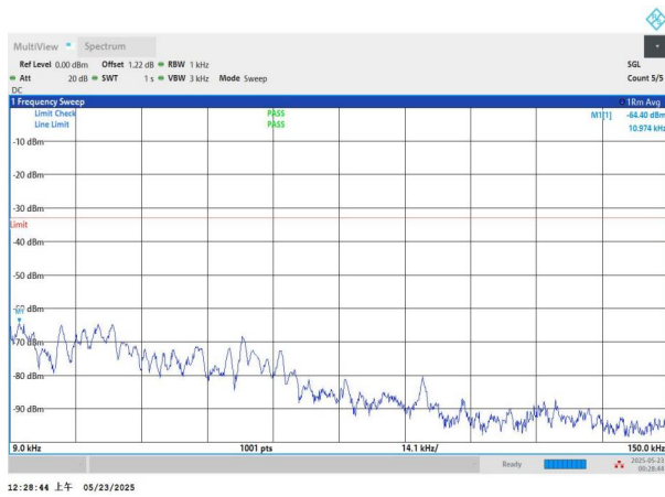
NTNV-n5-PC3-15-10-M-DFT-BPSK-Edge_1RB_Left-0.009-0.15-PASS
