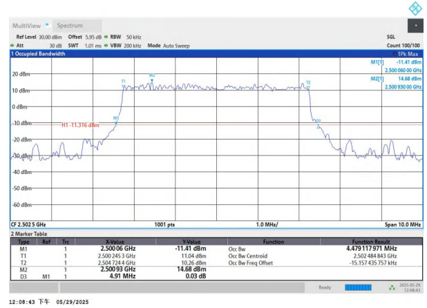
NTNV-n7-PC3-15-5-L-DFT-QPSK-Outer_Full-Ant1-PASS
