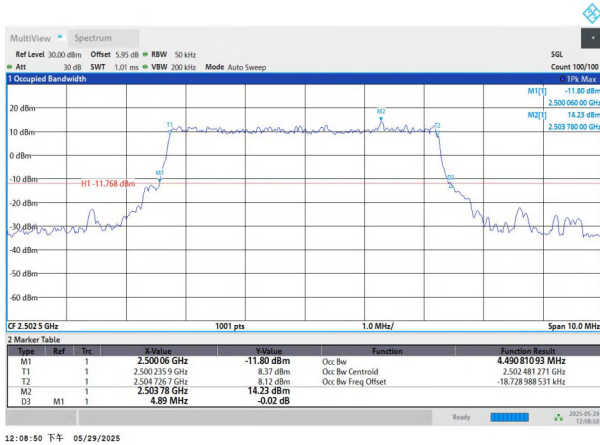
NTNV-n7-PC3-15-5-L-DFT-16QAM-Outer_Full-Ant1-PASS
