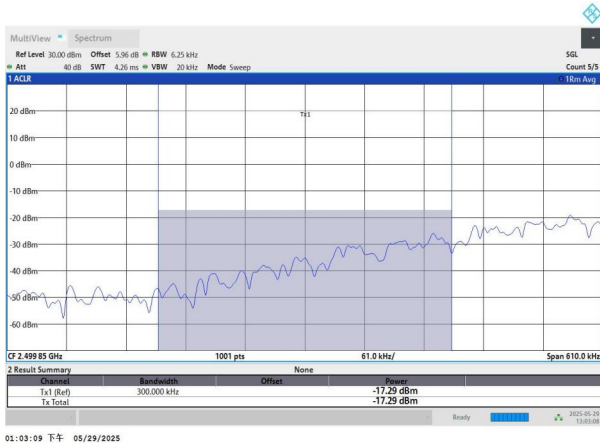
NTNV-n7-PC3-15-15-L-DFT-BPSK-Edge_1RB_Left-PASS_Final1
