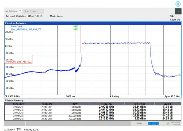
NTNV-n7-PC3-15-15-L-DFT-BPSK-Outer_Full-PASS
