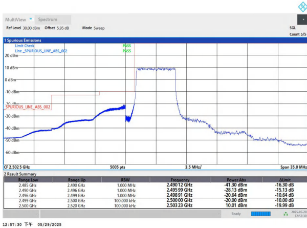
NTNV-n7-PC3-15-5-L-DFT-QPSK-Outter_Full-PASS
