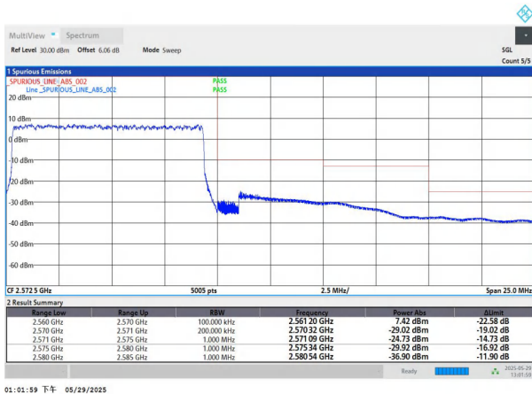
NTNV-n7-PC3-15-10-H-DFT-QPSK-Outer_Full-PASS
