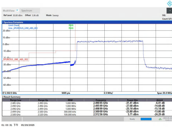
NTNV-n7-PC3-15-15-L-DFT-QPSK-Outer_Full-PASS
