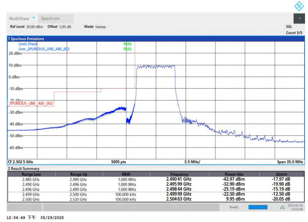
NTNV-n7-PC3-15-5-L-DFT-BPSK-Outter_Full-PASS
