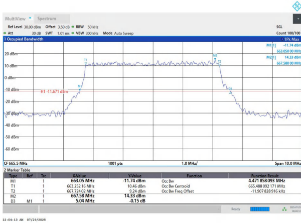
NTNV-n71-PC3-15-5-L-DFT-BPSK-Outter_Full-Ant1-PASS
