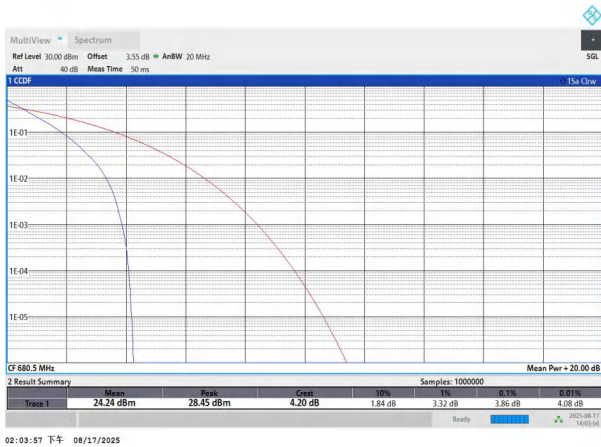
NTNV-n71-PC3-15-20-M-DFT-BPSK-Outer_Full-PASS
