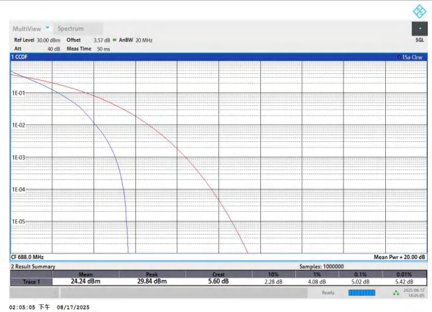
NTNV-n71-PC3-15-20-H-DFT-QPSK-Outer_Full-PASS
