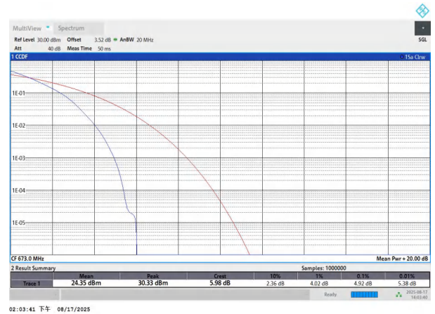
NTNV-n71-PC3-15-20-L-DFT-QPSK-Outer_Full-PASS
