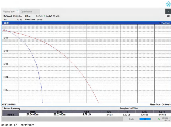
NTNV-n71-PC3-15-20-L-DFT-BPSK-Outer_Full-PASS
