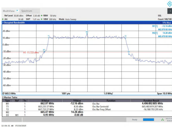
NTNV-n71-PC3-15-5-L-DFT-16QAM-Outter_Full-Ant1-PASS
