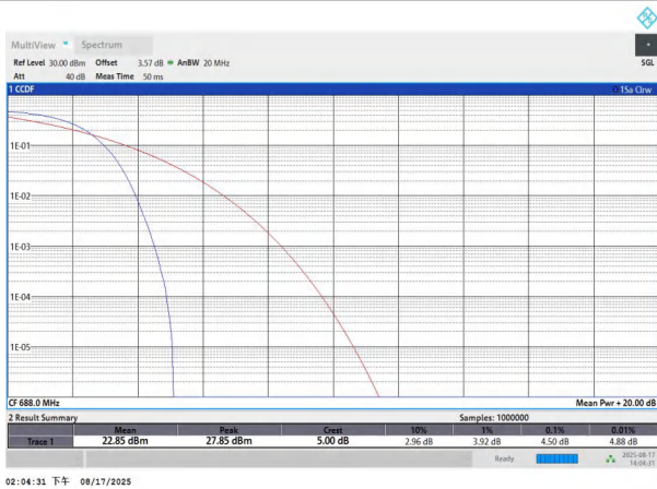
NTNV-n71-PC3-15-20-H-DFT-BPSK-Outer_Full-PASS
