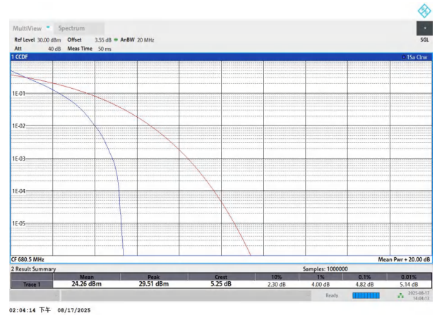
NTNV-n71-PC3-15-20-M-DFT-QPSK-Outer_Full-PASS
