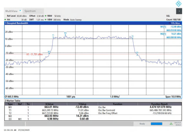
NTNV-n71-PC3-15-5-L-DFT-QPSK-Outter_Full-Ant1-PASS
