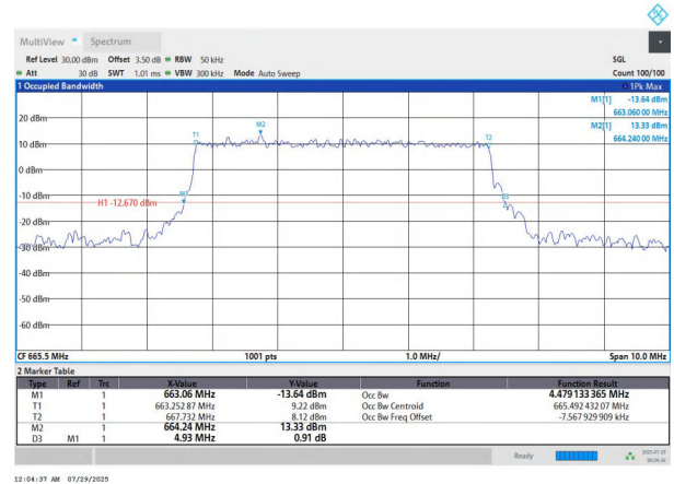
NTNV-n71-PC3-15-5-L-DFT-64QAM-Outter_Full-Ant1-PASS
