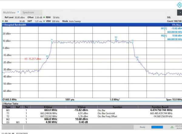
NTNV-n71-PC3-15-5-L-DFT-256QAM-Outter_Full-Ant1-PASS
