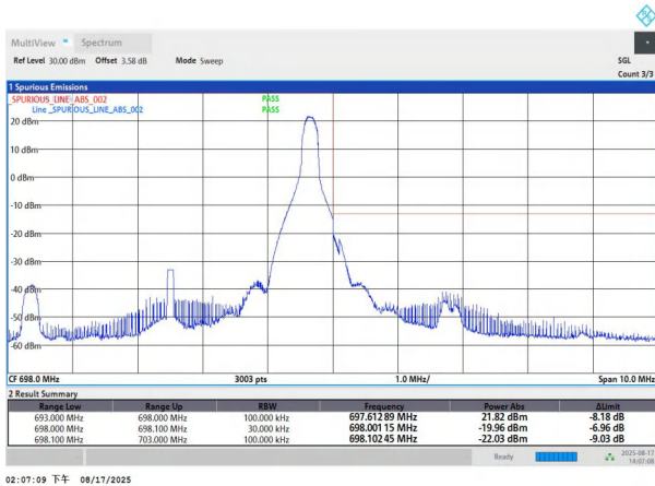
NTNV-n71-PC3-15-5-H-DFT-BPSK-Edge_1RB_Right-PASS
