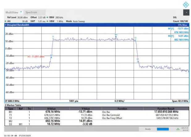
NTNV-n71-PC3-15-20-H-DFT-QPSK-Outter_Full-Ant1-PASS
