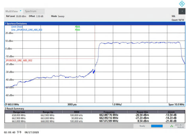
NTNV-n71-PC3-15-5-L-DFT-BPSK-Outer_Full-PASS
