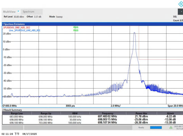
NTNV-n71-PC3-15-15-H-DFT-BPSK-Edge_1RB_Right-PASS
