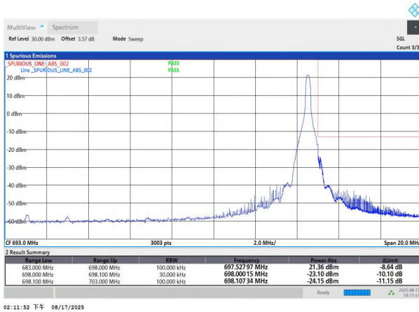
NTNV-n71-PC3-15-15-H-DFT-QPSK-Edge_1RB_Right-PASS
