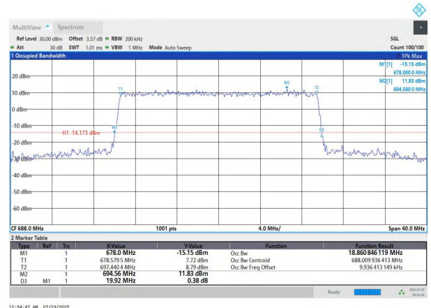
NTNV-n71-PC3-15-20-H-CP-QPSK-Outter_Full-Ant1-PASS
