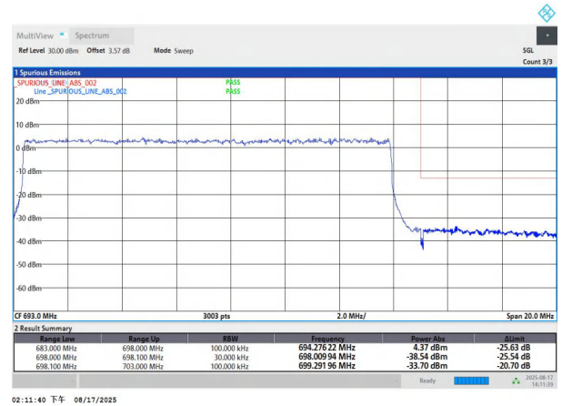
NTNV-n71-PC3-15-15-H-DFT-QPSK-Outer_Full-PASS
