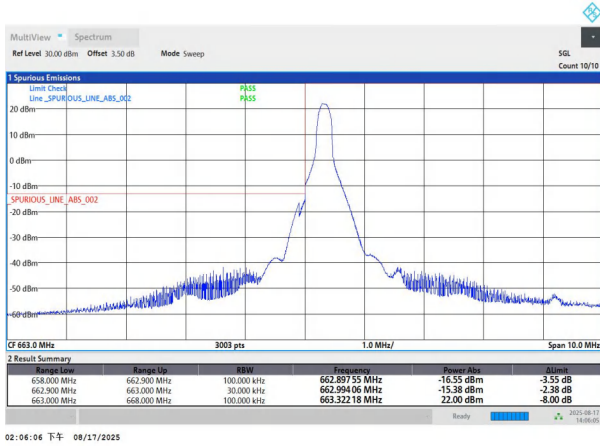
NTNV-n71-PC3-15-5-L-DFT-BPSK-Edge_1RB_Left-PASS
