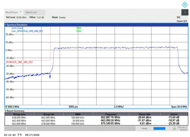
NTNV-n71-PC3-15-15-L-DFT-QPSK-Outer_Full-PASS
