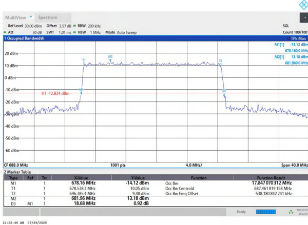
NTNV-n71-PC3-15-20-H-DFT-16QAM-Outter_Full-Ant1-PASS
