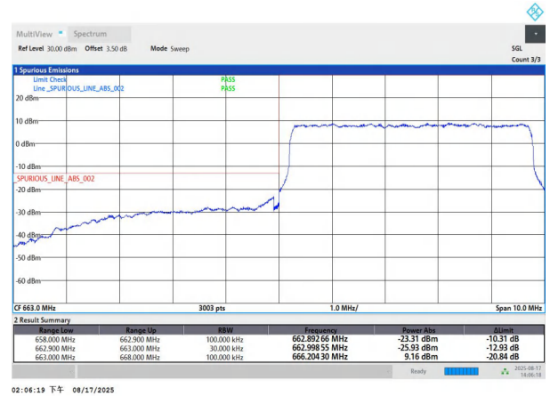
NTNV-n71-PC3-15-5-L-DFT-QPSK-Outer_Full-PASS
