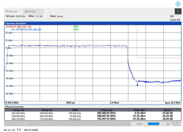
NTNV-n71-PC3-15-15-H-DFT-BPSK-Outer_Full-PASS
