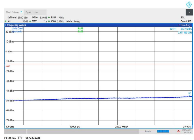
NTNV-n71-PC3-15-15-L-DFT-QPSK-Edge_1RB_Left-1000-3000-P ASS
