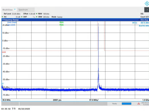
NTNV-n71-PC3-15-15-L-DFT-BPSK-Edge_1RB_Left-30-1000-PA
