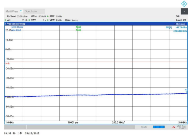
NTNV-n71-PC3-15-15-M-DFT-BPSK-Edge_1RB_Left-1000-3000- PASS
