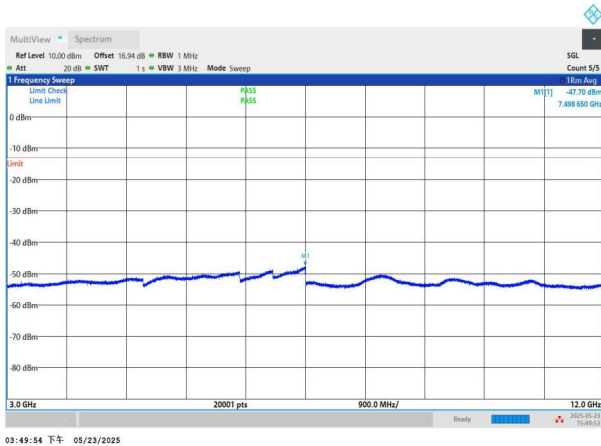
NTNV-n71-PC3-15-20-L-CP-QPSK-Edge_1RB_Left-3000-12000- PASS
