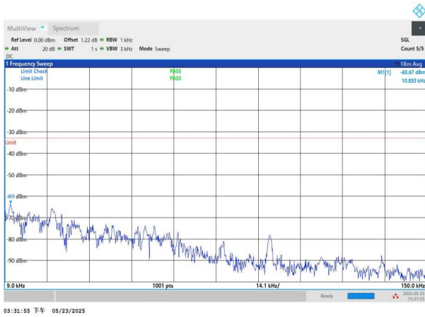
NTNV-n71-PC3-15-10-H-DFT-QPSK-Edge_1RB_Left-0.009-0.15- PASS
