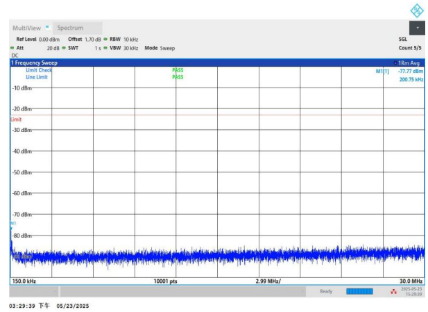
NTNV-n71-PC3-15-10-M-CP-QPSK-Edge_1RB_Left-0.15-30-PAS S
