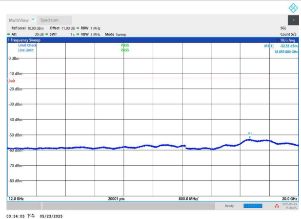
NTNV-n71-PC3-15-10-H-CP-QPSK-Edge_1RB_Left-12000-20000-PASS
