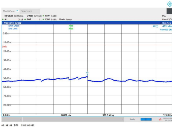
NTNV-n71-PC3-15-15-M-DFT-BPSK-Edge_1RB_Left-3000-1200 0-PASS
