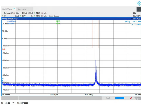
NTNV-n71-PC3-15-15-H-CP-QPSK-Edge_1RB_Left-30-1000-PA SS
