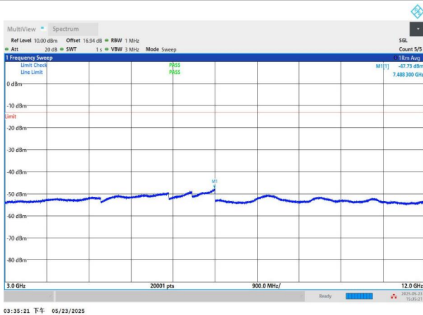
NTNV-n71-PC3-15-15-L-DFT-BPSK-Edge_1RB_Left-3000-12000
