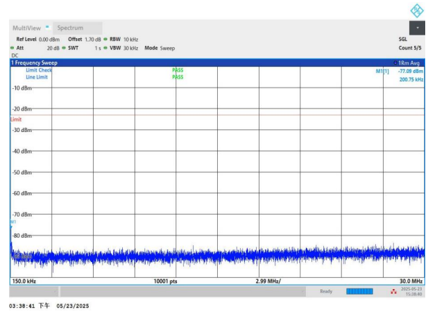
NTNV-n71-PC3-15-15-M-DFT-BPSK-Edge_1RB_Left-0.15-30-PA SS
