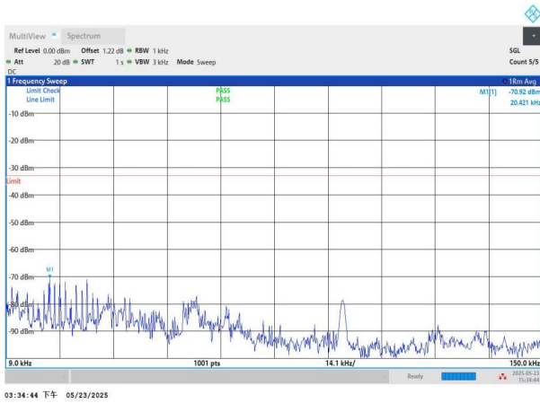
NTNV-n71-PC3-15-15-L-DFT-BPSK-Edge_1RB_Left-0.009-0.15-
