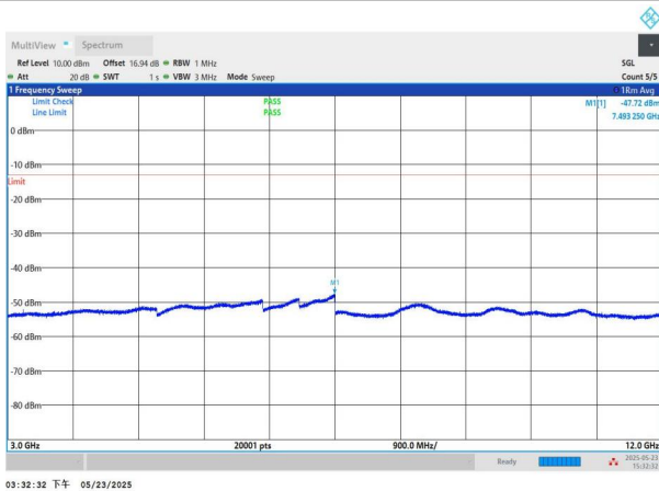
NTNV-n71-PC3-15-10-H-DFT-QPSK-Edge_1RB_Left-3000-1200 0-PASS
