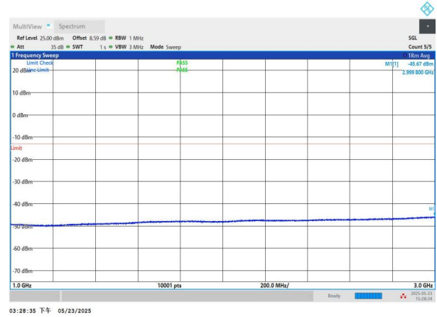
NTNV-n71-PC3-15-10-M-DFT-QPSK-Edge_1RB_Left-1000-3000- PASS
