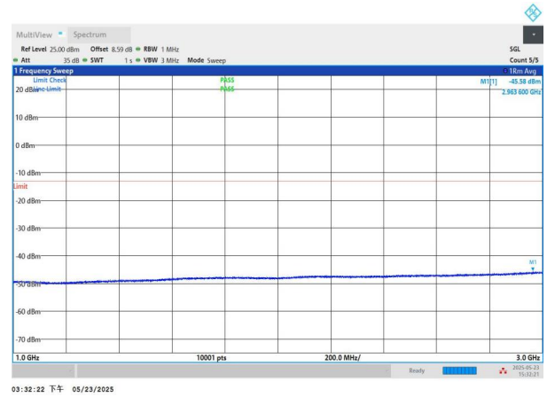
NTNV-n71-PC3-15-10-H-DFT-QPSK-Edge_1RB_Left-1000-3000- PASS
