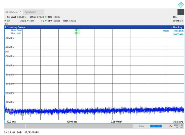
NTNV-n71-PC3-15-10-M-DFT-QPSK-Edge_1RB_Left-0.15-30-PA SS
