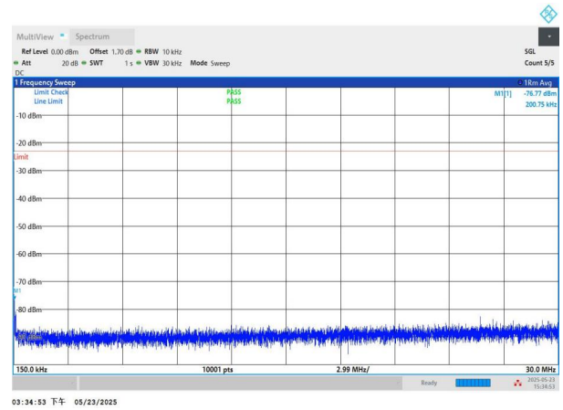
NTNV-n71-PC3-15-15-L-DFT-BPSK-Edge_1RB_Left-0.15-30-PAS
