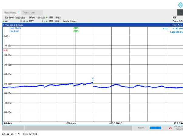
NTNV-n71-PC3-15-15-H-DFT-QPSK-Edge_1RB_Left-3000-1200 0-PASS
