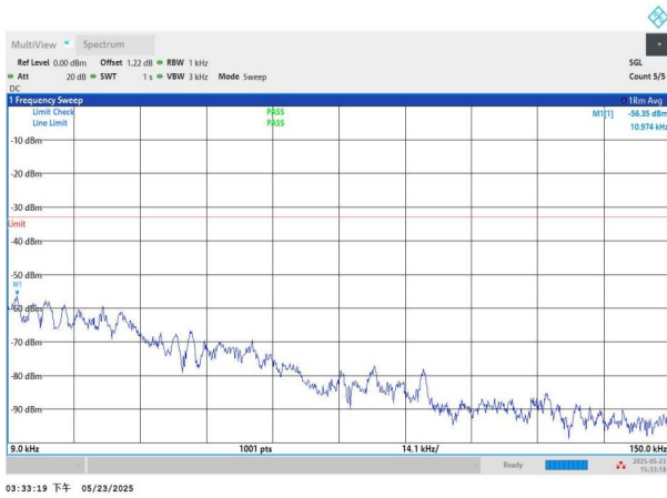
NTNV-n71-PC3-15-10-H-CP-QPSK-Edge_1RB_Left-0.009-0.15-PASS
