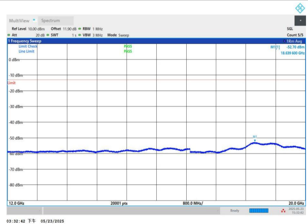
NTNV-n71-PC3-15-10-H-DFT-QPSK-Edge_1RB_Left-12000-2000 0-PASS
