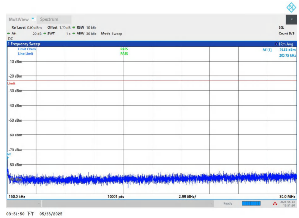
NTNV-n71-PC3-15-20-M-DFT-QPSK-Edge_1RB_Left-0.15-30-PA SS
