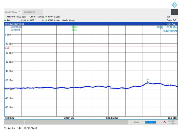
NTNV-n71-PC3-15-15-H-DFT-QPSK-Edge_1RB_Left-12000-2000 0-PASS
