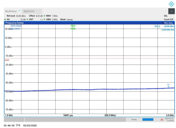
NTNV-n71-PC3-15-15-H-DFT-QPSK-Edge_1RB_Left-1000-3000- PASS
