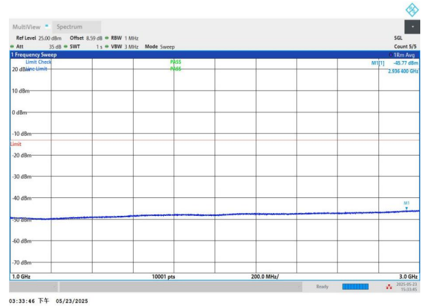
NTNV-n71-PC3-15-10-H-CP-QPSK-Edge_1RB_Left-1000-3000-PASS
