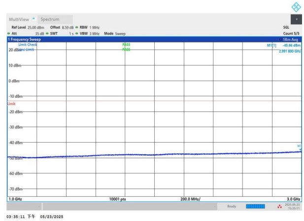
NTNV-n71-PC3-15-15-L-DFT-BPSK-Edge_1RB_Left-1000-3000-P
