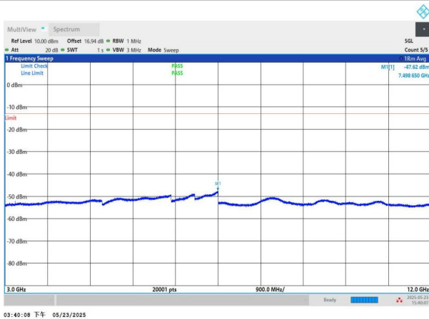
NTNV-n71-PC3-15-15-M-DFT-QPSK-Edge_1RB_Left-3000-1200 0-PASS
