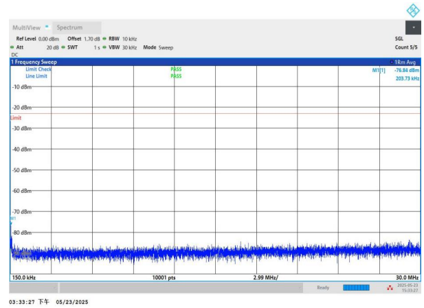
NTNV-n71-PC3-15-10-H-CP-QPSK-Edge_1RB_Left-0.15-30-PASS
