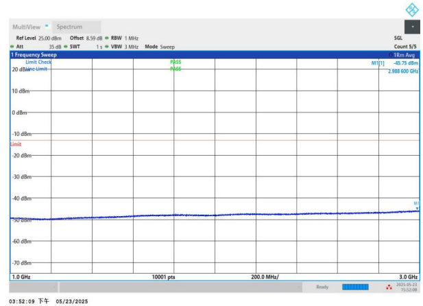
NTNV-n71-PC3-15-20-M-DFT-QPSK-Edge_1RB_Left-1000-3000- PASS
