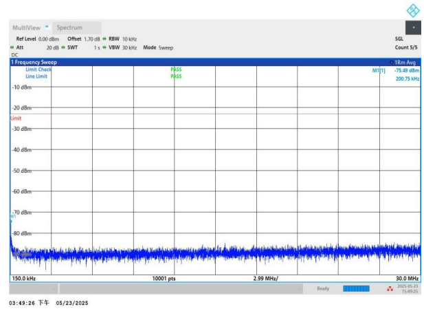
NTNV-n71-PC3-15-20-L-CP-QPSK-Edge_1RB_Left-0.15-30-PAS S
