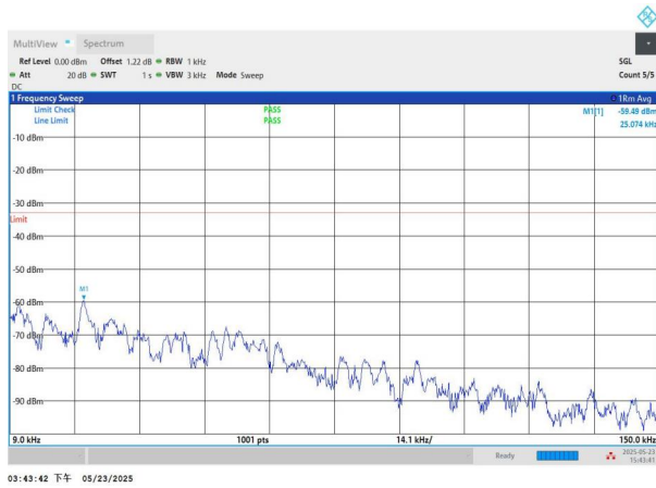
NTNV-n71-PC3-15-15-H-DFT-QPSK-Edge_1RB_Left-0.009-0.15- PASS
