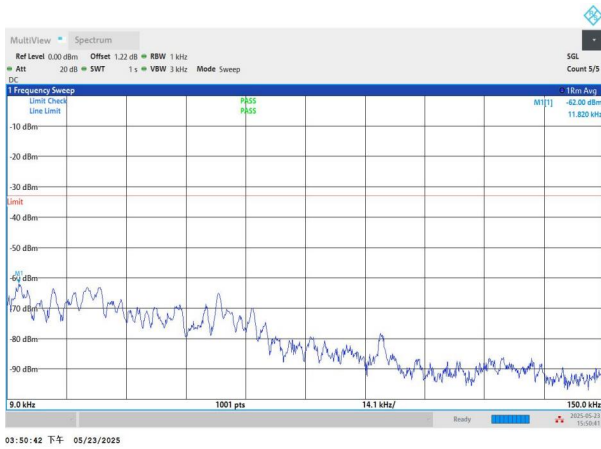
NTNV-n71-PC3-15-20-M-DFT-BPSK-Edge_1RB_Left-0.009-0.15- PASS
