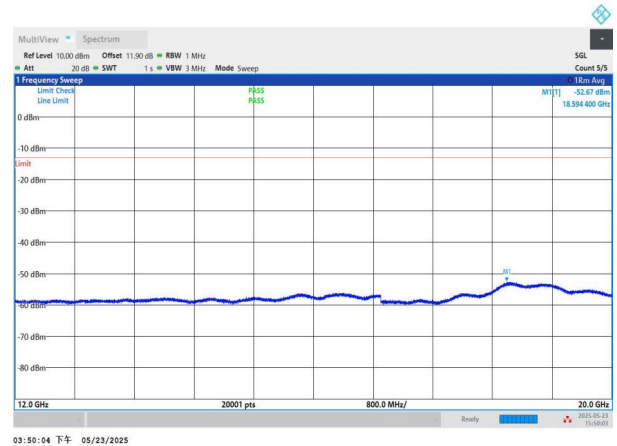
NTNV-n71-PC3-15-20-L-CP-QPSK-Edge_1RB_Left-12000-20000- PASS
