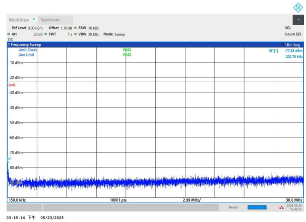
NTNV-n71-PC3-15-15-H-CP-QPSK-Edge_1RB_Left-0.15-30-PAS S
