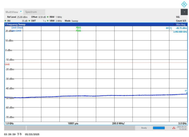
NTNV-n71-PC3-15-15-M-DFT-QPSK-Edge_1RB_Left-1000-3000- PASS
