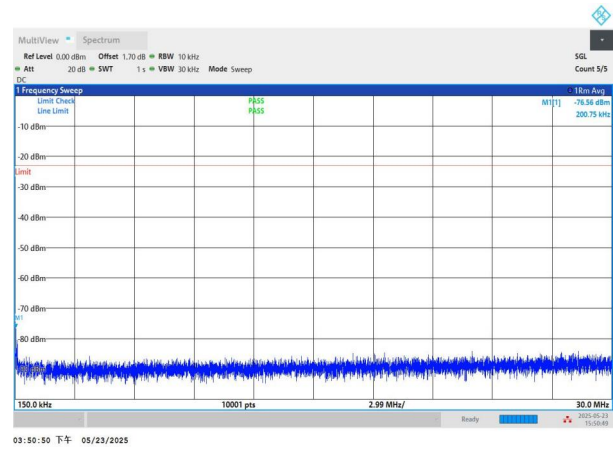
NTNV-n71-PC3-15-20-M-DFT-BPSK-Edge_1RB_Left-0.15-30-PA SS
