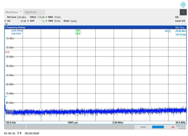
NTNV-n71-PC3-15-15-H-DFT-QPSK-Edge_1RB_Left-0.15-30-PA SS
