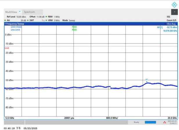
NTNV-n71-PC3-15-15-M-DFT-QPSK-Edge_1RB_Left-12000-2000 0-PASS
