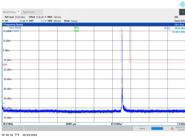
NTNV-n71-PC3-15-15-L-DFT-QPSK-Edge_1RB_Left-30-1000-PA SS
