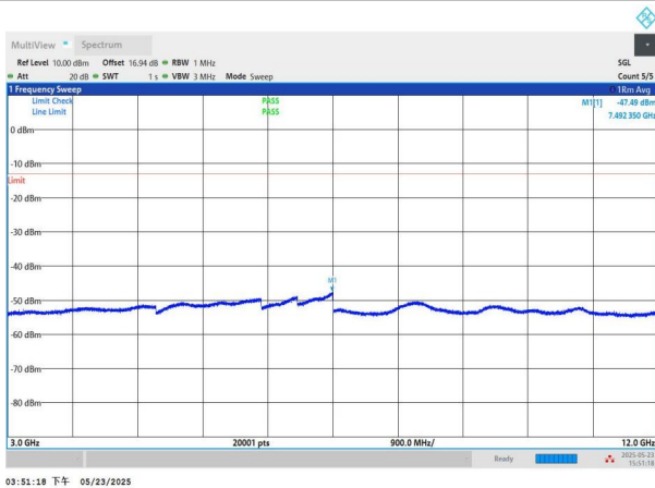
NTNV-n71-PC3-15-20-M-DFT-BPSK-Edge_1RB_Left-3000-1200 0-PASS
