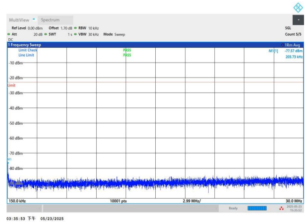
NTNV-n71-PC3-15-15-L-DFT-QPSK-Edge_1RB_Left-0.15-30-PAS S
