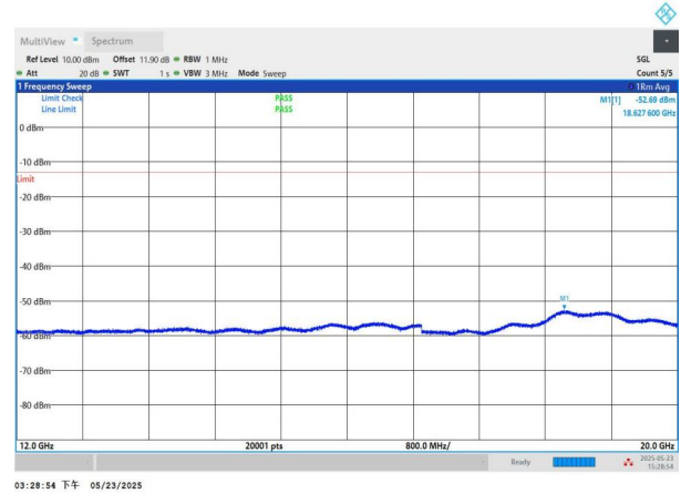
NTNV-n71-PC3-15-10-M-DFT-QPSK-Edge_1RB_Left-12000-2000 0-PASS
