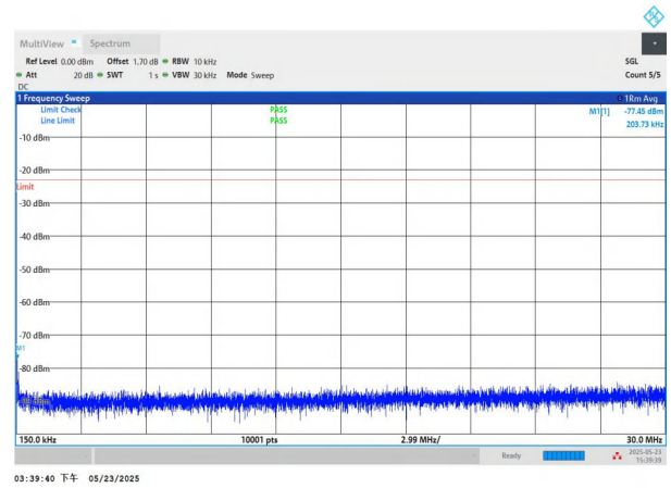
NTNV-n71-PC3-15-15-M-DFT-QPSK-Edge_1RB_Left-0.15-30-PA SS
