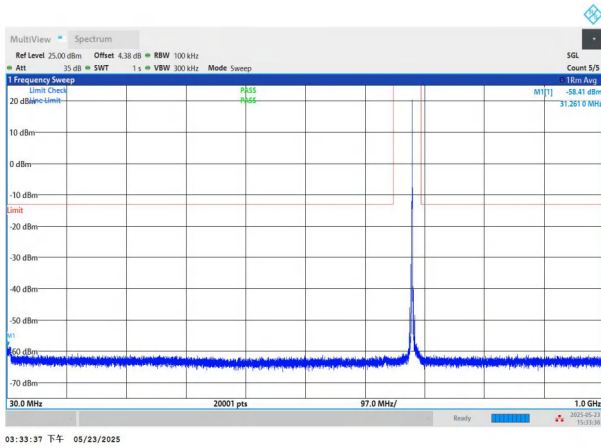
NTNV-n71-PC3-15-10-H-CP-QPSK-Edge_1RB_Left-30-1000-PA
