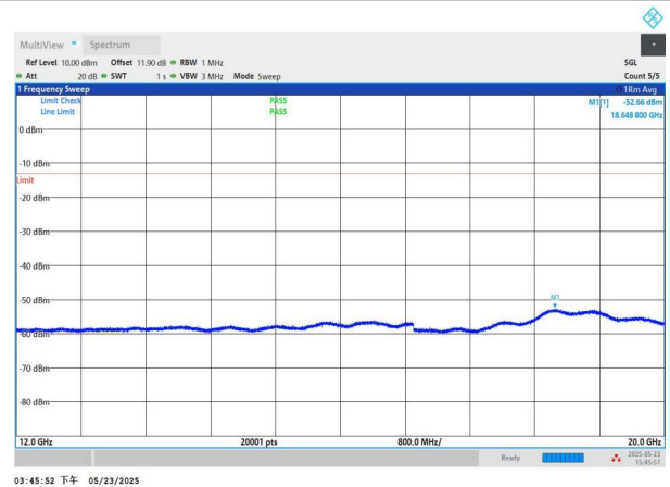
NTNV-n71-PC3-15-15-H-CP-QPSK-Edge_1RB_Left-12000-20000 -PASS
