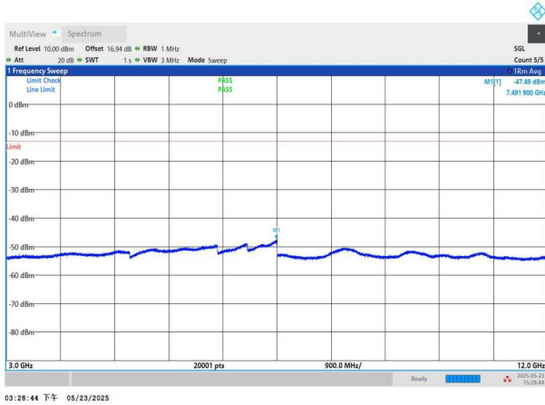
NTNV-n71-PC3-15-10-M-DFT-QPSK-Edge_1RB_Left-3000-1200 0-PASS
