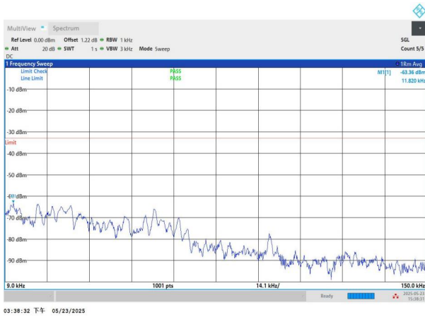
NTNV-n71-PC3-15-15-M-DFT-BPSK-Edge_1RB_Left-0.009-0.15- PASS
