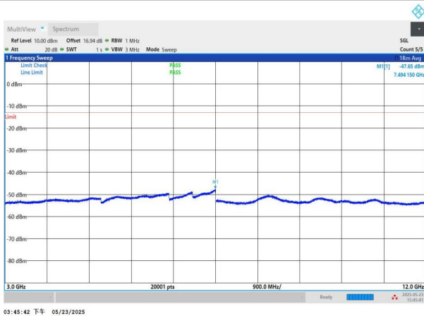
NTNV-n71-PC3-15-15-H-CP-QPSK-Edge_1RB_Left-3000-12000 -PASS
