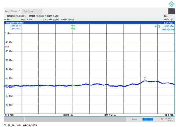
NTNV-n71-PC3-15-15-M-DFT-BPSK-Edge_1RB_Left-12000-2000 0-PASS
