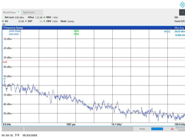
NTNV-n71-PC3-15-10-M-CP-QPSK-Edge_1RB_Left-0.009-0.15- PASS
