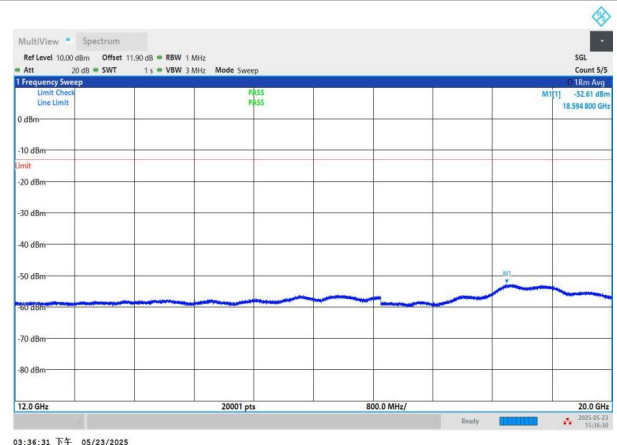
NTNV-n71-PC3-15-15-L-DFT-QPSK-Edge_1RB_Left-12000-2000 0-PASS
