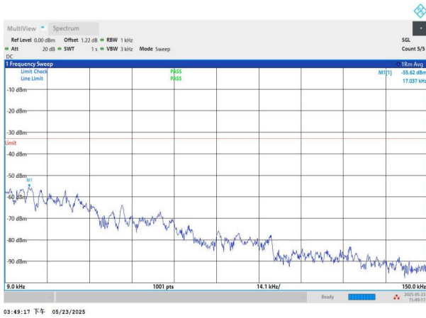
NTNV-n71-PC3-15-20-L-CP-QPSK-Edge_1RB_Left-0.009-0.15-P ASS
