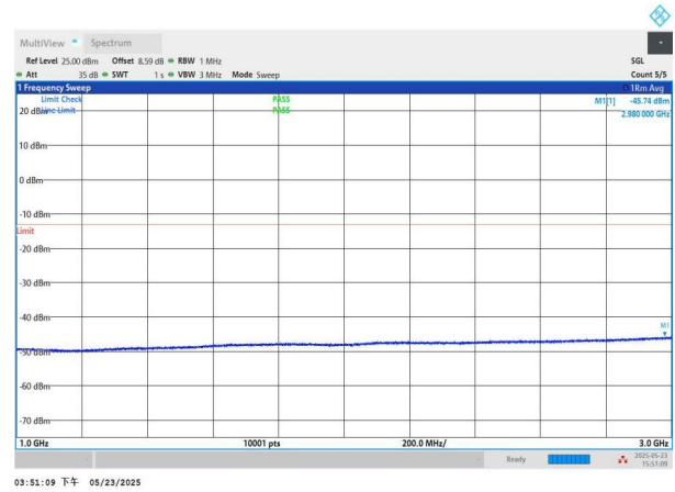
NTNV-n71-PC3-15-20-M-DFT-BPSK-Edge_1RB_Left-1000-3000- PASS
