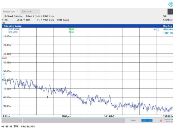
NTNV-n71-PC3-15-15-H-CP-QPSK-Edge_1RB_Left-0.009-0.15- PASS
