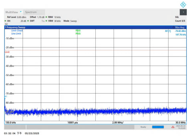
NTNV-n71-PC3-15-10-H-DFT-QPSK-Edge_1RB_Left-0.15-30-PA- SS
