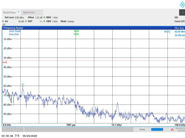
NTNV-n71-PC3-15-15-L-DFT-QPSK-Edge_1RB_Left-0.009-0.15- PASS
