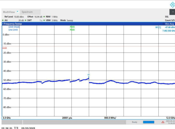
NTNV-n71-PC3-15-15-L-DFT-QPSK-Edge_1RB_Left-3000-1200 0-PASS
