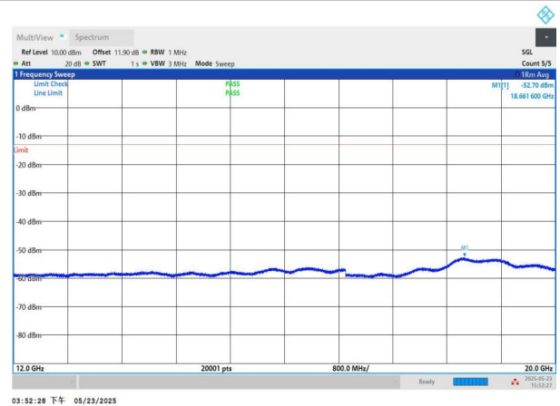
NTNV-n71-PC3-15-20-M-DFT-QPSK-Edge_1RB_Left-12000-2000 0-PASS
