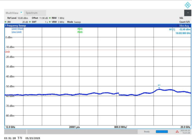
NTNV-n71-PC3-15-20-M-DFT-BPSK-Edge_1RB_Left-12000-2000 0-PASS
