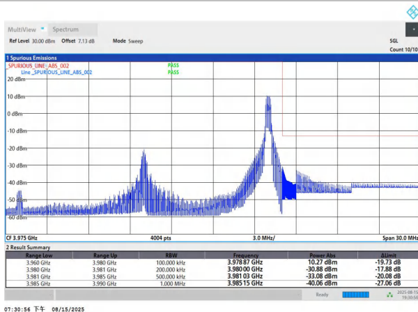
NTNV-n77(3700-3980)-PC2-30-20-H-DFT-BPSK-Edge_1RB_Right-P ASS
