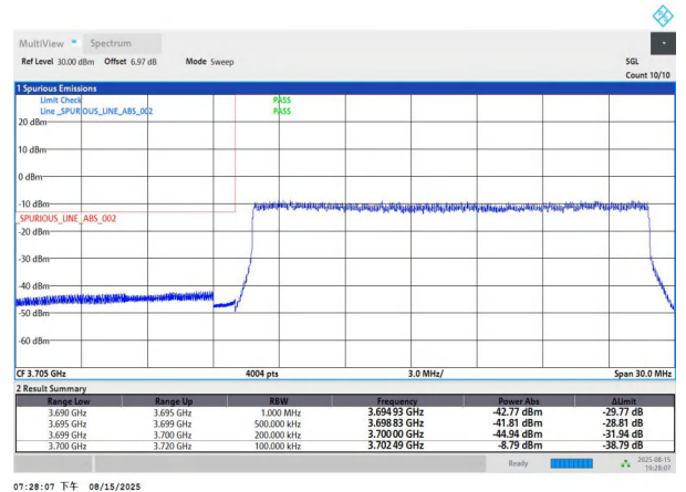
NTNV-n77(3700-3980)-PC2-30-20-L-DFT-QPSK-Outer_Full-P ASS
