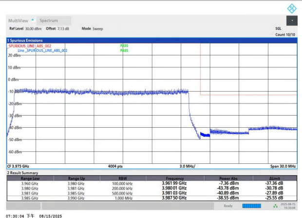
NTNV-n77(3700-3980)-PC2-30-20-H-DFT-BPSK-Outer_Full-P ASS
