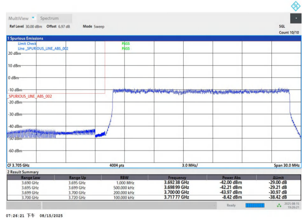
NTNV-n77(3700-3980)-PC2-30-20-L-DFT-BPSK-Outer_Full-P ASS
