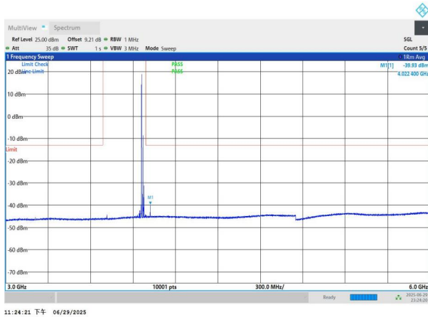
NTNV-n77(3700-3980)-PC2-30-20-H-DFT-BPSK-Edge_1RB_Left -3000-6000-PASS
