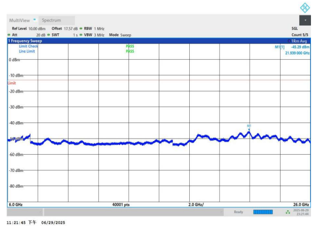
NTNV-n77(3700-3980)-PC2-30-20-M-DFT-BPSK-Edge_1RB_Left -6000-26000-PASS
