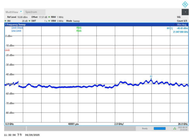
NTNV-n77(3700-3980)-PC2-30-30-H-DFT-BPSK-Edge_1RB_Left 6000-26000-PASS
