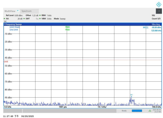
NTNV-n77(3700-3980)-PC2-30-30-L-DFT-QPSK-Edge_1RB_Left- 0.009-0.15-PASS
