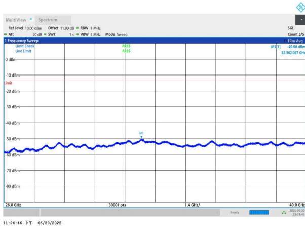
NTNV-n77(3700-3980)-PC2-30-20-H-DFT-BPSK-Edge_1RB_Left -26000-40000-PASS
