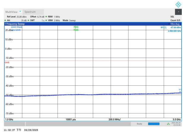
NTNV-n77(3700-3980)-PC2-30-30-H-DFT-BPSK-Edge_1RB_Left 1000-3000-PASS
