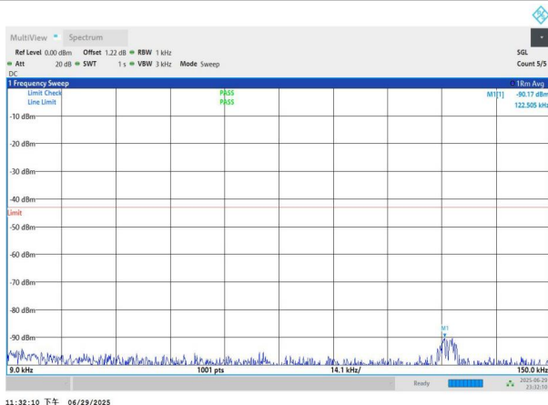
NTNV-n77(3700-3980)-PC2-30-30-H-DFT-BPSK-Edge_1RB_Left -0.009-0.15-PASS
