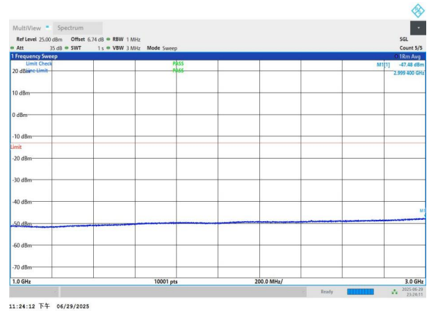
NTNV-n77(3700-3980)-PC2-30-20-H-DFT-BPSK-Edge_1RB_Left 1000-3000-PASS
