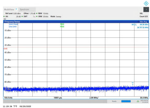
NTNV-n77(3700-3980)-PC2-30-30-M-DFT-BPSK-Edge_1RB_Left -0.15-30-PASS
