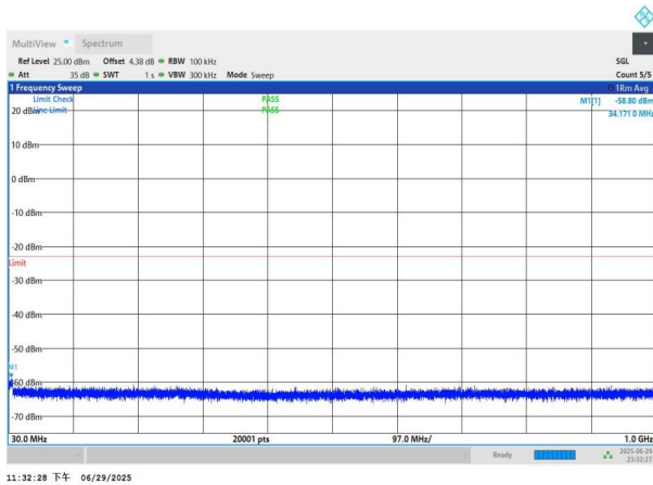
NTNV-n77(3700-3980)-PC2-30-30-H-DFT-BPSK-Edge_1RB_Left -30-1000-PASS
