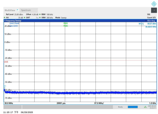
NTNV-n77(3700-3980)-PC2-30-20-H-DFT-QPSK-Edge_1RB_Left -30-1000-PASS
