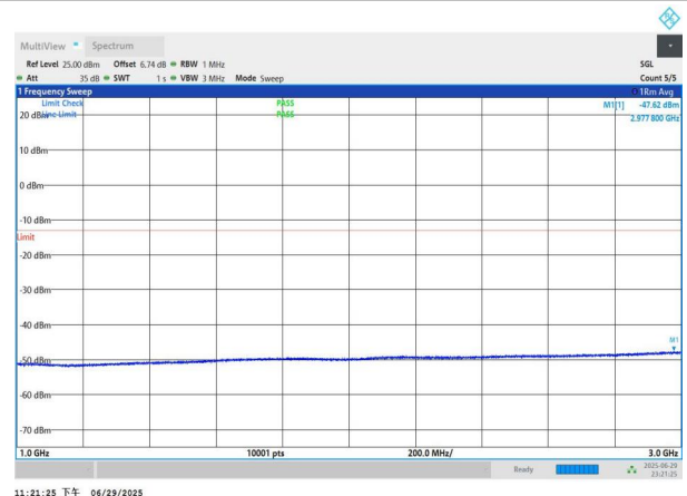
NTNV-n77(3700-3980)-PC2-30-20-M-DFT-BPSK-Edge_1RB_Left -1000-3000-PASS
