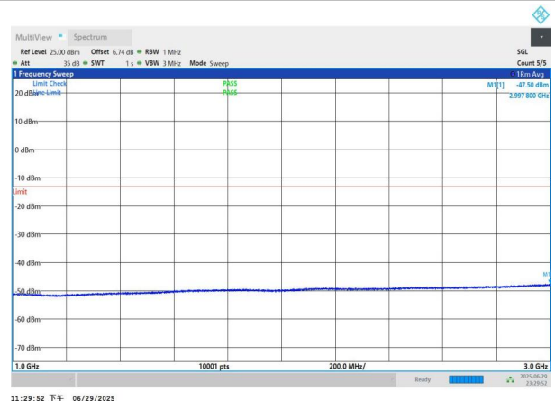
NTNV-n77(3700-3980)-PC2-30-30-M-DFT-BPSK-Edge_1RB_Left -1000-3000-PASS
