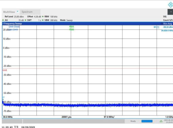
NTNV-n77(3700-3980)-PC2-30-30-M-DFT-BPSK-Edge_1RB_Left -30-1000-PASS
