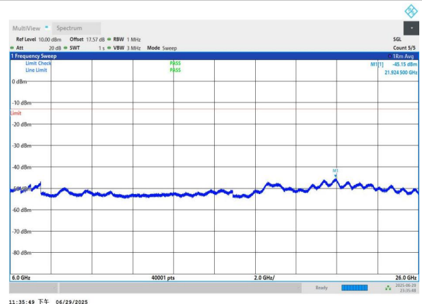
NTNV-n77(3700-3980)-PC2-30-40-L-DFT-BPSK-Edge_1RB_Left- 6000-26000-PASS
