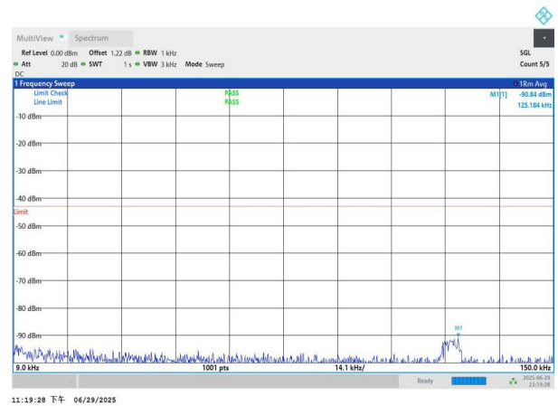
NTNV-n77(3700-3980)-PC2-30-20-L-DFT-QPSK-Edge_1RB_Left- 0.009-0.15-PASS
