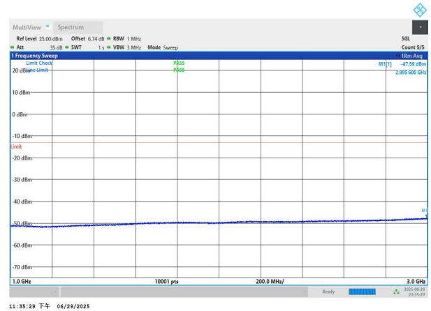
NTNV-n77(3700-3980)-PC2-30-40-L-DFT-BPSK-Edge_1RB_Left- 1000-3000-PASS
