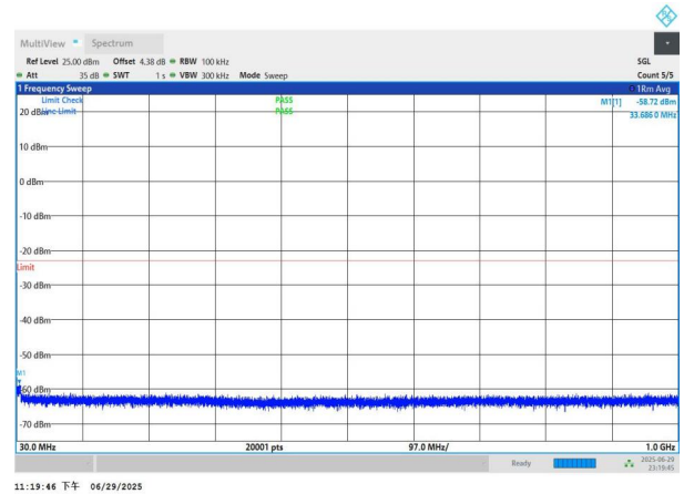
NTNV-n77(3700-3980)-PC2-30-20-L-DFT-QPSK-Edge_1RB_Left- 30-1000-PASS
