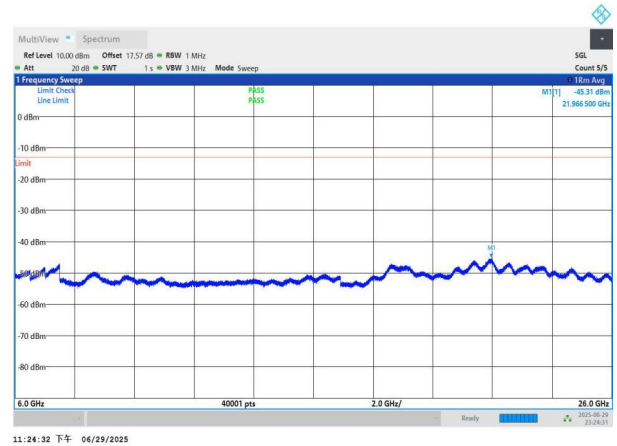
NTNV-n77(3700-3980)-PC2-30-20-H-DFT-BPSK-Edge_1RB_Left 6000-26000-PASS
