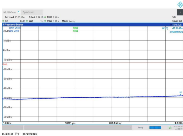
NTNV-n77(3700-3980)-PC2-30-20-M-DFT-QPSK-Edge_1RB_Left -1000-3000-PASS
