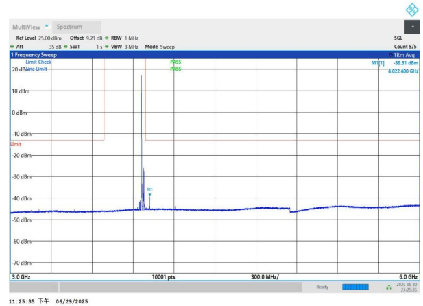
NTNV-n77(3700-3980)-PC2-30-20-H-DFT-QPSK-Edge_1RB_Left -3000-6000-PASS
