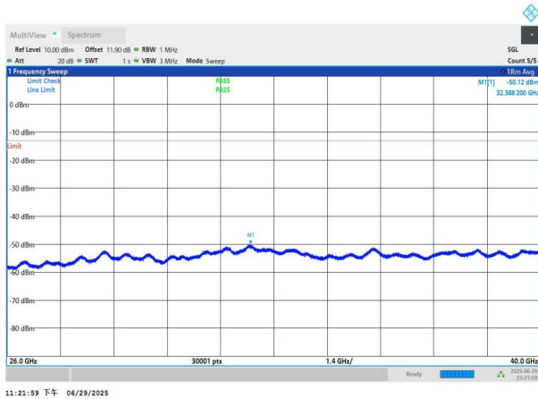
NTNV-n77(3700-3980)-PC2-30-20-M-DFT-BPSK-Edge_1RB_Left -26000-40000-PASS
