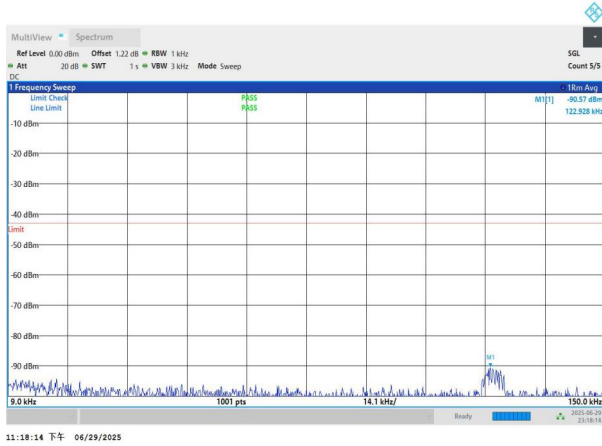
NTNV-n77(3700-3980)-PC2-30-20-L-DFT-BPSK-Edge_1RB_Left- 0.009-0.15-PASS
