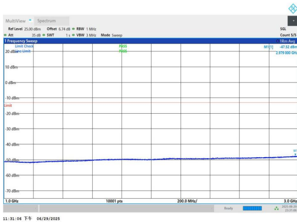
NTNV-n77(3700-3980)-PC2-30-30-M-DFT-QPSK-Edge_1RB_Left -1000-3000-PASS
