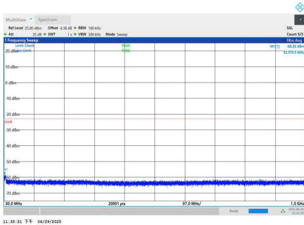
NTNV-n77(3700-3980)-PC2-30-40-L-DFT-BPSK-Edge_1RB_Left- 30-1000-PASS
