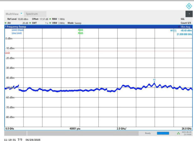
NTNV-n77(3700-3980)-PC2-30-20-L-DFT-BPSK-Edge_1RB_Left- 6000-26000-PASS
