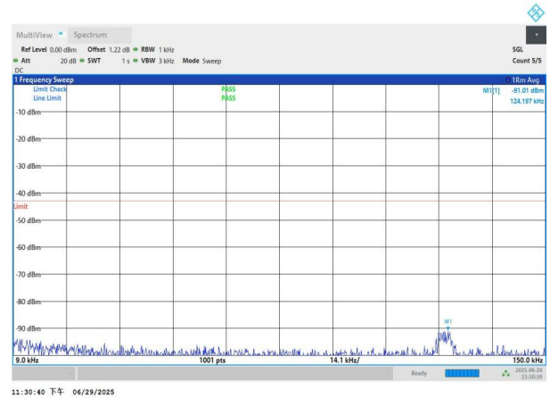
NTNV-n77(3700-3980)-PC2-30-30-M-DFT-QPSK-Edge_1RB_Left -0.009-0.15-PASS
