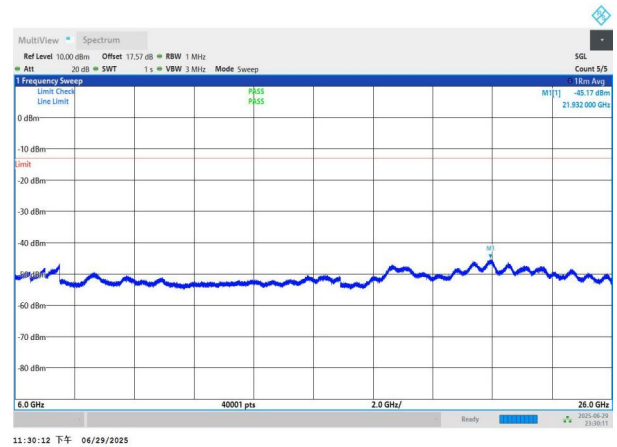
NTNV-n77(3700-3980)-PC2-30-30-M-DFT-BPSK-Edge_1RB_Left -6000-26000-PASS
