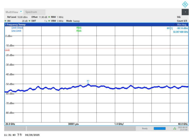
NTNV-n77(3700-3980)-PC2-30-30-M-DFT-QPSK-Edge_1RB_Left -26000-40000-PASS
