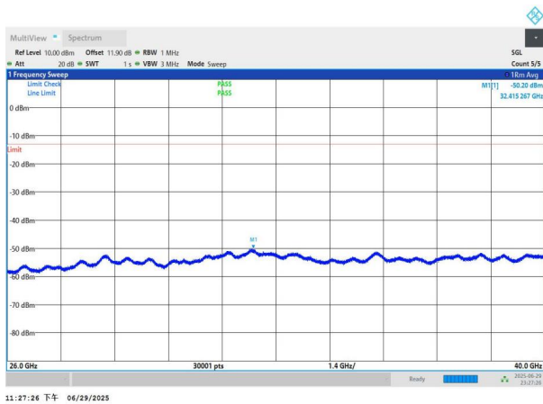
NTNV-n77(3700-3980)-PC2-30-30-L-DFT-BPSK-Edge_1RB_Left- 26000-40000-PASS
