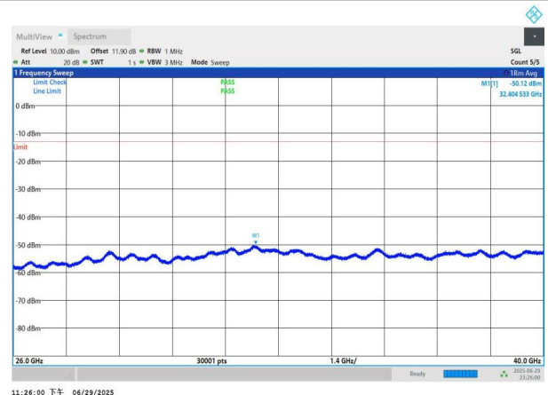
NTNV-n77(3700-3980)-PC2-30-20-H-DFT-QPSK-Edge_1RB_Left -26000-40000-PASS
