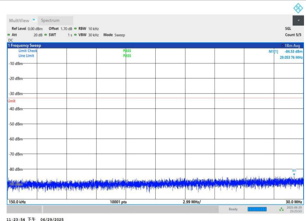
NTNV-n77(3700-3980)-PC2-30-20-H-DFT-BPSK-Edge_1RB_Left 0.15-30-PASS
