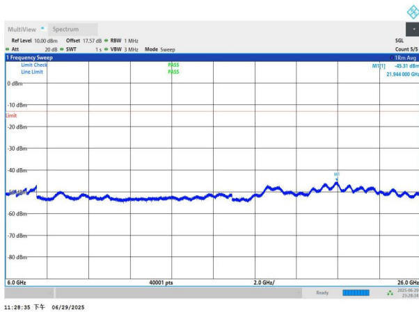
NTNV-n77(3700-3980)-PC2-30-30-L-DFT-QPSK-Edge_1RB_Left- 6000-26000-PASS
