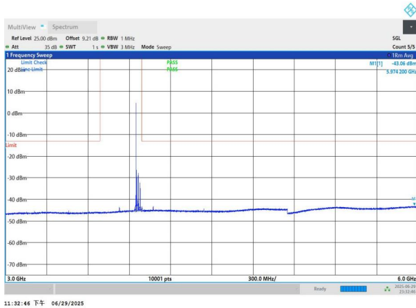
NTNV-n77(3700-3980)-PC2-30-30-H-DFT-BPSK-Edge_1RB_Left -3000-6000-PASS
