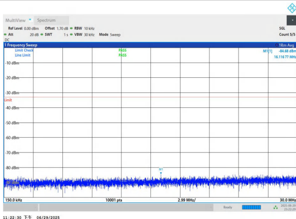
NTNV-n77(3700-3980)-PC2-30-20-M-DFT-QPSK-Edge_1RB_Left -0.15-30-PASS
