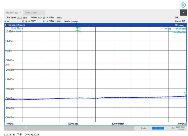
NTNV-n77(3700-3980)-PC2-30-20-L-DFT-BPSK-Edge_1RB_Left- 1000-3000-PASS
