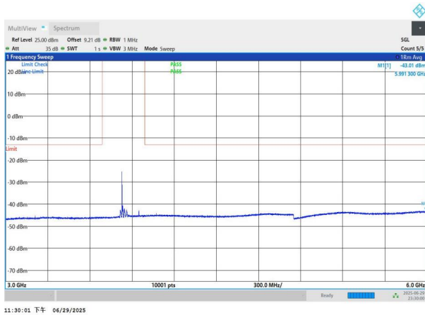
NTNV-n77(3700-3980)-PC2-30-30-M-DFT-BPSK-Edge_1RB_Left -3000-6000-PASS
