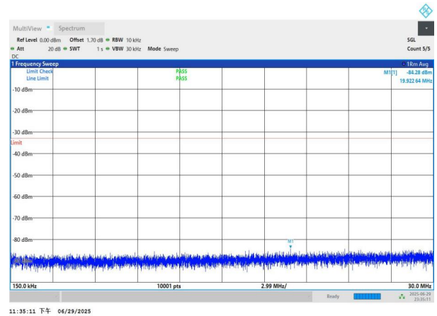
NTNV-n77(3700-3980)-PC2-30-40-L-DFT-BPSK-Edge_1RB_Left- 0.15-30-PASS
