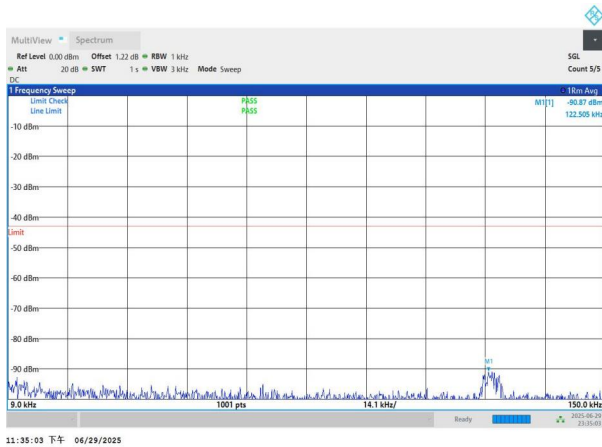
NTNV-n77(3700-3980)-PC2-30-40-L-DFT-BPSK-Edge_1RB_Left- 0.009-0.15-PASS
