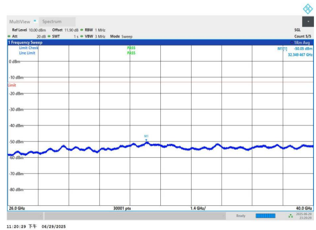
NTNV-n77(3700-3980)-PC2-30-20-L-DFT-QPSK-Edge_1RB_Left- 26000-40000-PASS
