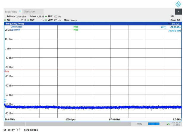
NTNV-n77(3700-3980)-PC2-30-30-L-DFT-QPSK-Edge_1RB_Left- 30-1000-PASS
