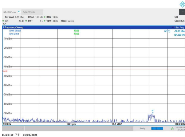
NTNV-n77(3700-3980)-PC2-30-20-M-DFT-BPSK-Edge_1RB_Left -0.009-0.15-PASS
