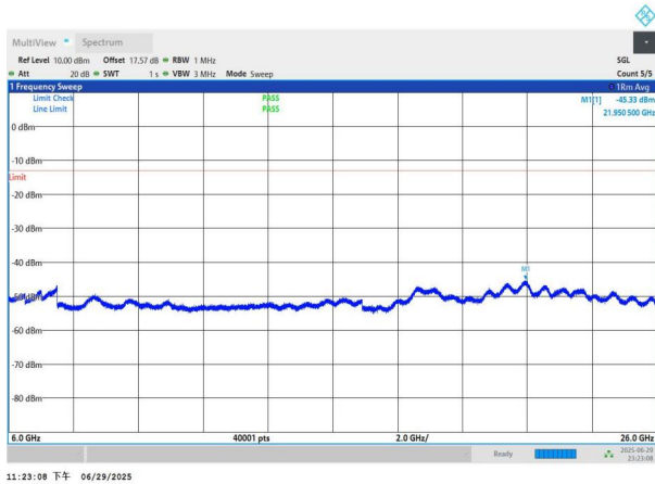
NTNV-n77(3700-3980)-PC2-30-20-M-DFT-QPSK-Edge_1RB_Left -6000-26000-PASS
