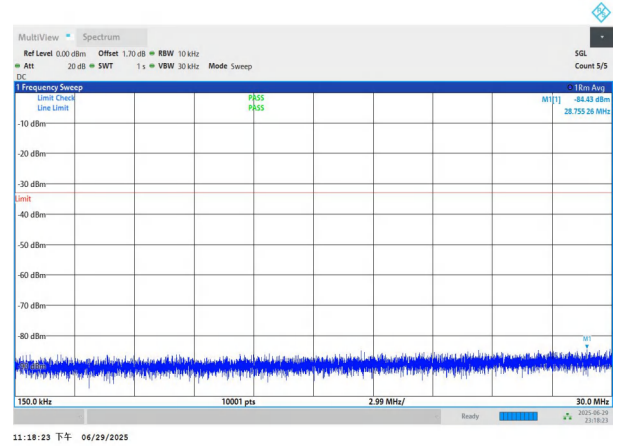
NTNV-n77(3700-3980)-PC2-30-20-L-DFT-BPSK-Edge_1RB_Left- 0.15-30-PASS
