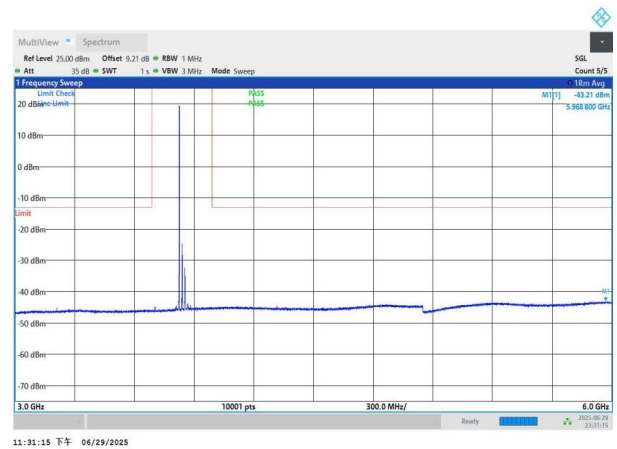
NTNV-n77(3700-3980)-PC2-30-30-M-DFT-QPSK-Edge_1RB_Left -3000-6000-PASS
