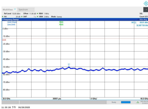
NTNV-n77(3700-3980)-PC2-30-30-M-DFT-BPSK-Edge_1RB_Left -26000-40000-PASS
