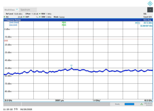
NTNV-n77(3700-3980)-PC2-30-20-M-DFT-QPSK-Edge_1RB_Left -26000-40000-PASS
