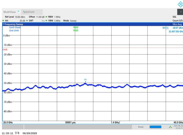
NTNV-n77(3700-3980)-PC2-30-30-H-DFT-BPSK-Edge_1RB_Left -26000-40000-PASS
