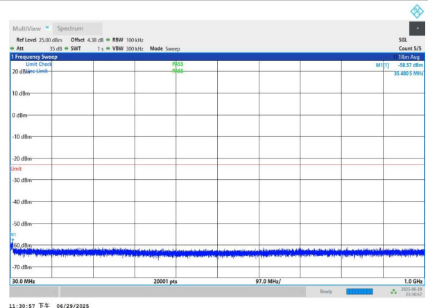
NTNV-n77(3700-3980)-PC2-30-30-M-DFT-QPSK-Edge_1RB_Left -30-1000-PASS
