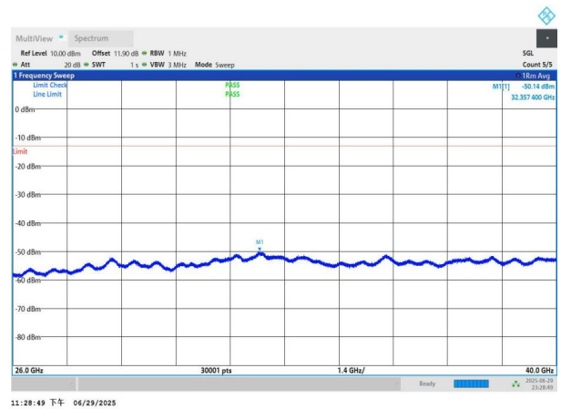
NTNV-n77(3700-3980)-PC2-30-30-L-DFT-QPSK-Edge_1RB_Left- 26000-40000-PASS
