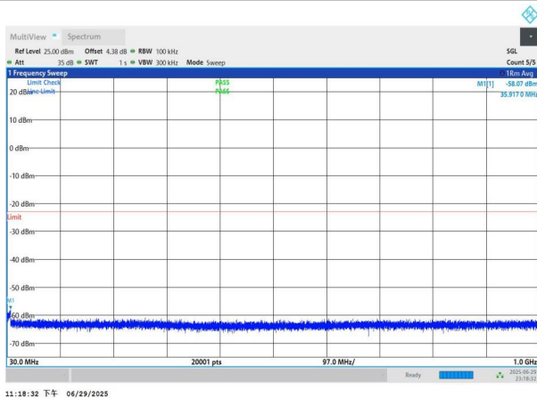
NTNV-n77(3700-3980)-PC2-30-20-L-DFT-BPSK-Edge_1RB_Left- 30-1000-PASS
