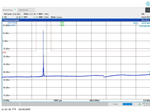
NTNV-n77(3700-3980)-PC2-30-20-M-DFT-BPSK-Edge_1RB_Left -3000-6000-PASS
