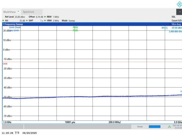
NTNV-n77(3700-3980)-PC2-30-20-H-DFT-QPSK-Edge_1RB_Left -1000-3000-PASS
