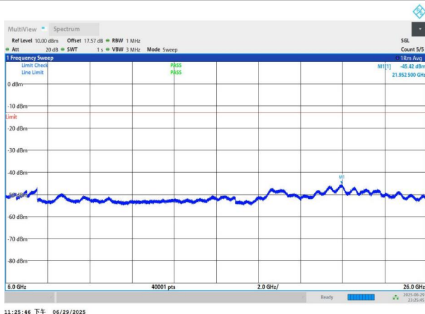
NTNV-n77(3700-3980)-PC2-30-20-H-DFT-QPSK-Edge_1RB_Left -6000-26000-PASS
