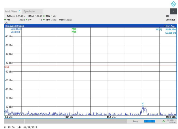
NTNV-n77(3700-3980)-PC2-30-20-H-DFT-QPSK-Edge_1RB_Left -0.009-0.15-PASS
