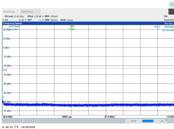
NTNV-n77(3700-3980)-PC2-30-20-H-DFT-BPSK-Edge_1RB_Left -30-1000-PASS
