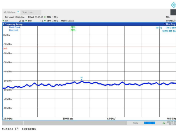
NTNV-n77(3700-3980)-PC2-30-20-L-DFT-BPSK-Edge_1RB_Left- 26000-40000-PASS
