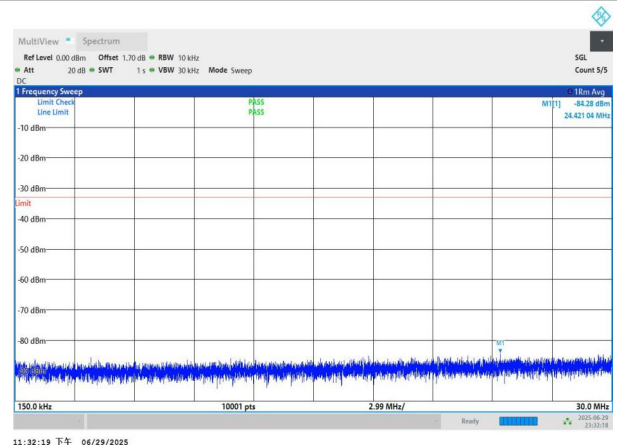
NTNV-n77(3700-3980)-PC2-30-30-H-DFT-BPSK-Edge_1RB_Left 0.15-30-PASS
