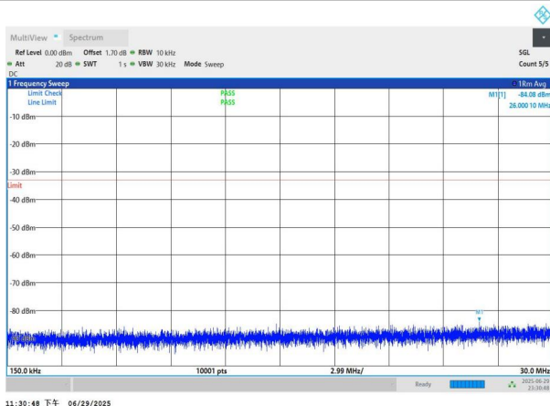
NTNV-n77(3700-3980)-PC2-30-30-M-DFT-QPSK-Edge_1RB_Left -0.15-30-PASS
