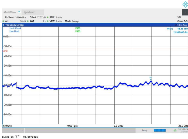
NTNV-n77(3700-3980)-PC2-30-30-M-DFT-QPSK-Edge_1RB_Left -6000-26000-PASS
