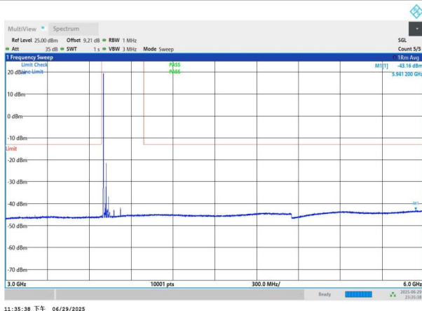
NTNV-n77(3700-3980)-PC2-30-40-L-DFT-BPSK-Edge_1RB_Left- 3000-6000-PASS
