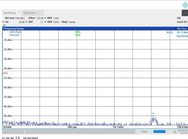
NTNV-n77(3700-3980)-PC2-30-20-H-DFT-BPSK-Edge_1RB_Left -0.009-0.15-PASS
