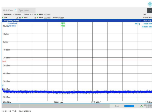
NTNV-n77(3700-3980)-PC2-30-20-M-DFT-BPSK-Edge_1RB_Left -30-1000-PASS
