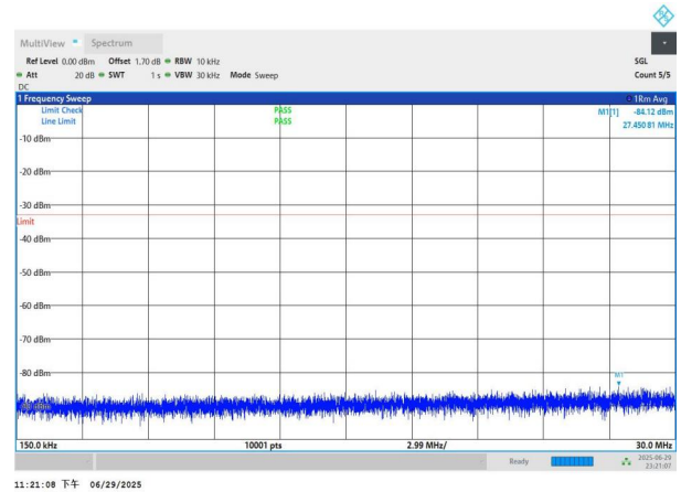
NTNV-n77(3700-3980)-PC2-30-20-M-DFT-BPSK-Edge_1RB_Left -0.15-30-PASS
