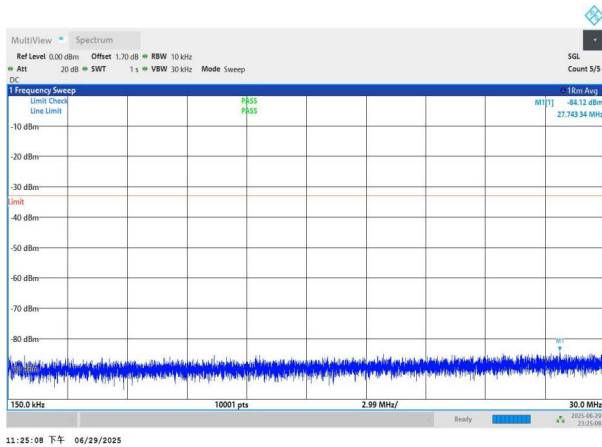
NTNV-n77(3700-3980)-PC2-30-20-H-DFT-QPSK-Edge_1RB_Left -0.15-30-PASS
