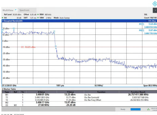
NTNV-n77(3450-3550)-PC2-30-40-H-DFT-BPSK-Outer_Full-Ant1 -PASS
