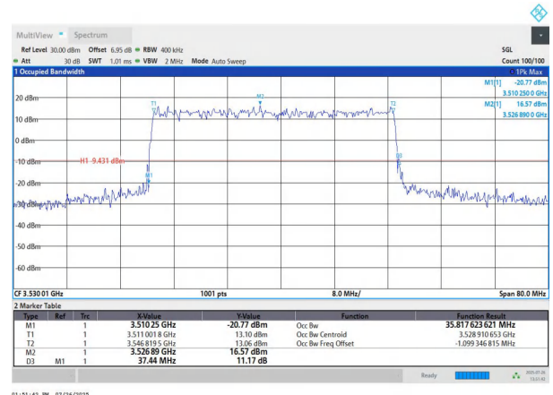
NTNV-n77(3450-3550)-PC2-30-40-H-DFT-QPSK-Outer_Full-Ant1 PASS
