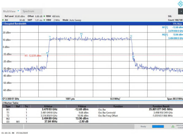
NTNV-n77(3450-3550)-PC2-30-40-M-DFT-64QAM-Outer_Full-An t1-PASS
